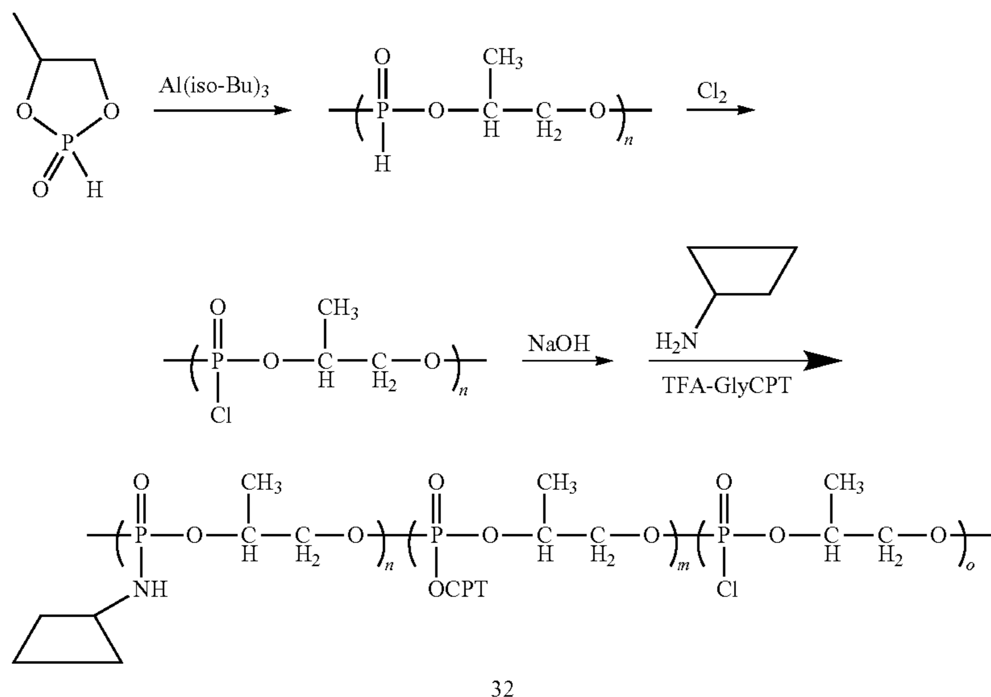
Scheme XXXIV
