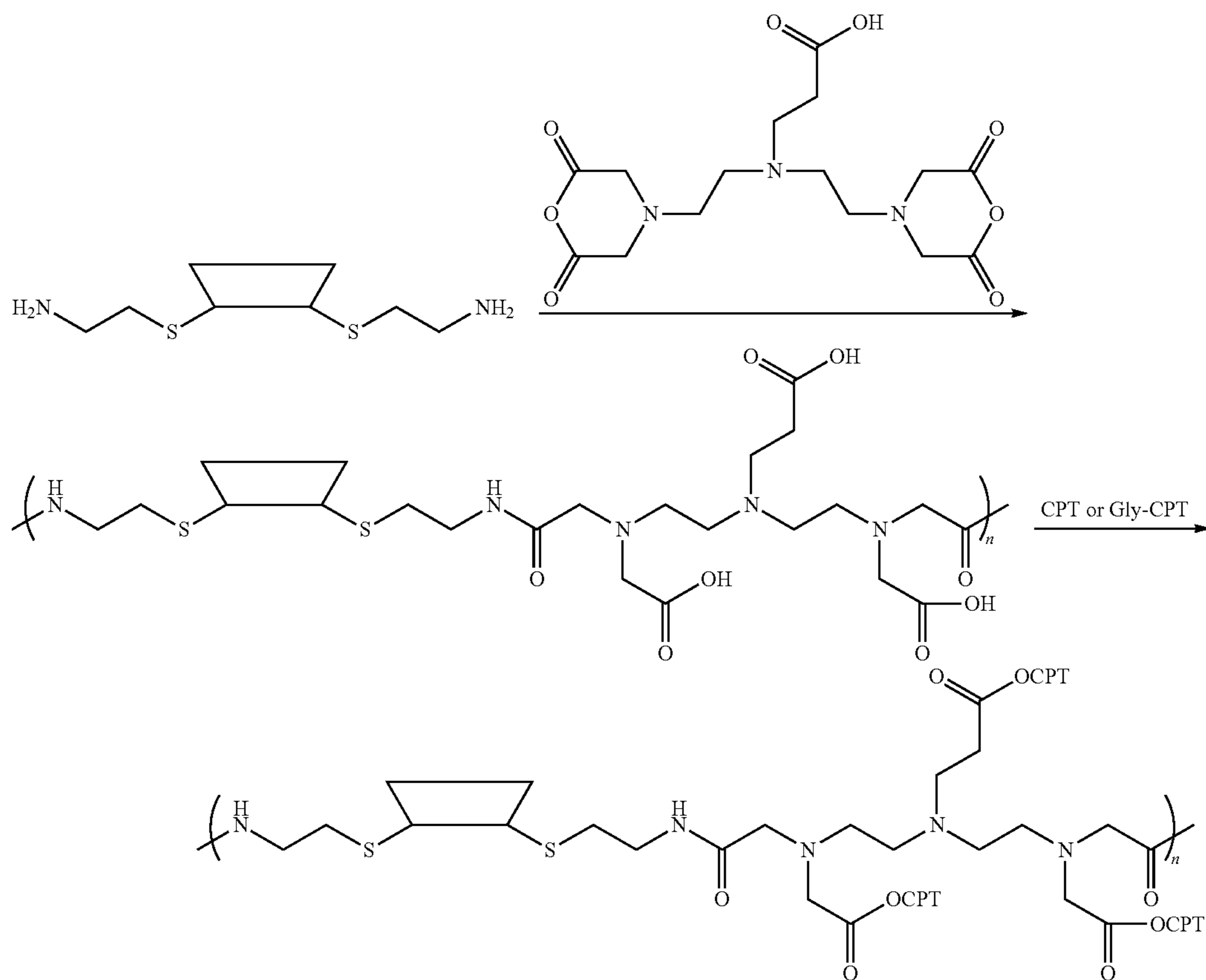
Scheme V
