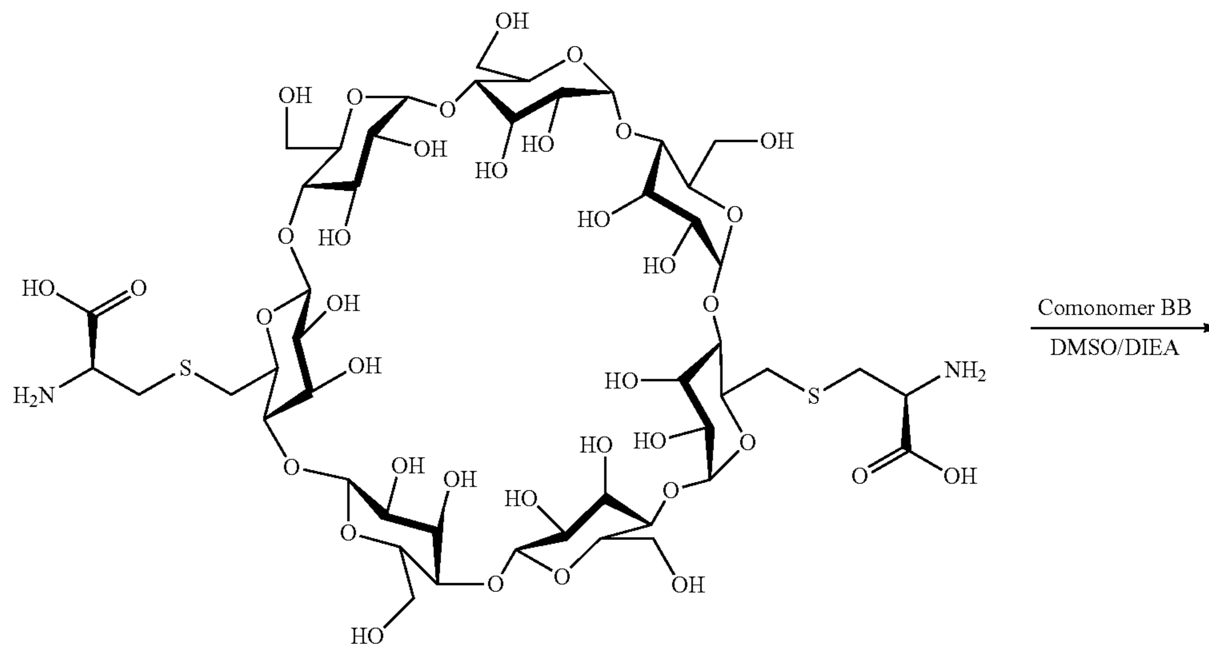
Scheme XXXVIIIb
