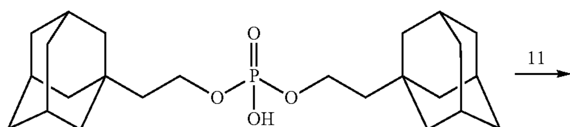
Scheme XXXXVIII
