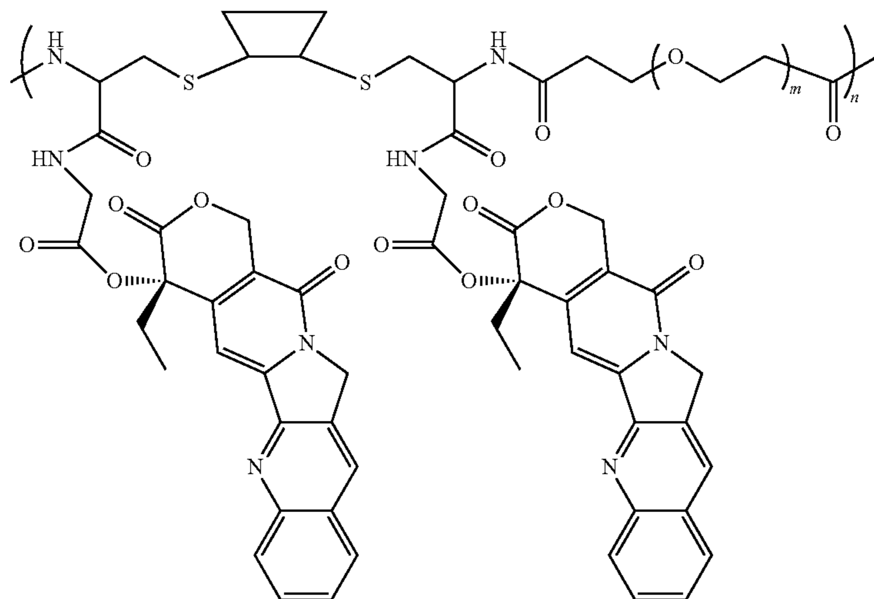
Scheme XXXXIII
