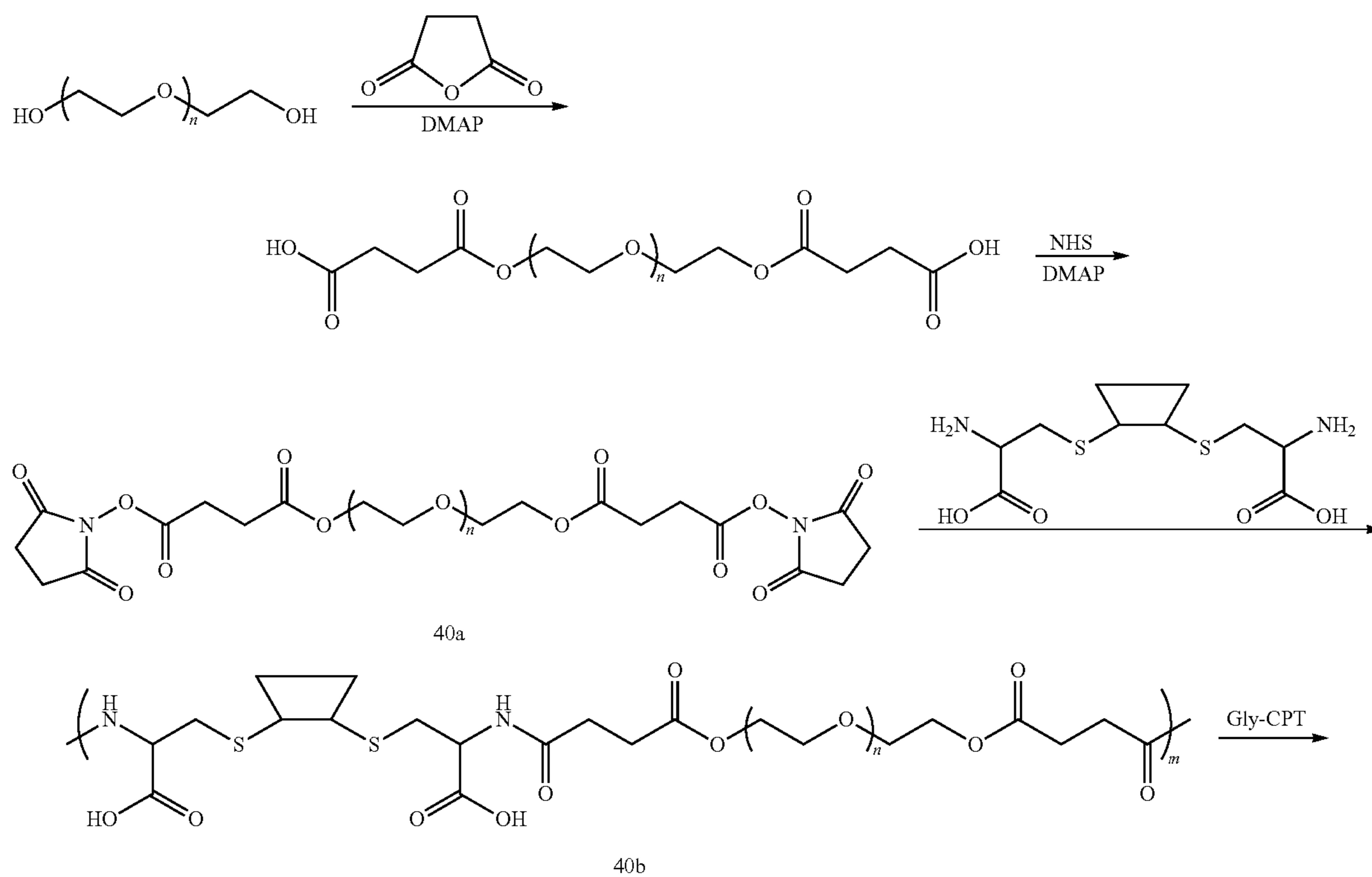
Scheme XXXXI
