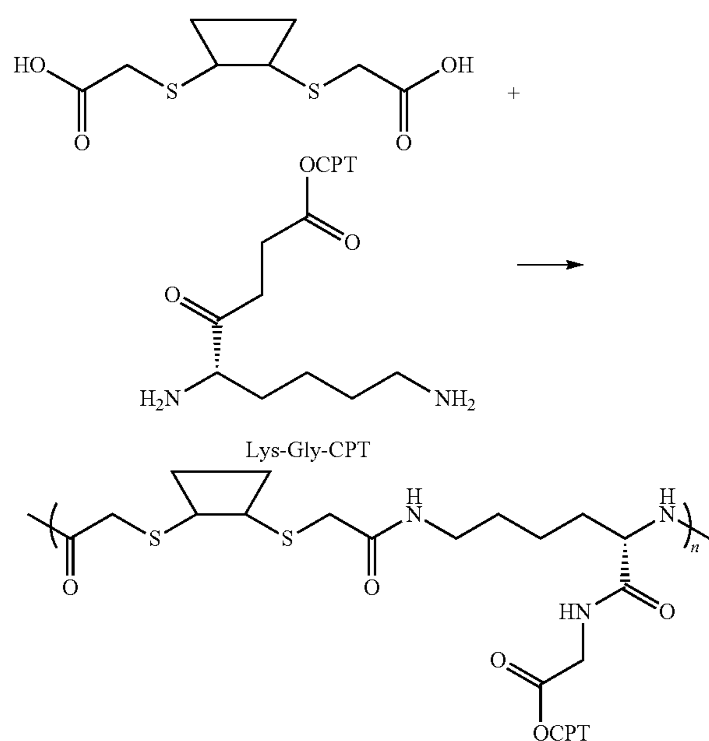
Scheme VIII
