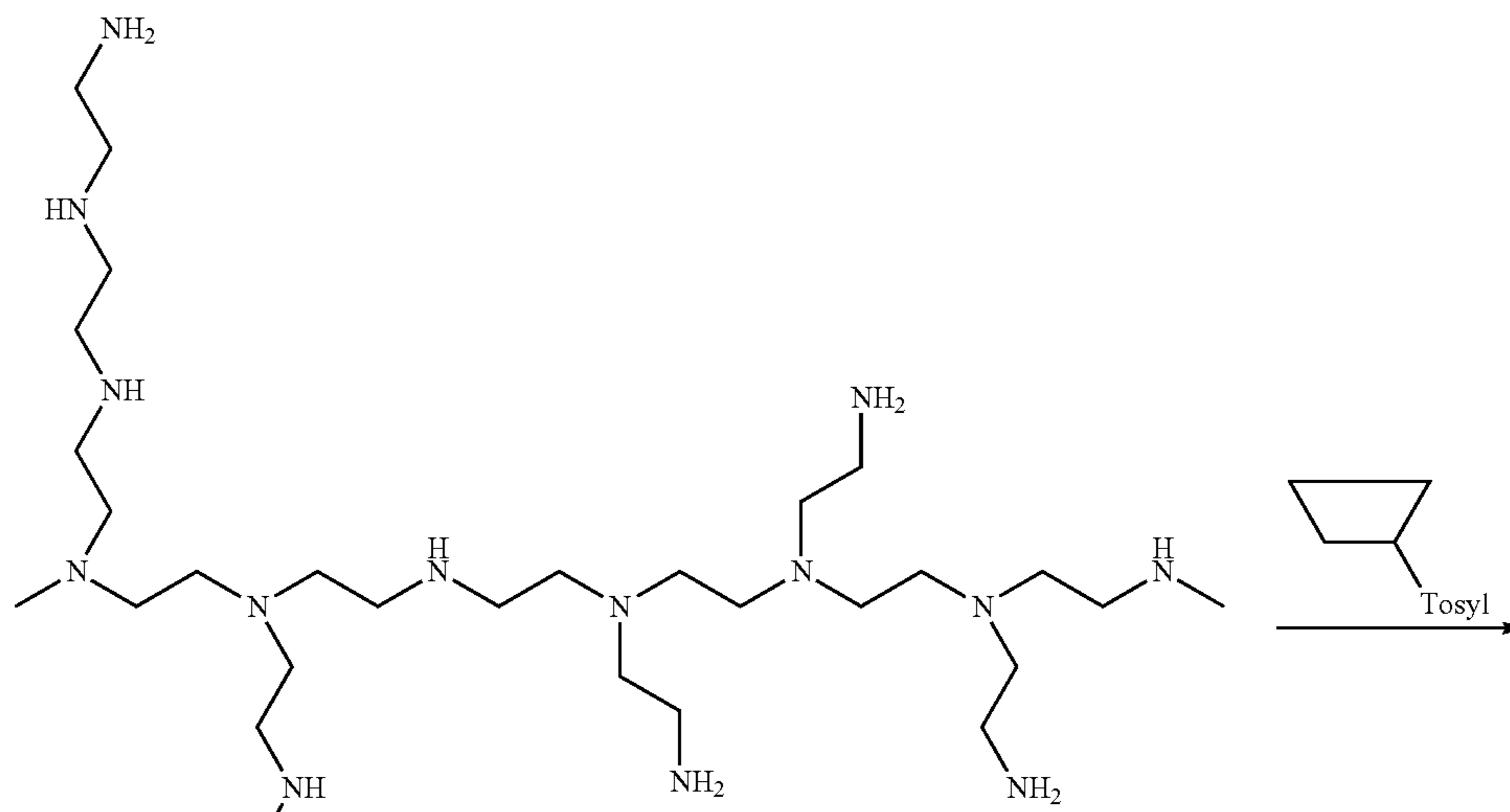
Scheme XXXIV
