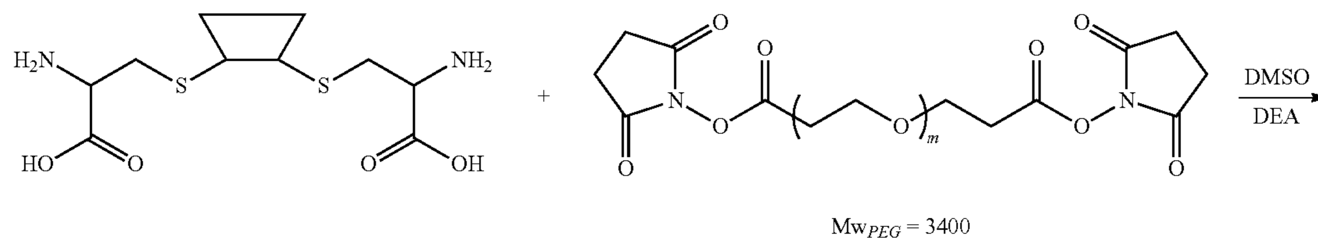
Scheme XIII
