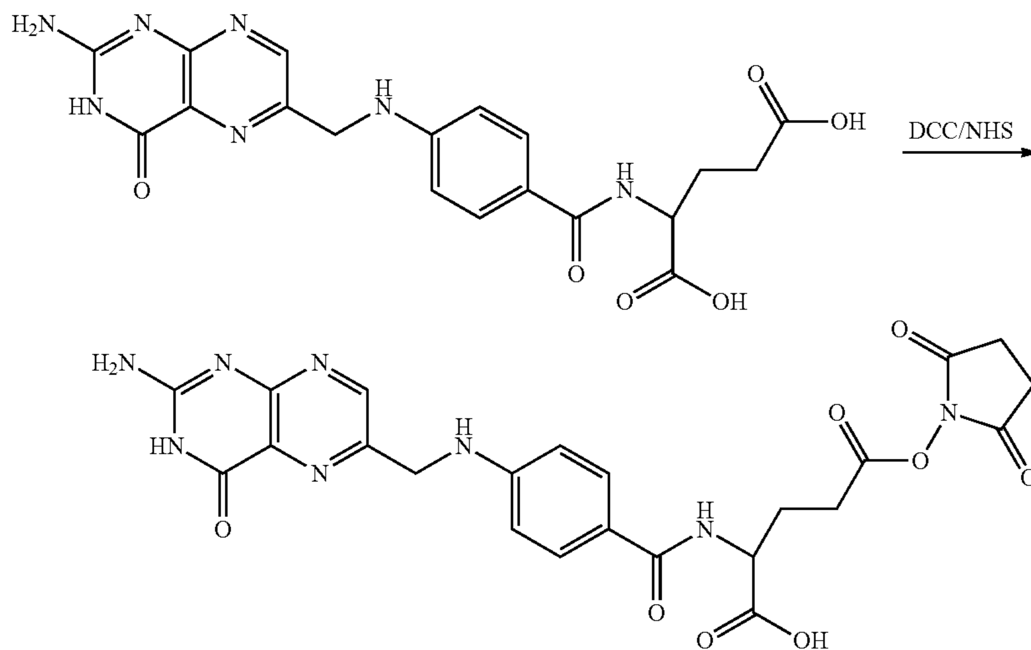
Scheme XXXXIX
