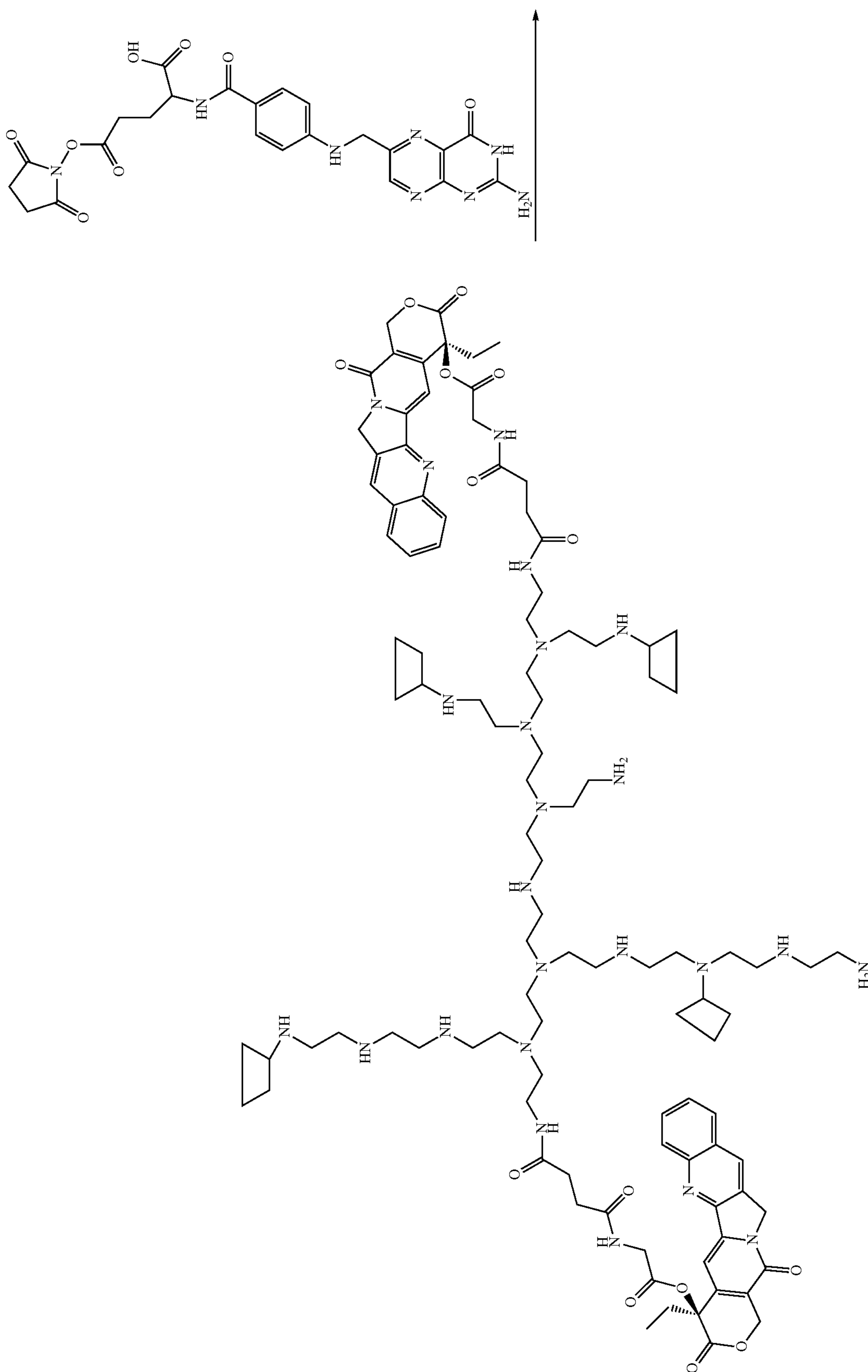
Scheme II
