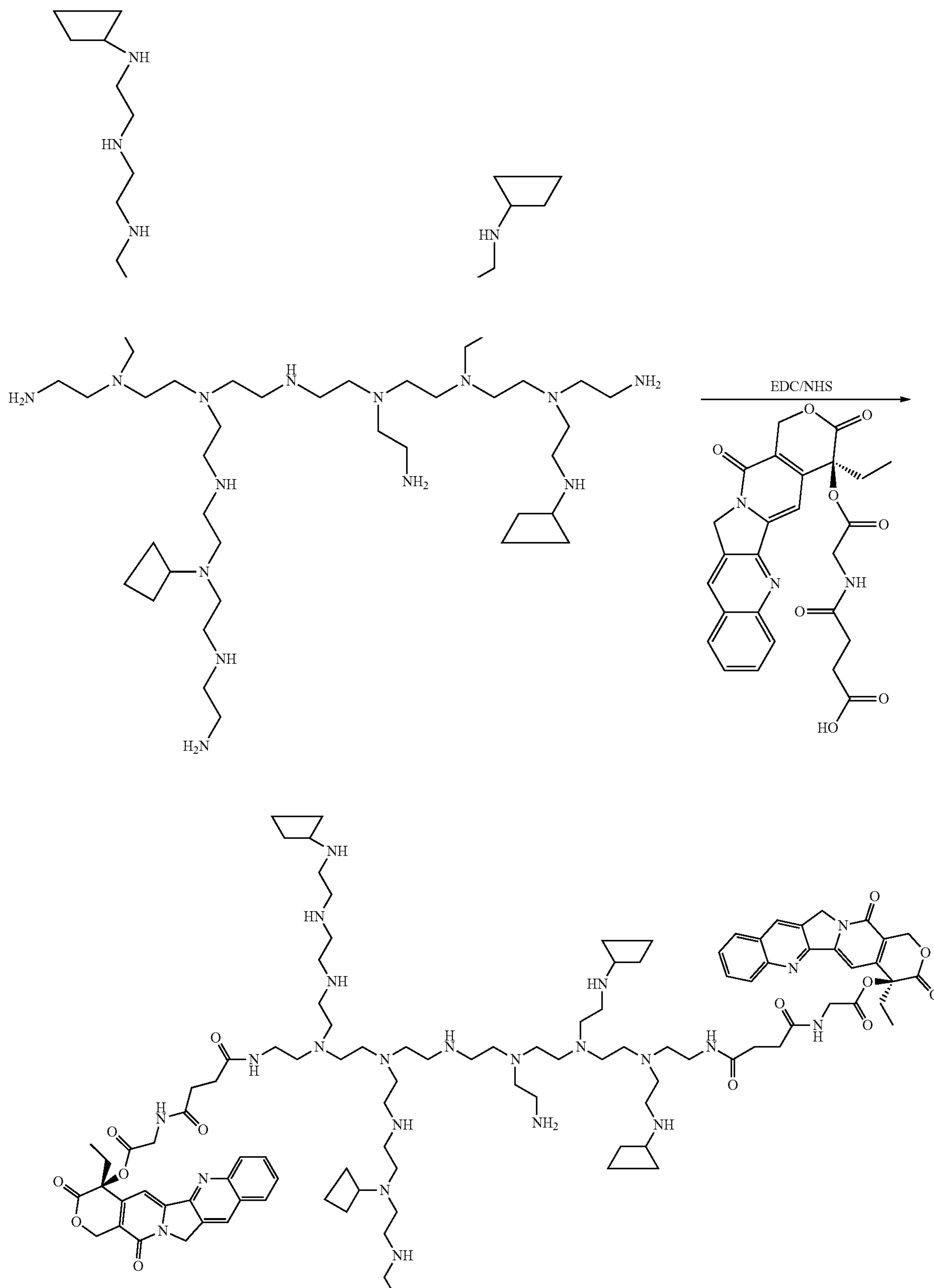
Scheme XXXXV
