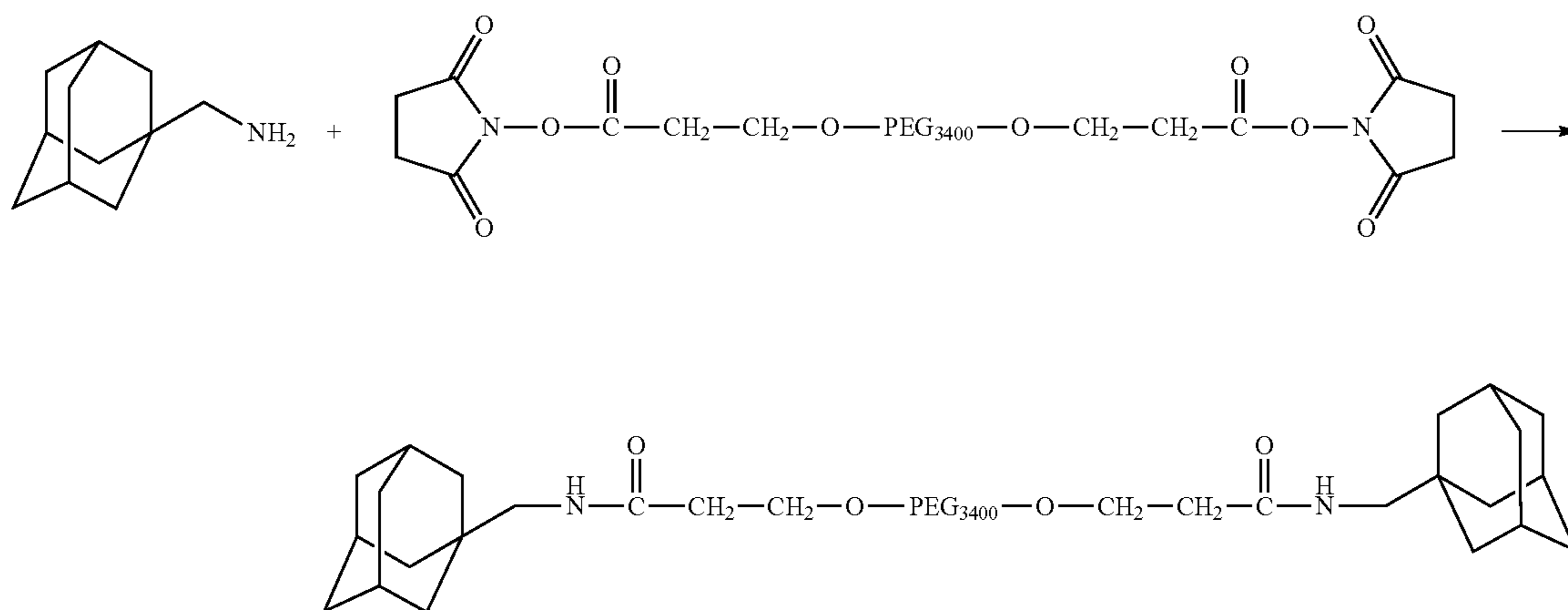
Scheme XXXXVI
