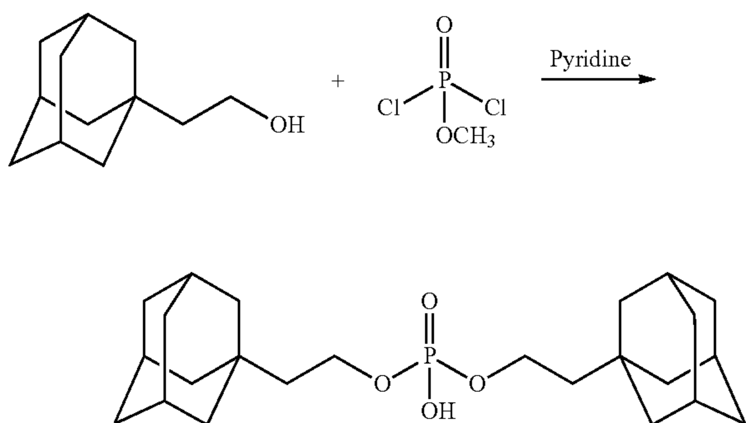
Scheme XXXXVII
