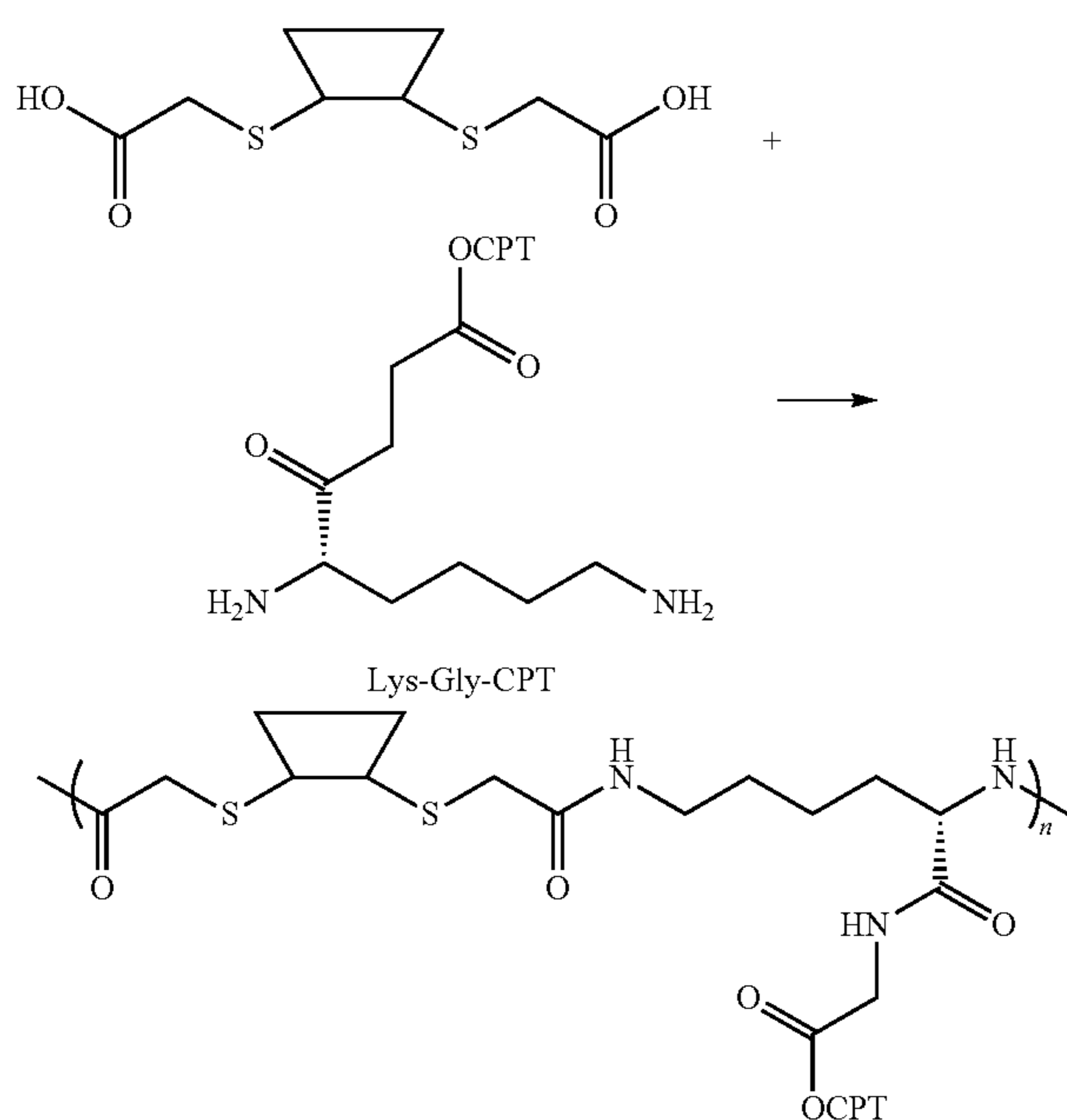
Scheme VIII
