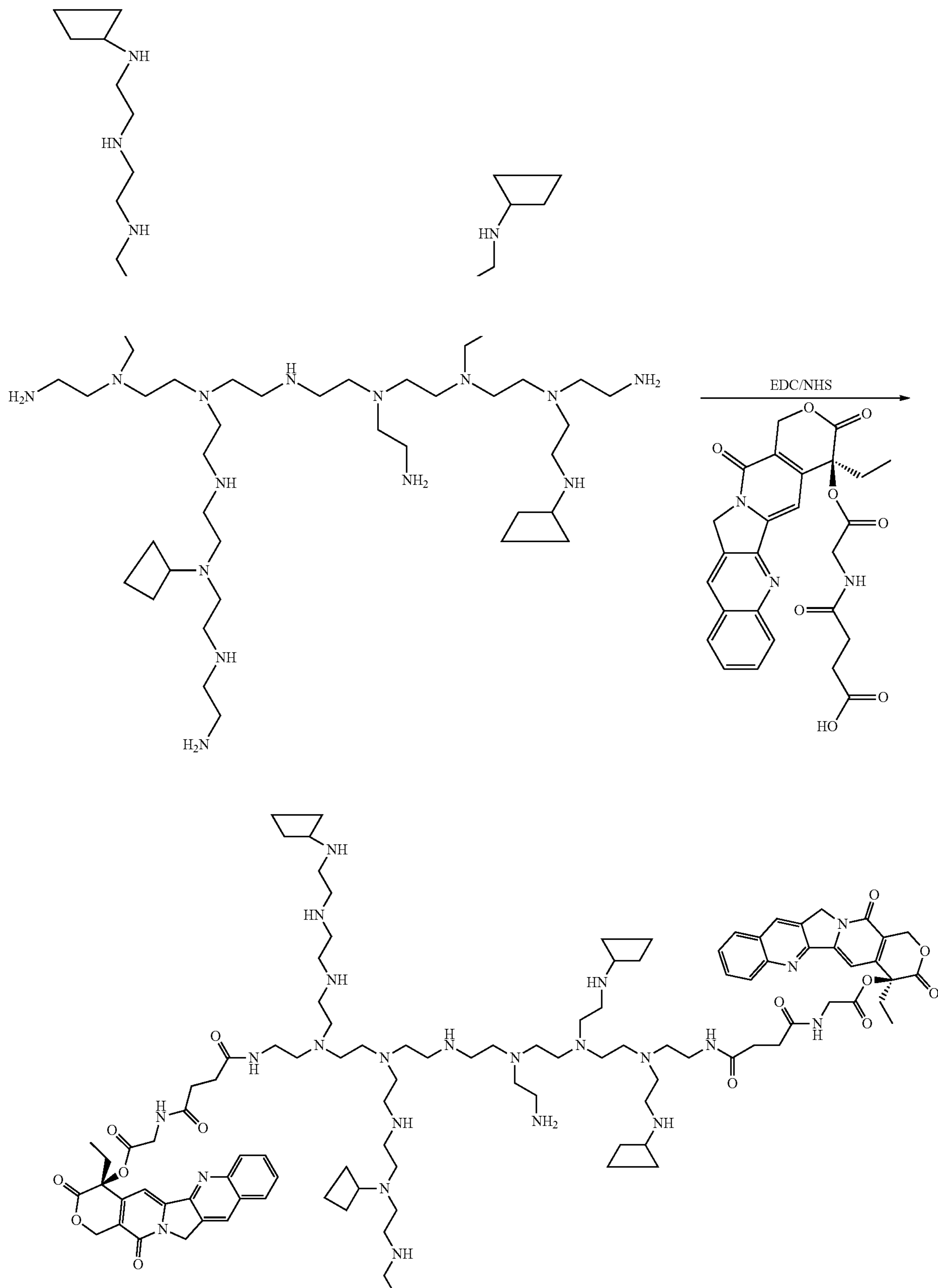
Scheme XXXXV
