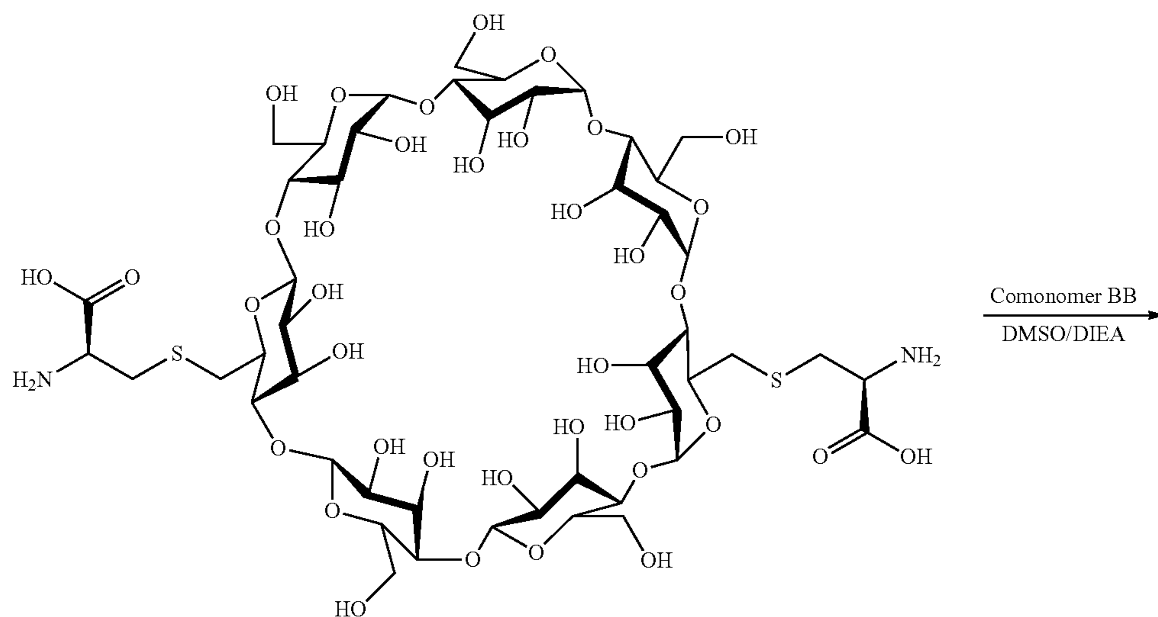
Scheme XXXVIIIb
