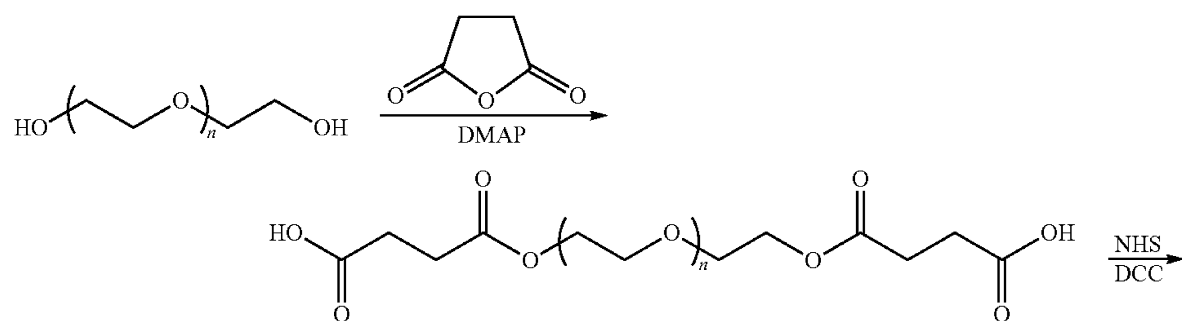
Scheme XIV
