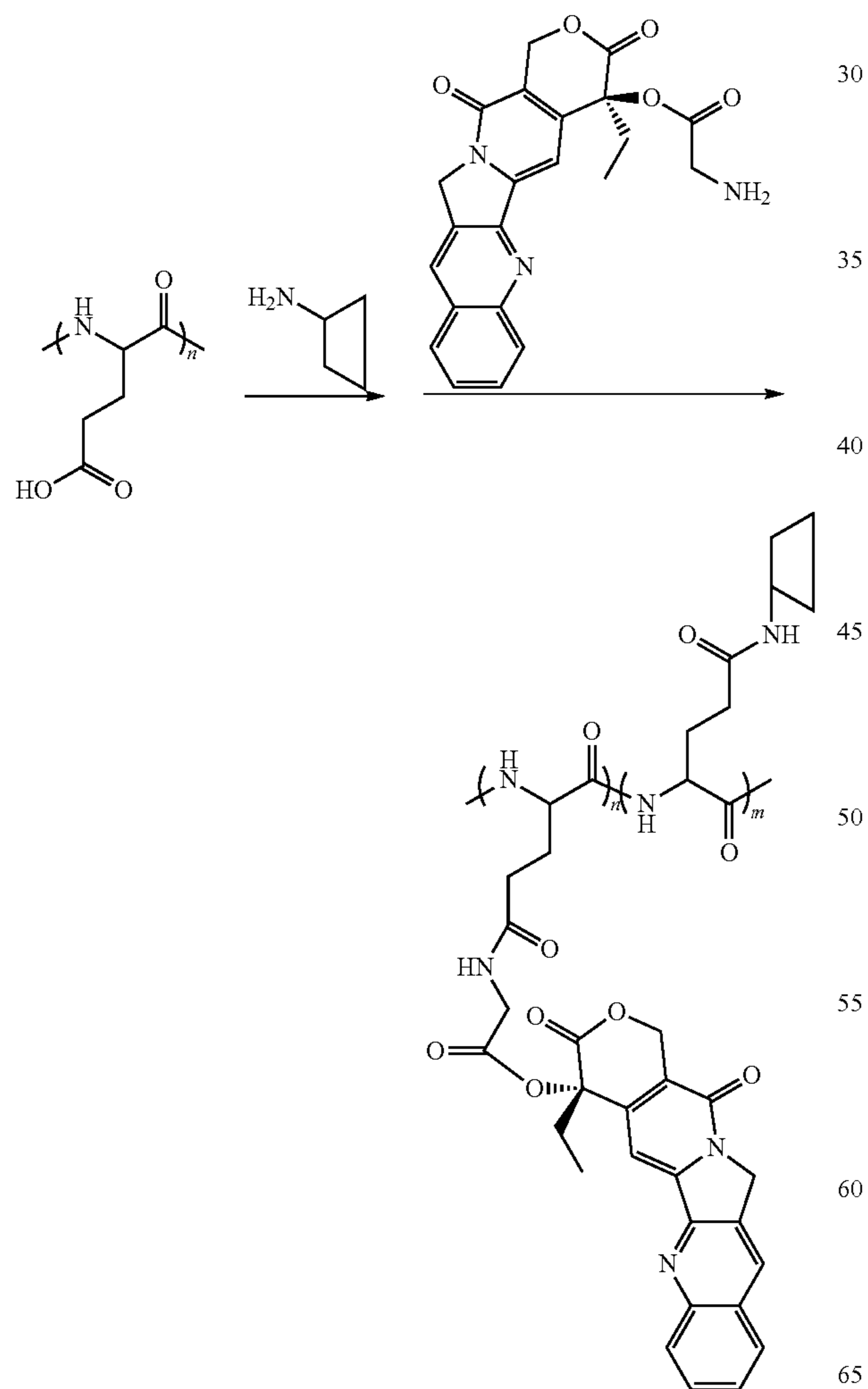
Scheme XII
