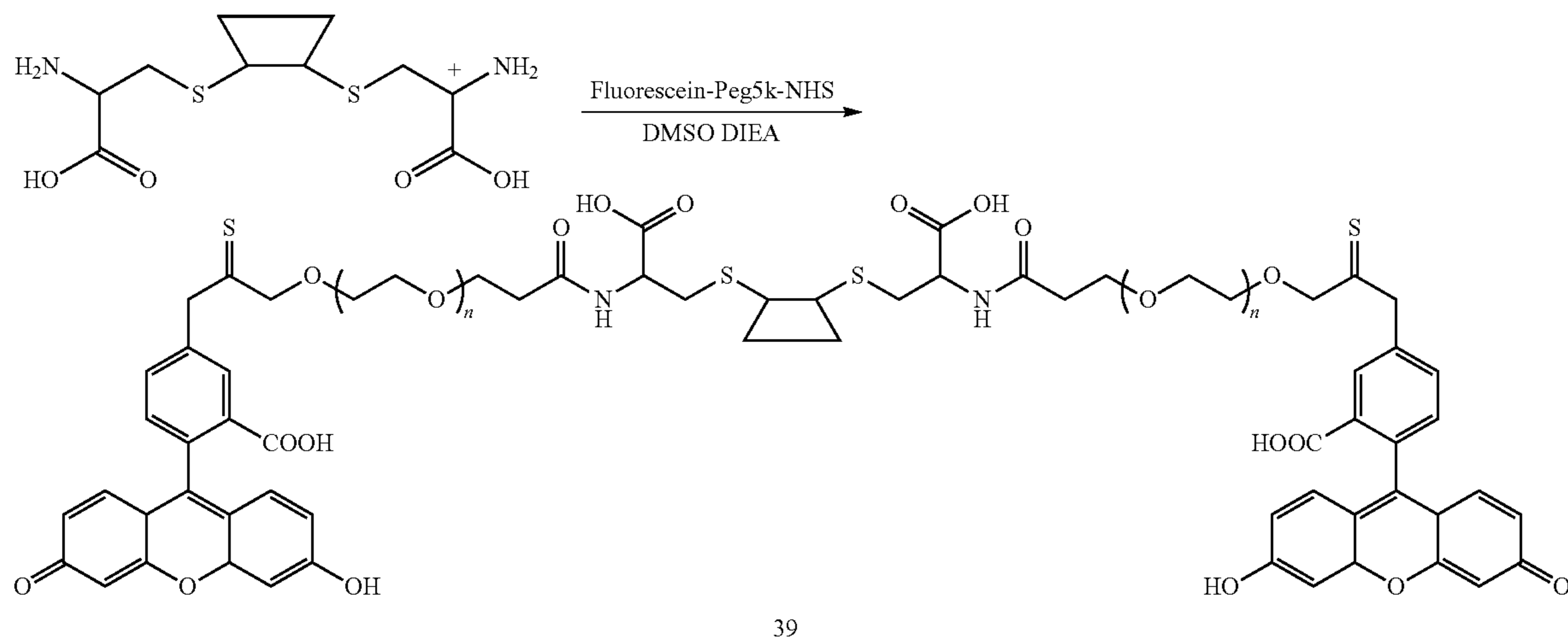
Scheme XXXX
