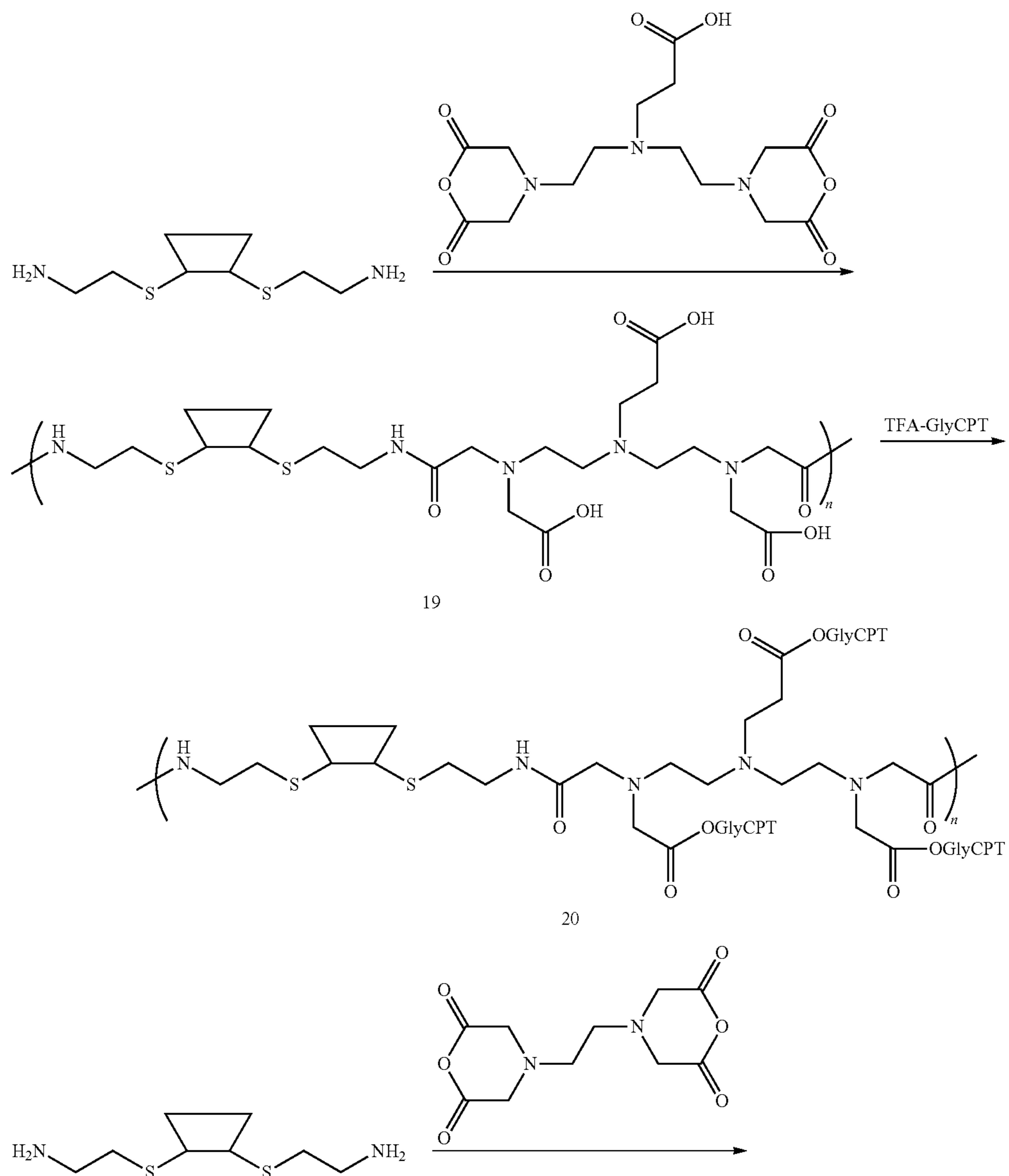
Scheme XXIX
