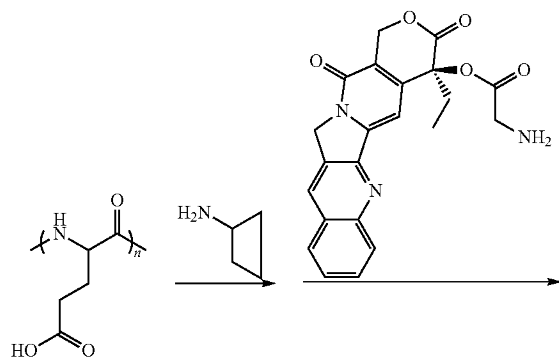
Scheme XII
