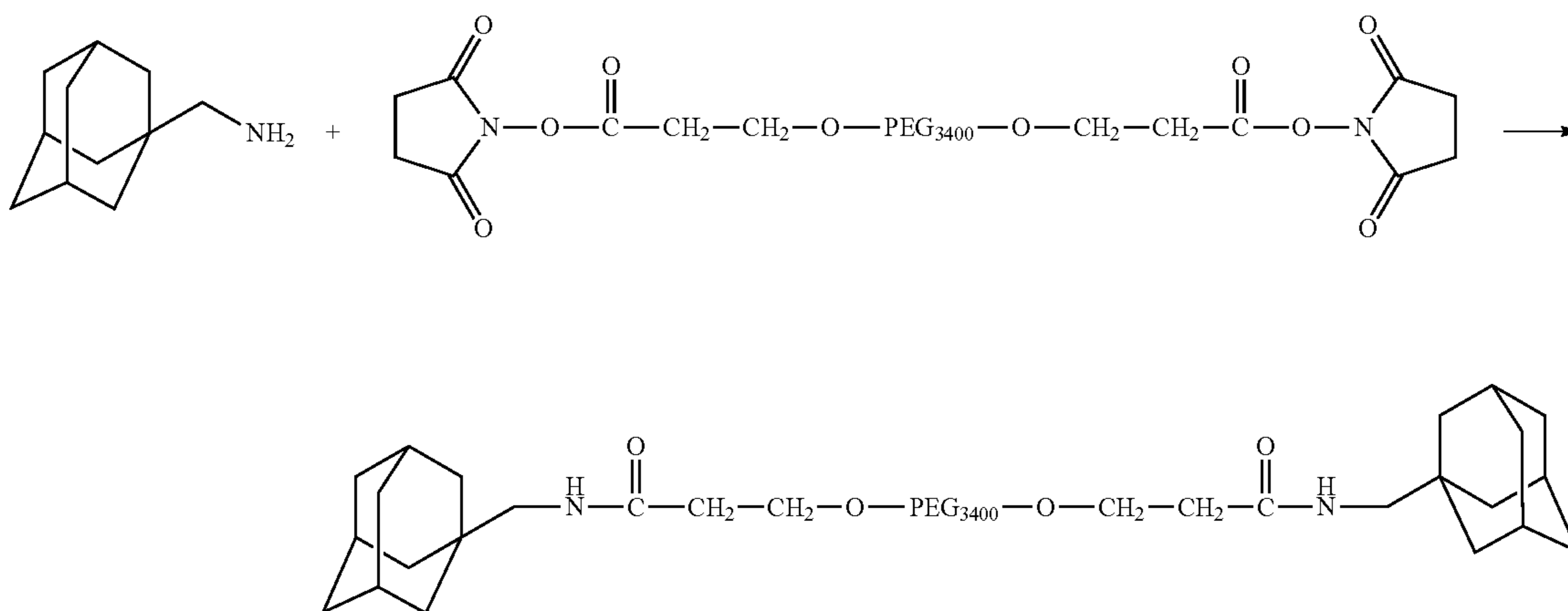
Scheme XXXXVI
