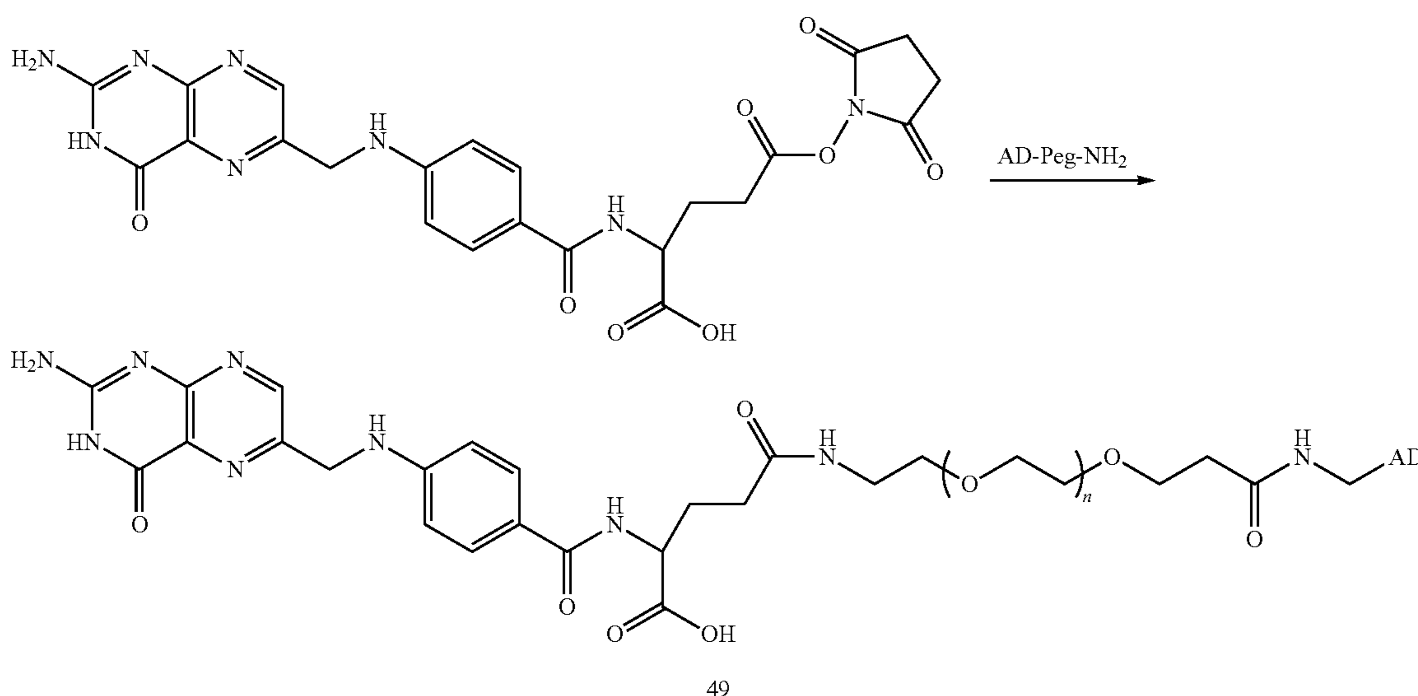
Scheme L
