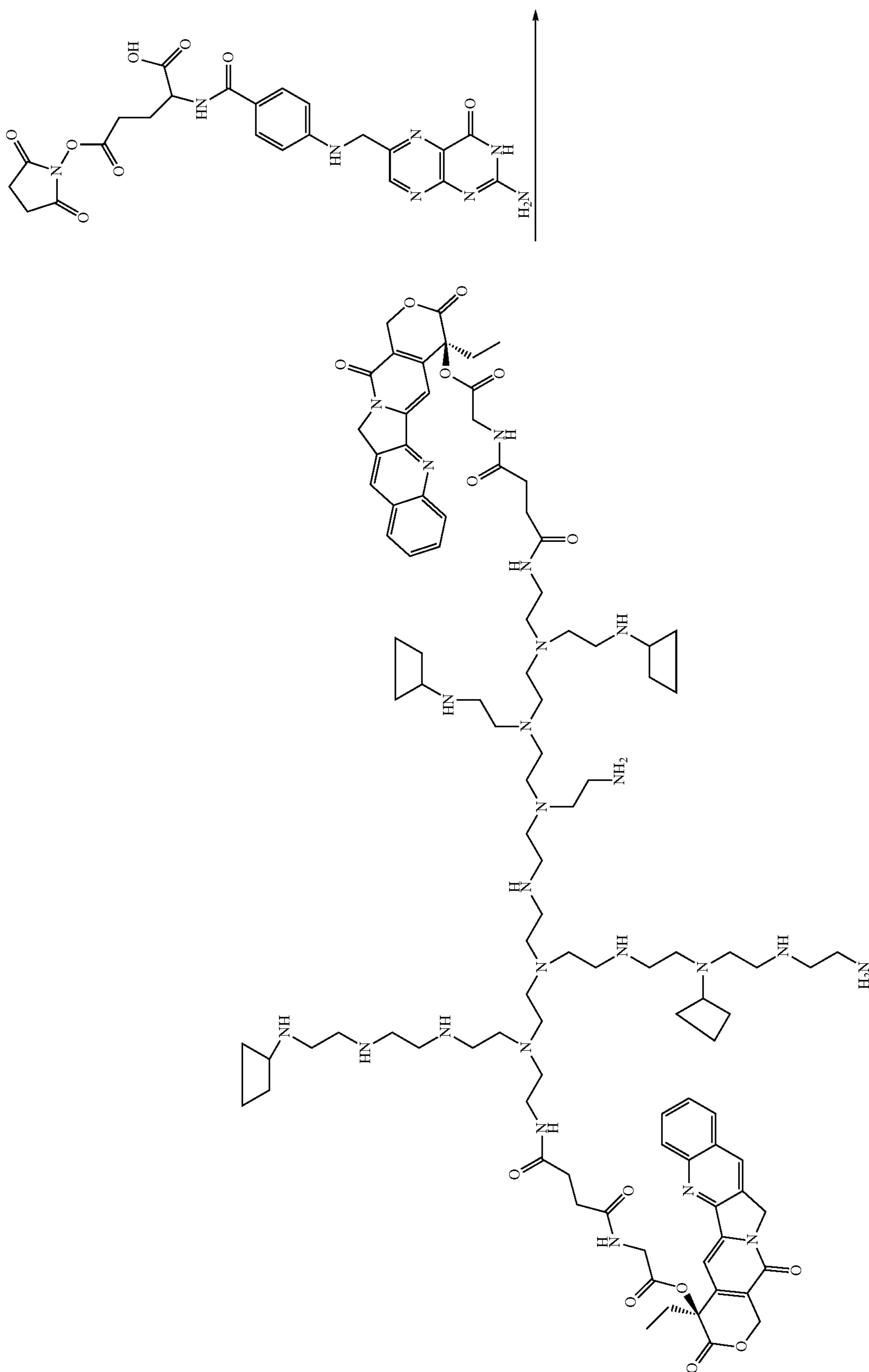
Scheme II
