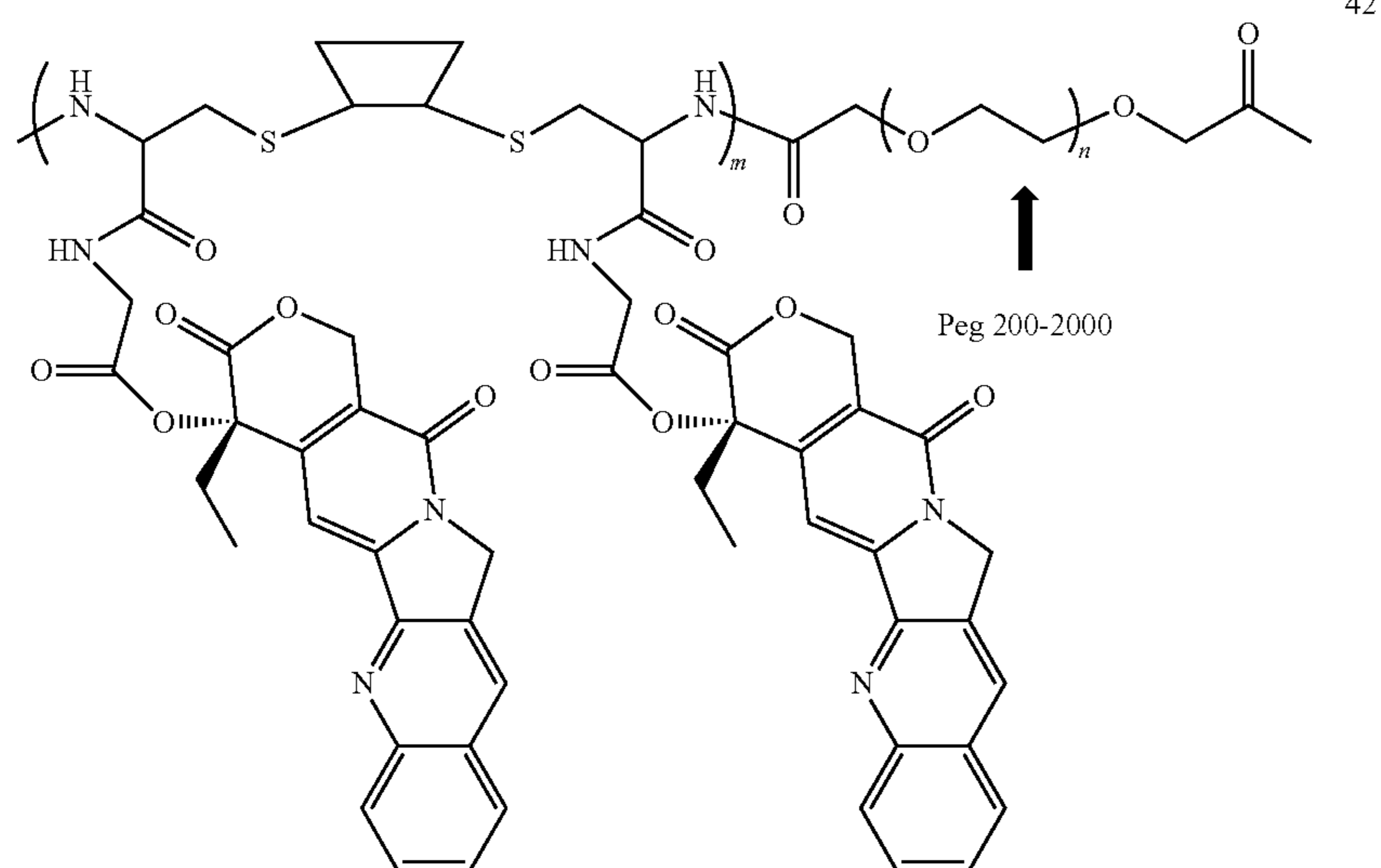
Scheme XXXXII
