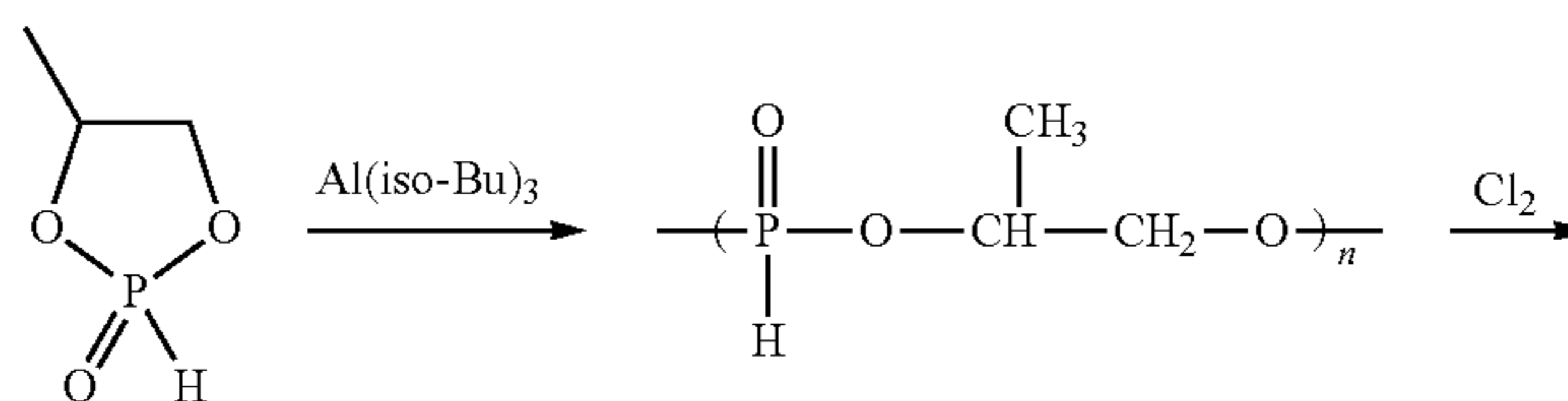
Scheme IX
