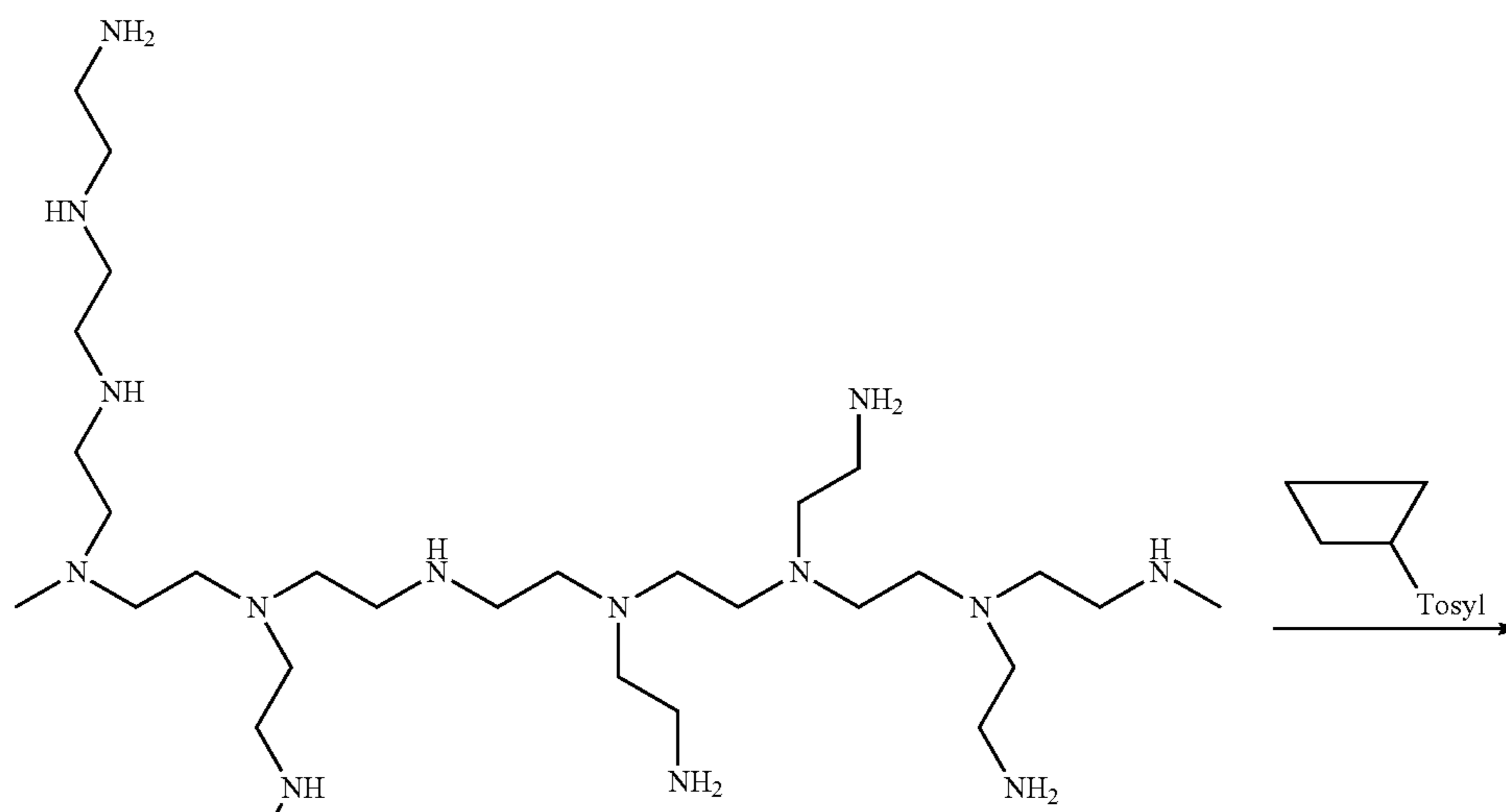
Scheme XXXIV
