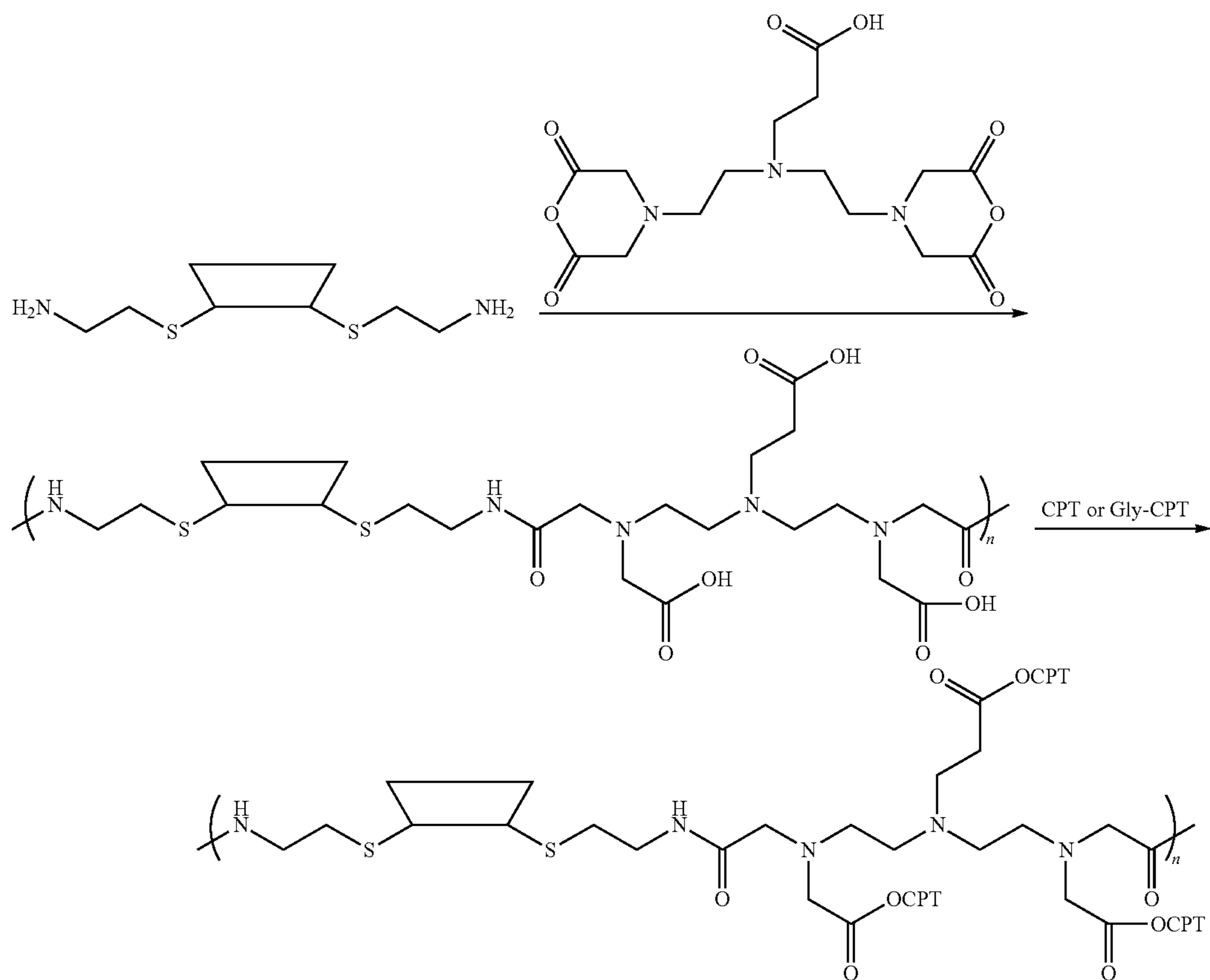
Scheme V
