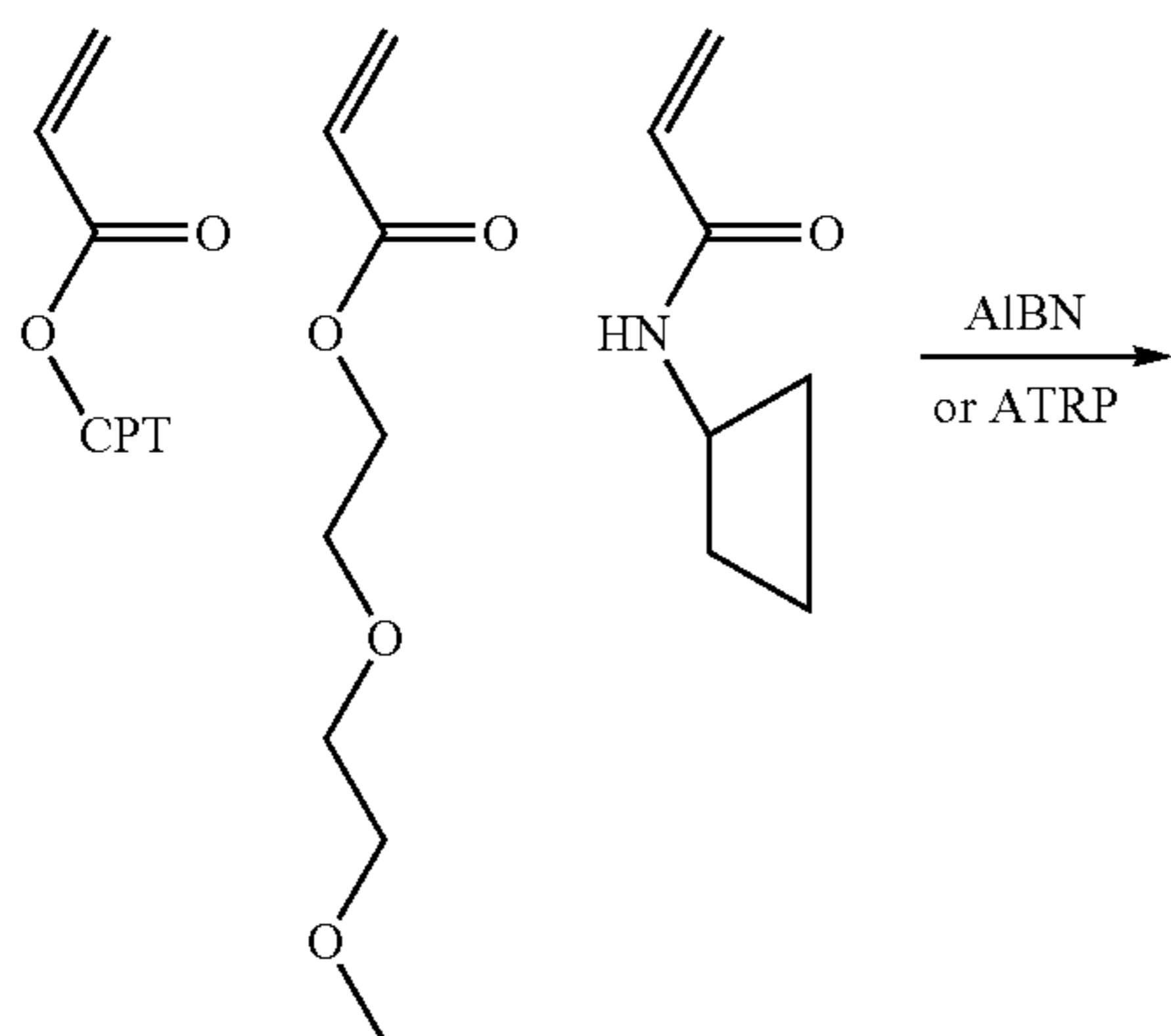
Scheme XXXV
