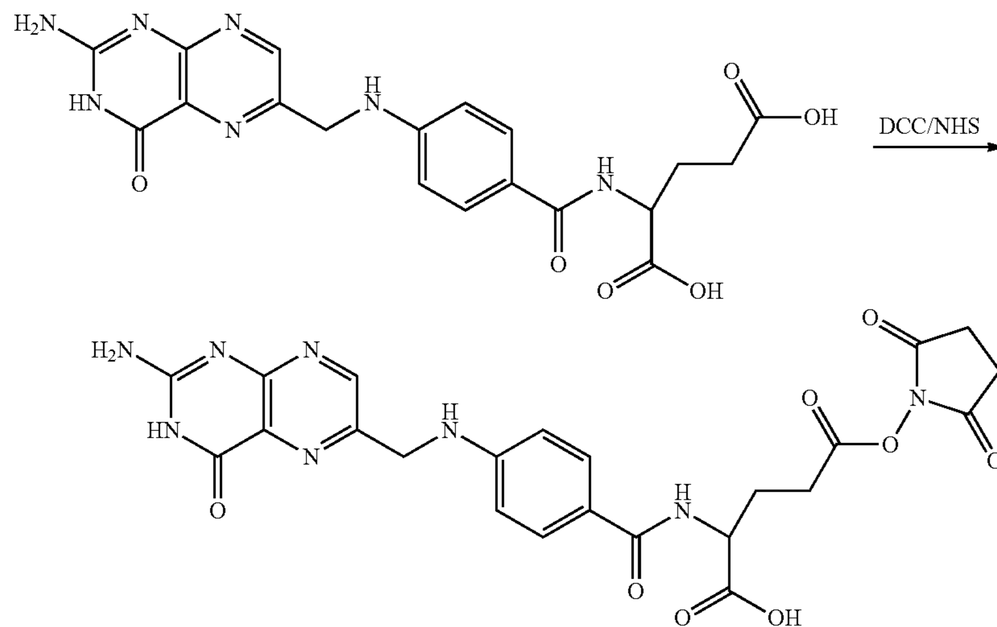
Scheme XXXXIX
