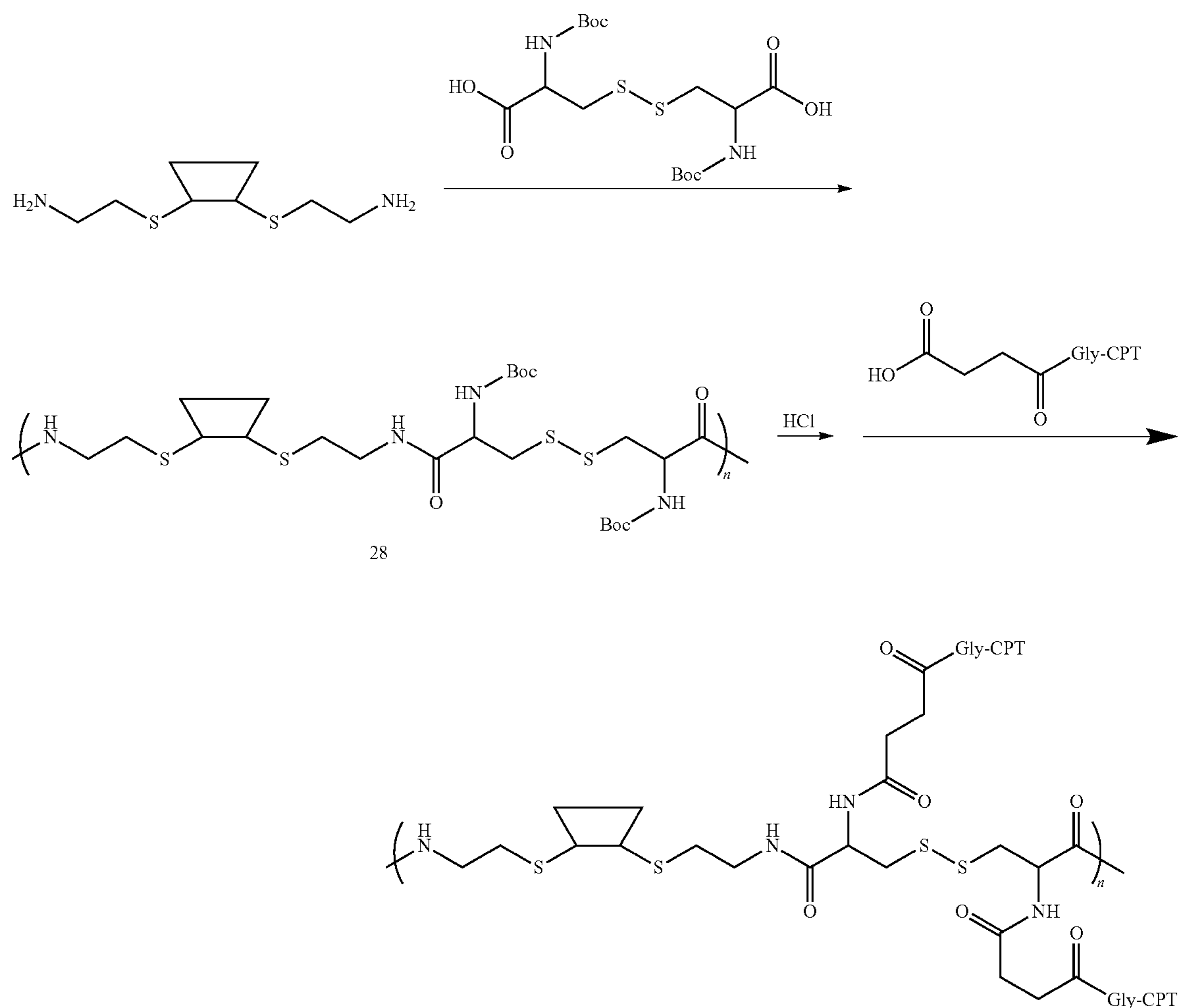
Scheme XXXIII
