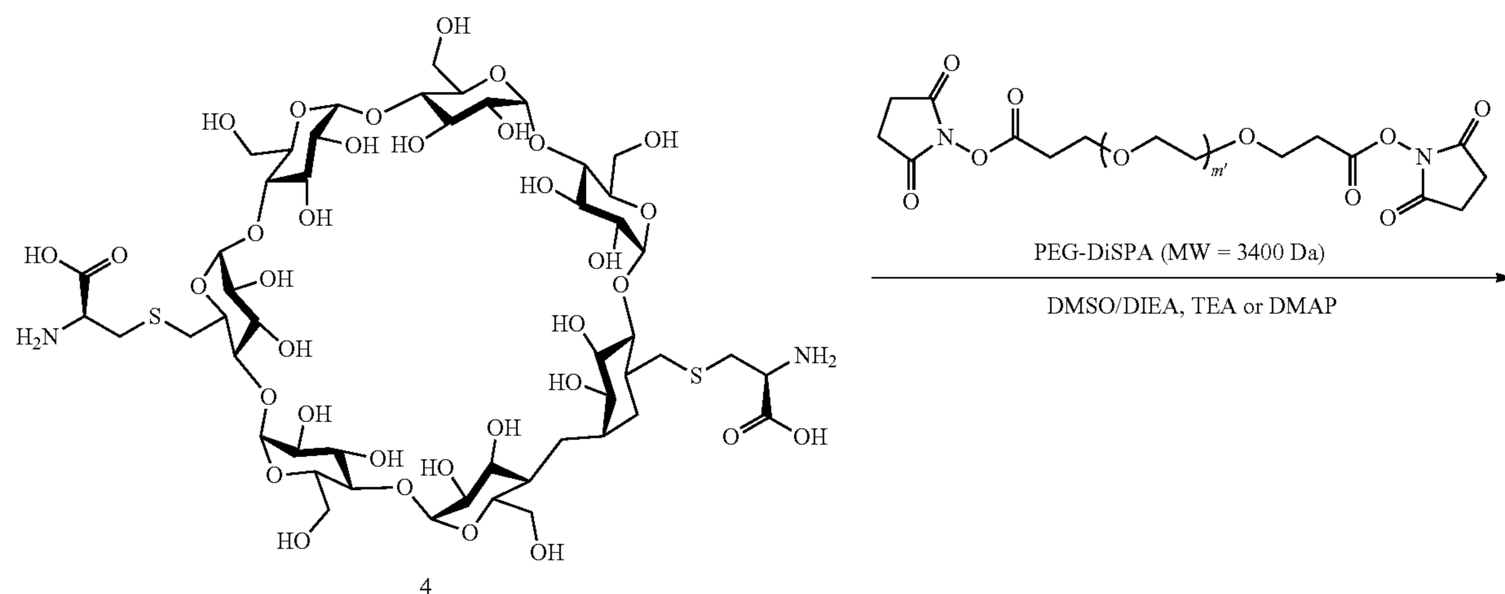
Scheme XXXVIIIa
