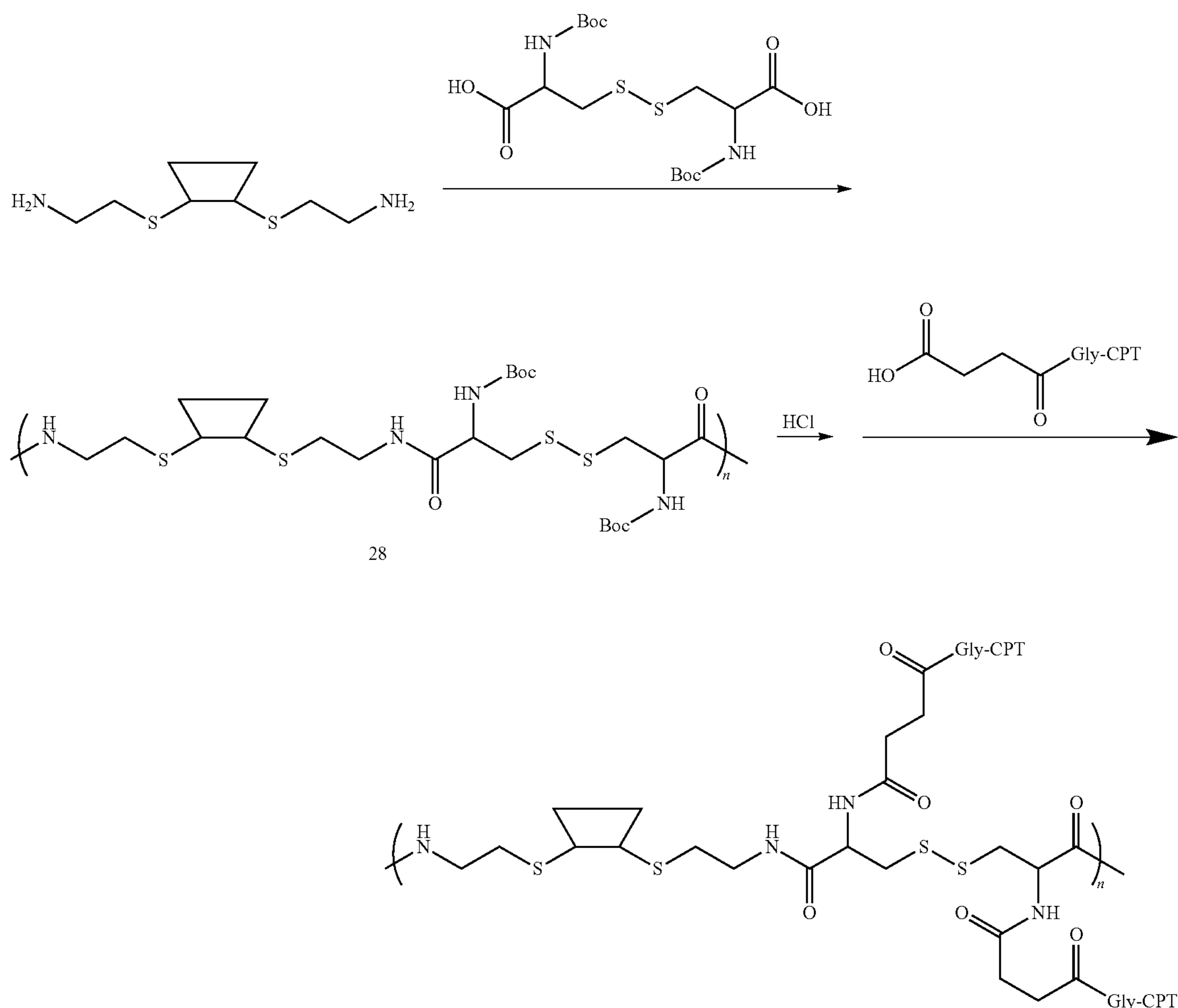
Scheme XXXIII
