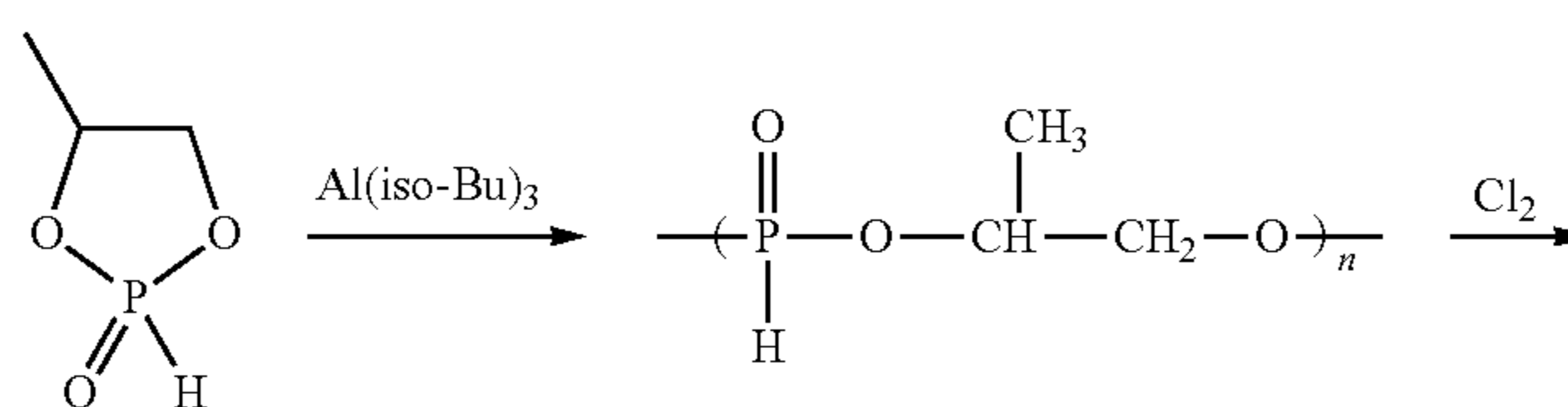
Scheme IX
