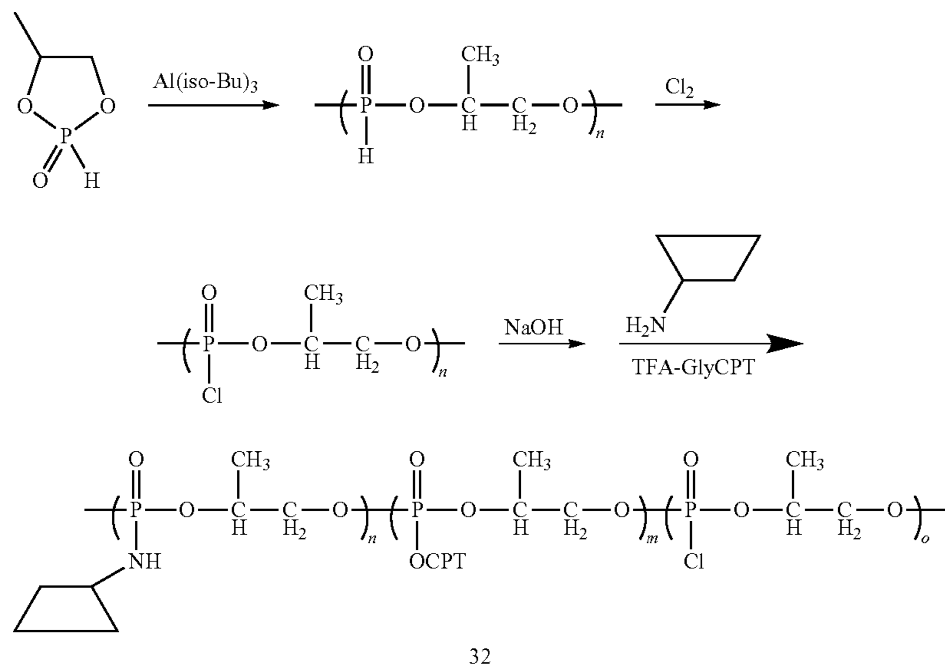
Scheme XXXIV
