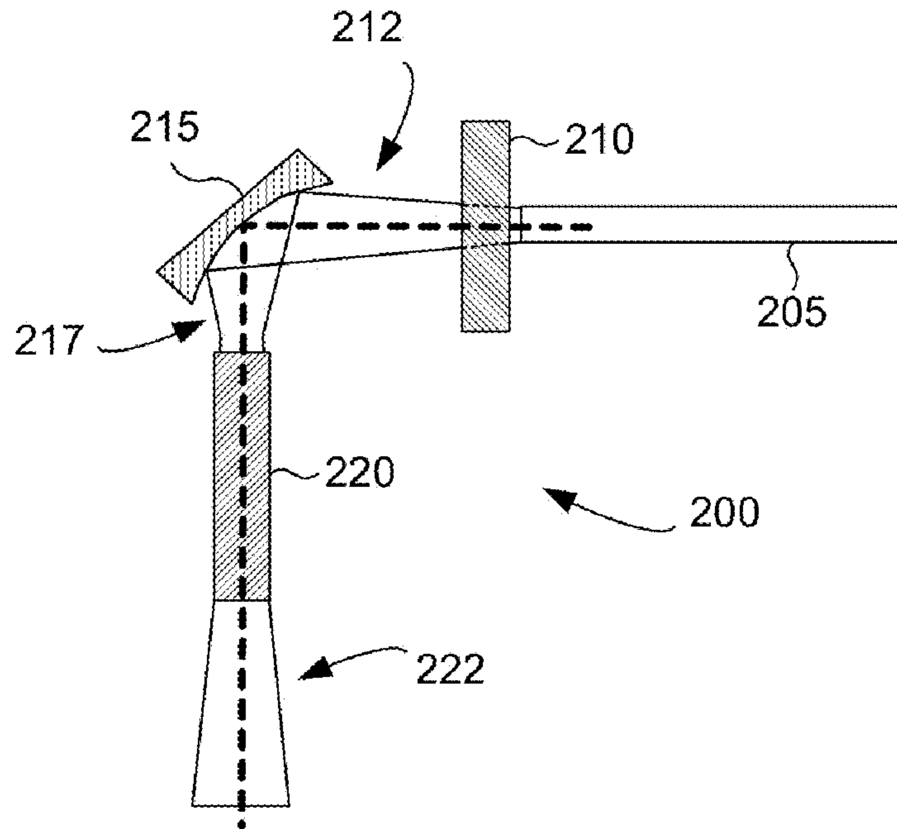
FIG. 2 (Prior Art)
