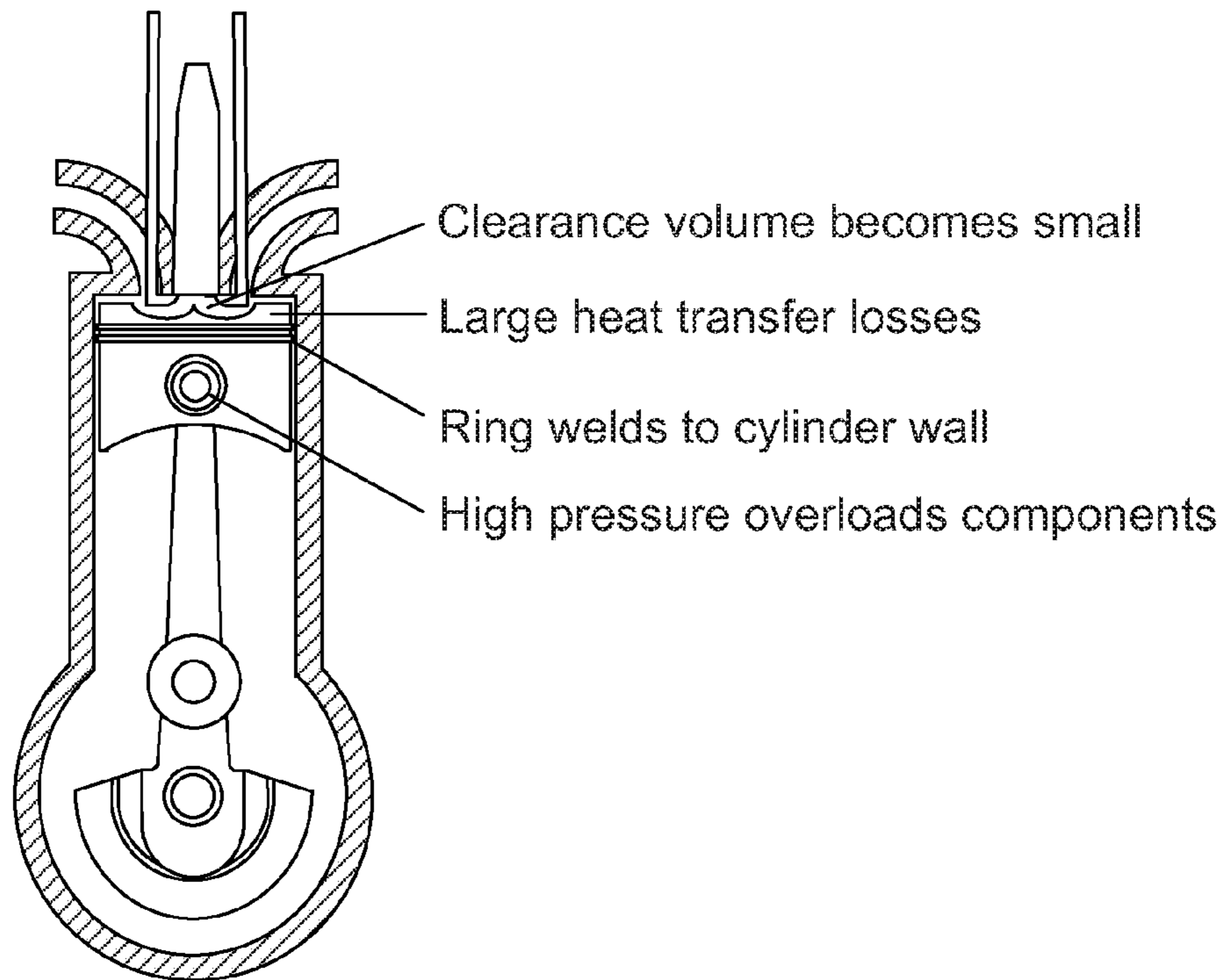
FIG. 3 (Prior Art)
