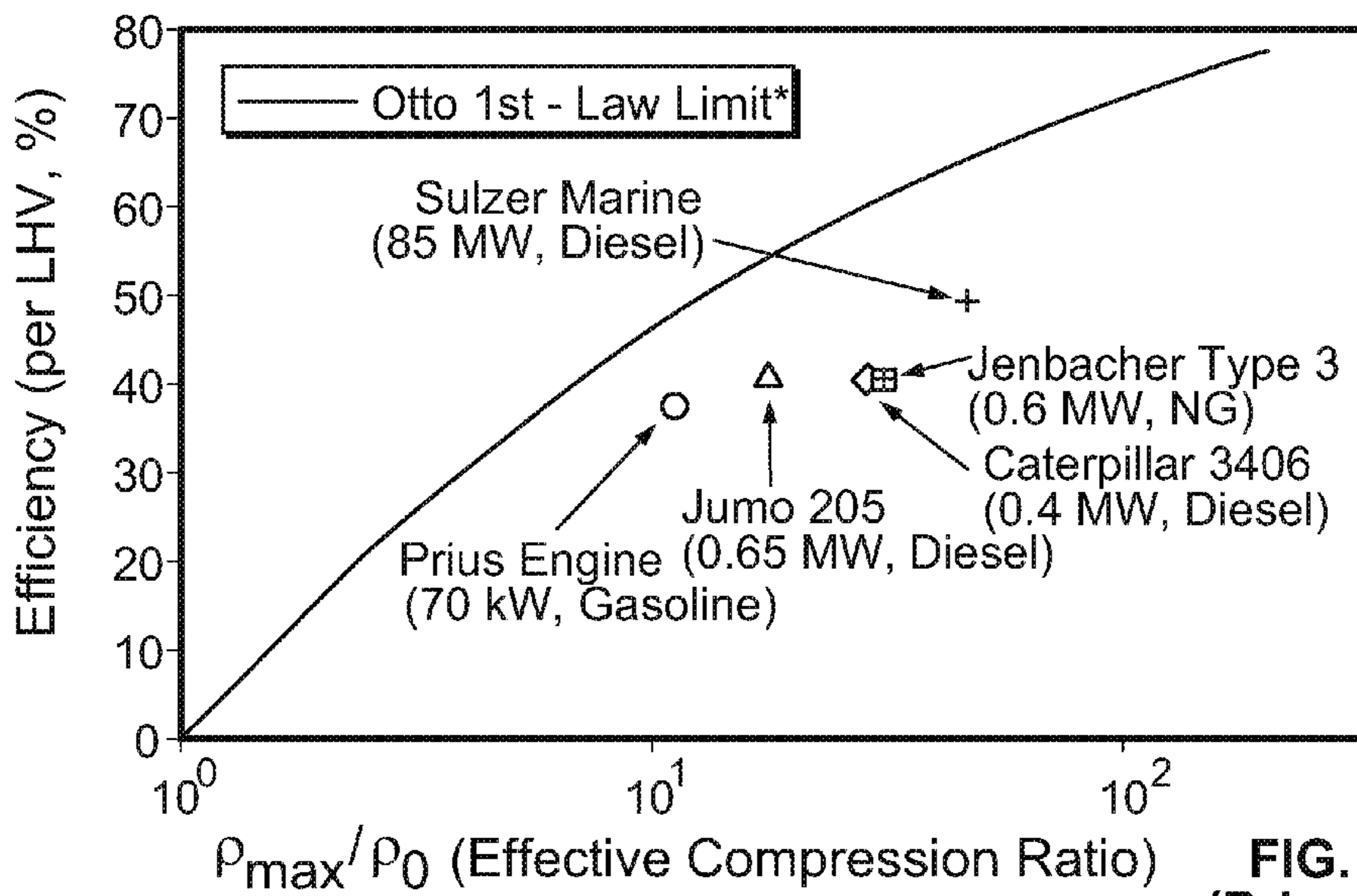
FIG. 1 (Prior Art)
