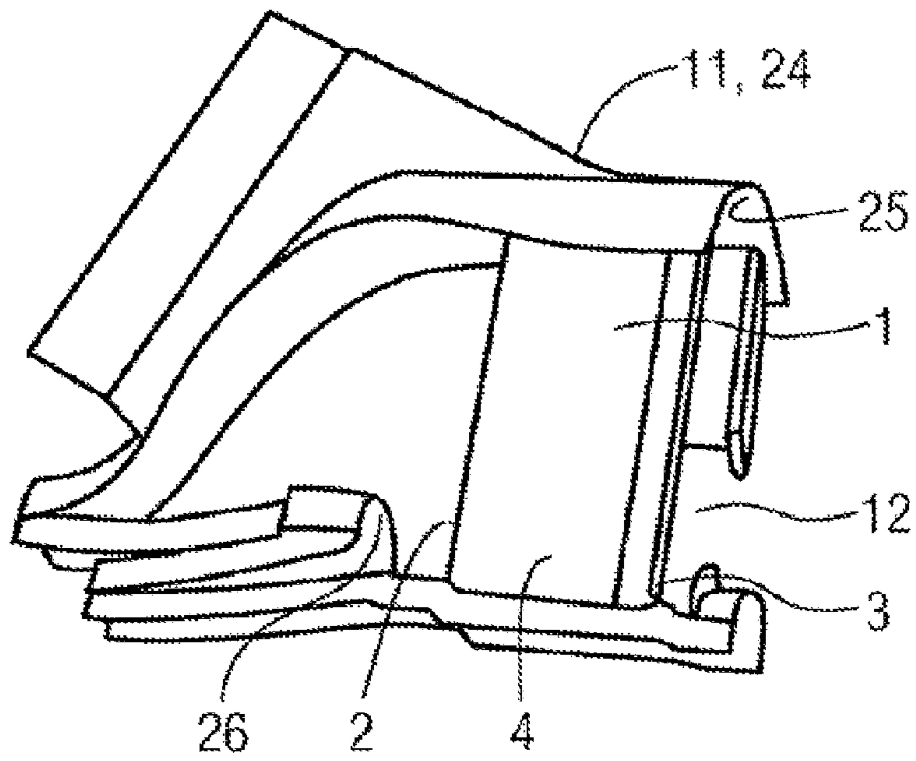
PRIOR ART
