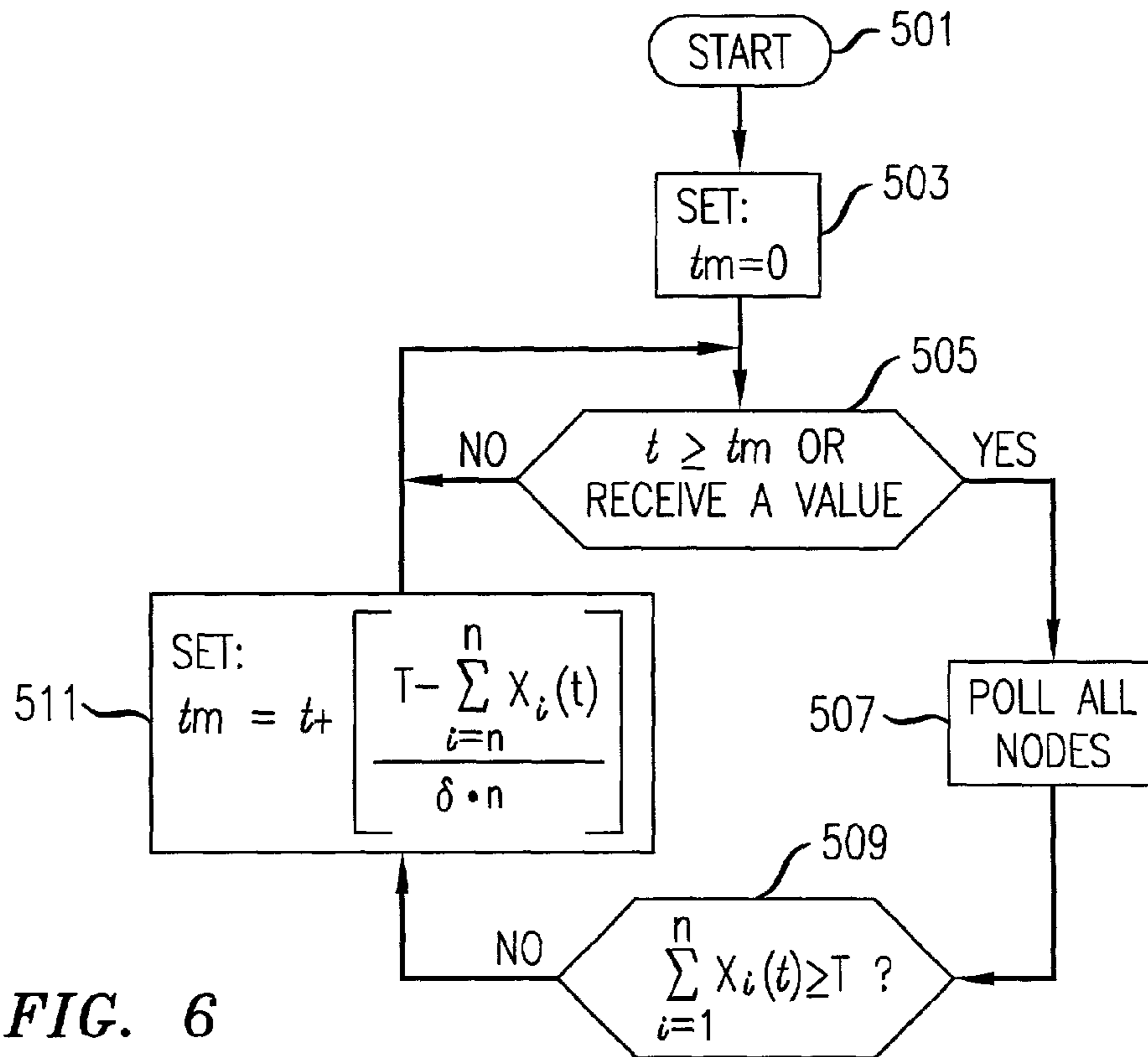
ADVANCED RATE NODE PROCESS
