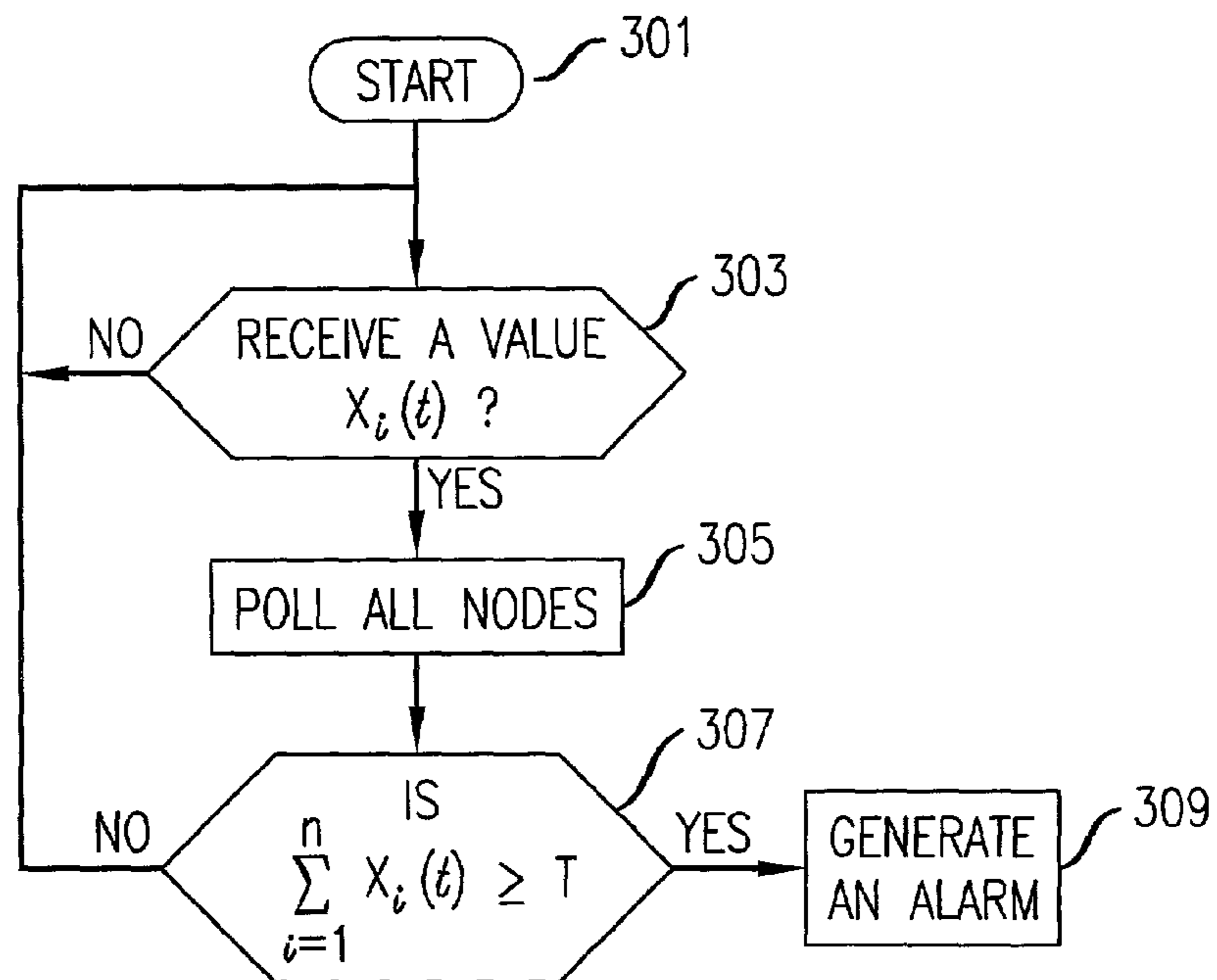
SIMPLE VALUE CENTRALIZED PROCESS
