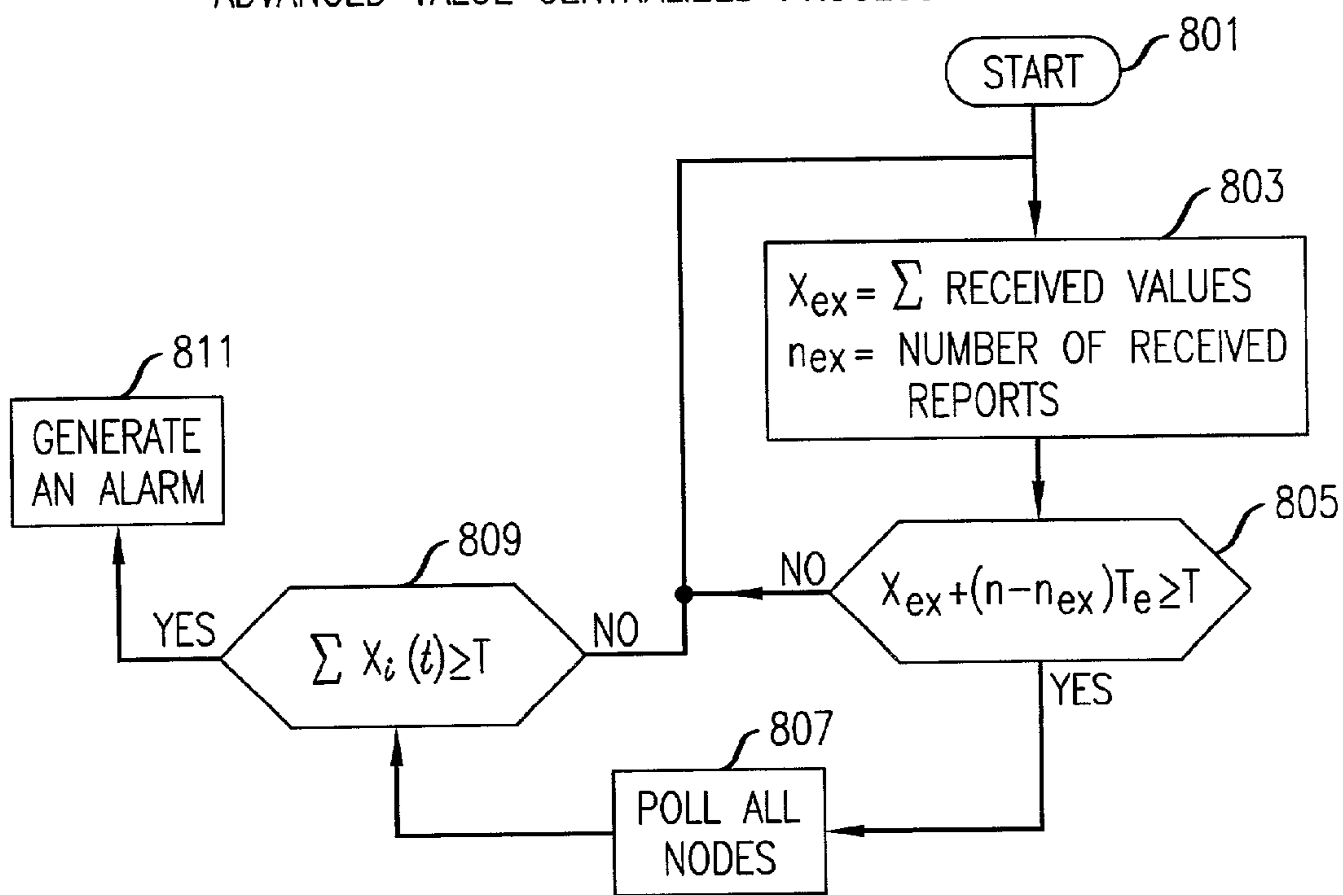
FIG. 8 ADVANCED VALUE CENTRALIZED PROCESS
