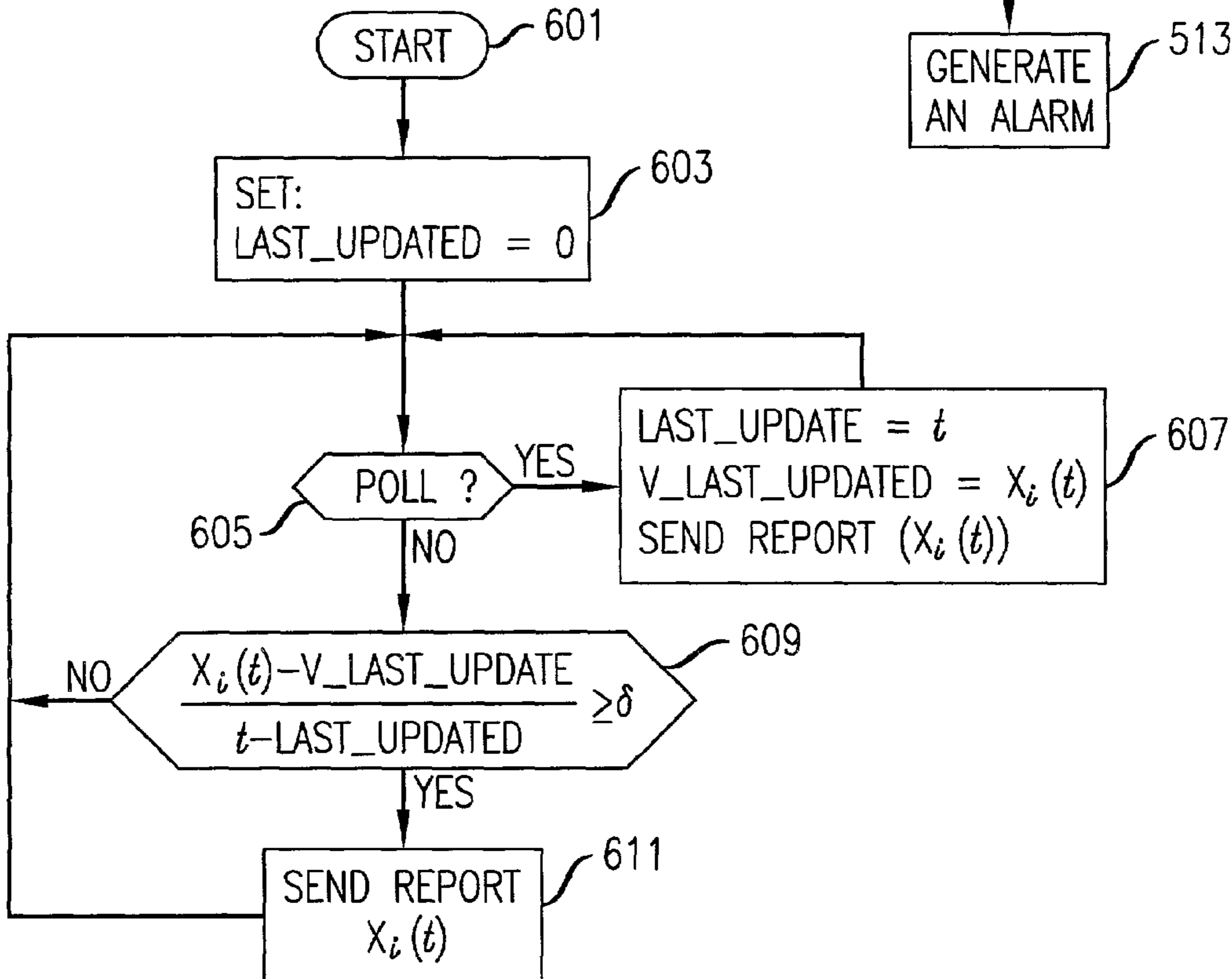
ADVANCED RATE NODE PROCESS
