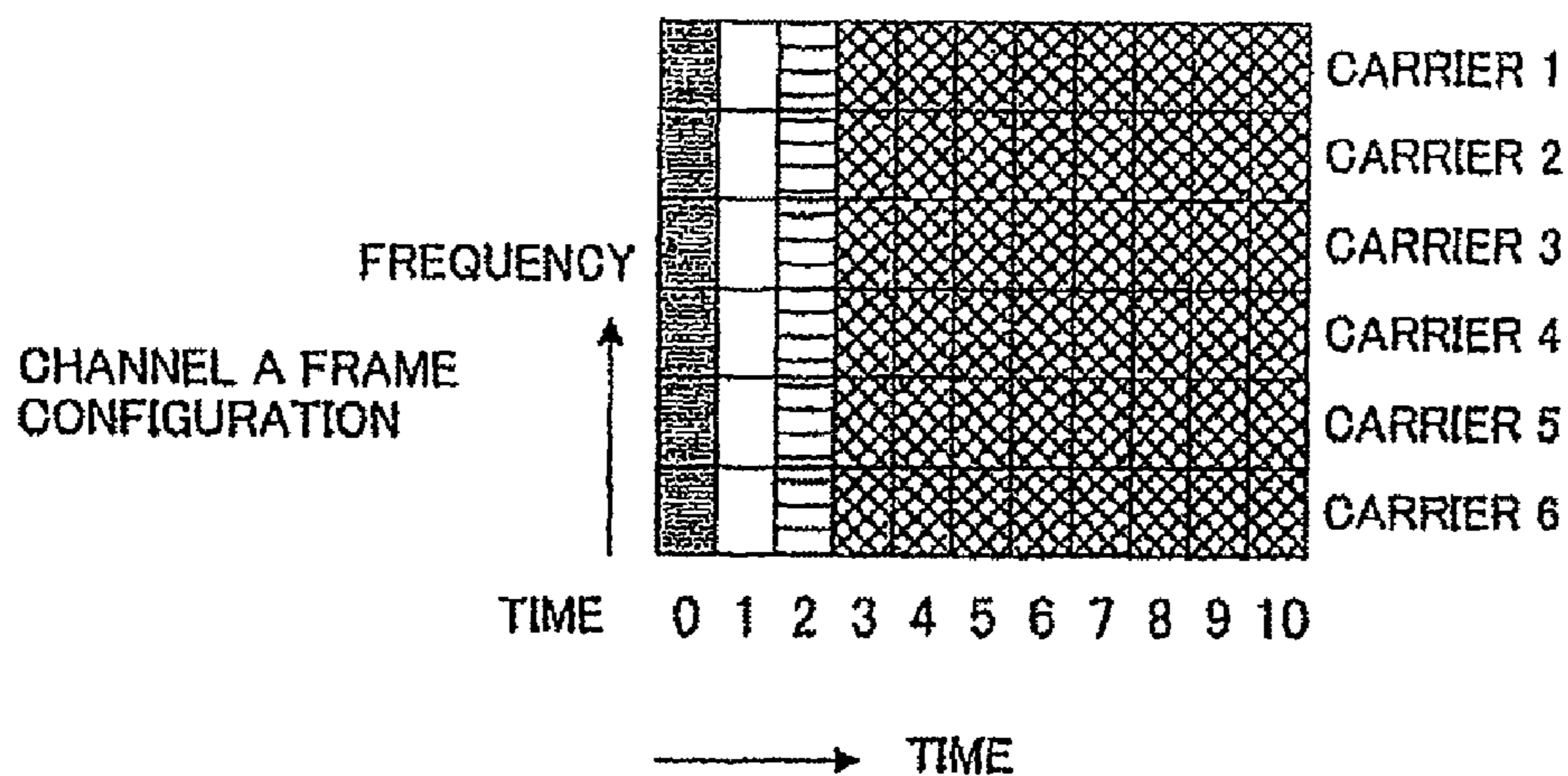
BASE STATION TRANSMIT SIGNAL FRAME CONFIGURATION
