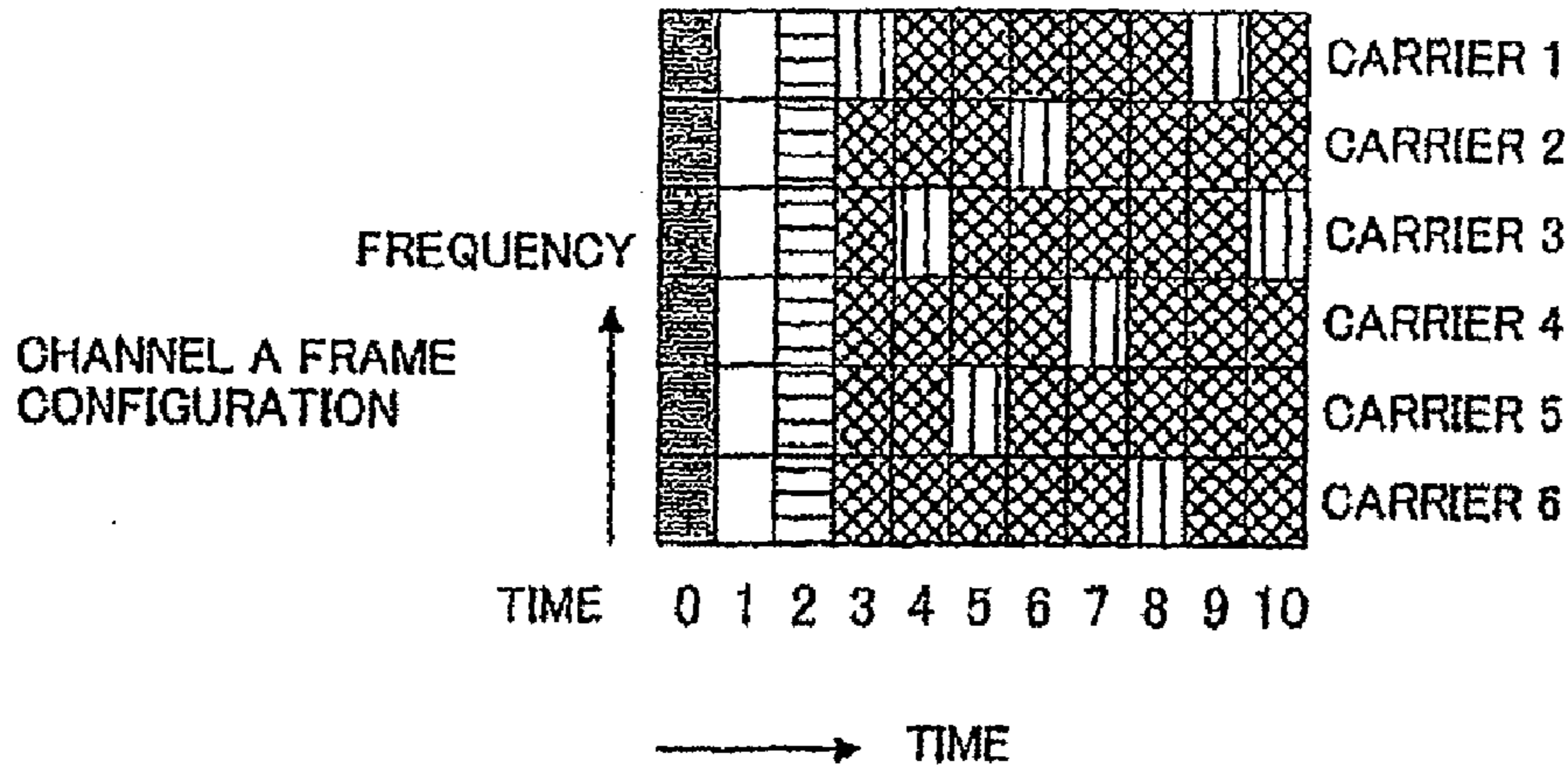
BASE STATION TRANSMIT SIGNAL FRAME CONFIGURATION
