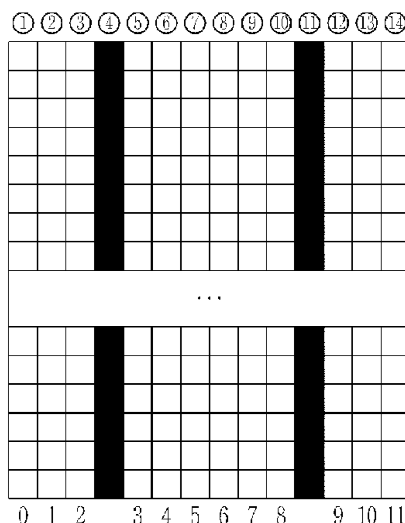
■ Resource element allocated for RS mapping
