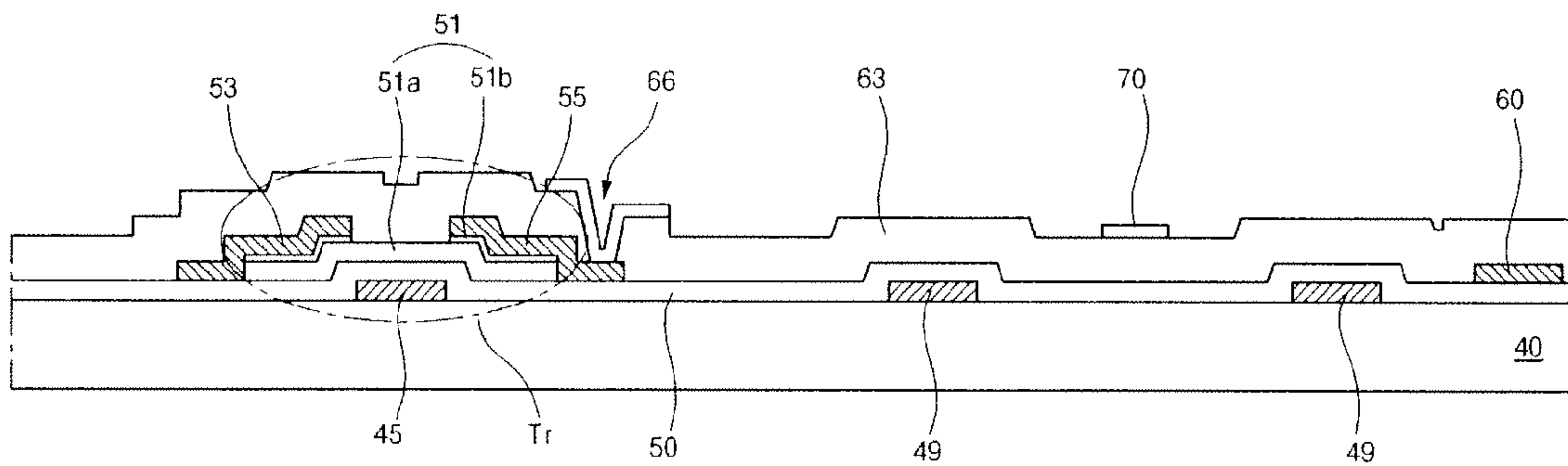
FIG. 4 Related Art
