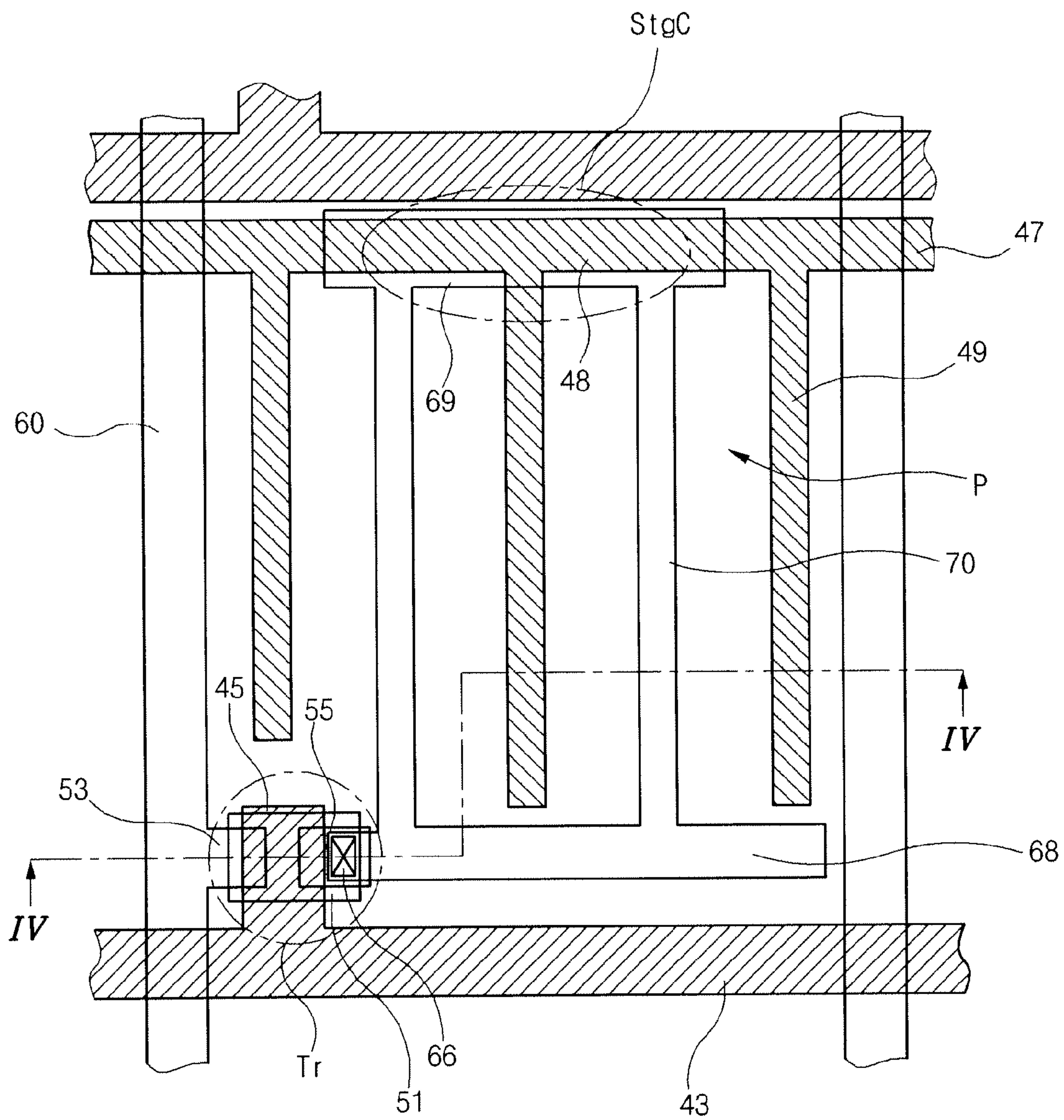
FIG 3 Related Art
