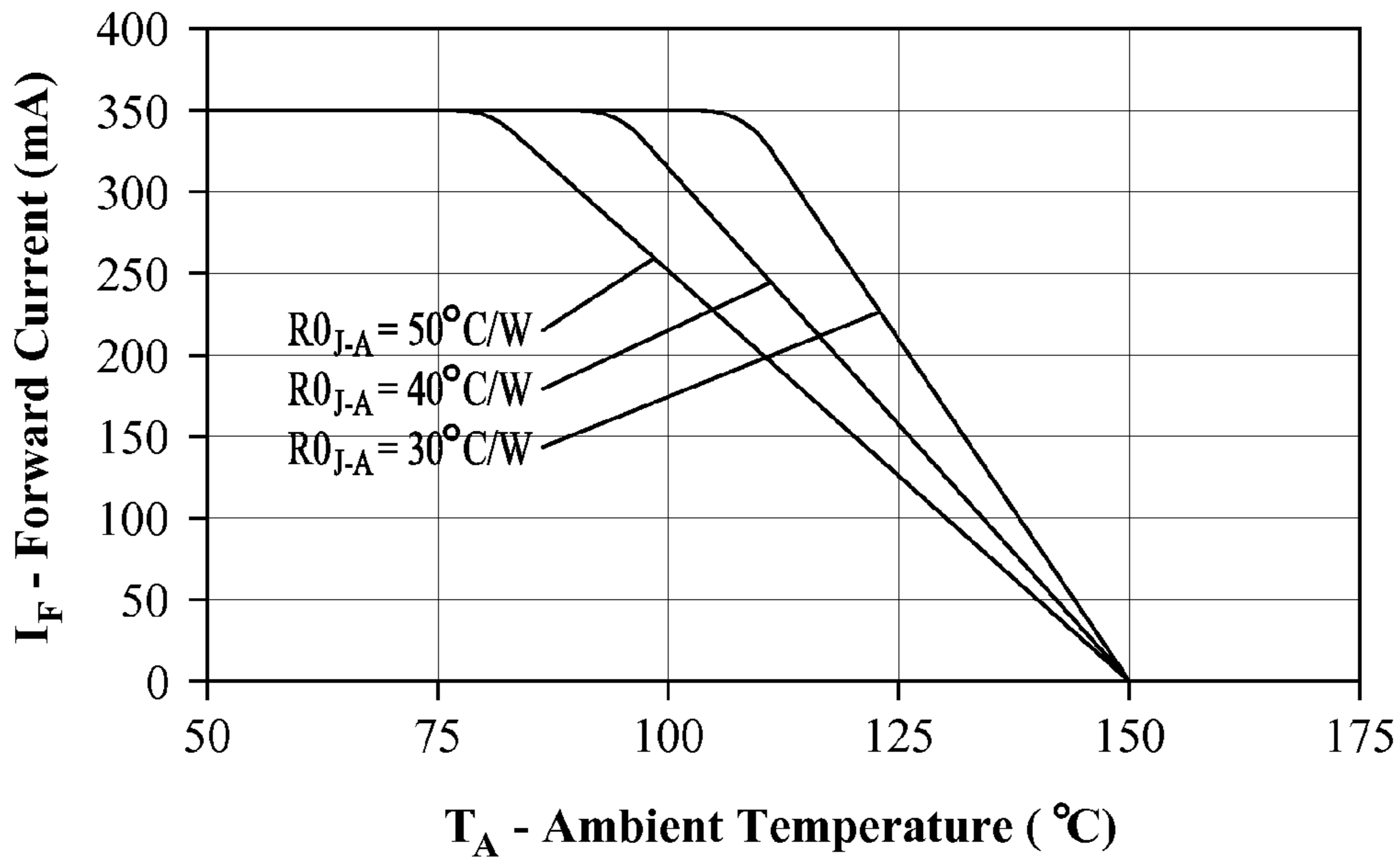
Current Derating Curve for 350 mA Drive Current White
