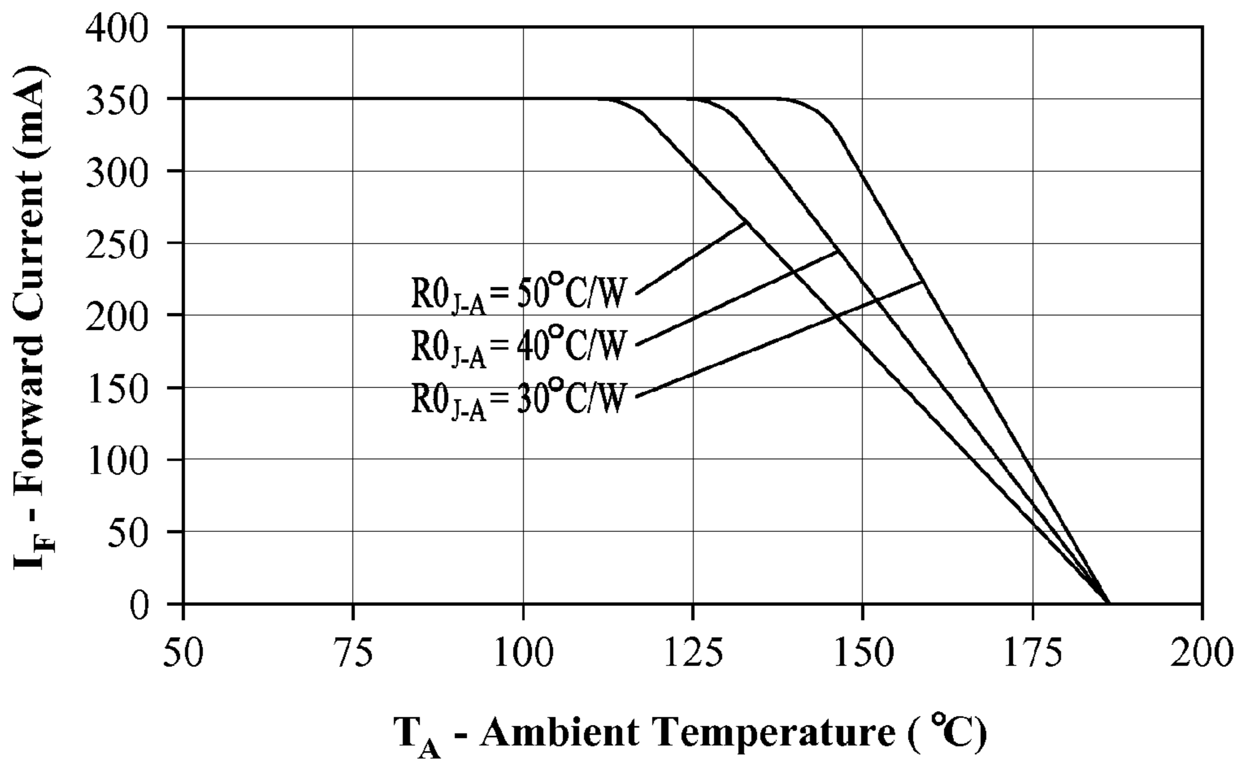
Current Derating Curve for 350 mA Drive Current Green, Cyan, Blue and Royal Blue
