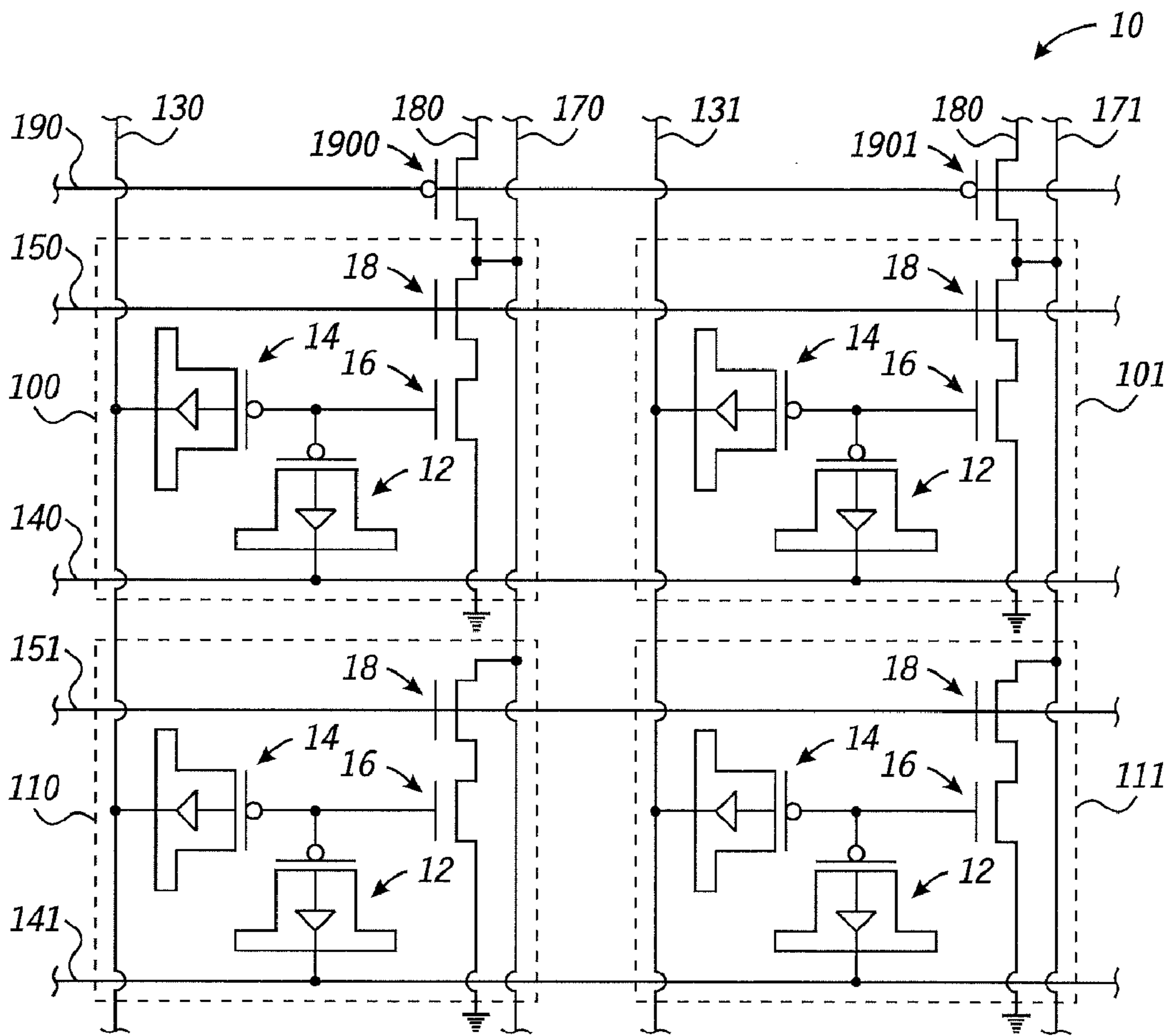
FIG. 1 (PRIOR ART)
