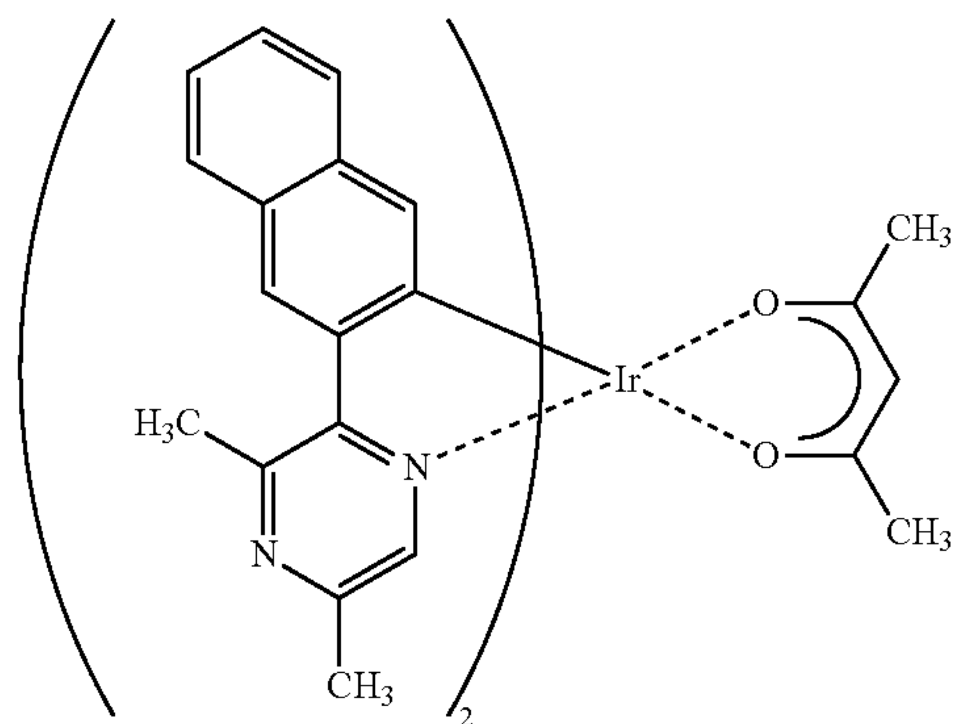
[Ir(dm2npr) 2 (acac)]
