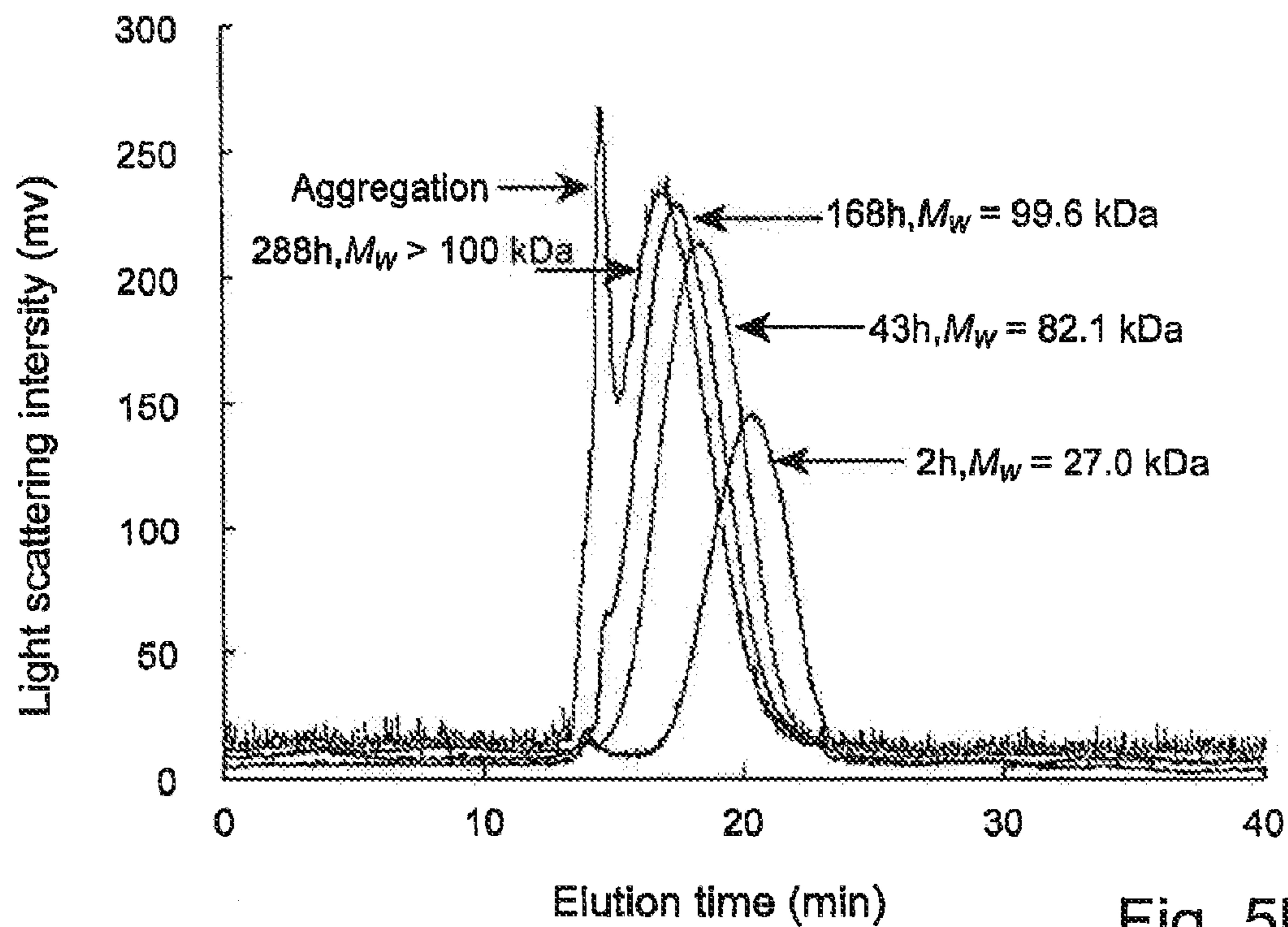
Polymerization control by adjusting polymerization time
