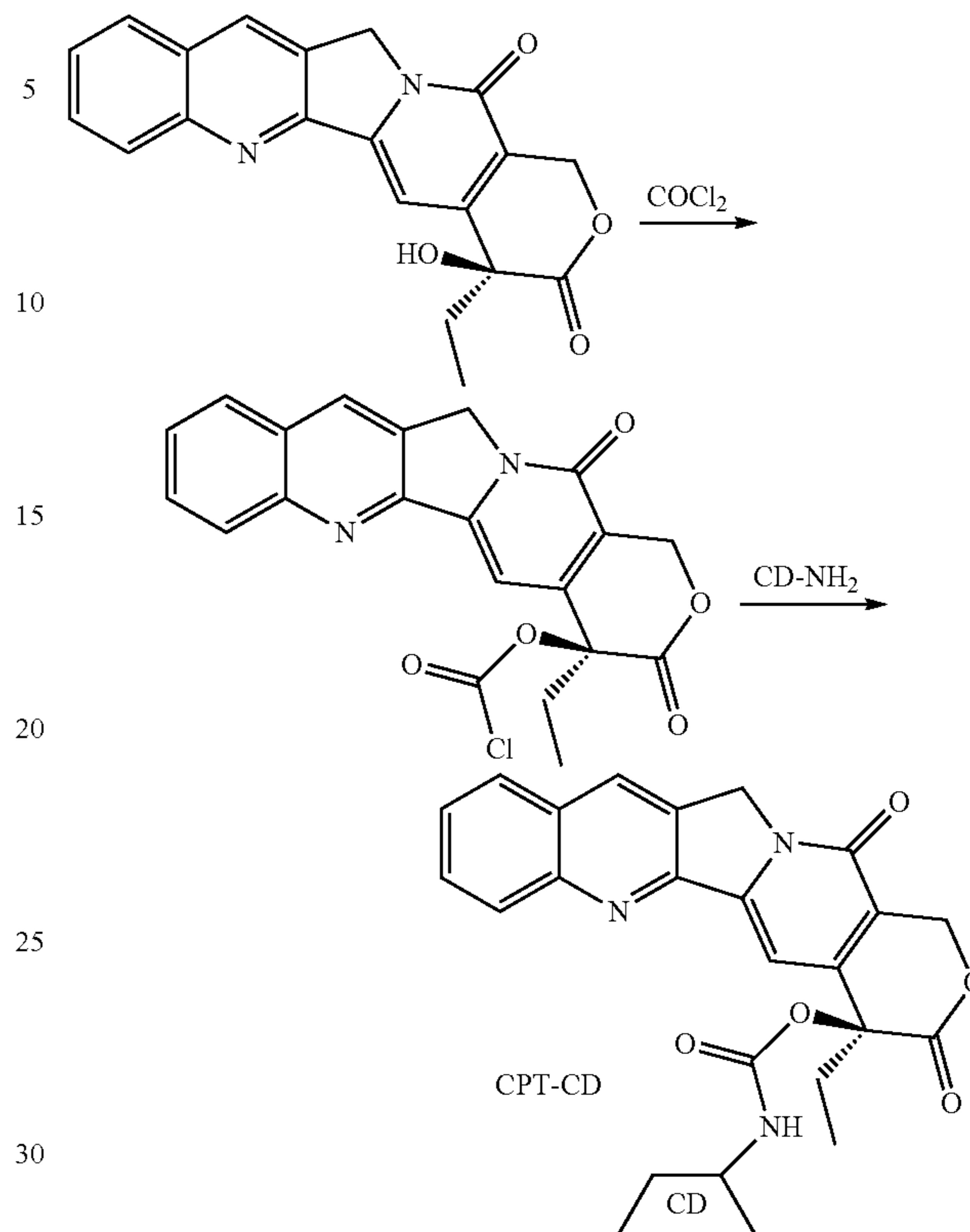
Scheme I
