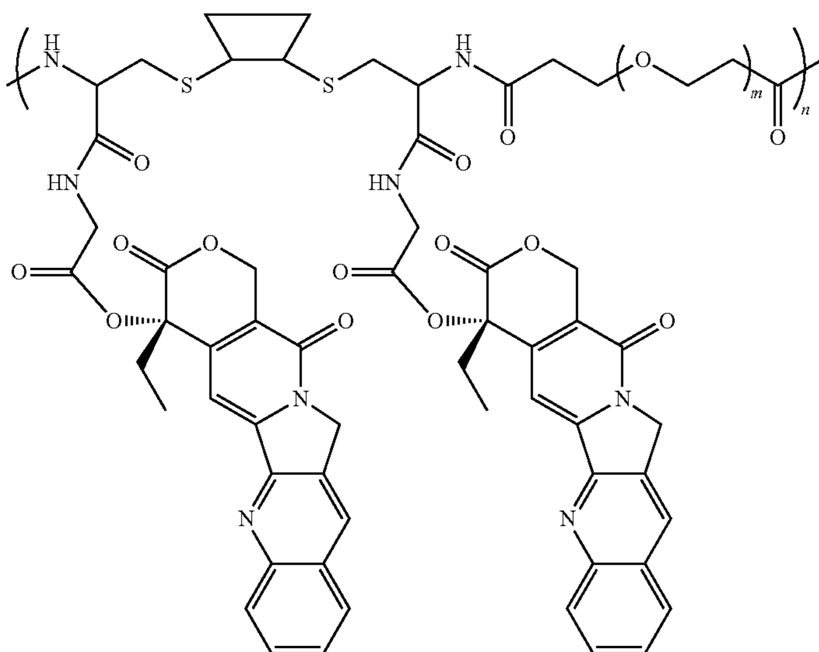
Scheme XXXXIII
