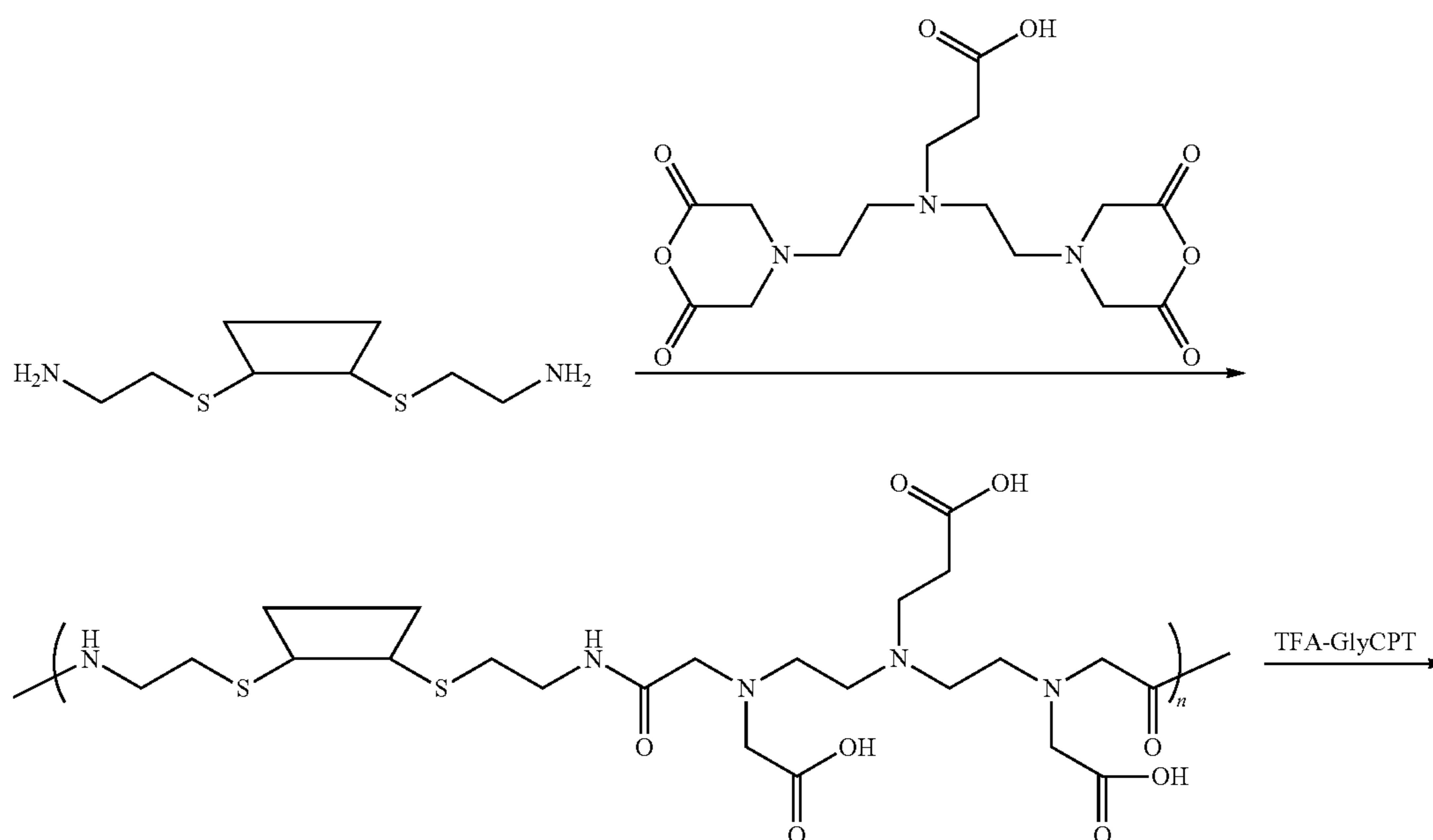
Scheme XXIX
