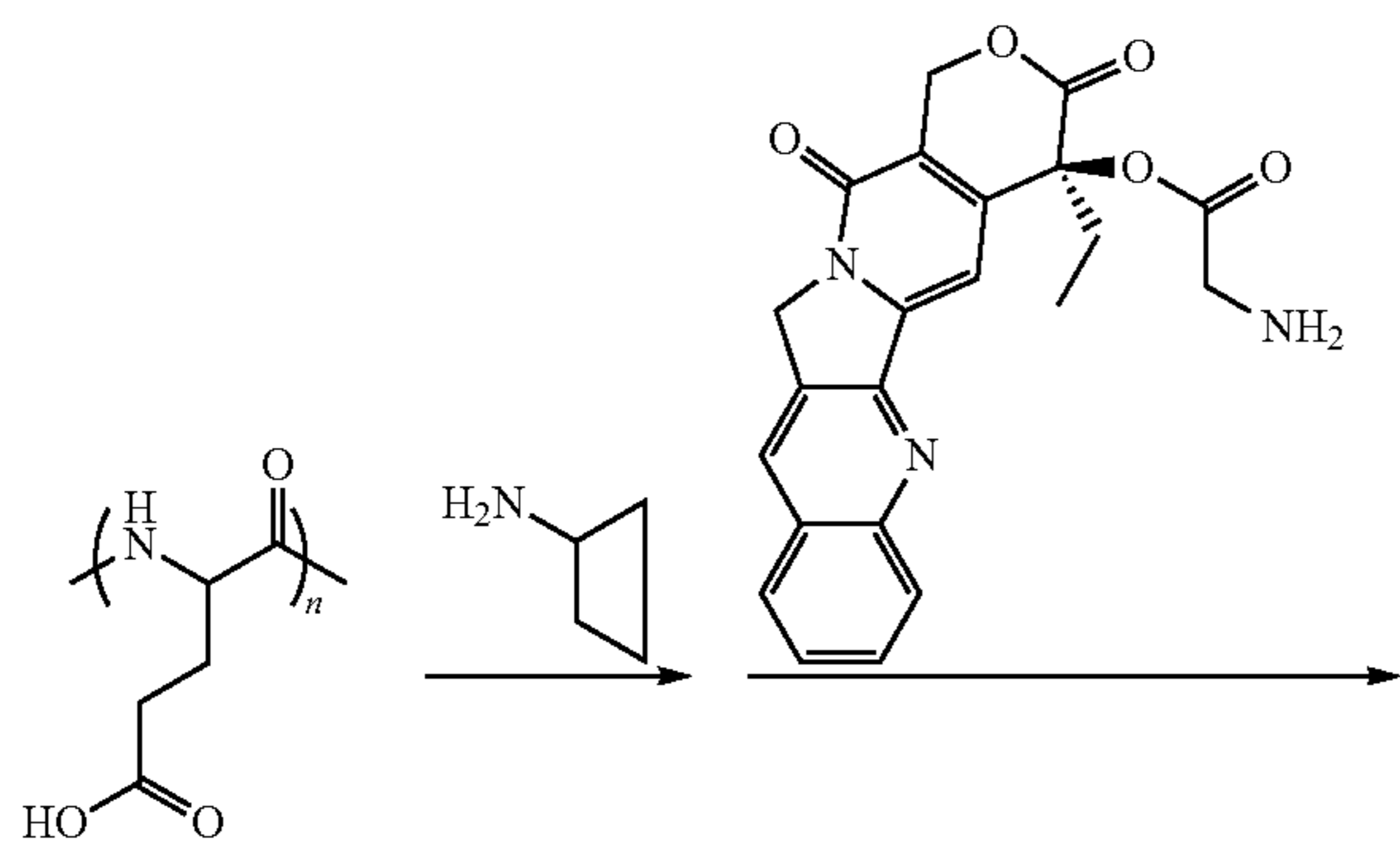
Scheme XXXVII
