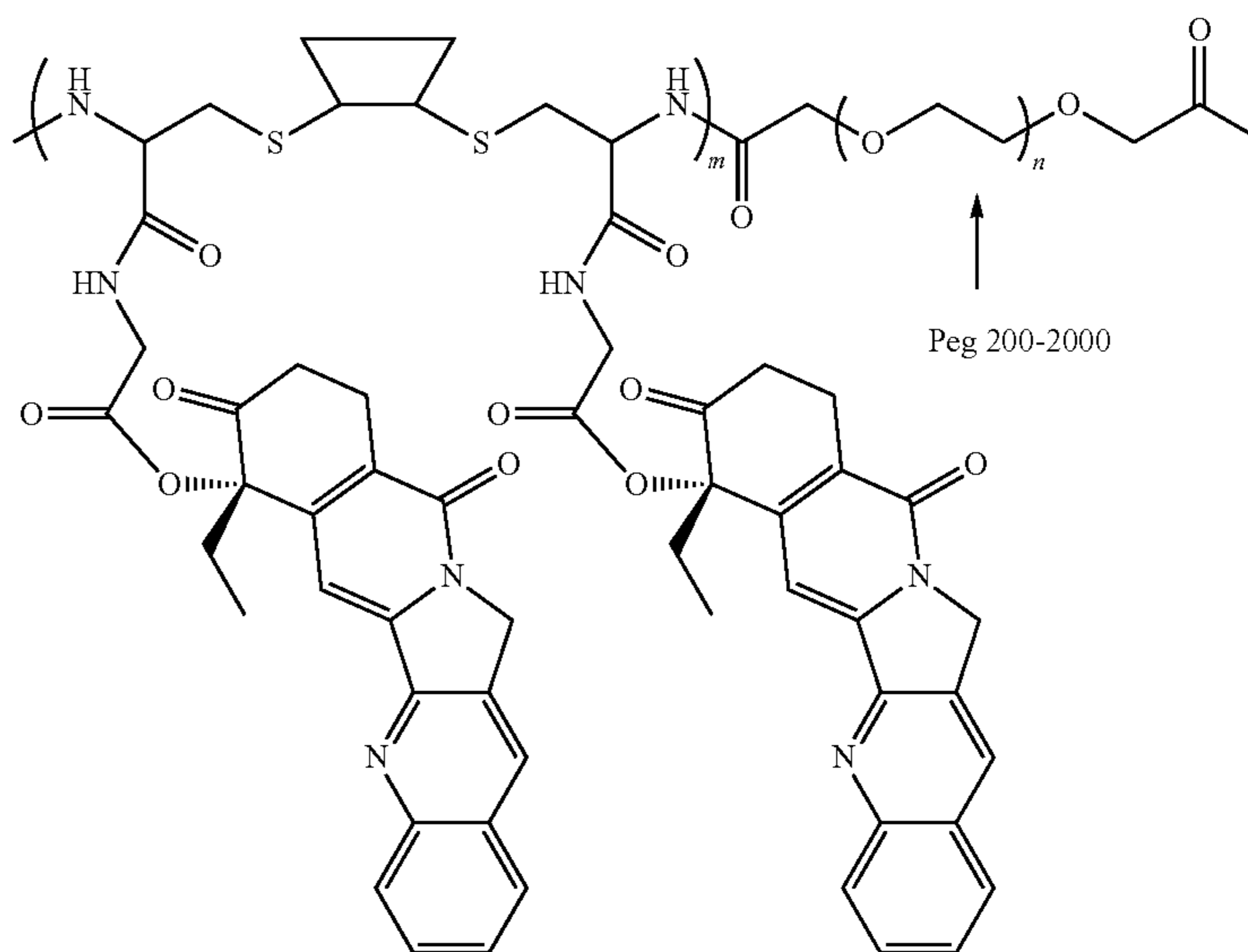
Scheme XXXXII
