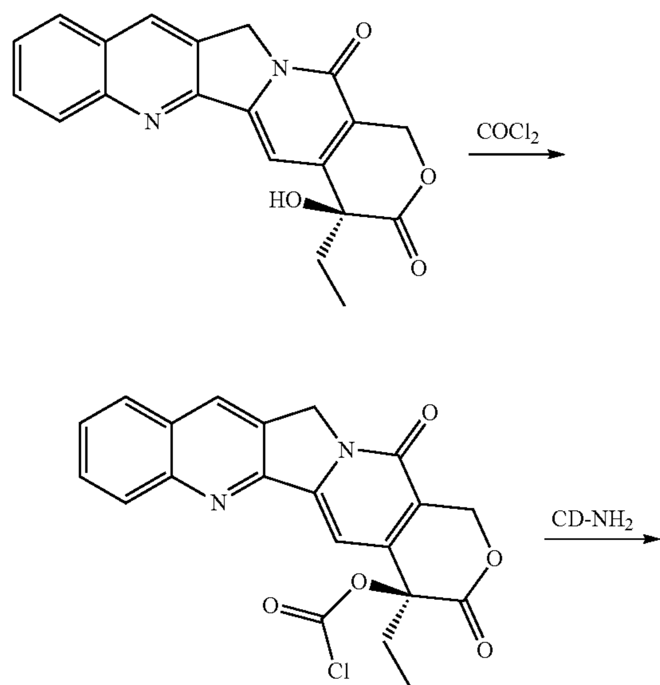
Scheme XXVIII
