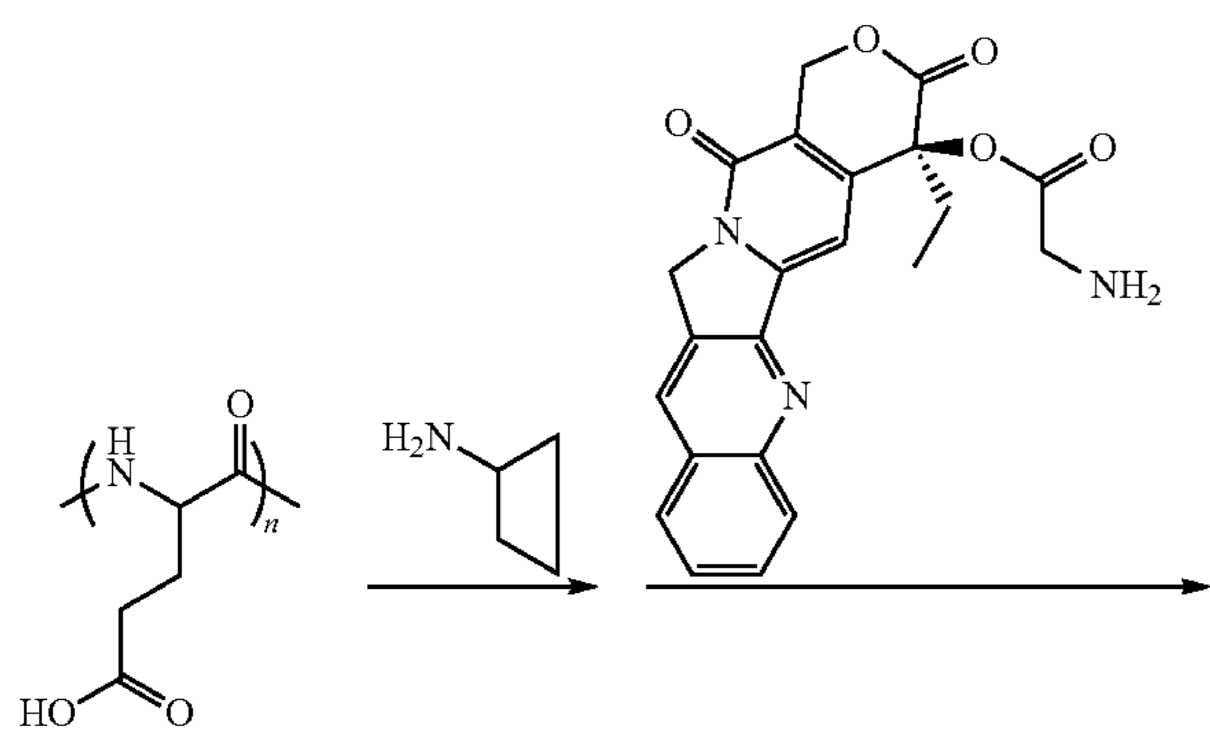
Scheme XXXVII
