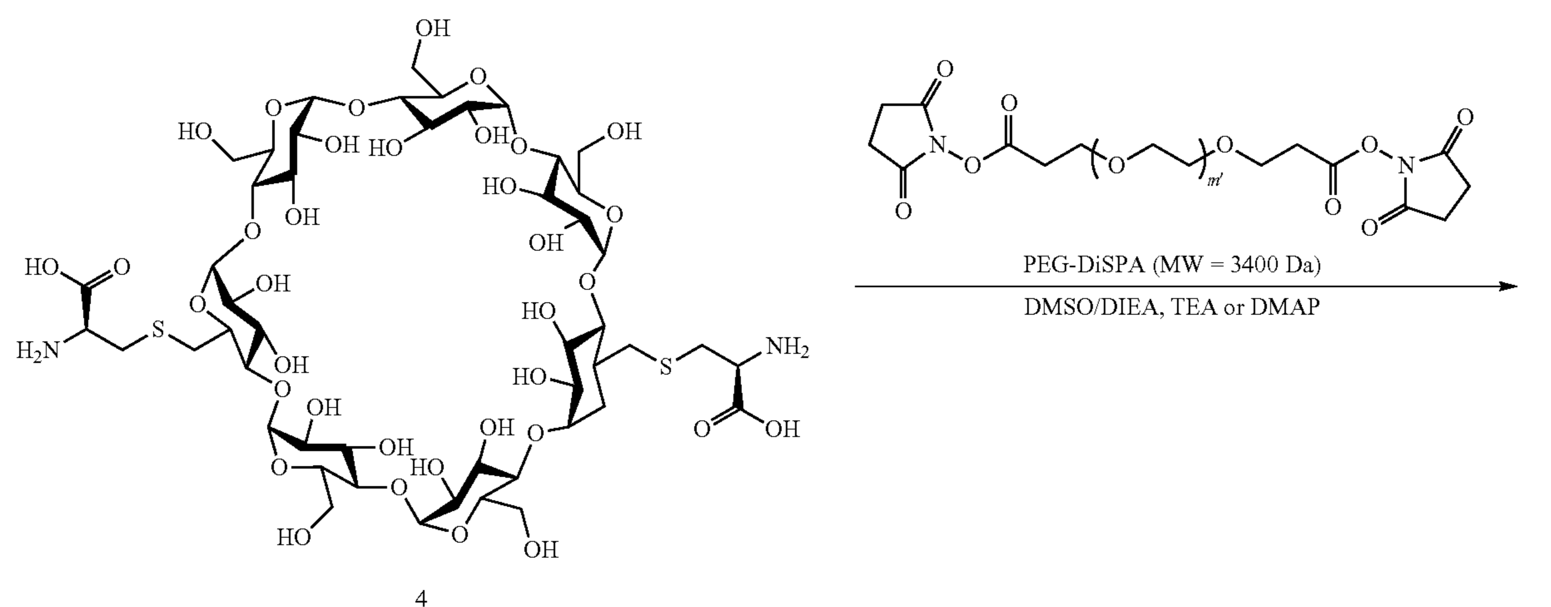
Scheme XXXVIIIa
