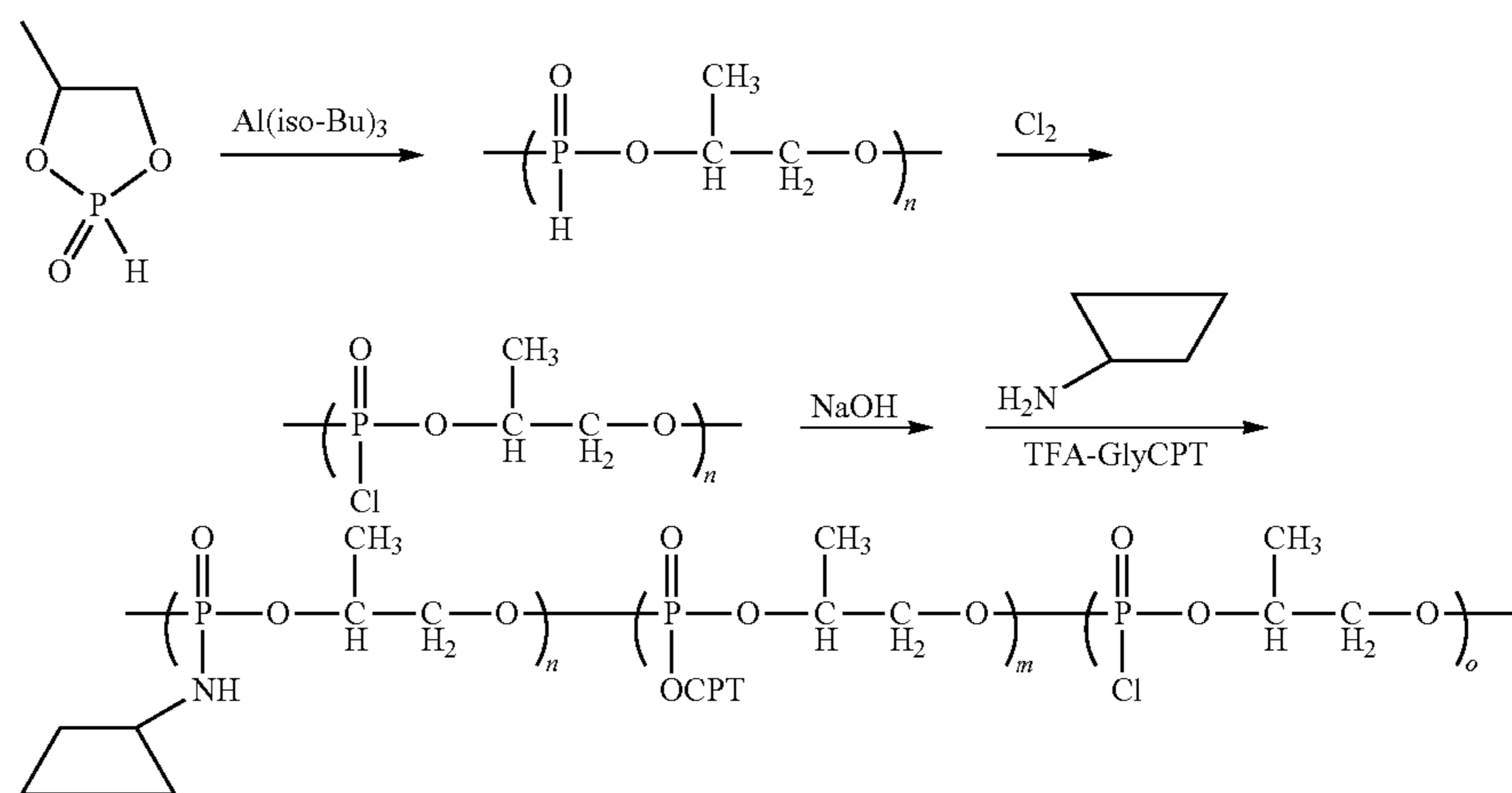
Scheme XXXIV
