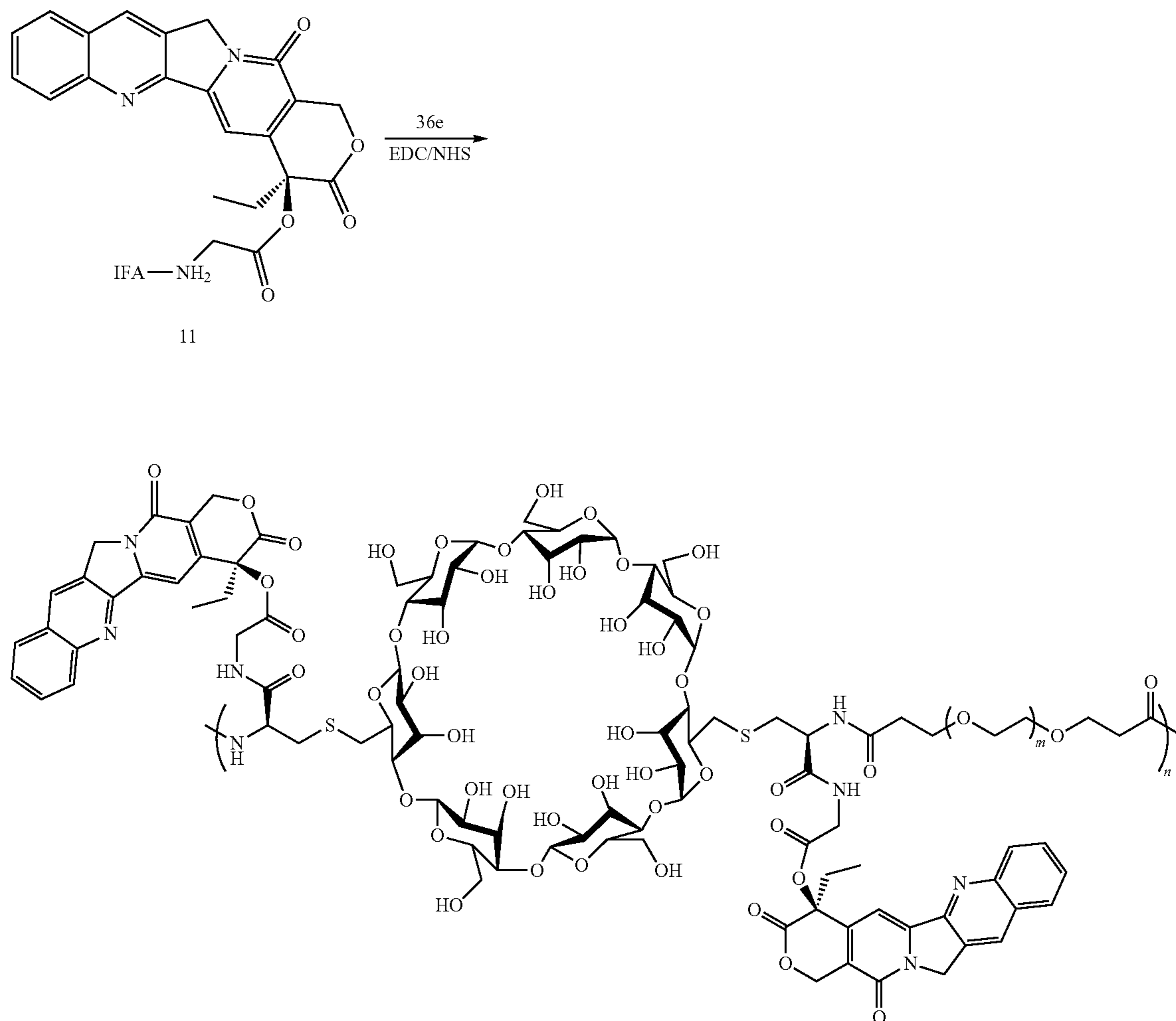
Scheme XXXIX
