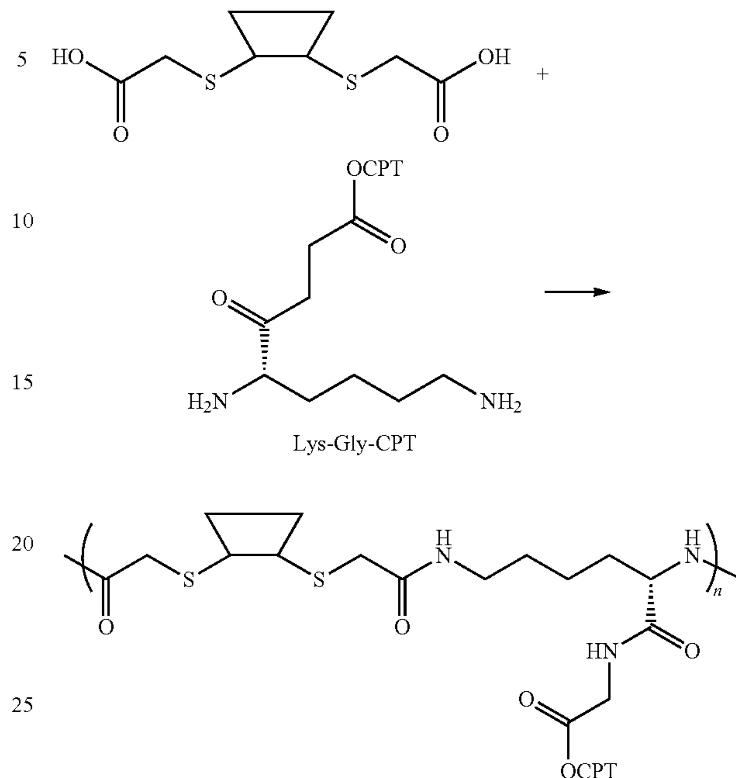
Scheme VIII
