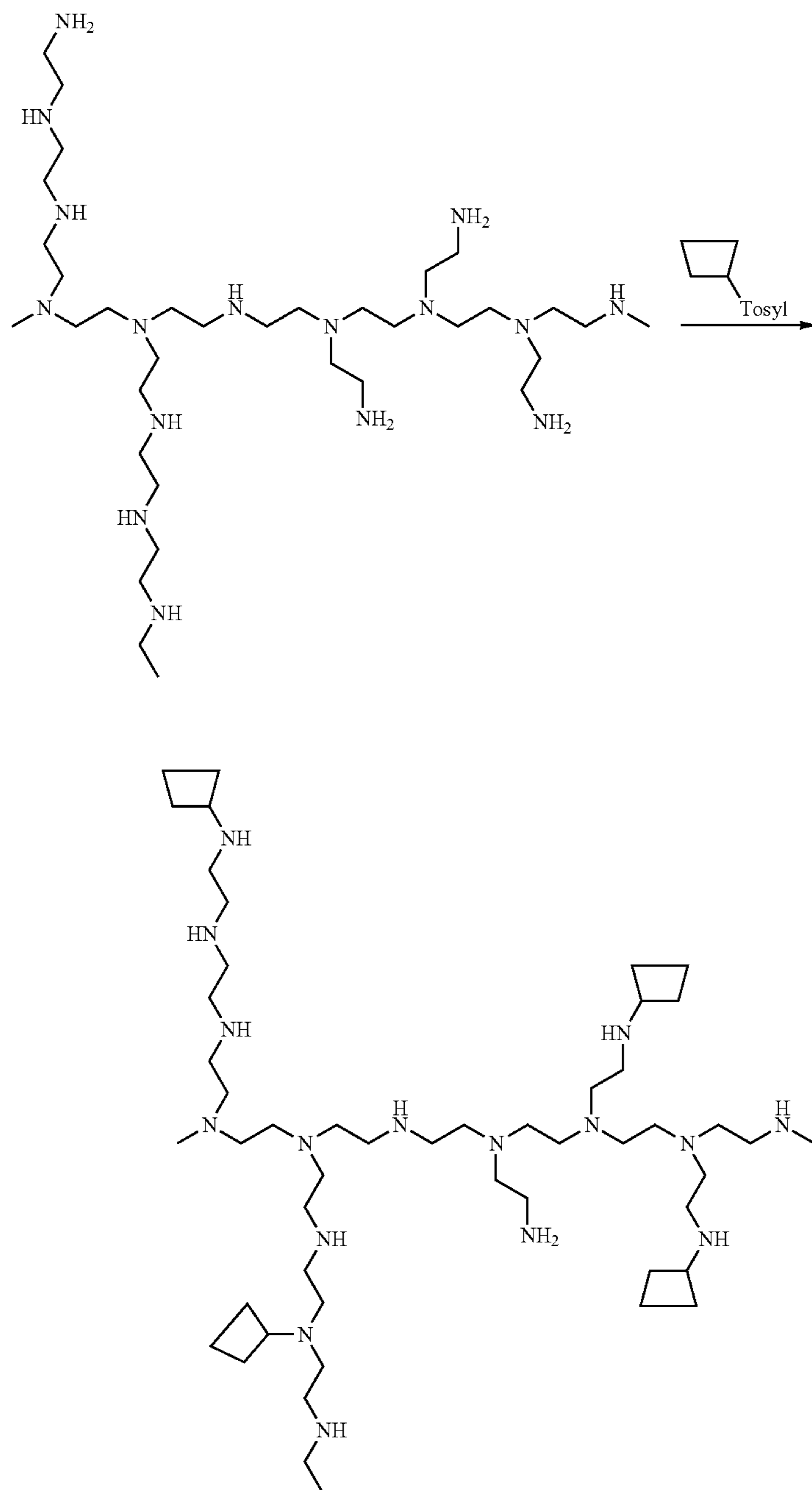
Scheme XXXXIV
