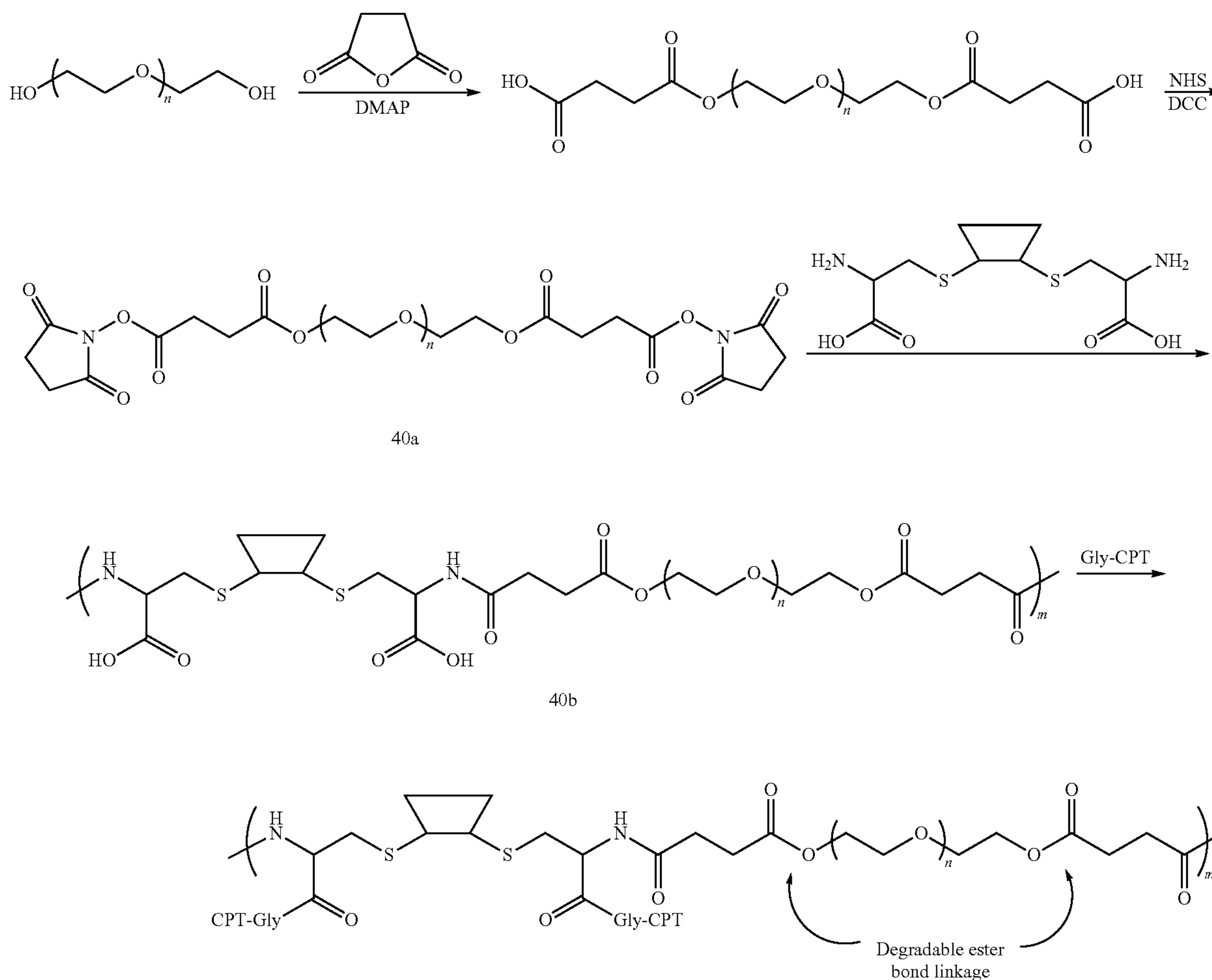
Scheme XXXXI
