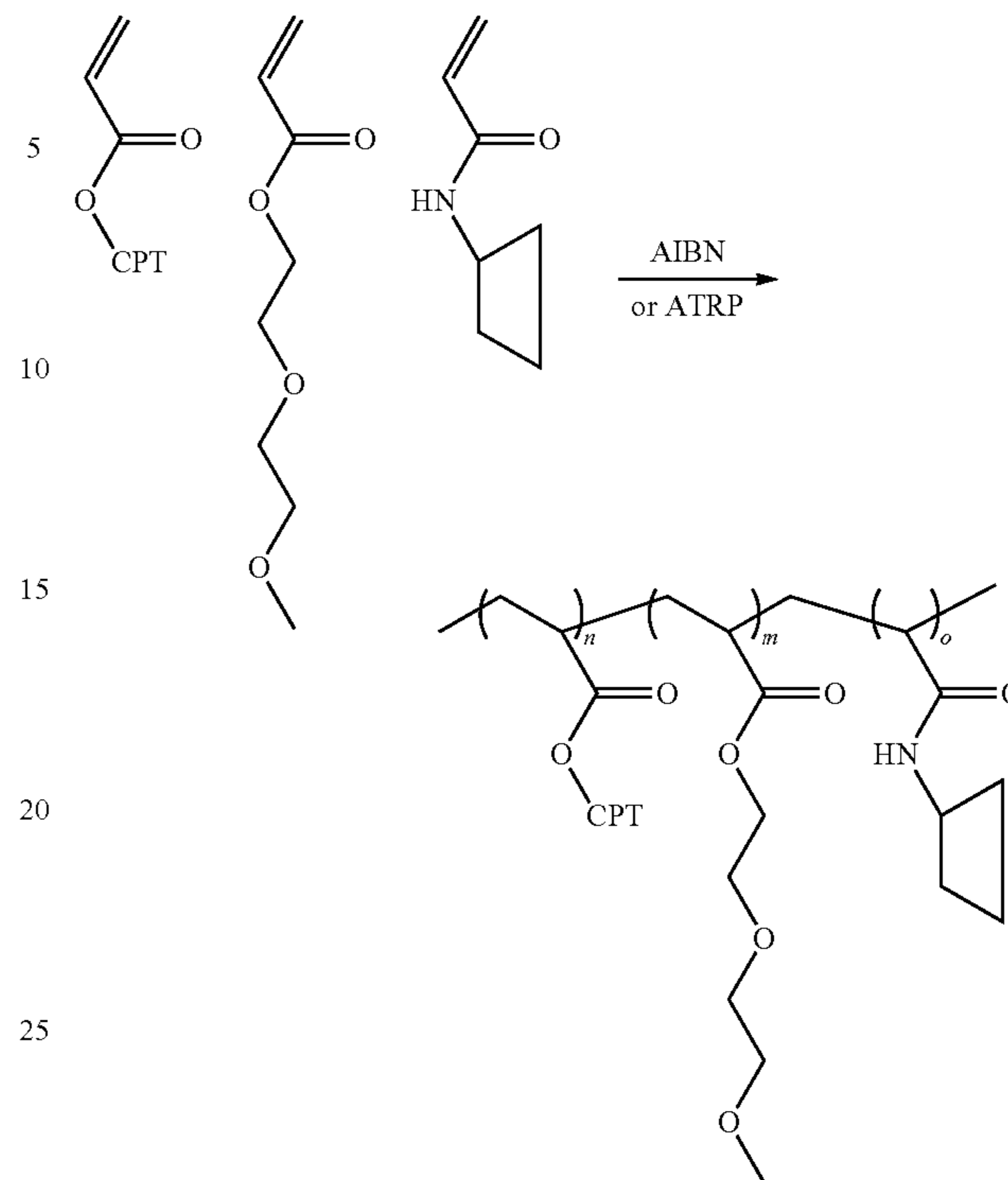
Scheme X
