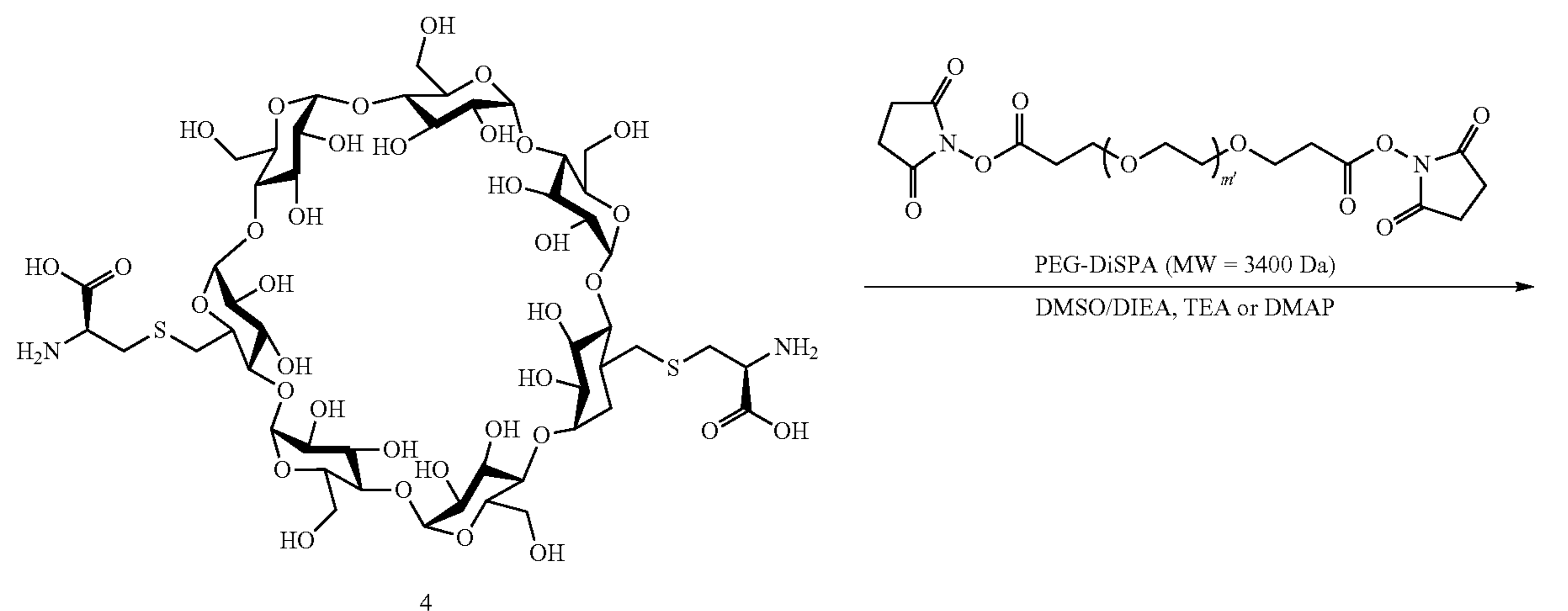
Scheme XXXVIIIa
