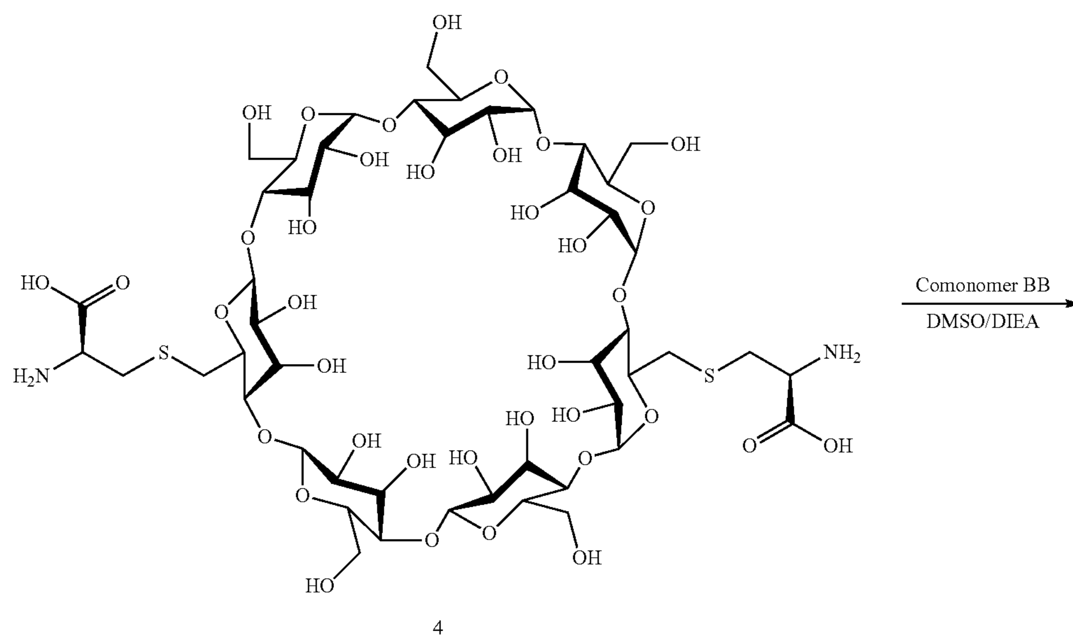
Scheme XXXVIIIb
