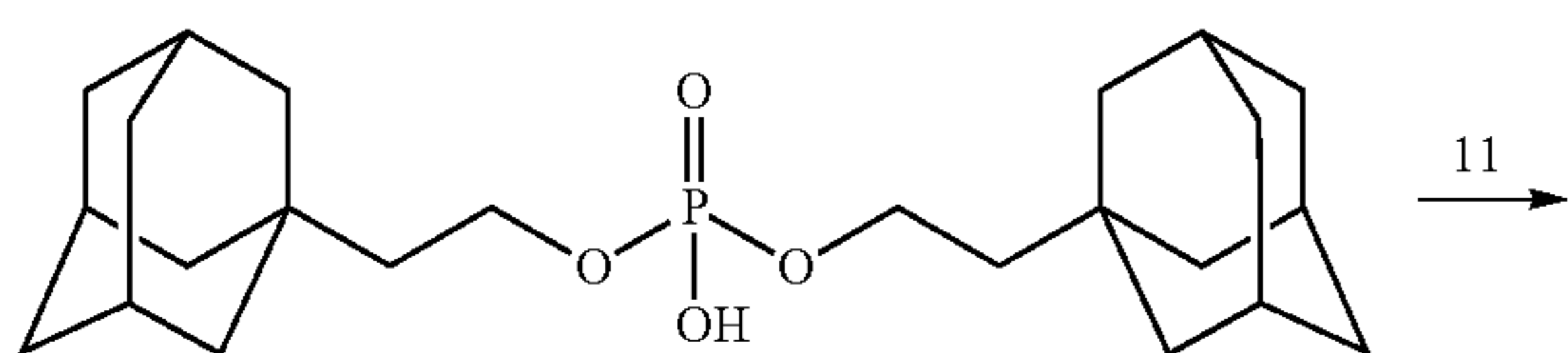
Scheme XXXXVIII
