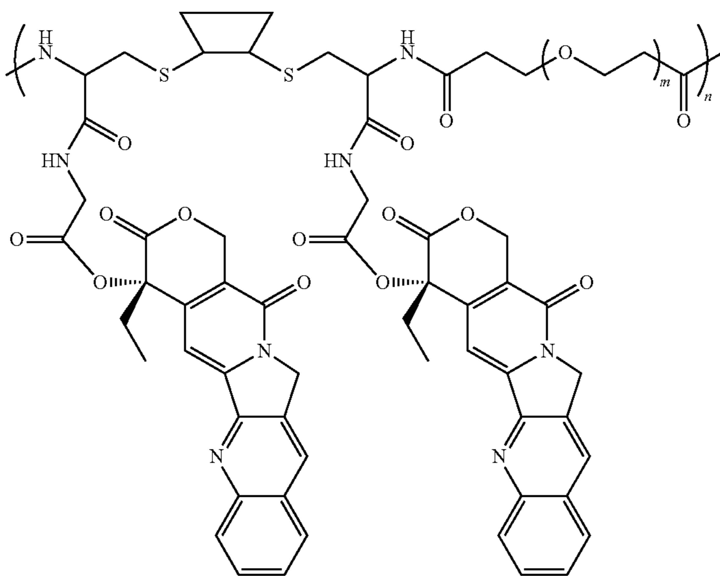
Scheme XXXXIII
