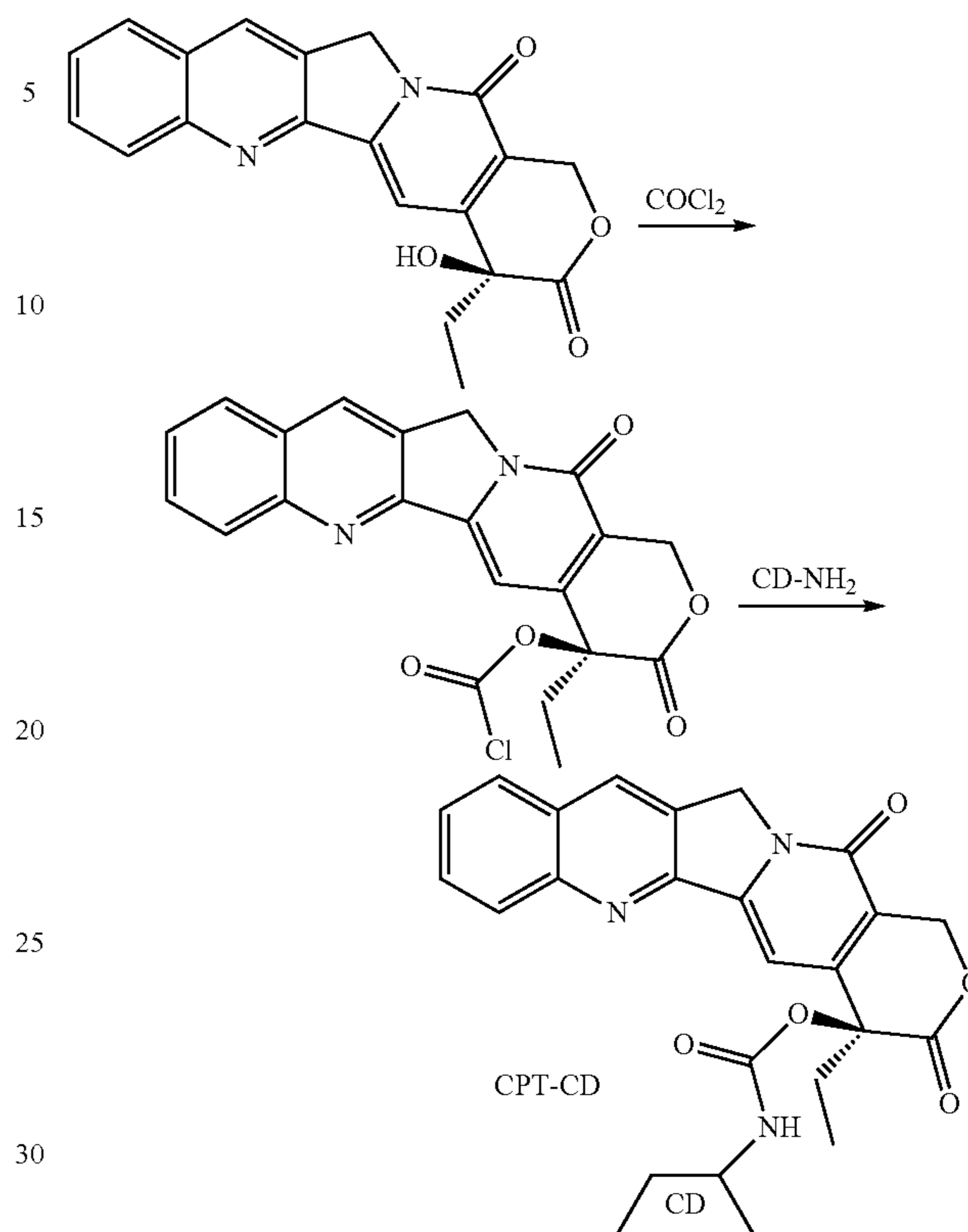
Scheme I
