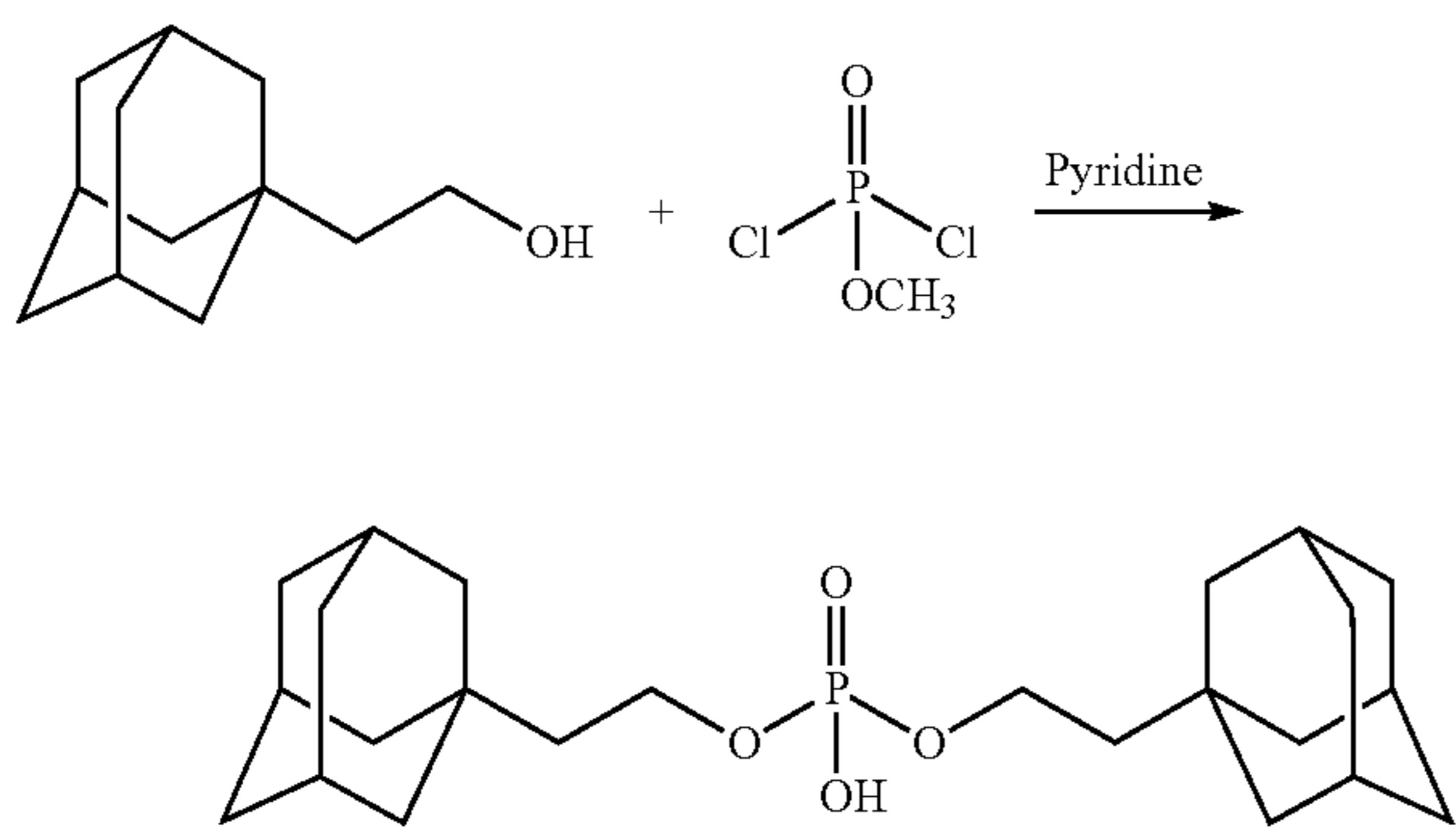
Scheme XXXXVII
