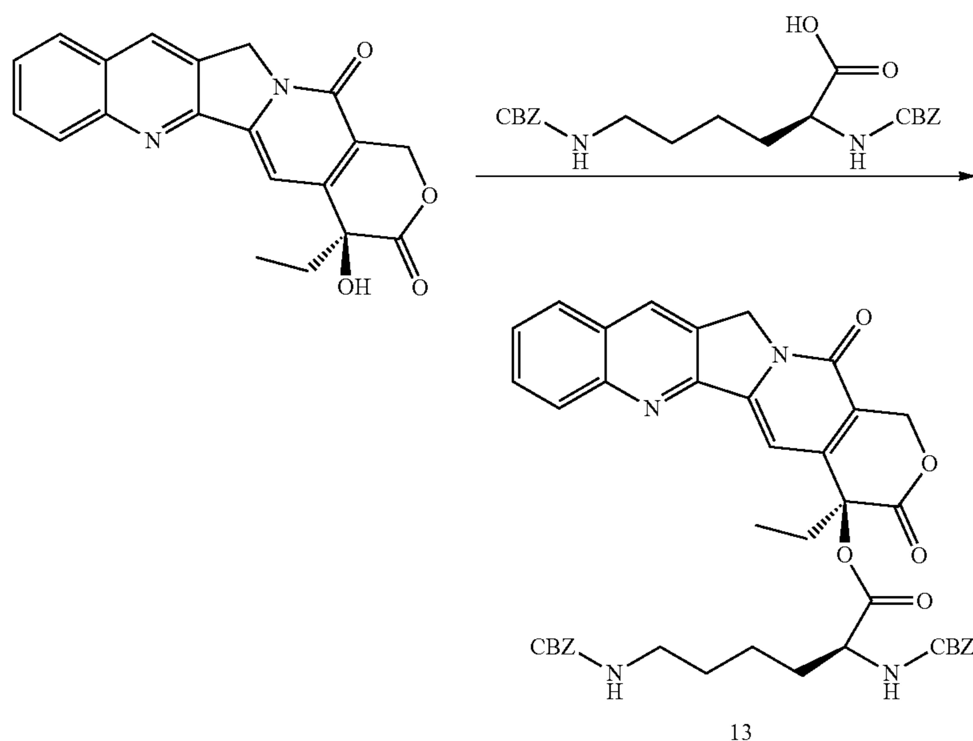
Scheme XXVII
