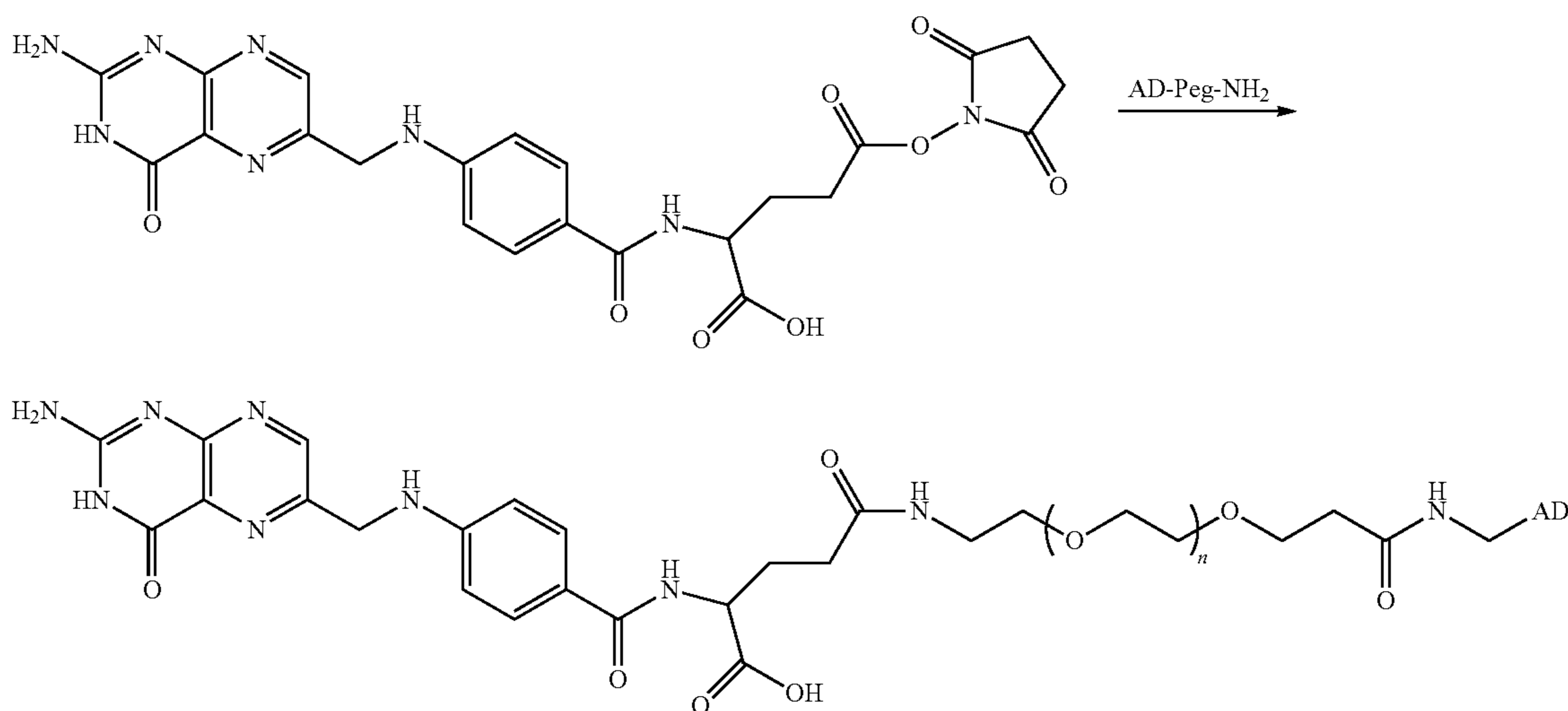
Scheme L
