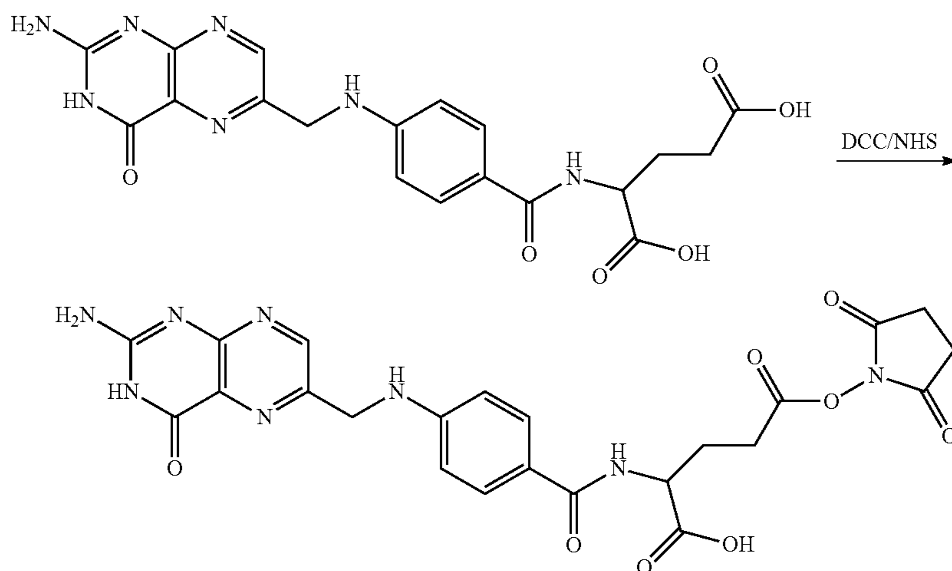
Scheme XXXXIX
