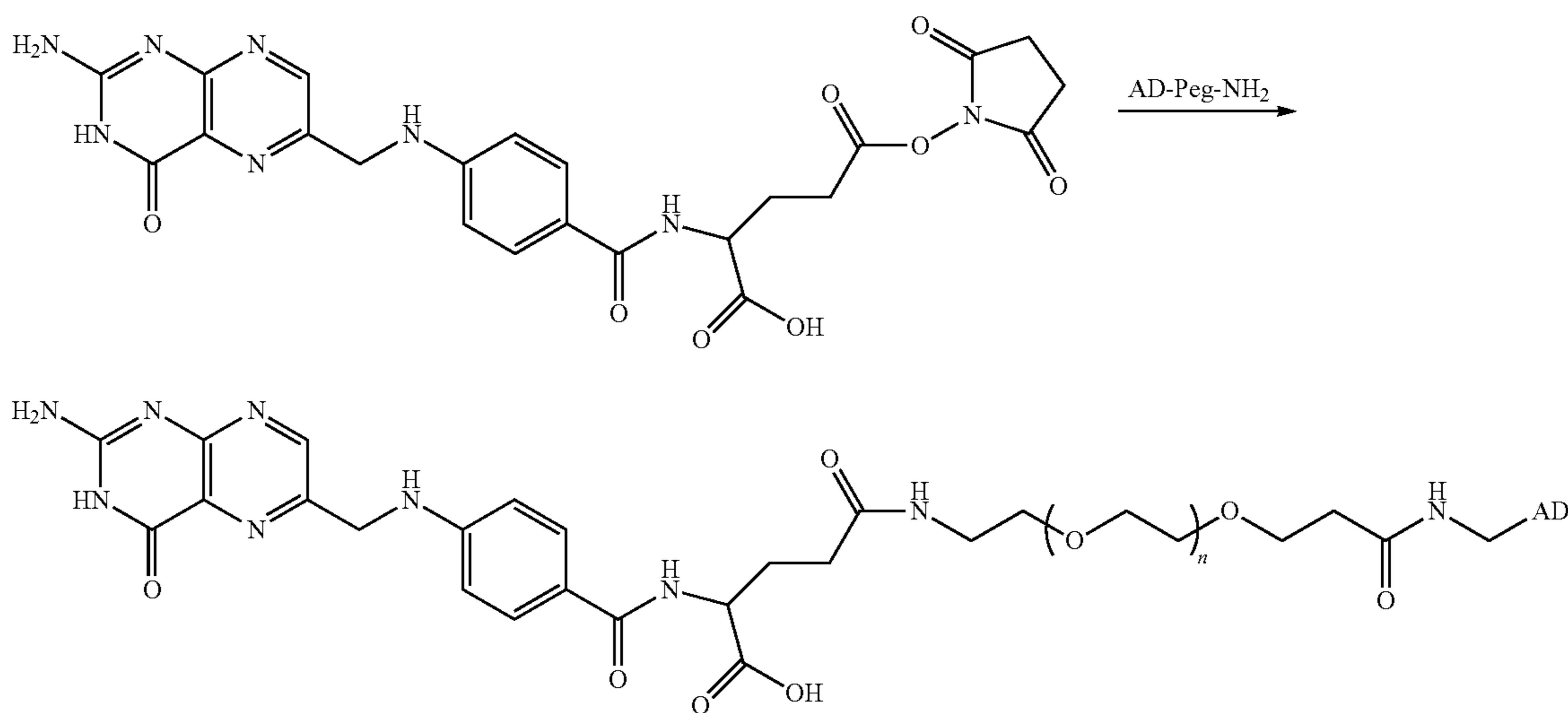
Scheme L
