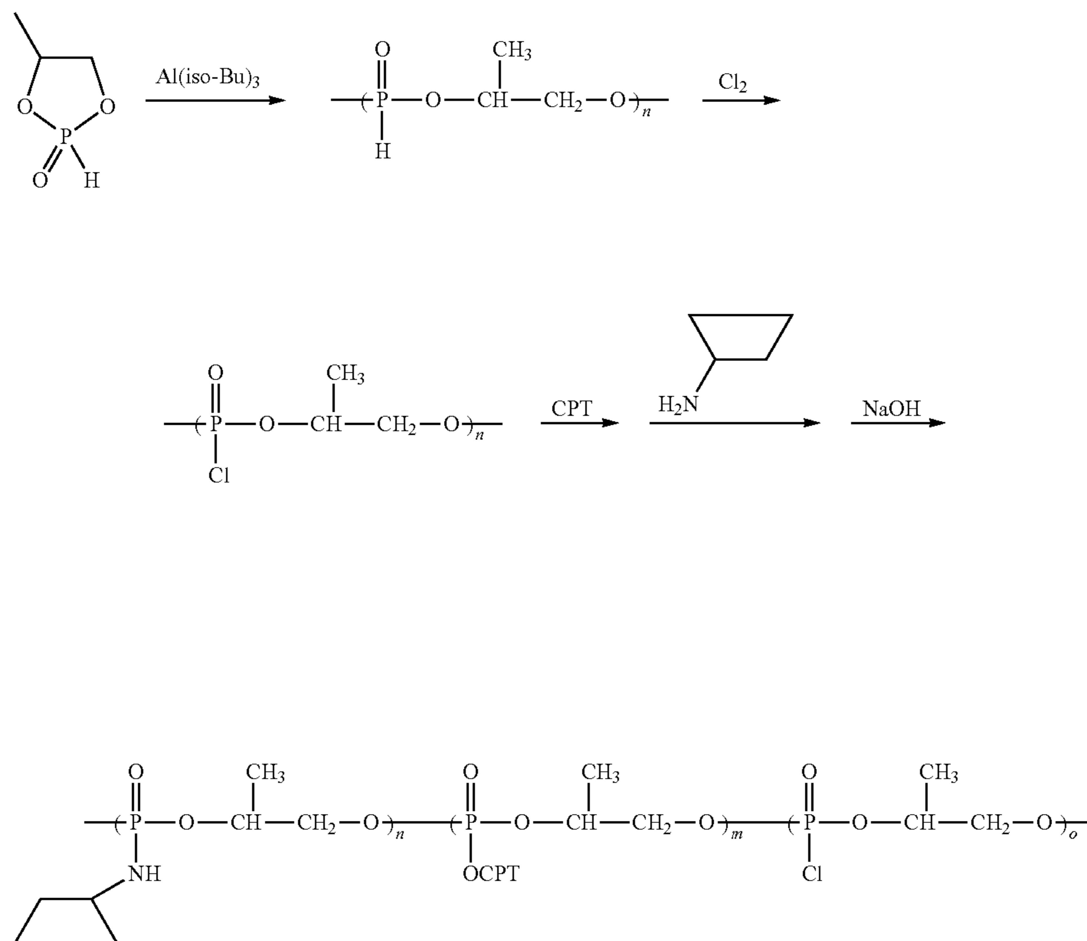
Scheme IX
