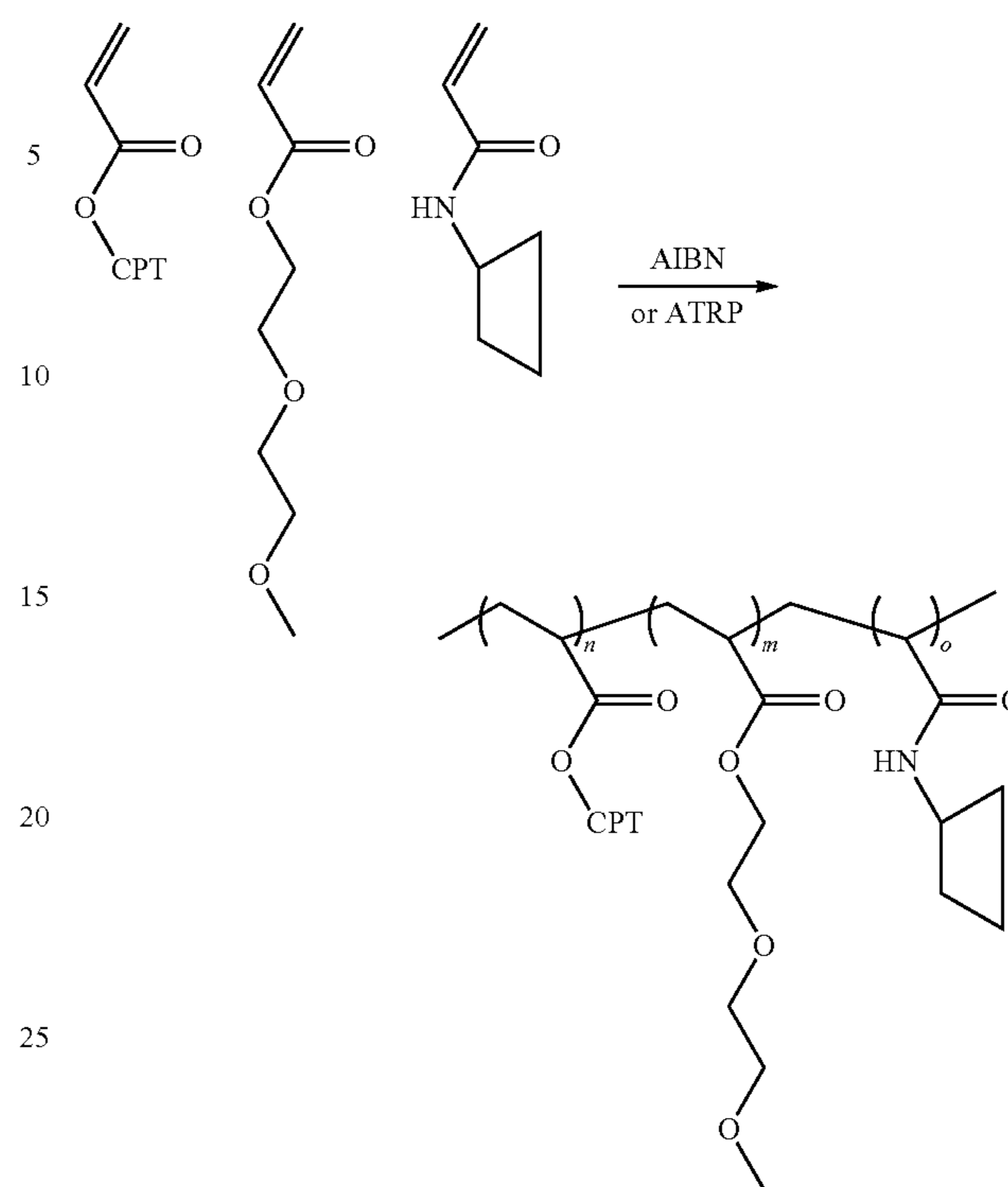
Scheme X
