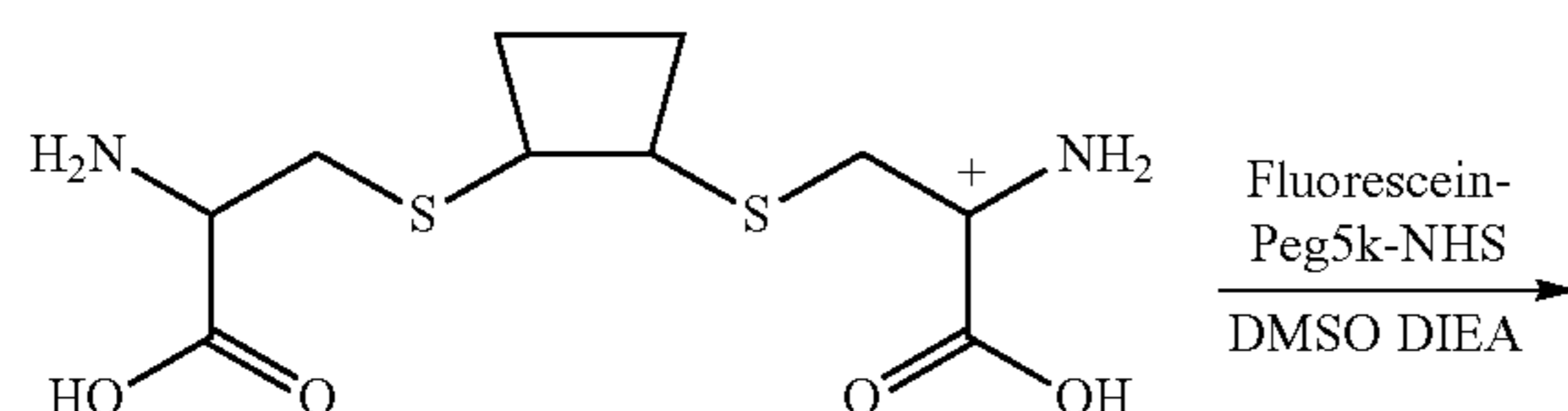
Scheme XXXX
