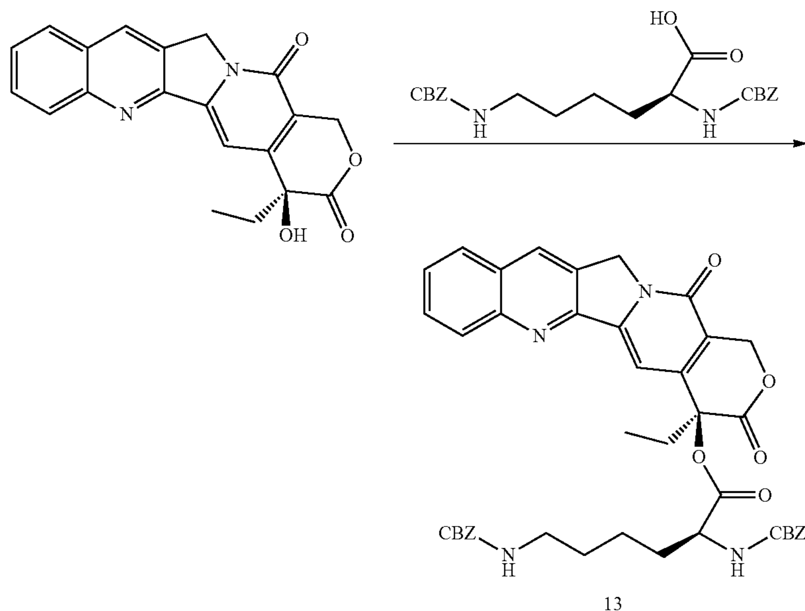
Scheme XXVII
