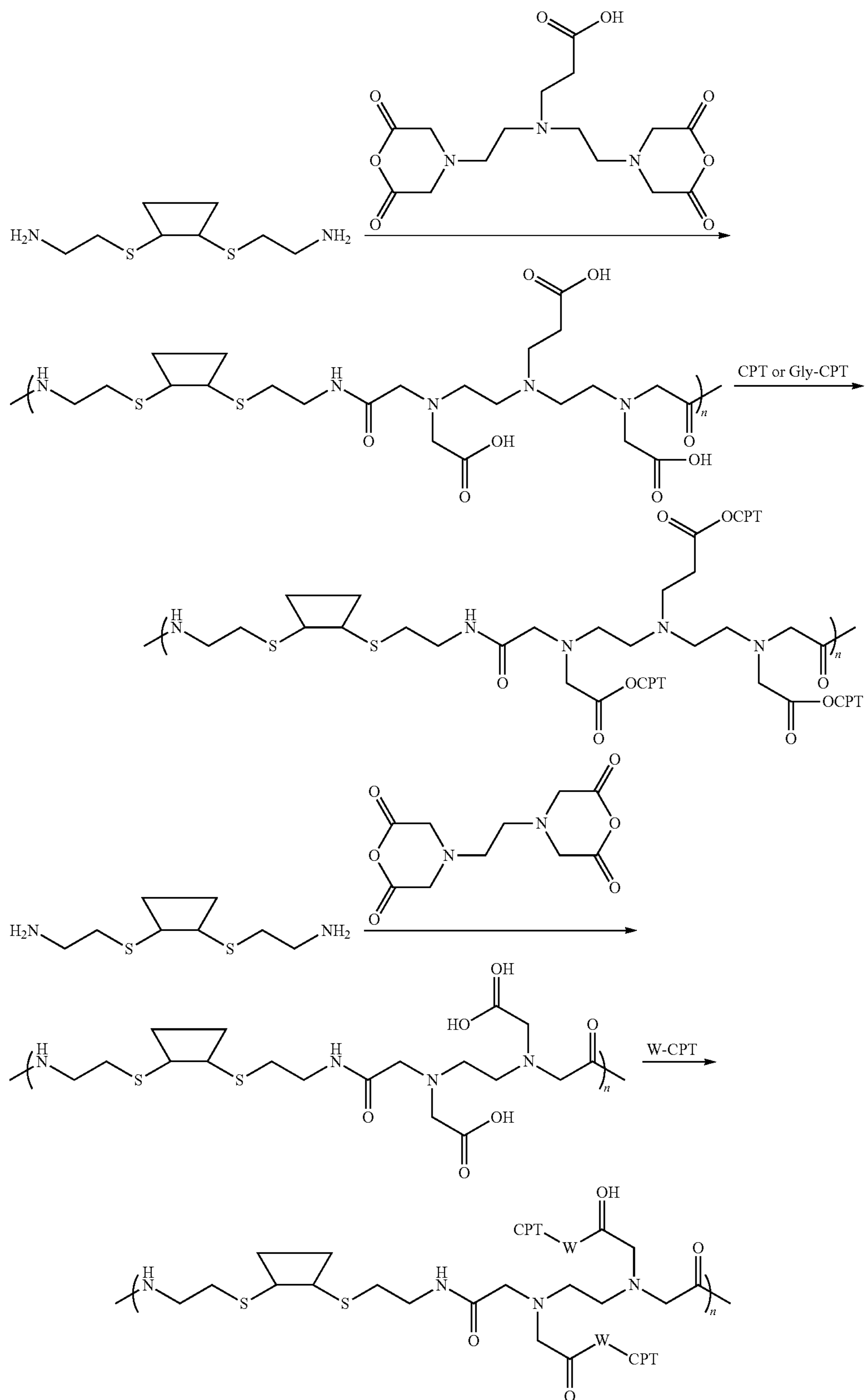
Scheme V
