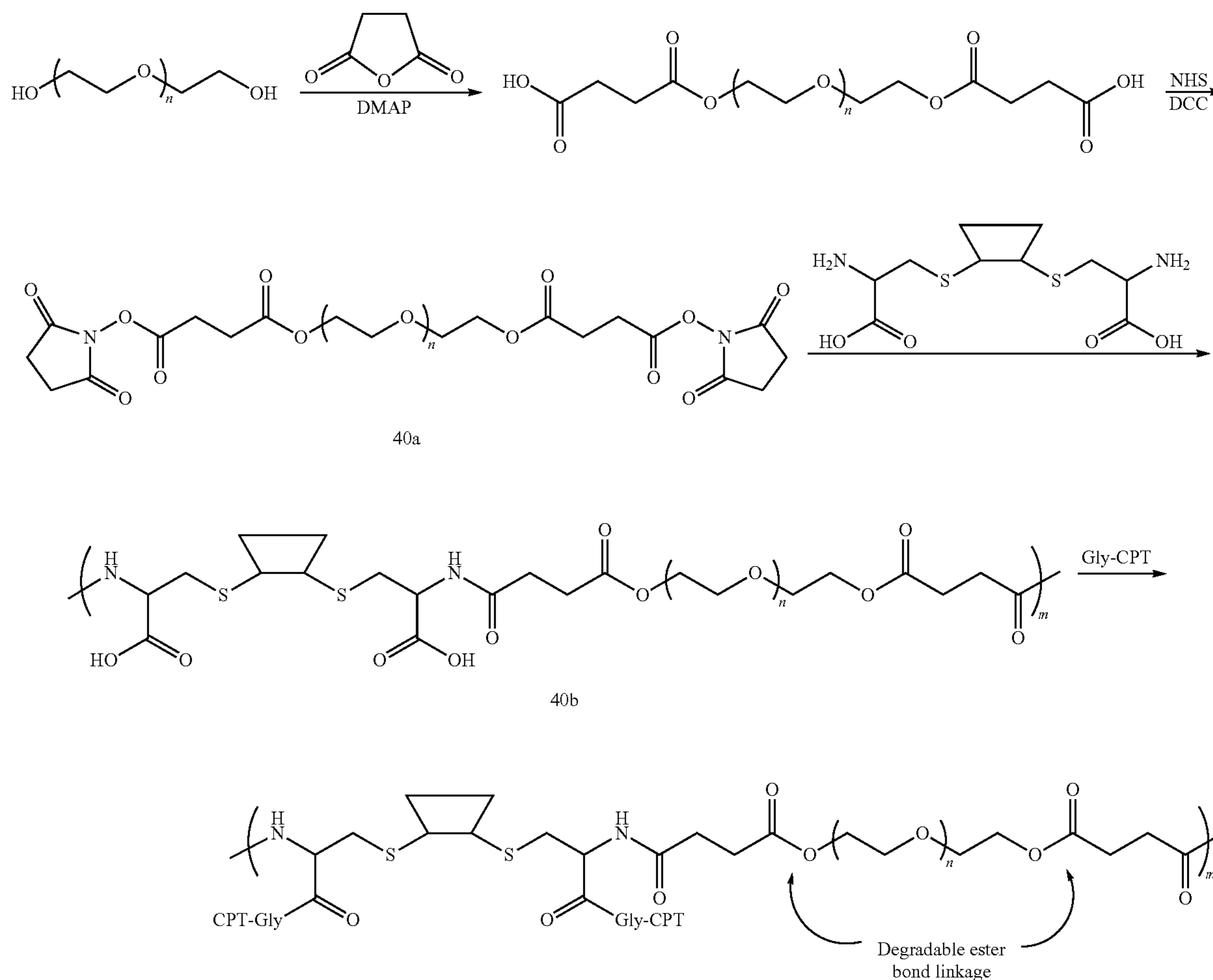
Scheme XXXXI
