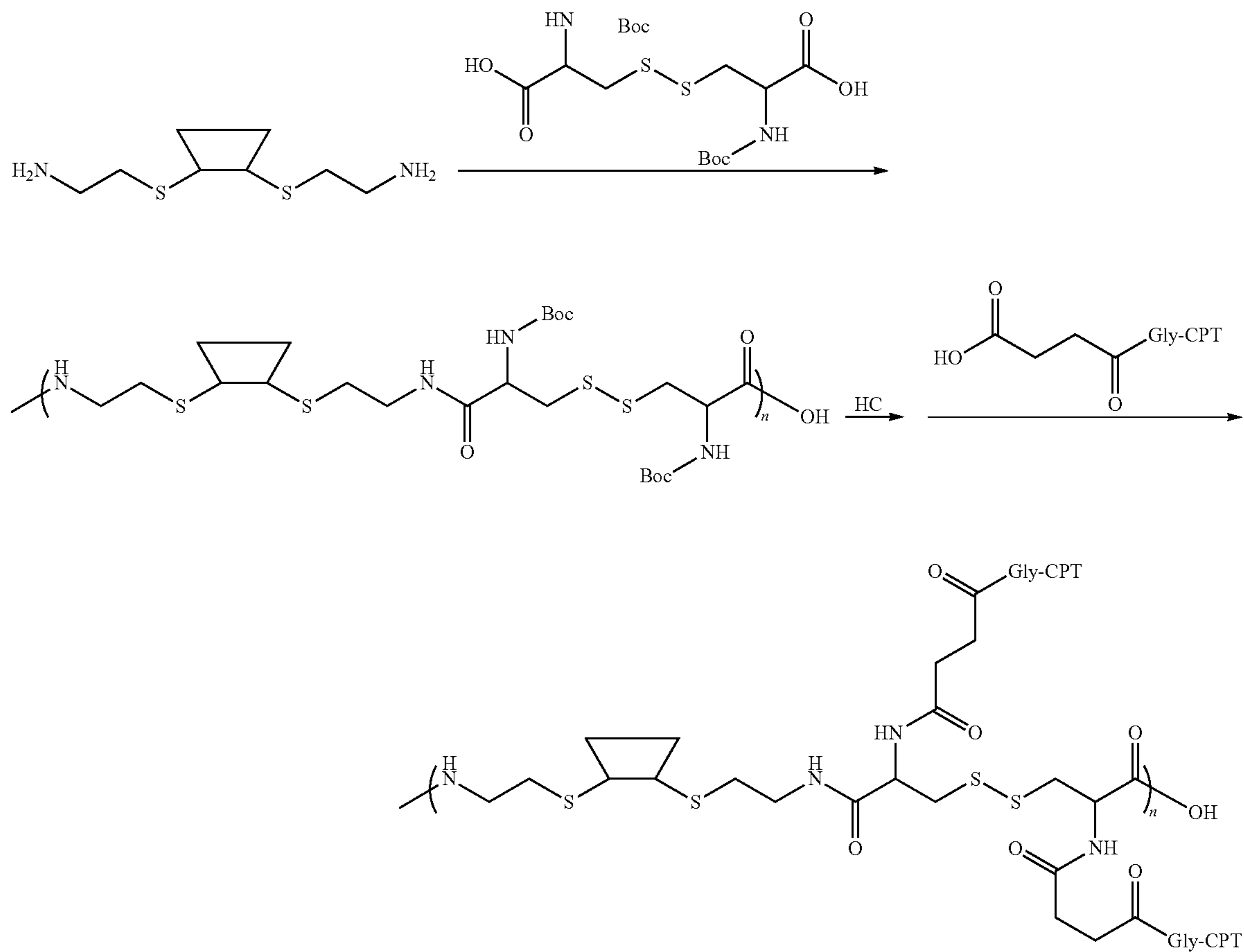
Scheme VII
