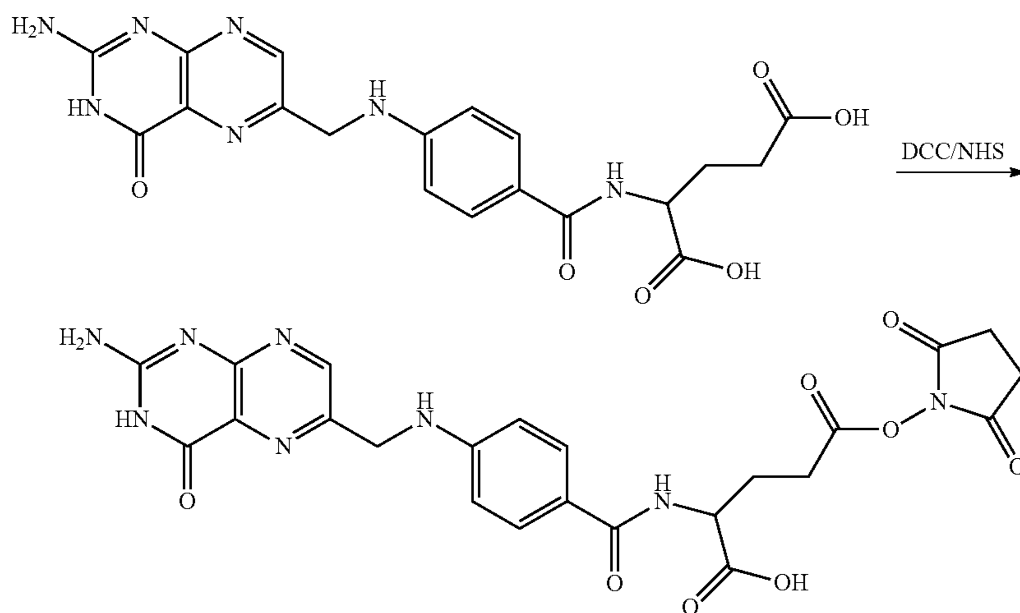
Scheme XXXXIX
