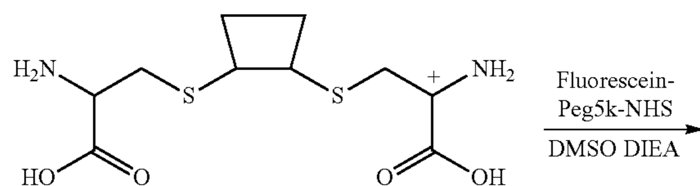
Scheme XXXX
