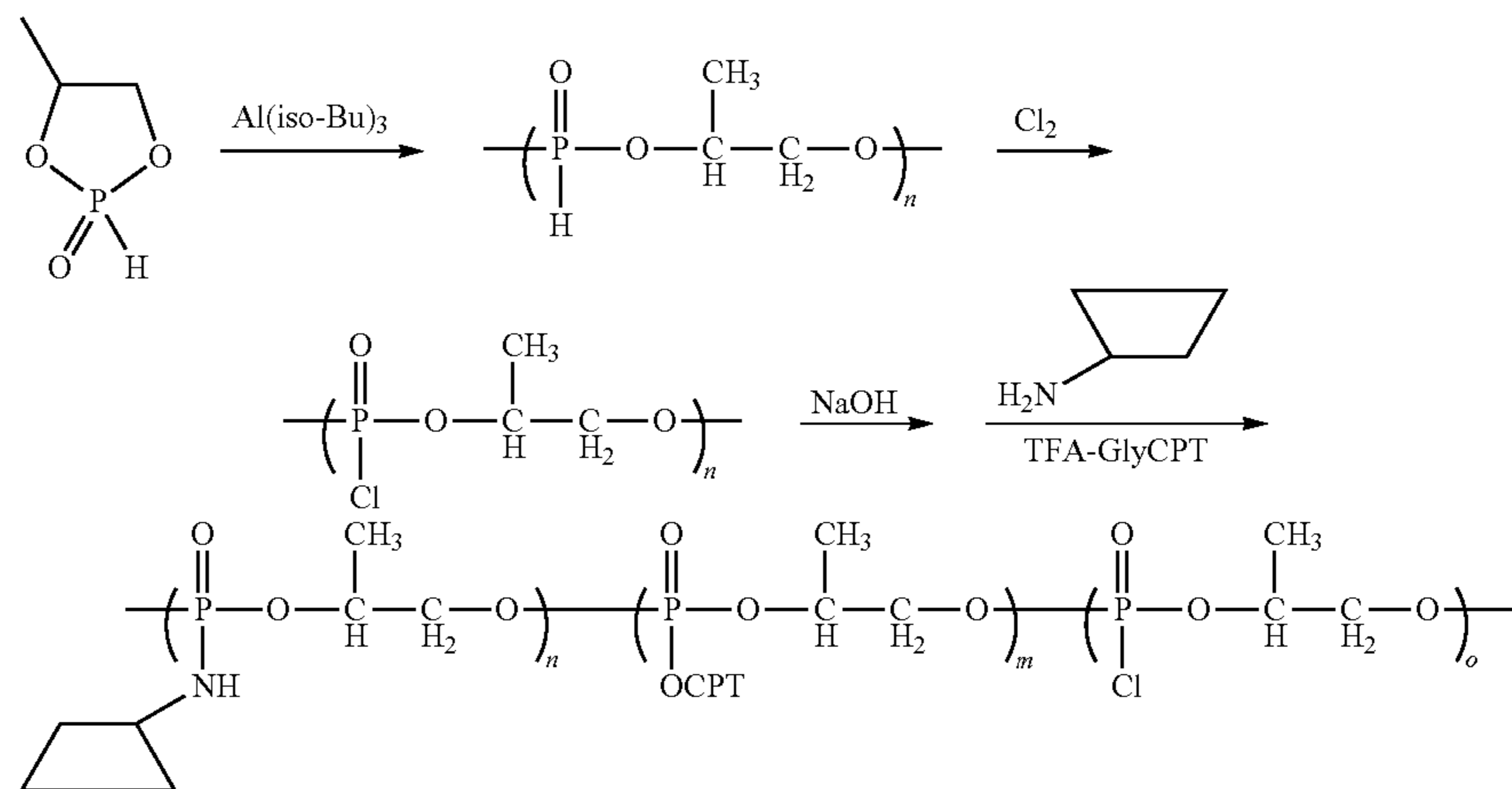
Scheme XXXIV
