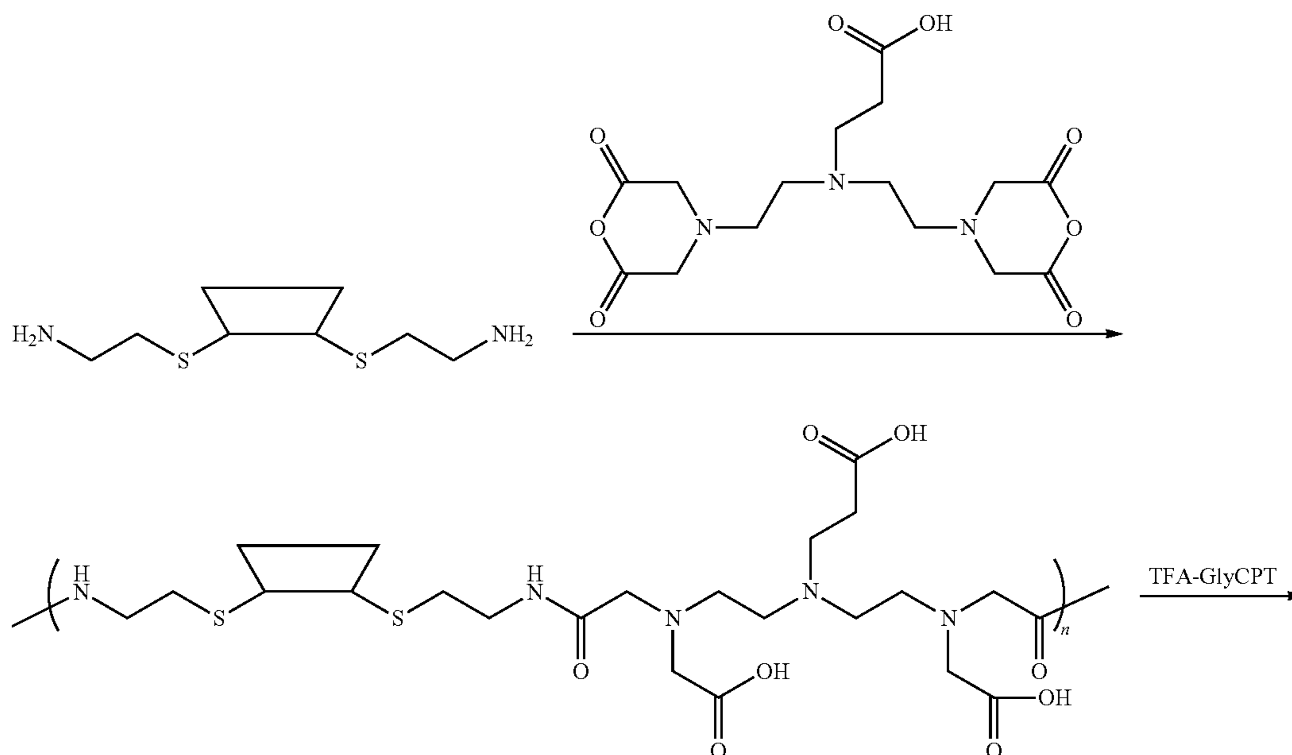
Scheme XXIX
