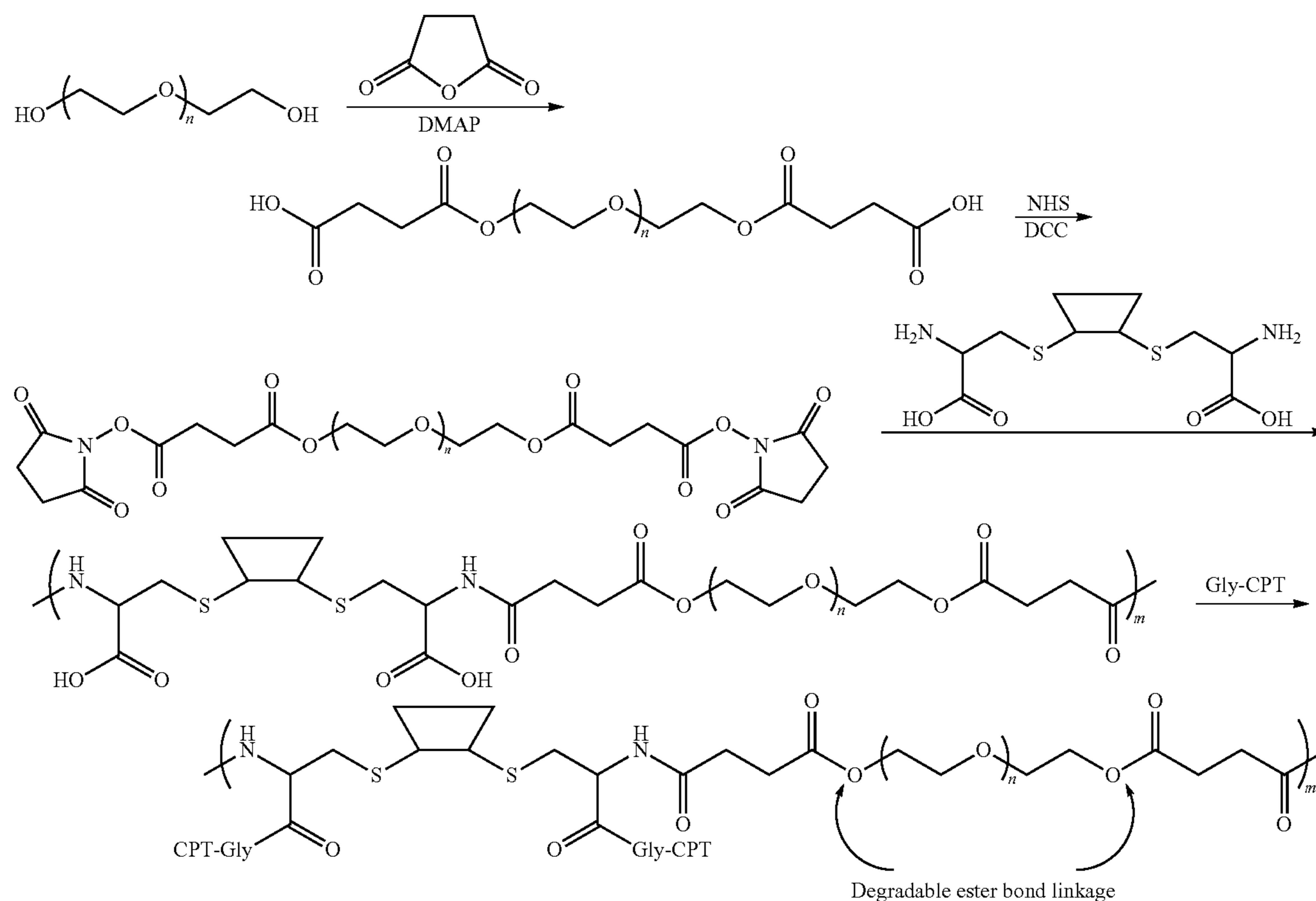
Scheme XIV
