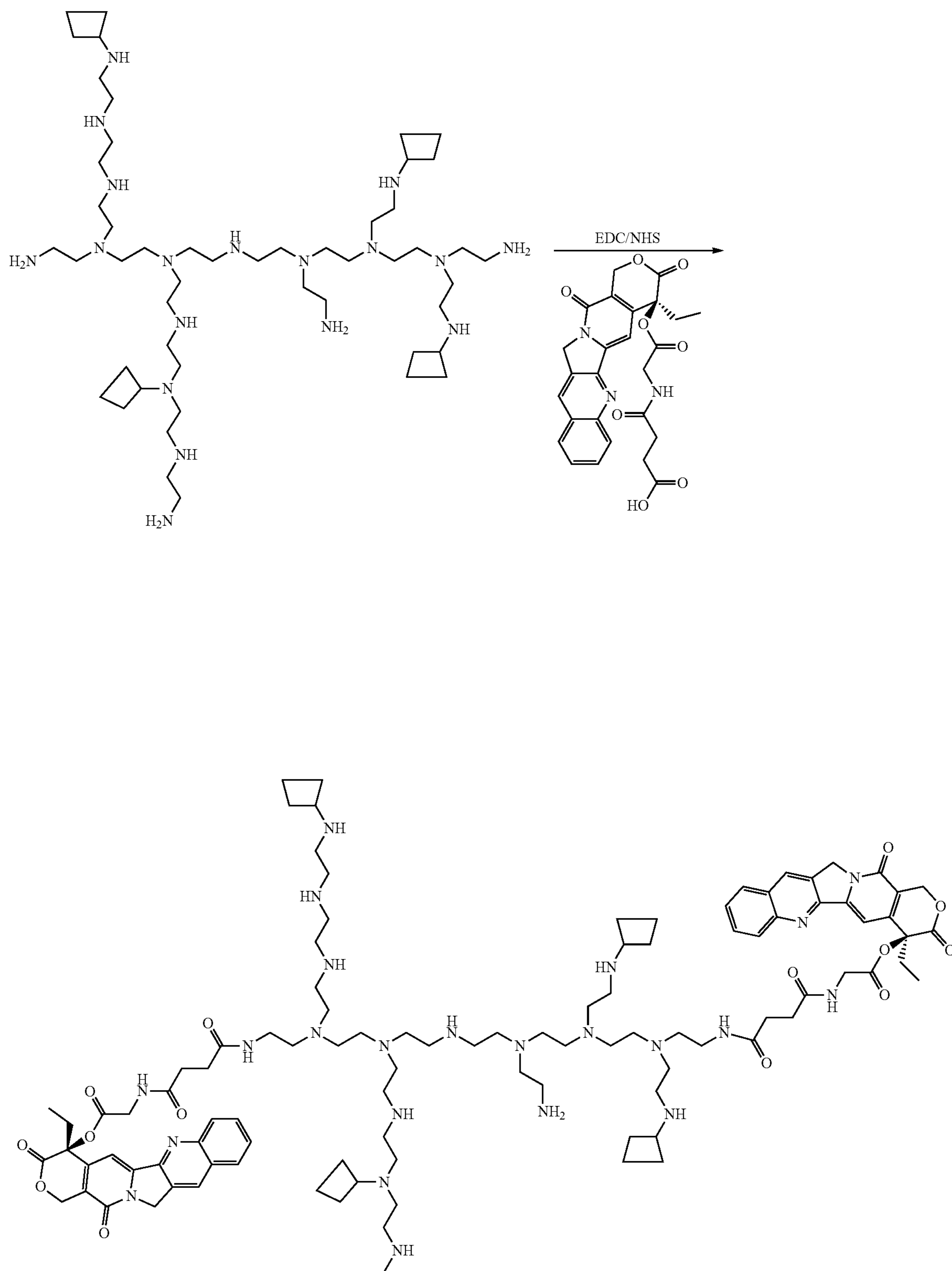
Scheme XXXXV
