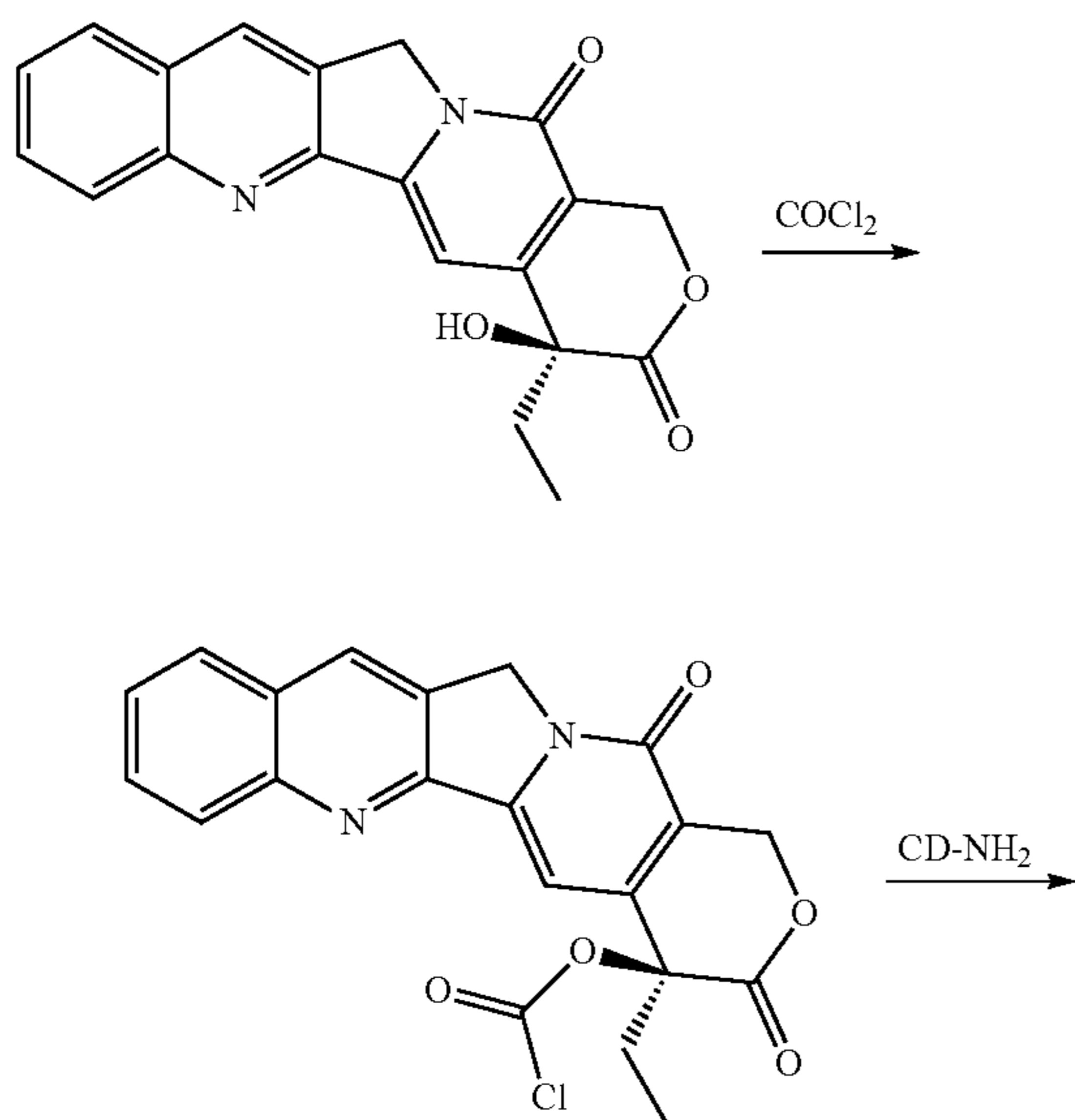
Scheme XXVIII
