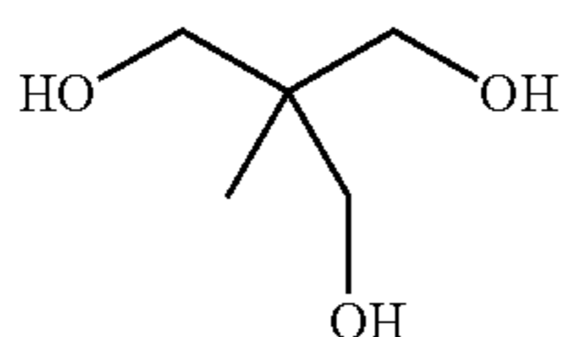
1,1,1-Tris(hydroxymethyl)ethane
