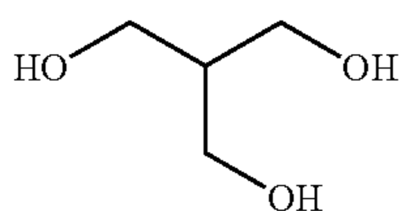
2-(hydroxymethyl)-1,3-propanediol
