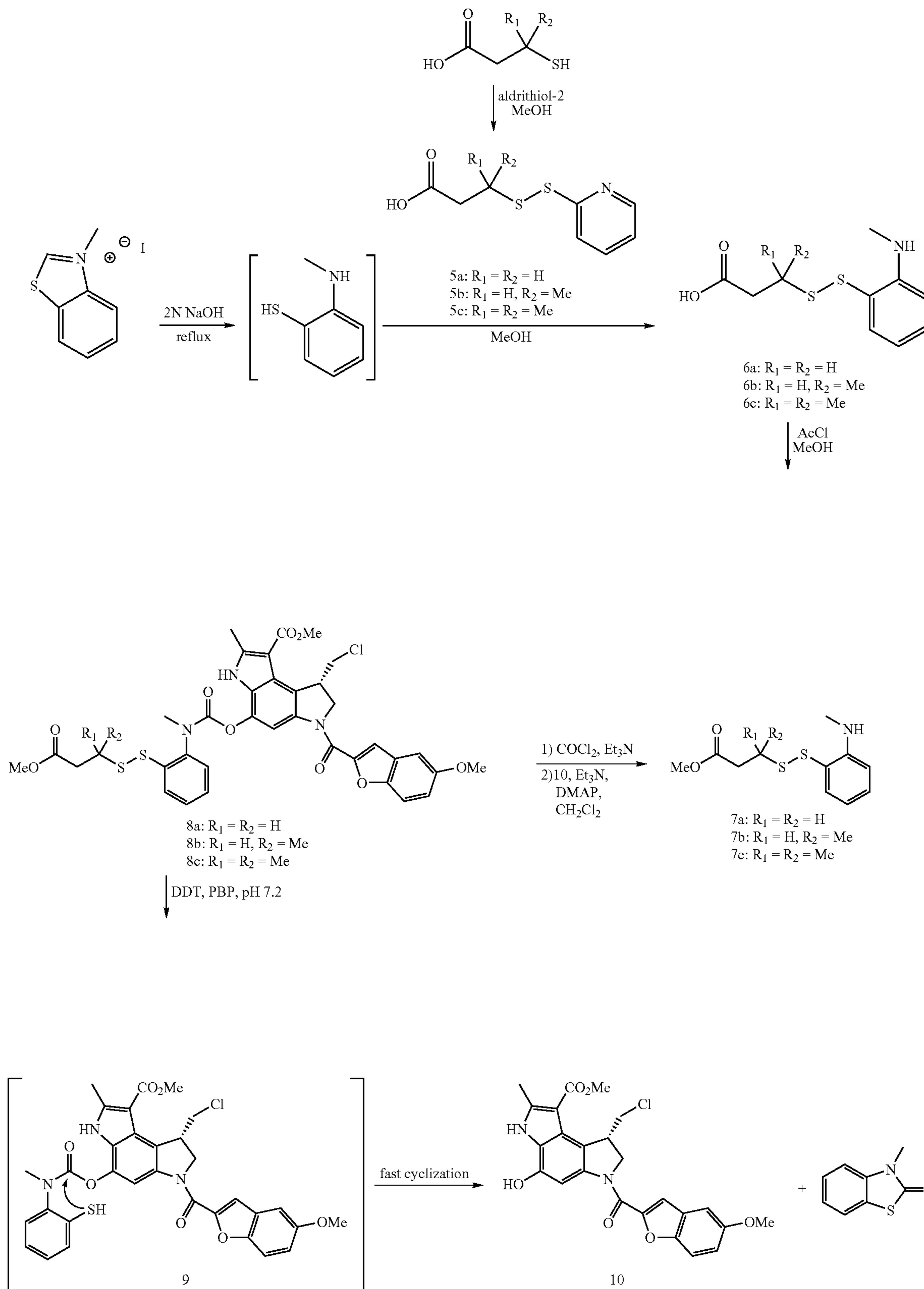
Scheme 2
