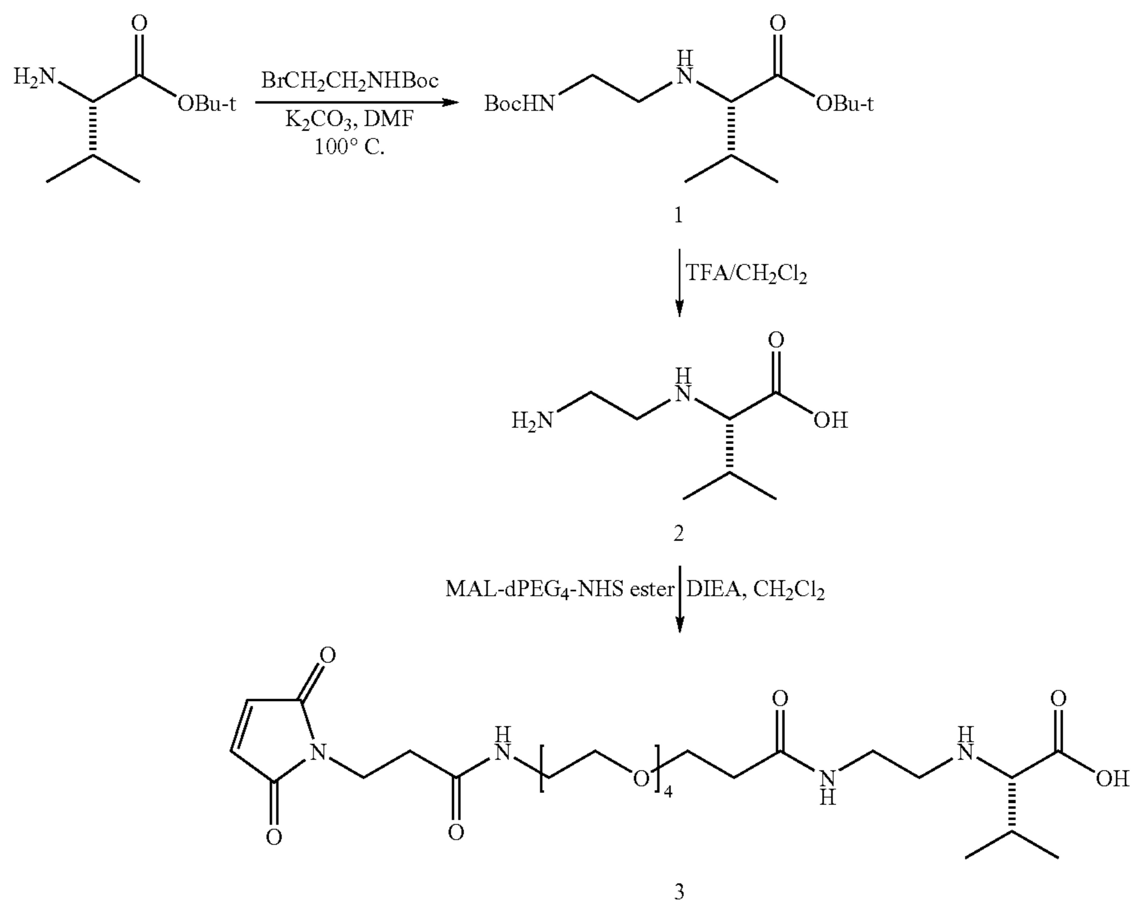
Scheme 1
