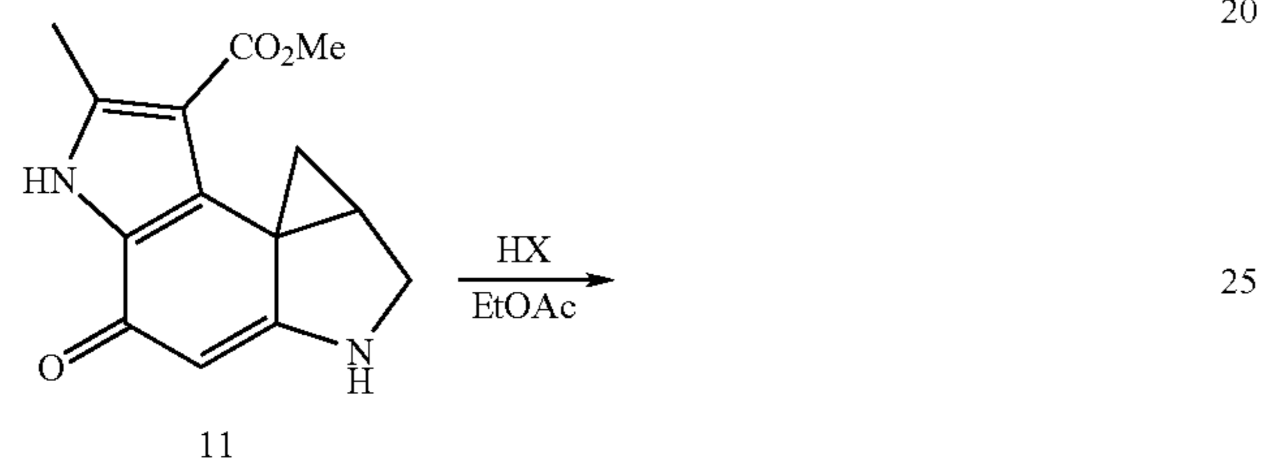
Scheme 3
