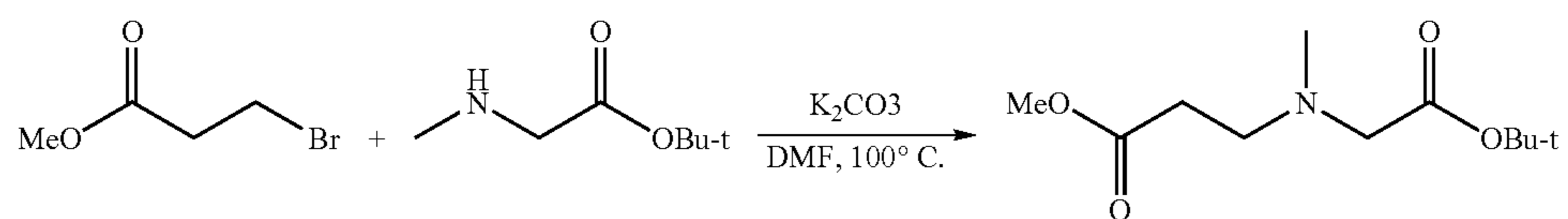
Scheme 5
