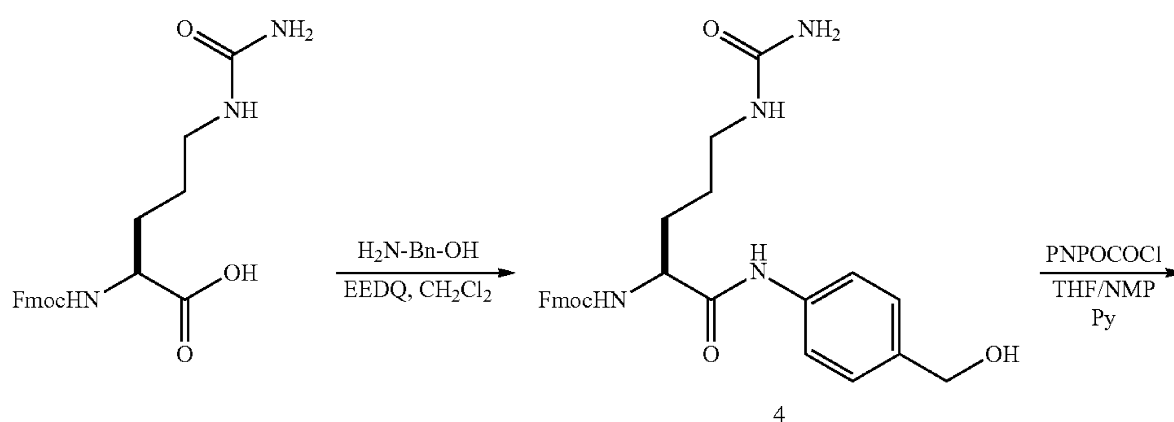
Scheme 2
