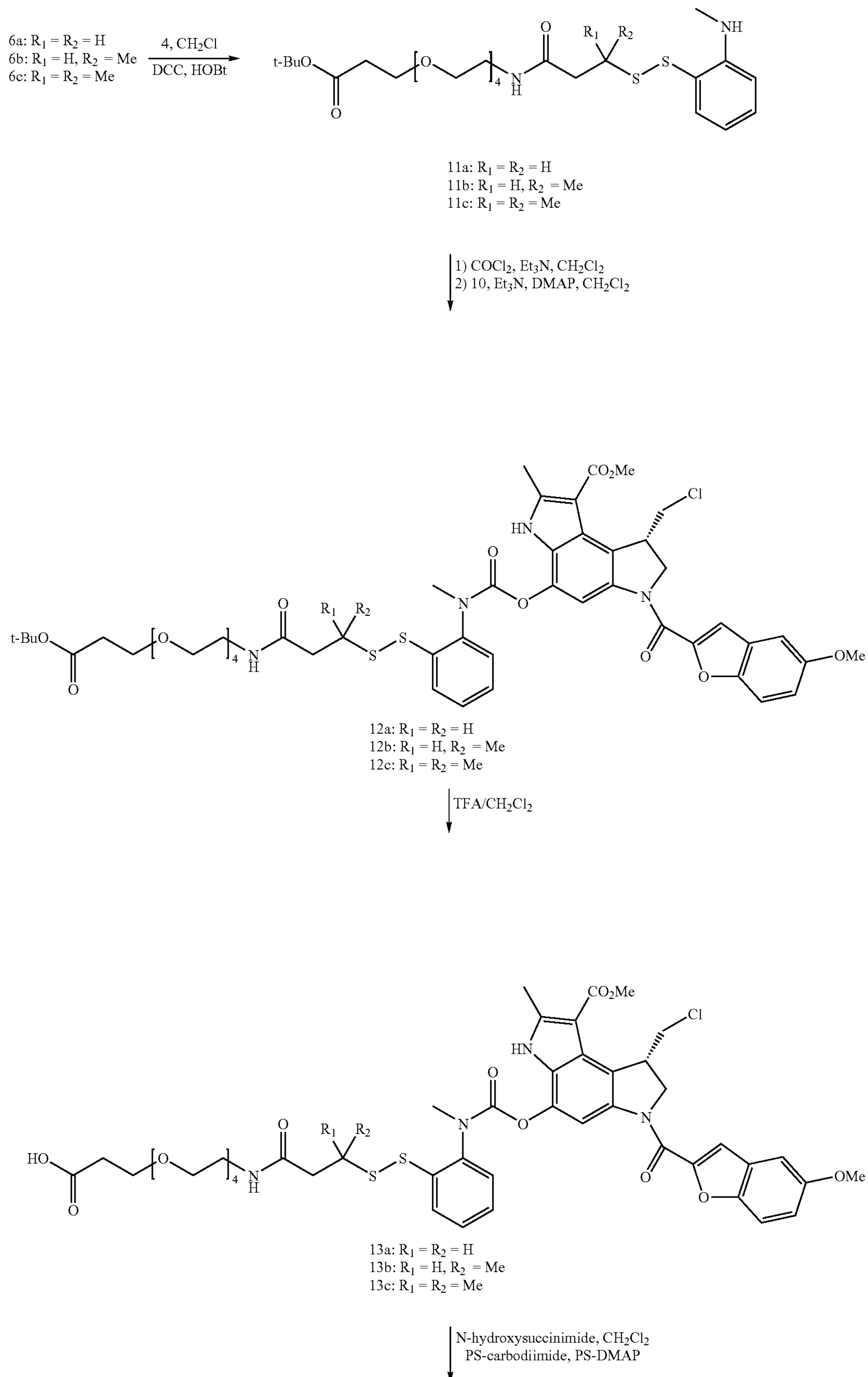
Scheme 3
