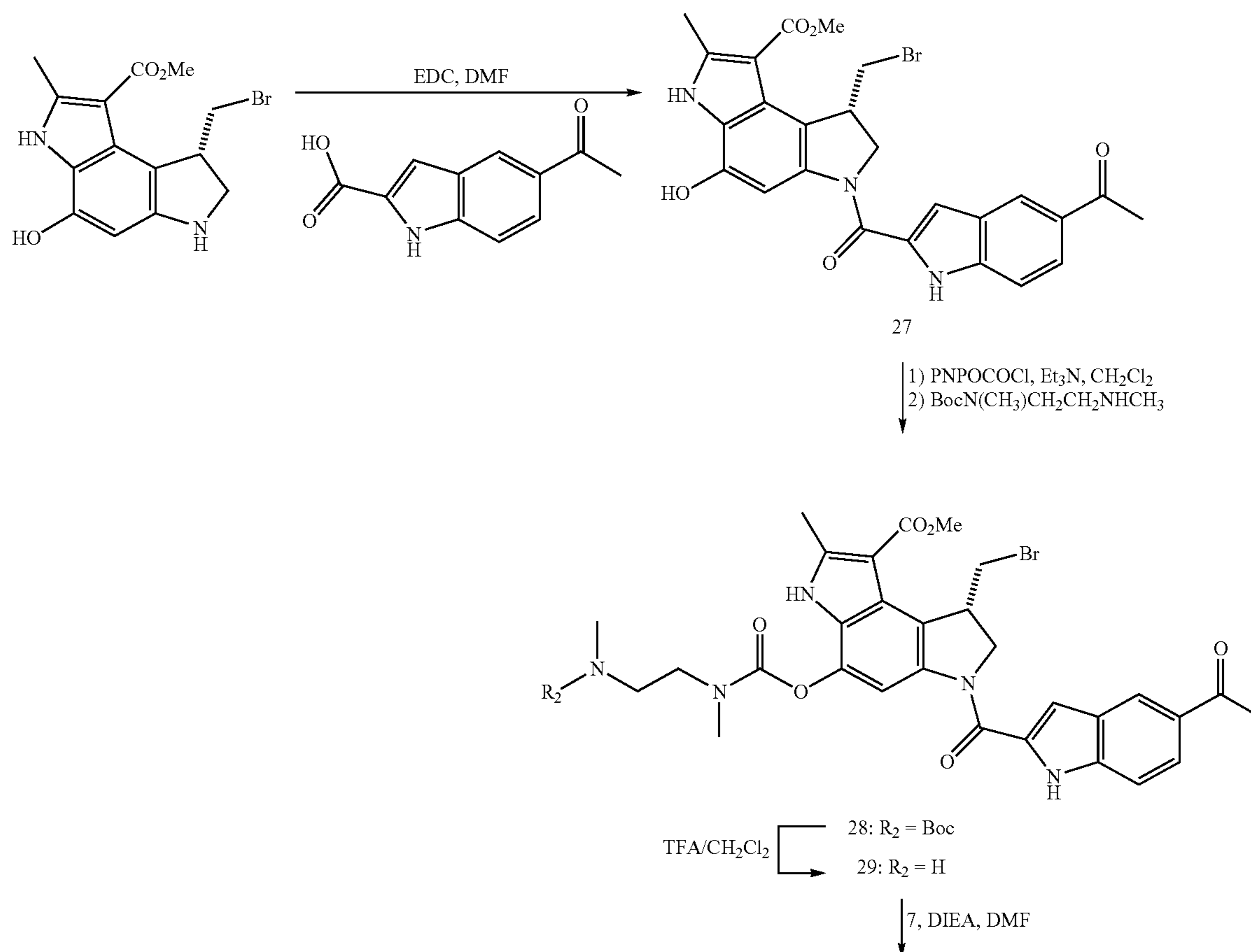
Scheme 6
