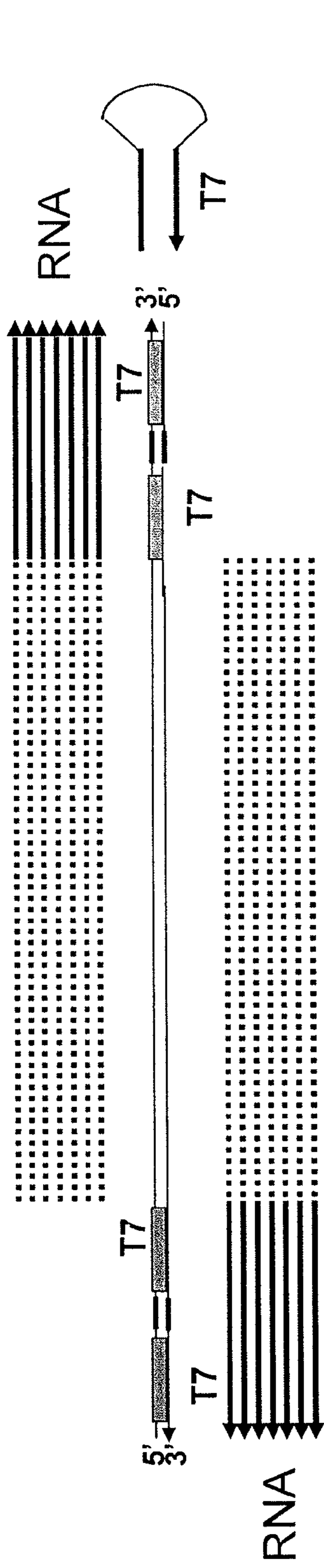
A. T7 promoter sequence is in the stem of the stem-loop oligonucleotide
