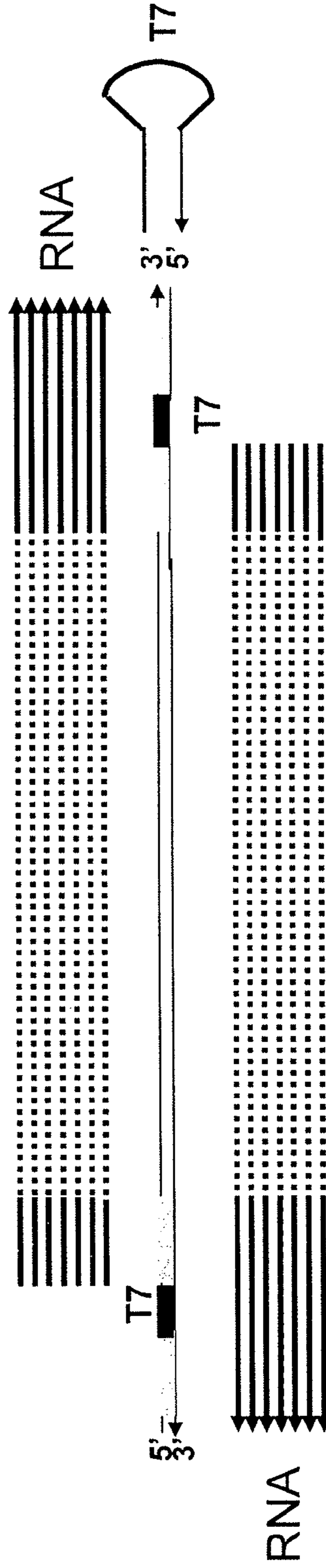
B. T7 promoter sequence is within the loop of the stem-loop oligonucleotide
