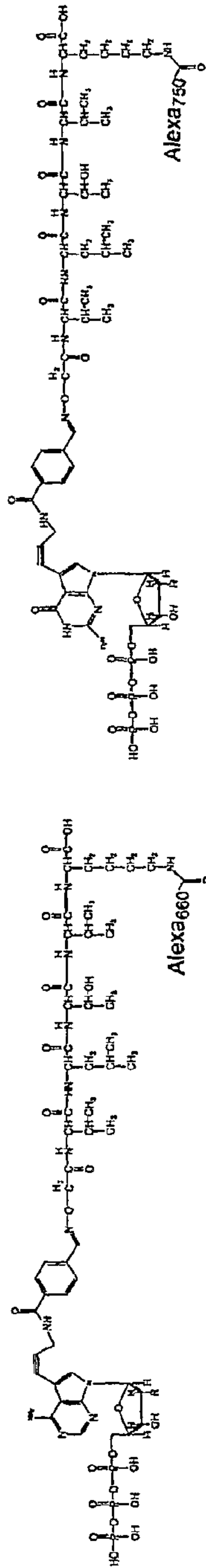
dCTP-TAMRA (540/564 nm)
