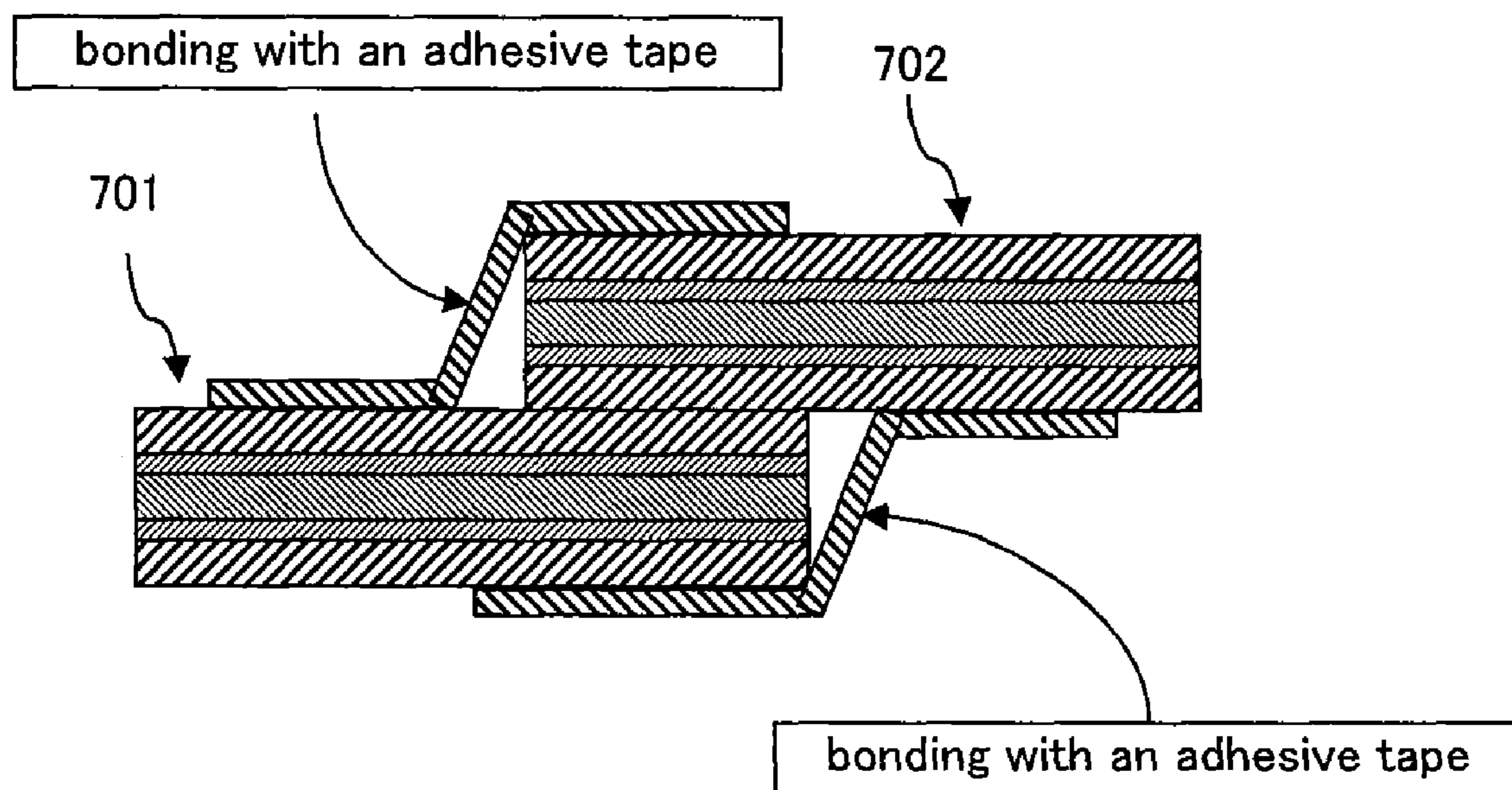
(b) Conventional Method for Joining (2)
