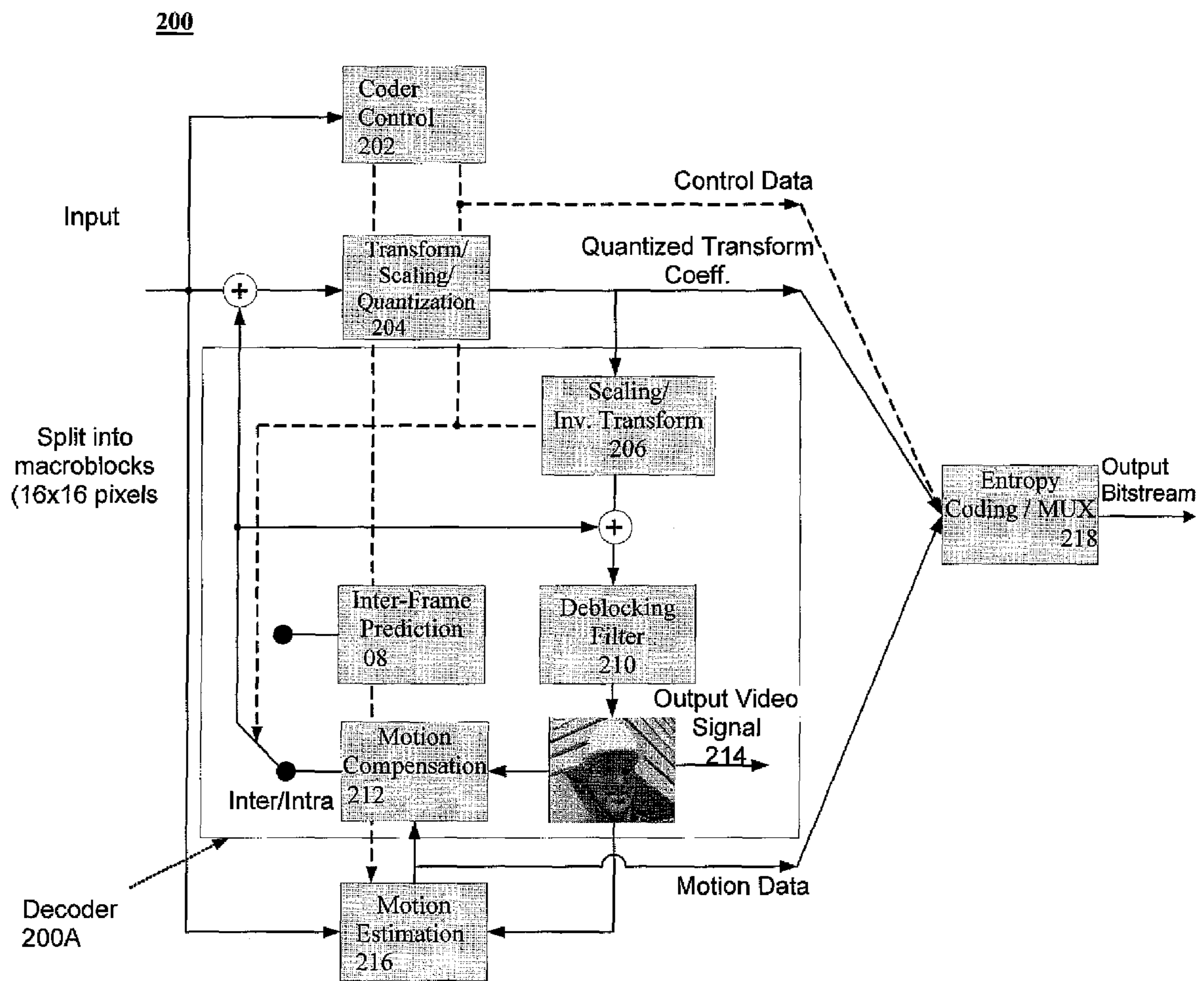
FIG. 2: Single-Layer Video Encoder
