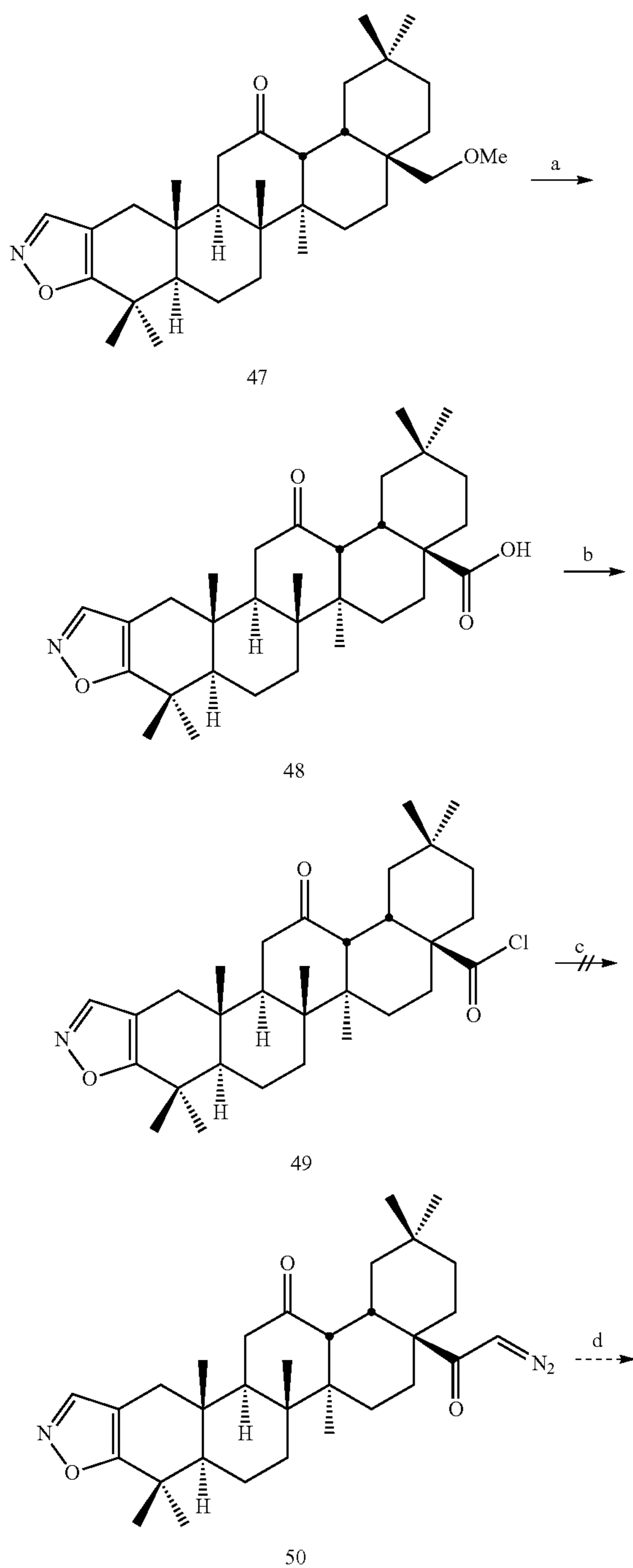
Scheme 24:
