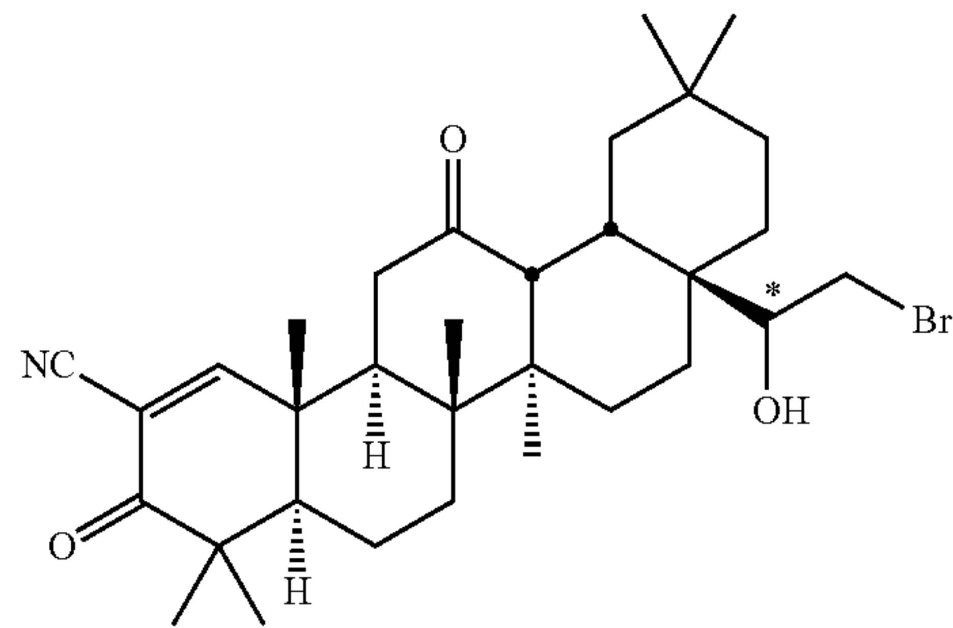
63284 (diastereomer of 63283 at secondary alcohol position)
