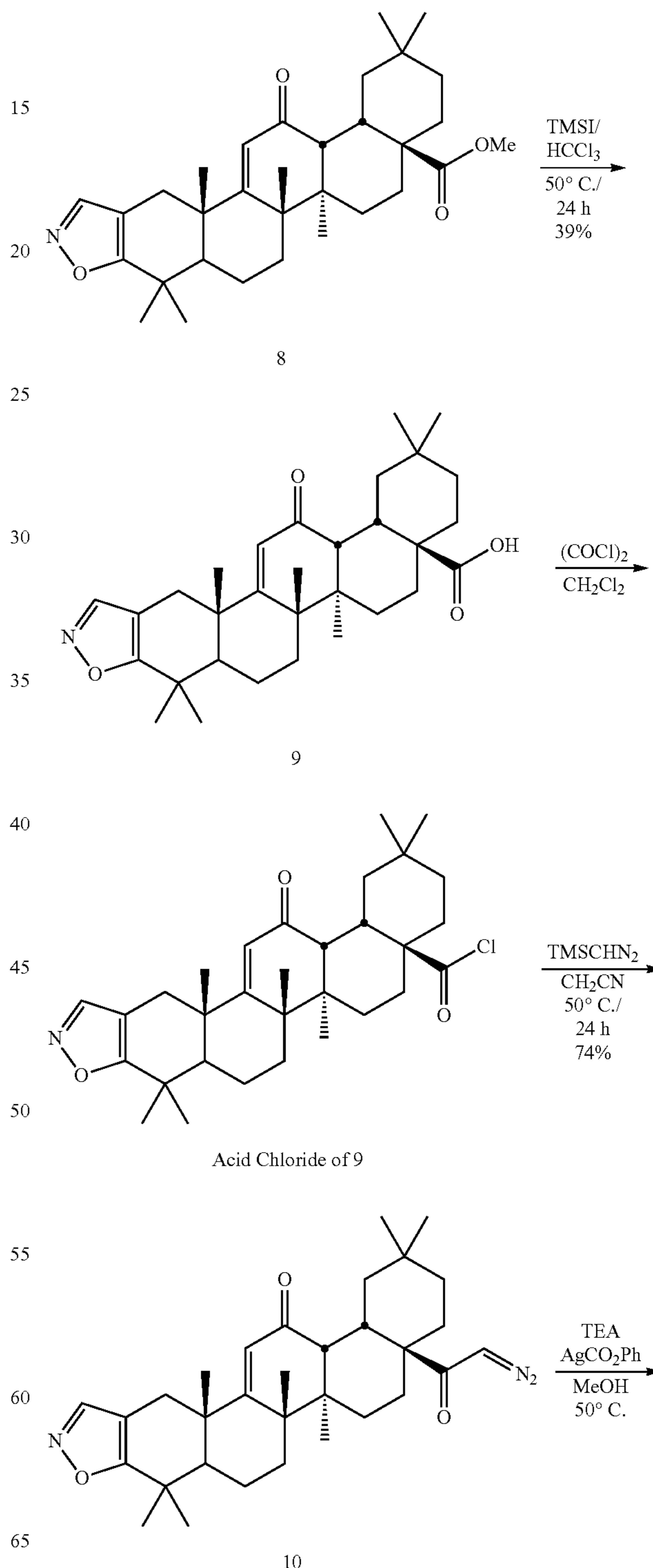
Scheme 1:
