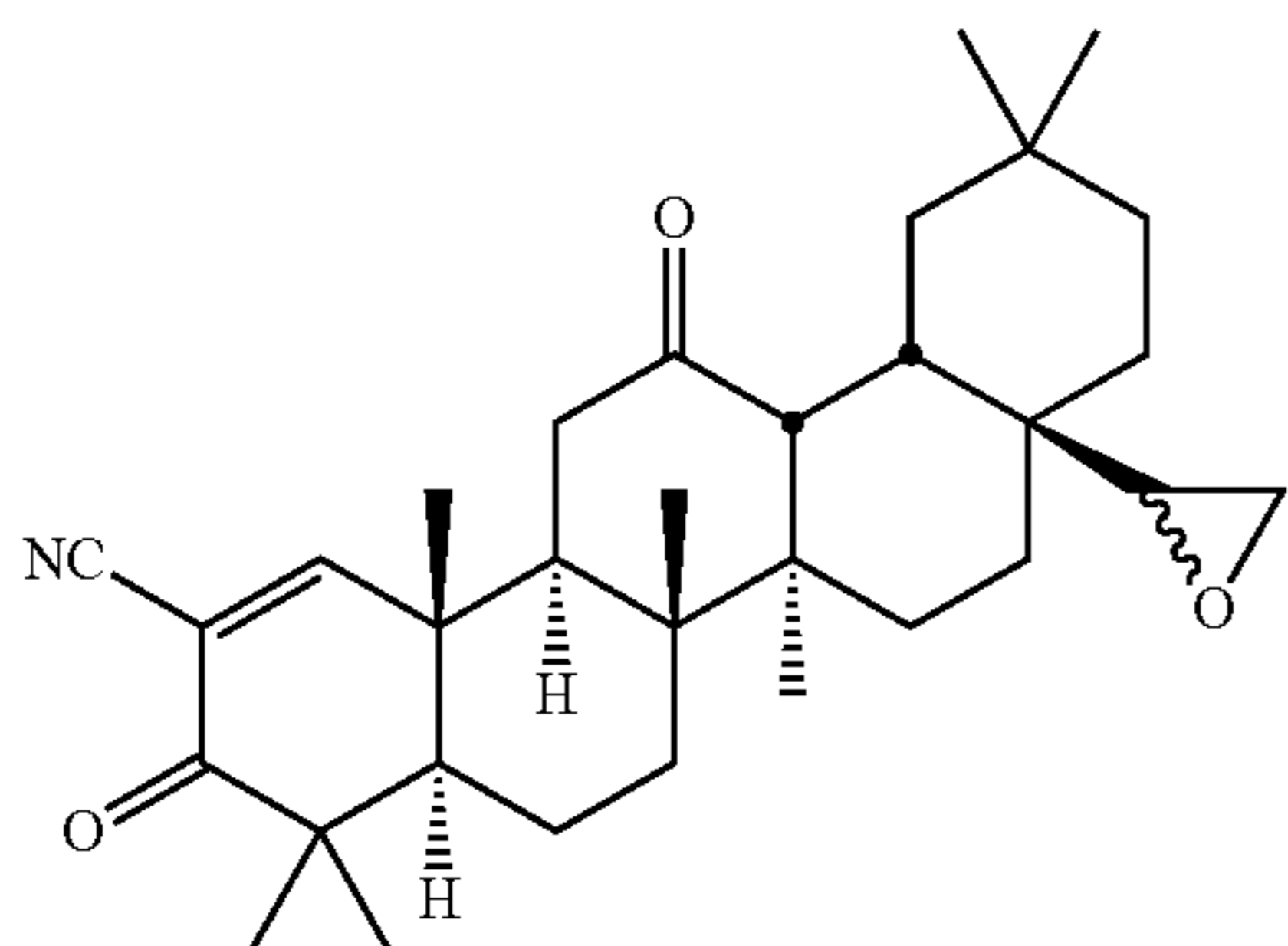
63275 (mixture of two epoxide diastereomers 63786 and 63287)
