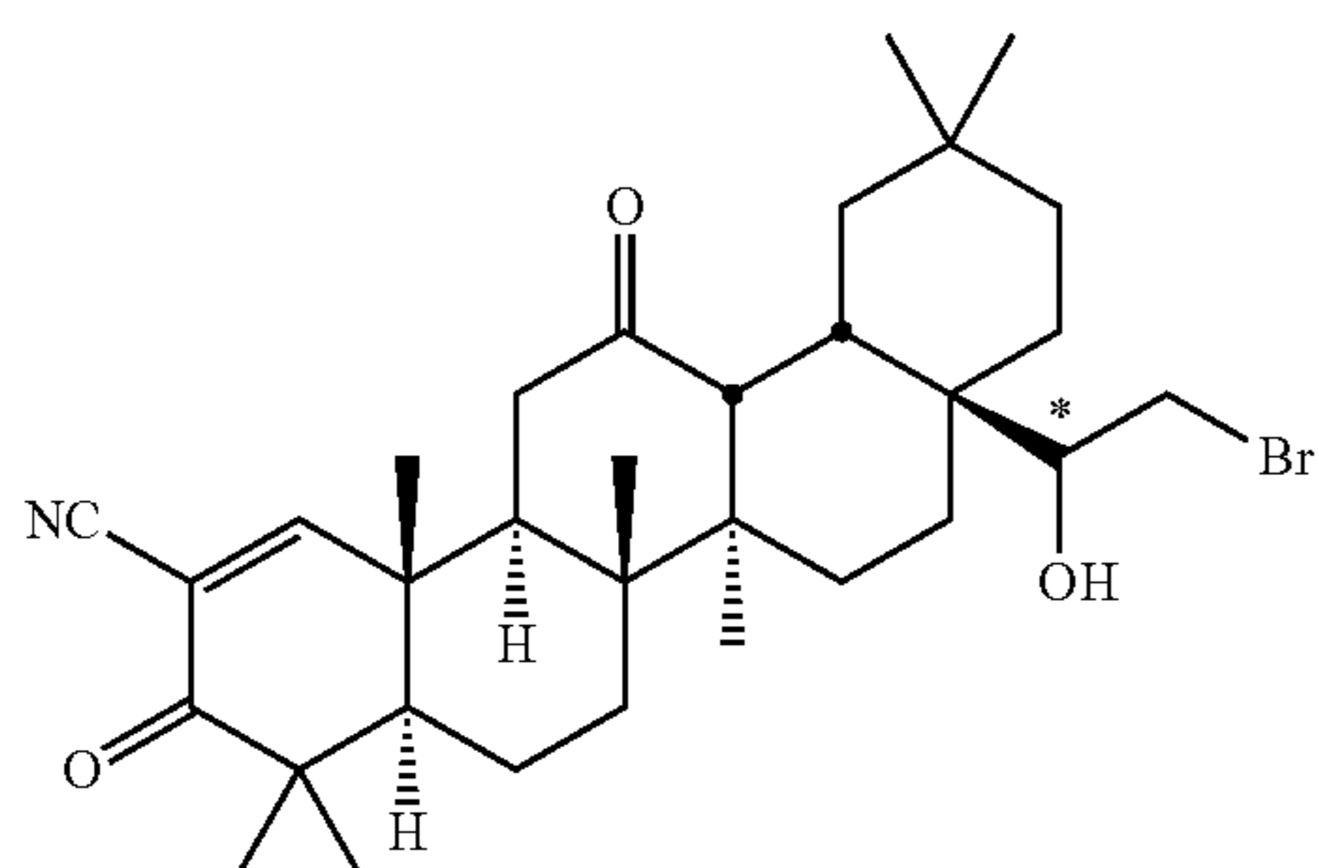
63283 (diastereomer of 63284 at secondary alcohol position)
