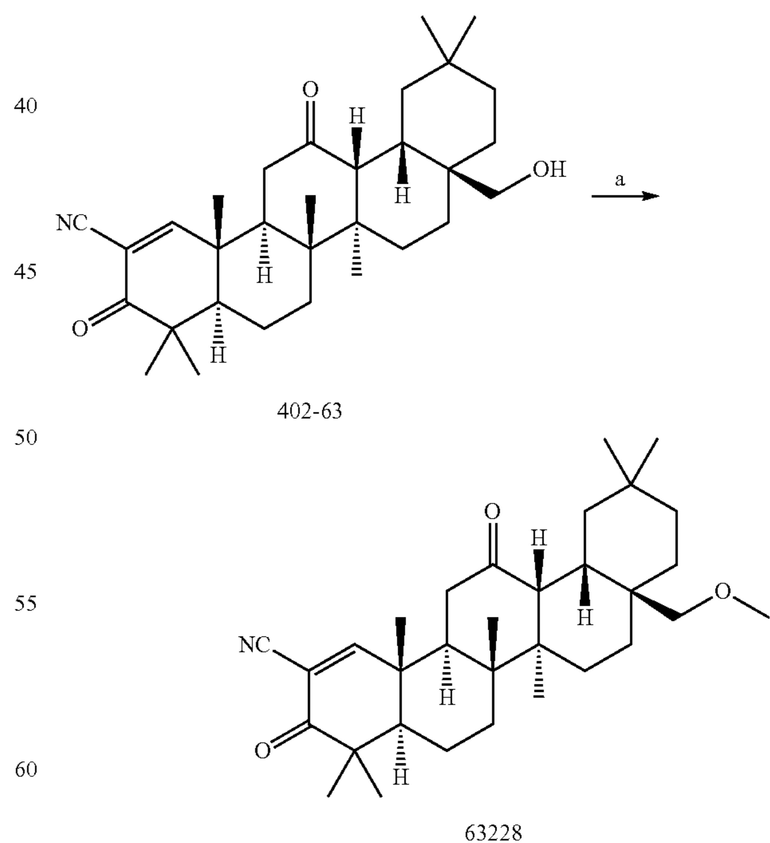
Scheme 11:
