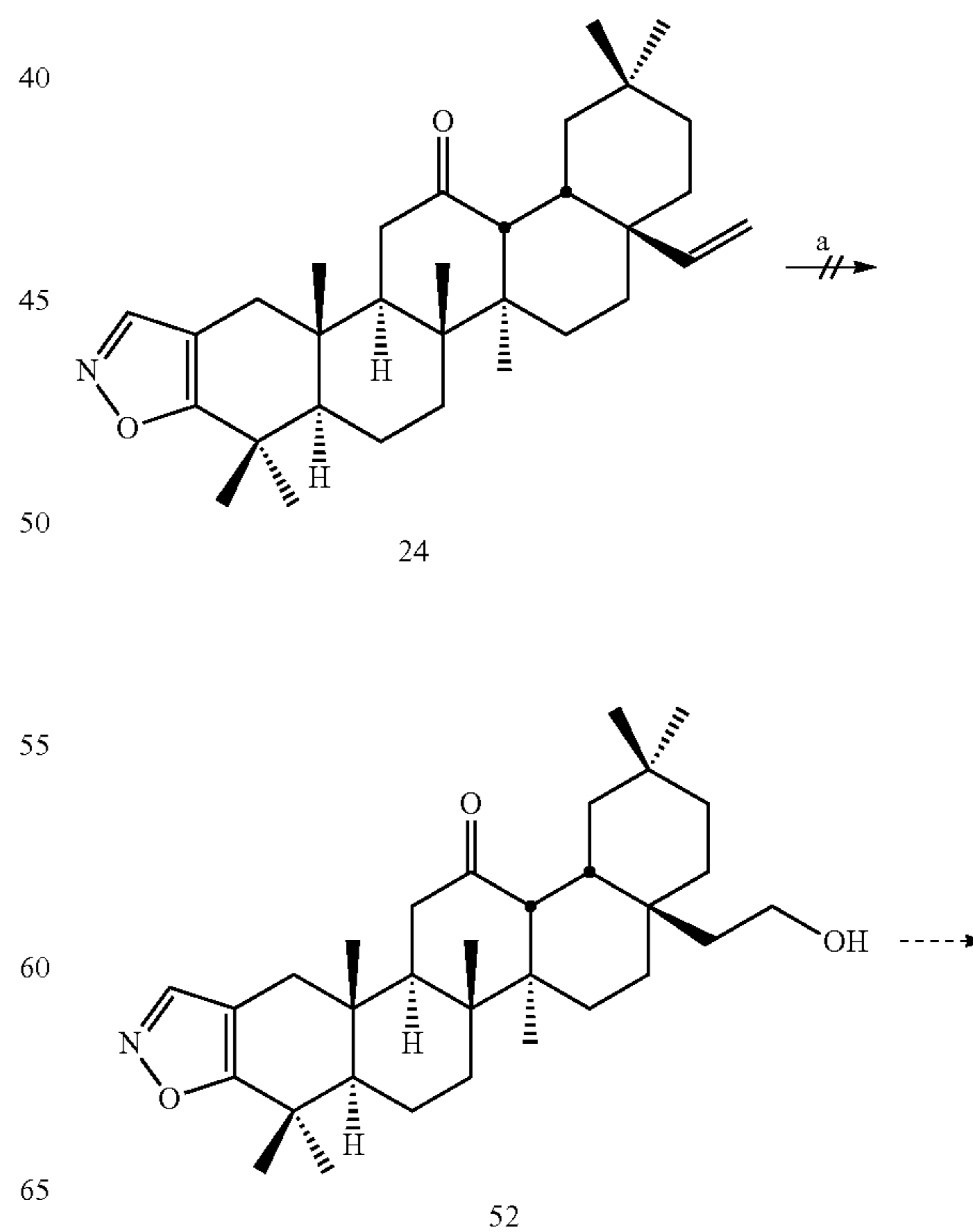
Scheme 25:
