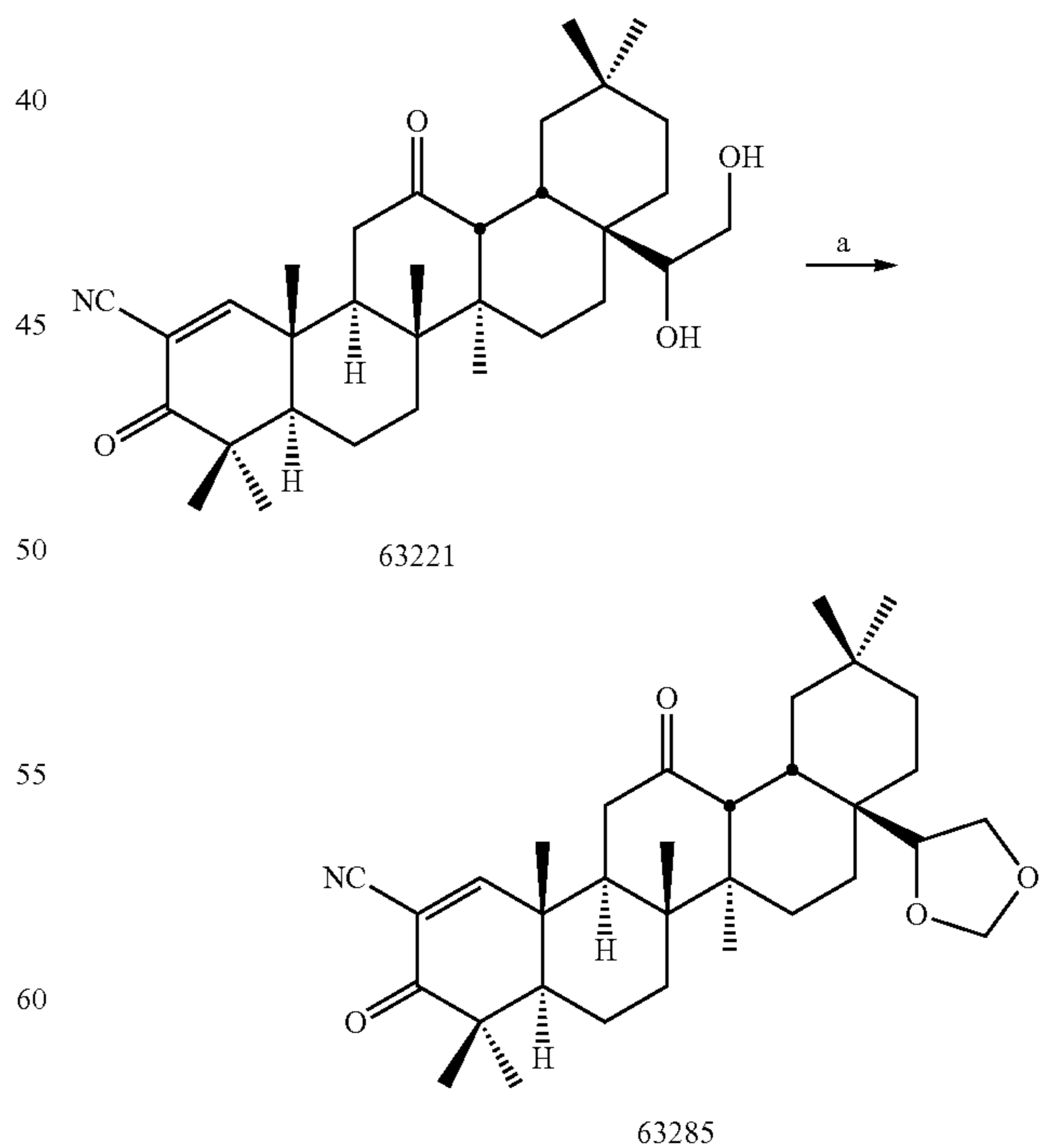
Scheme 19:
