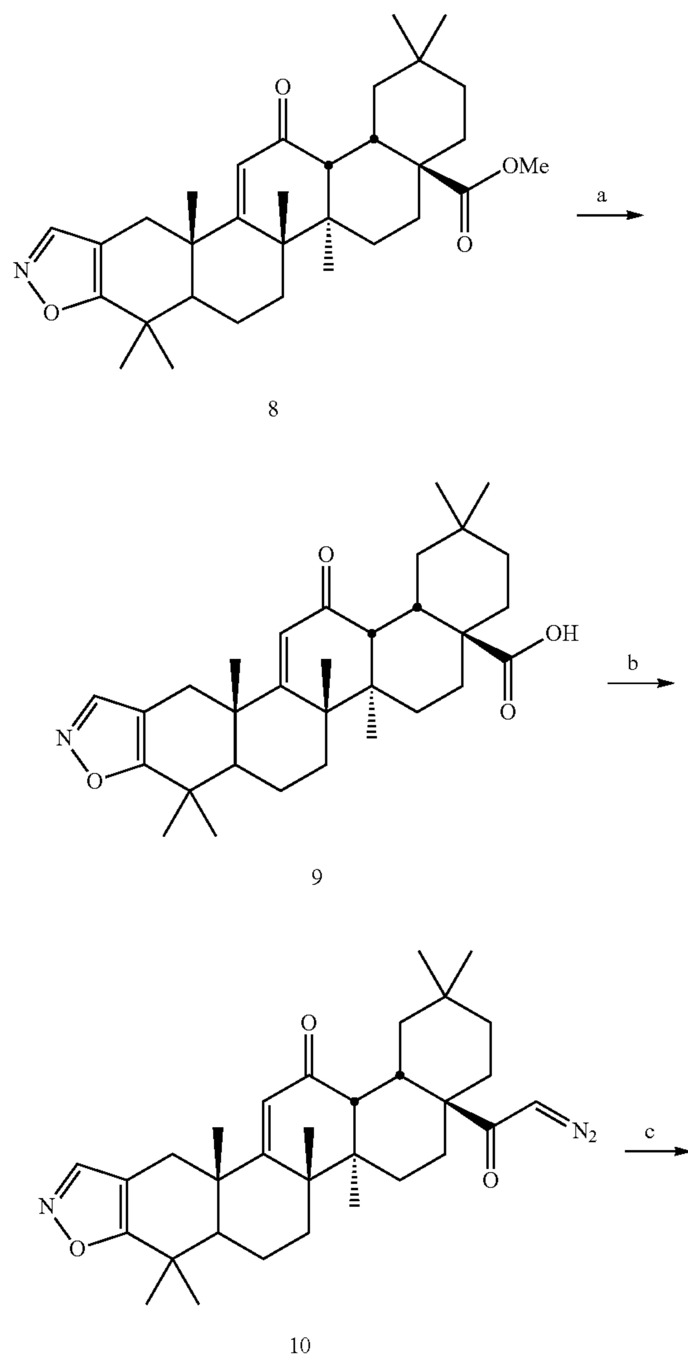
Scheme 3:
