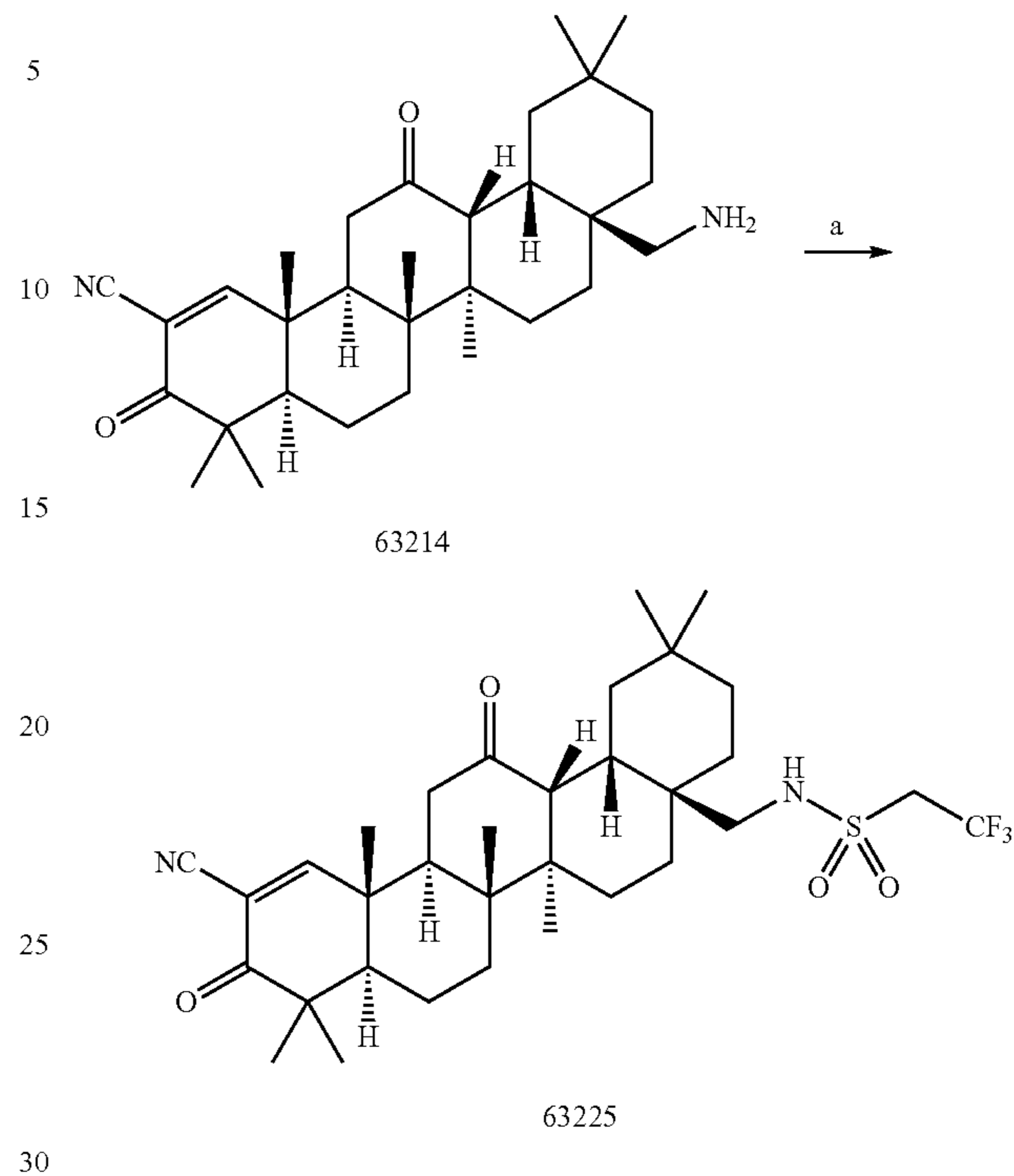
Scheme 10:
