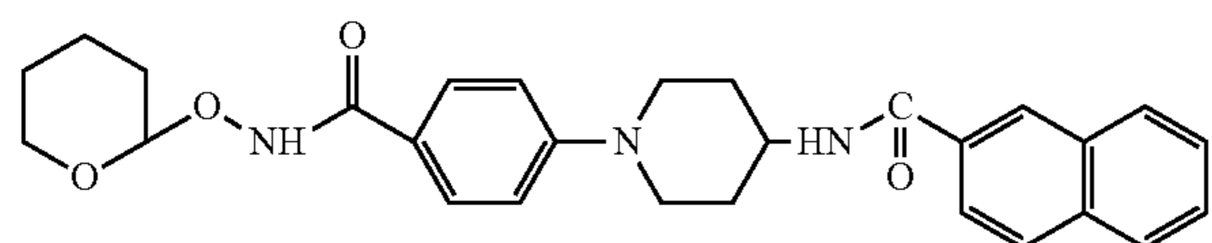
intermediate 10
