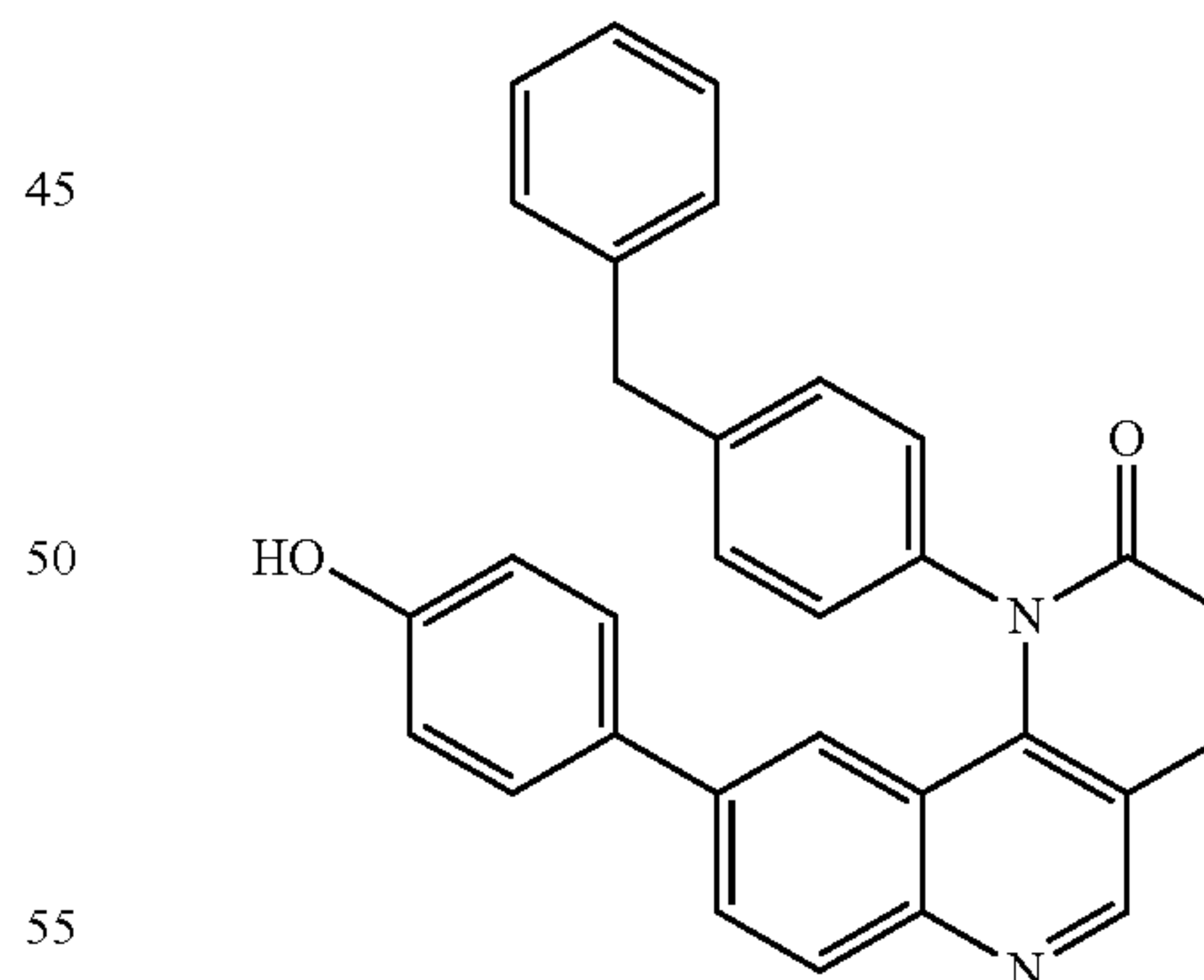
4-(4-benzylphenylamino)-6-chloroquinoline-3-carbaldehyde
