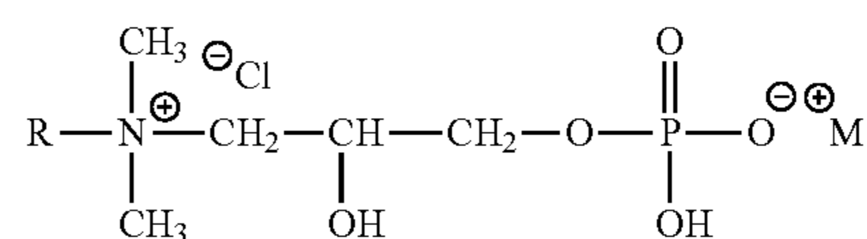
Alkyl phosphobetaines
