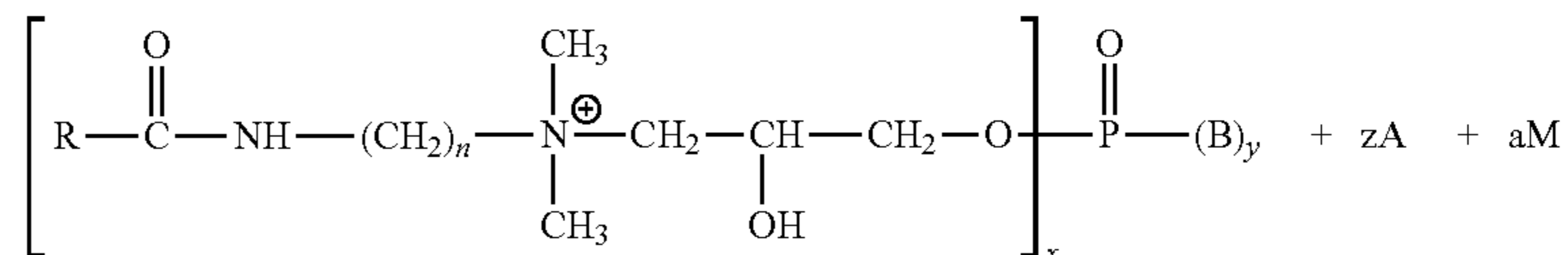
Phospholipids
