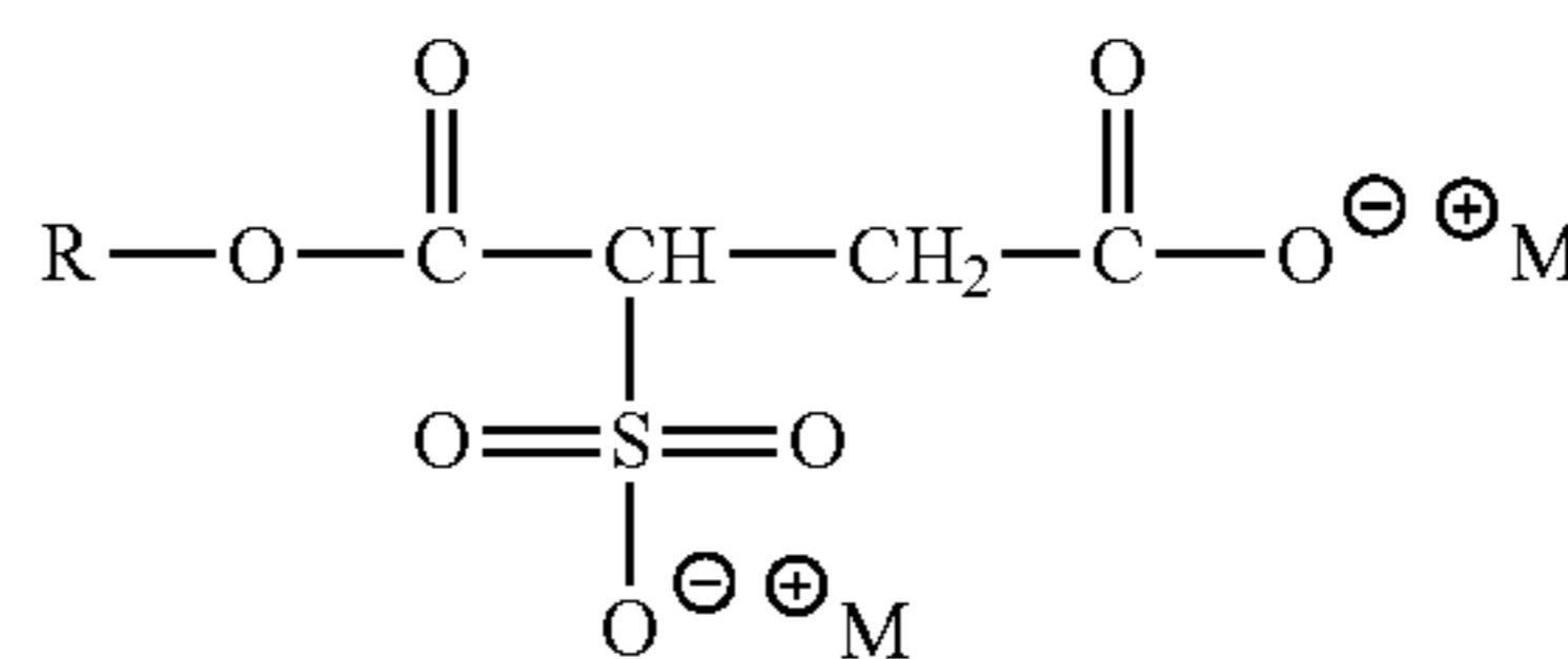
Alkyl sulfosuccinates
