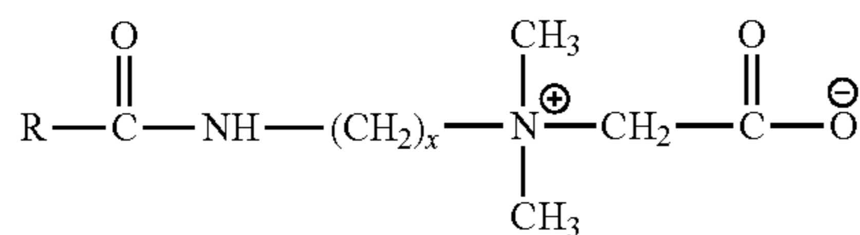
Alkylamidoalkyl betaines
