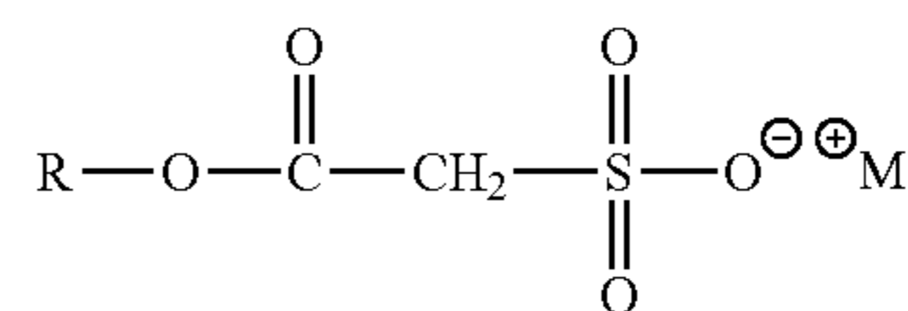
Alkyl sulfoacetates
