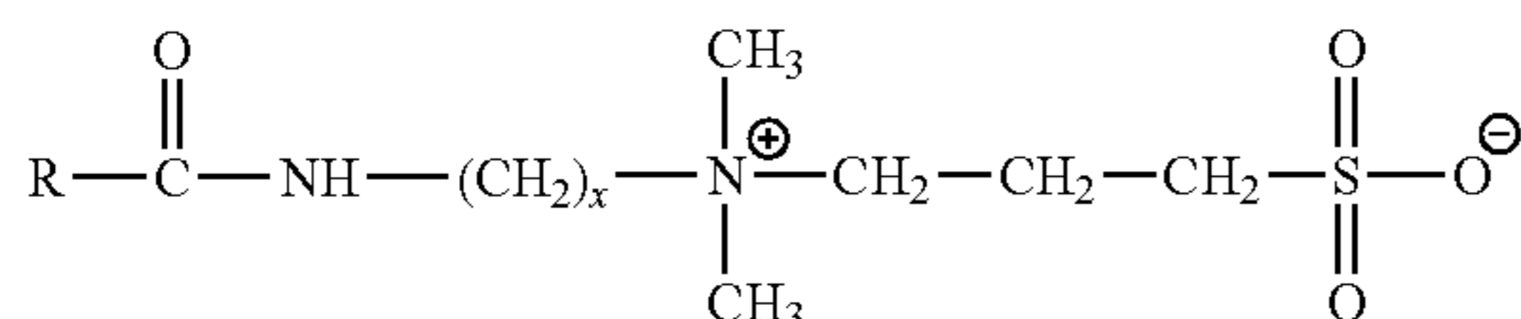
Alkylamidoalkyl sultaines
