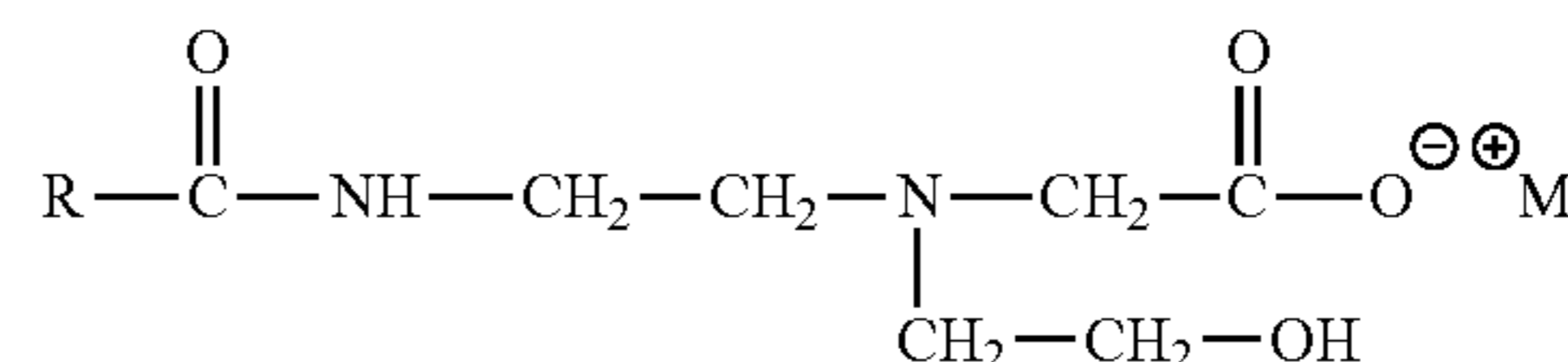
Alkyl amphotoacetates
