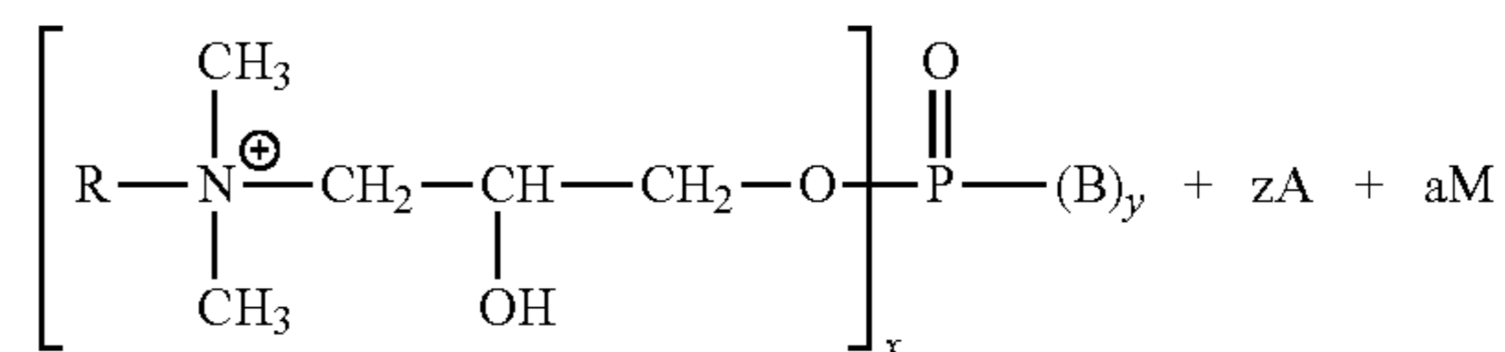
Phospholipids
