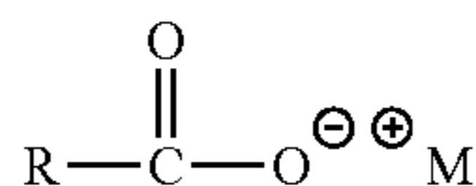
Alkyl carboxylates
