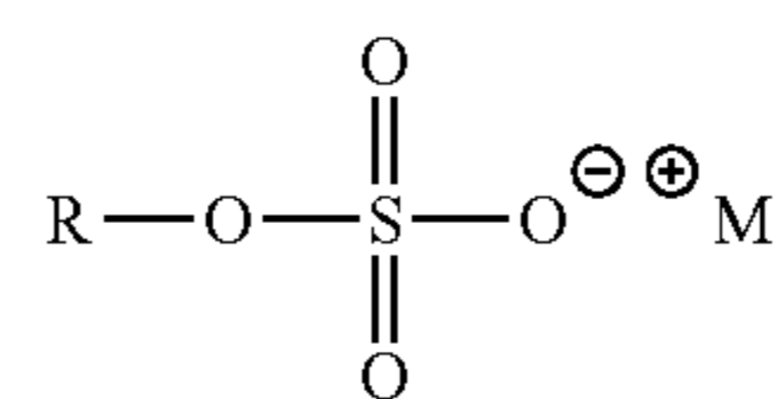
Alkyl sulfates
