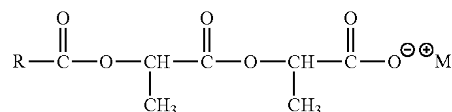
Acyl lactylates
