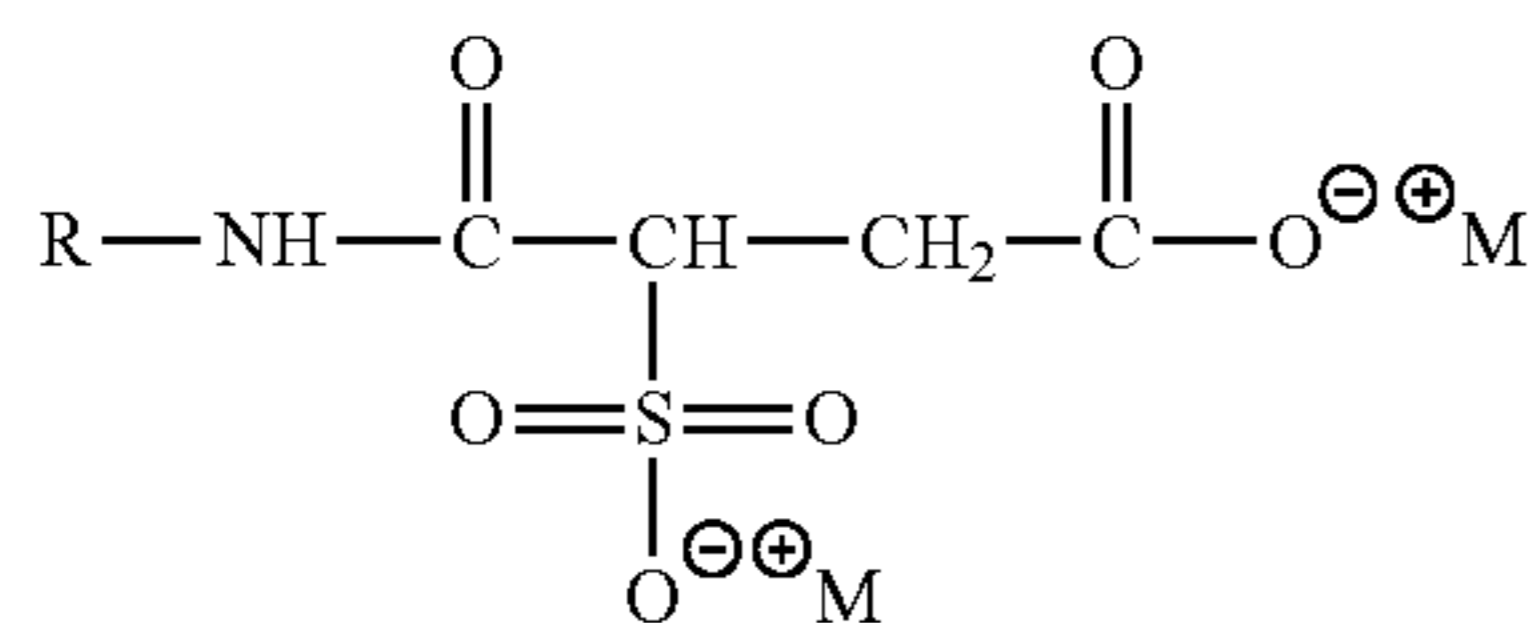
Alkyl sulfosuccinamates
