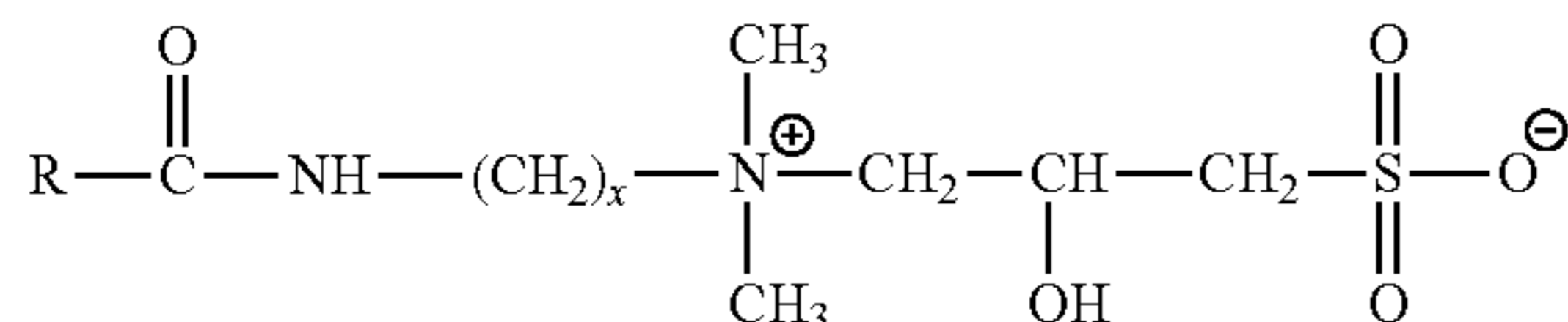
Alkylamidoalkyl hydroxysultaines
