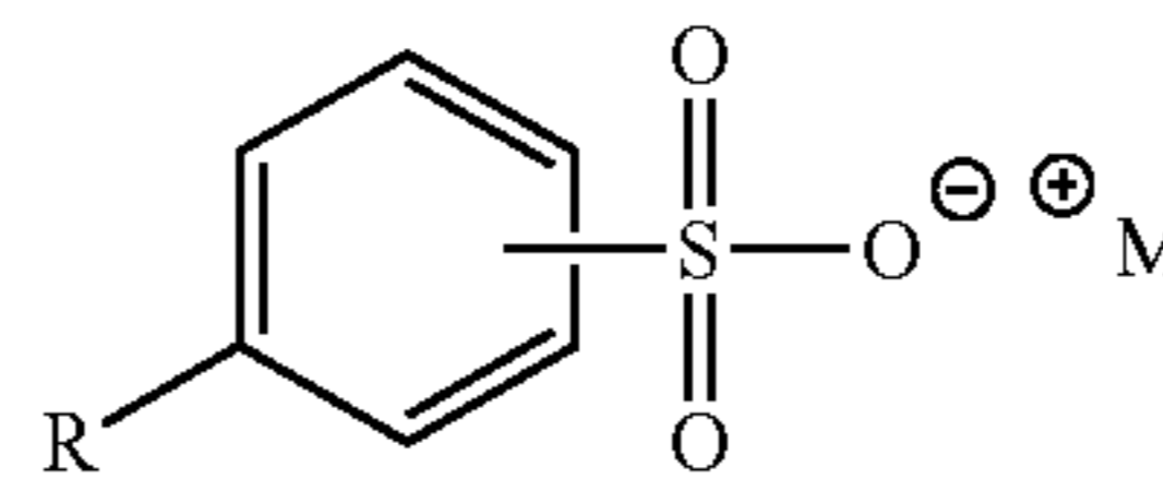
Alkylaryl sulfonates
