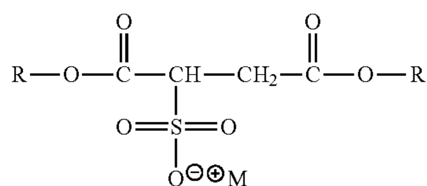
Dialkyl sulfosuccinates
