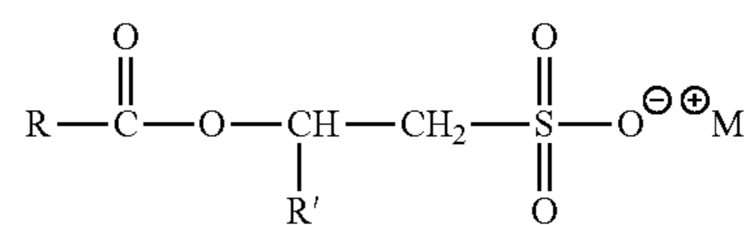
Acyl isethionates
