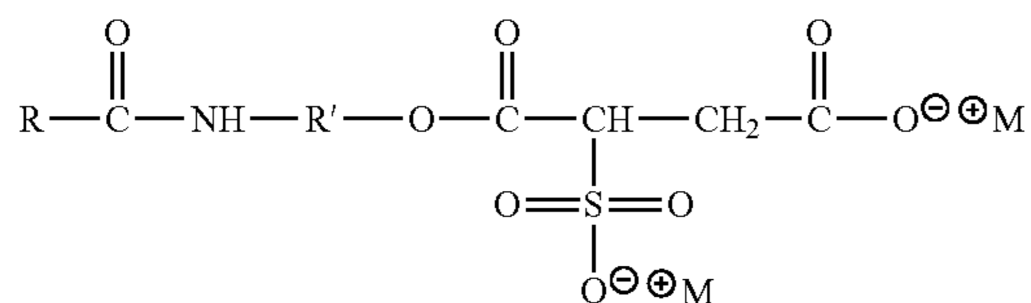
Alkylamidoalkyl sulfosuccinates
