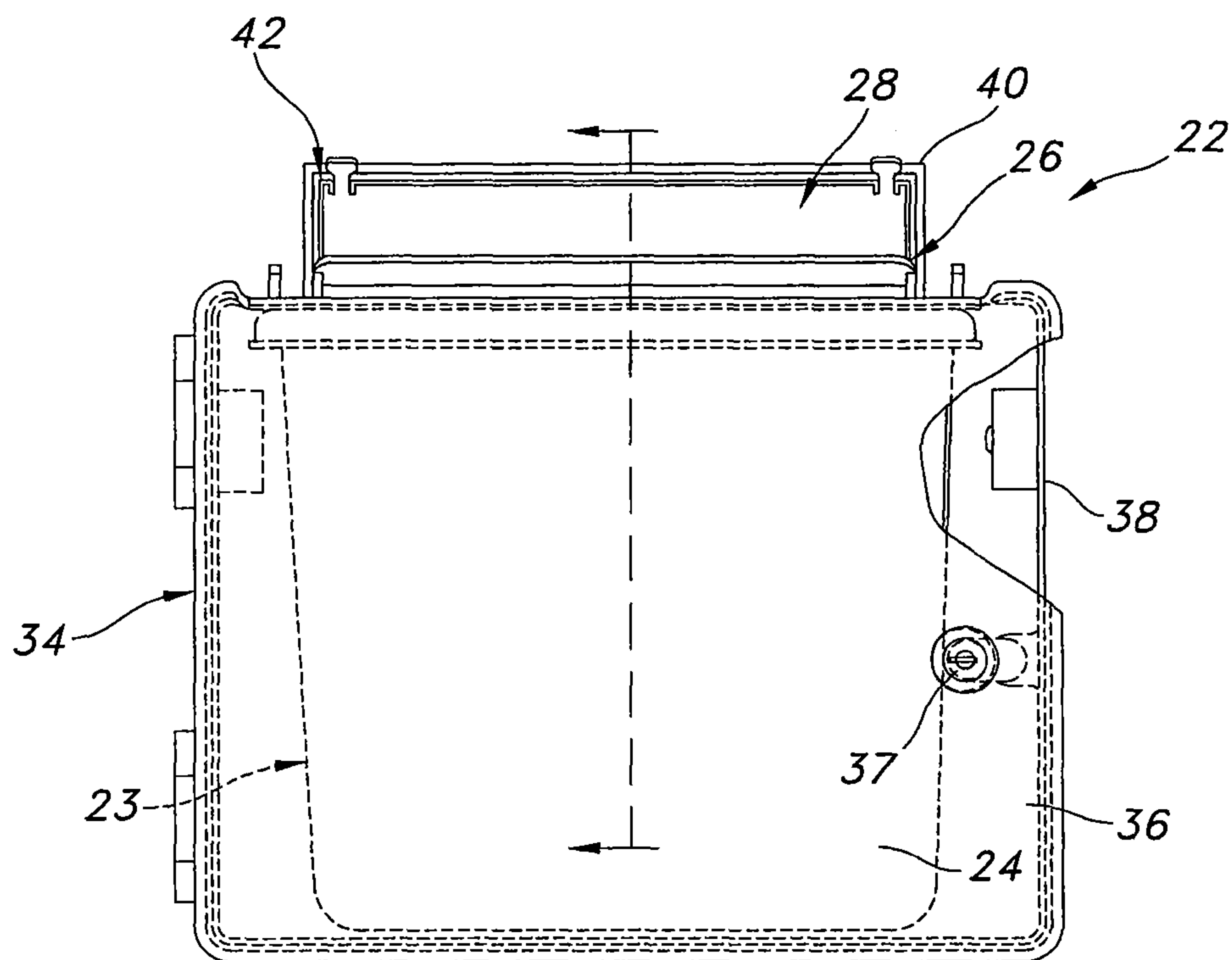
FIG. 3 (Prior Art)
