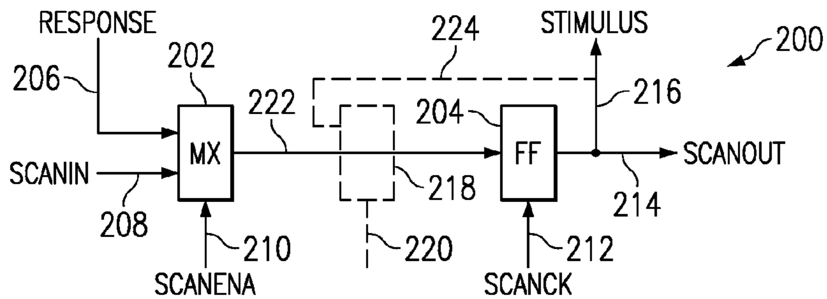
FIG. 2 (PRIOR ART)
