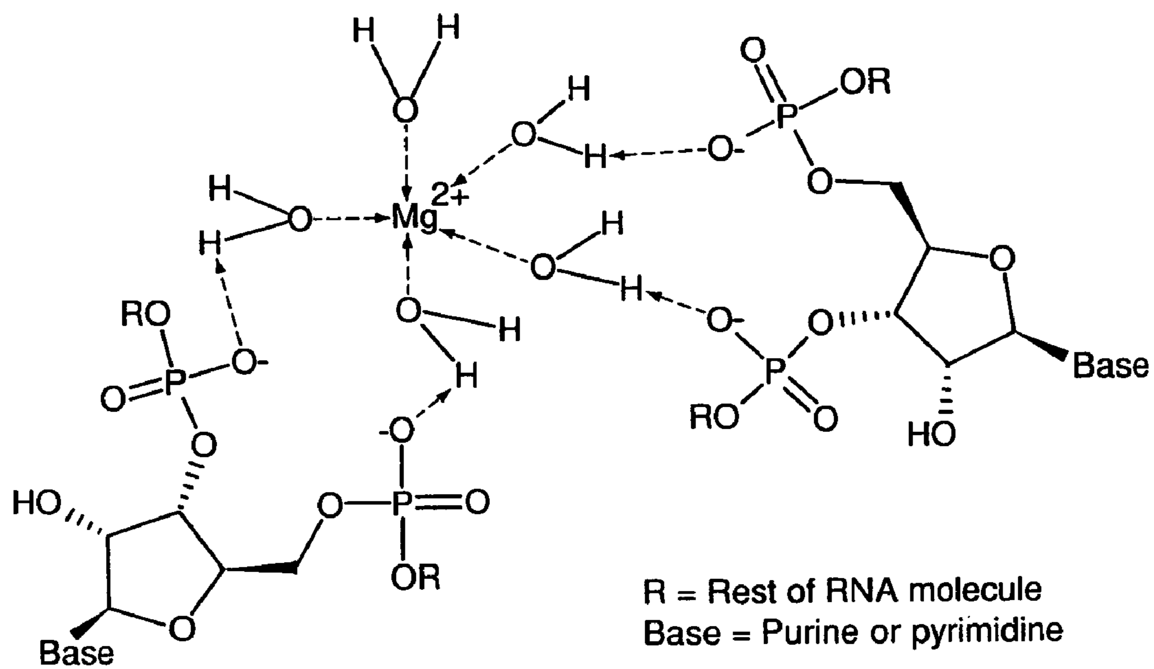
Outer sphere RNA:Magnesium Coordination Complex
