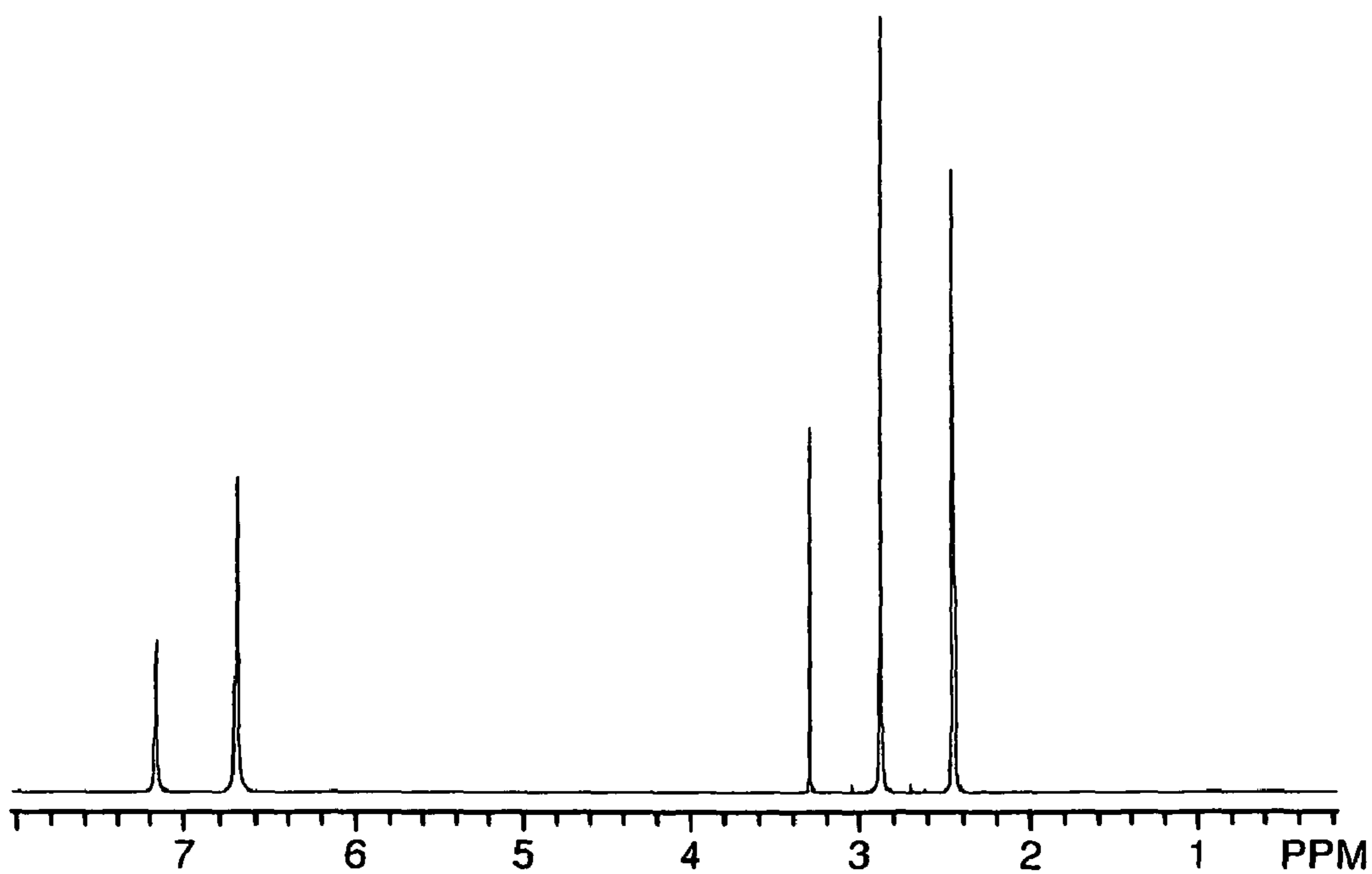
Proton NMR of Dimethylbiguanide
