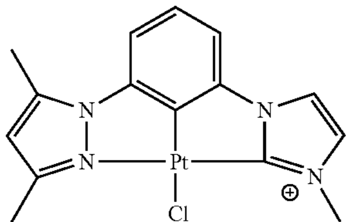
DMPz-Ph-MIzCb-PtCl
