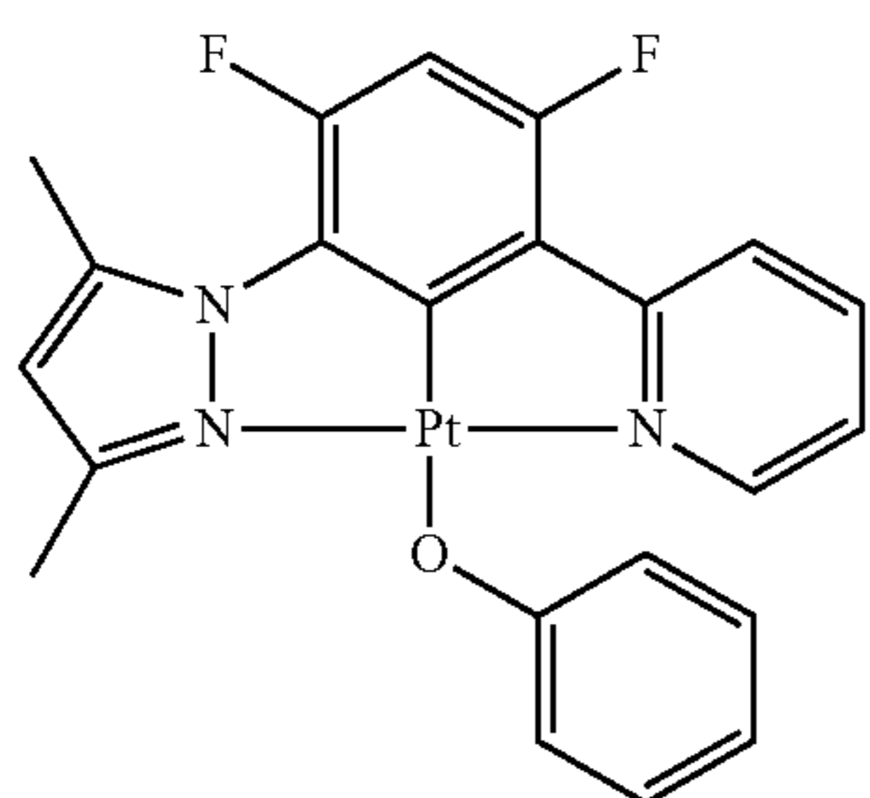
DMPz-DFPh-Py-PtOPh
