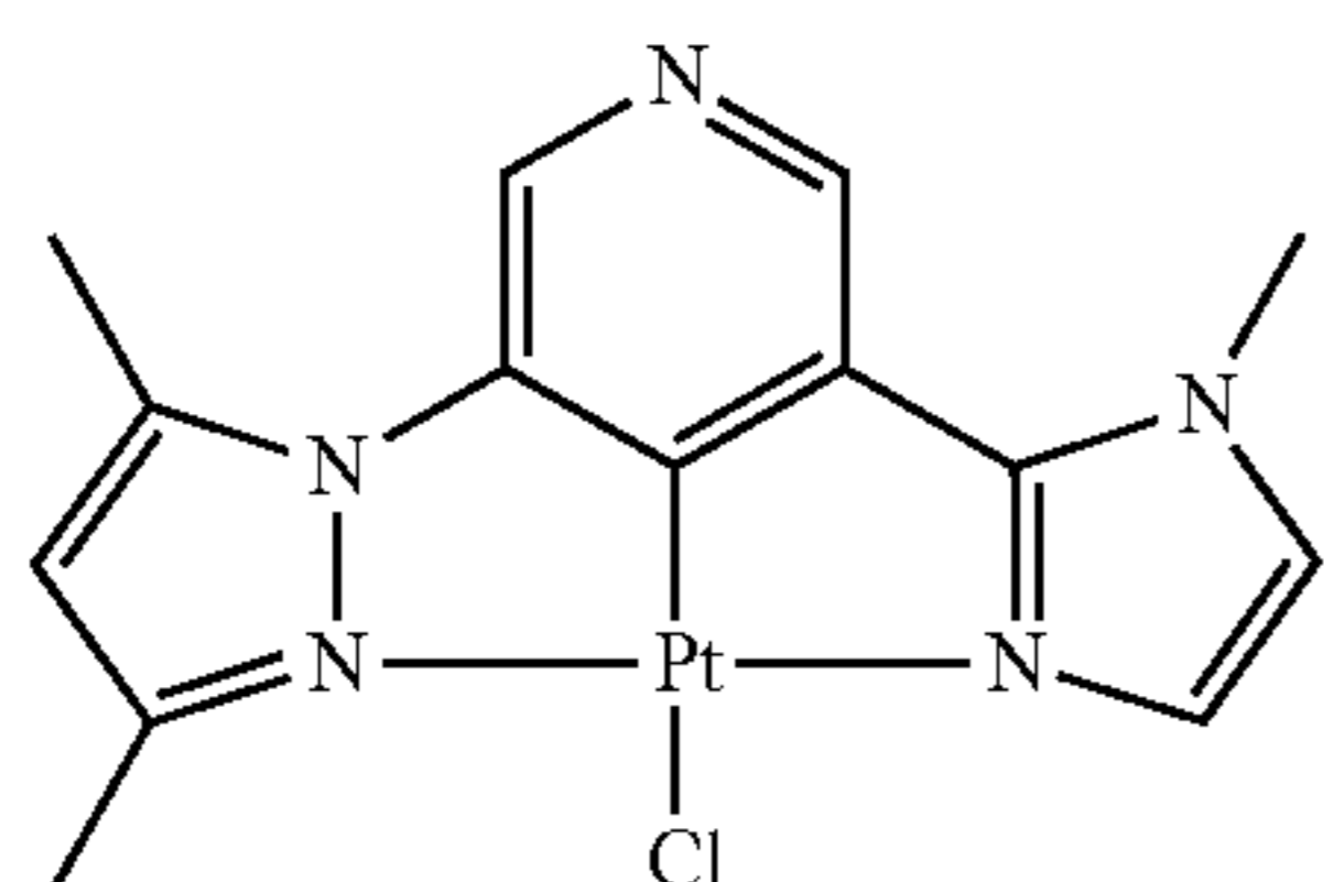
DMPz-Ph-MIz-PtCl
