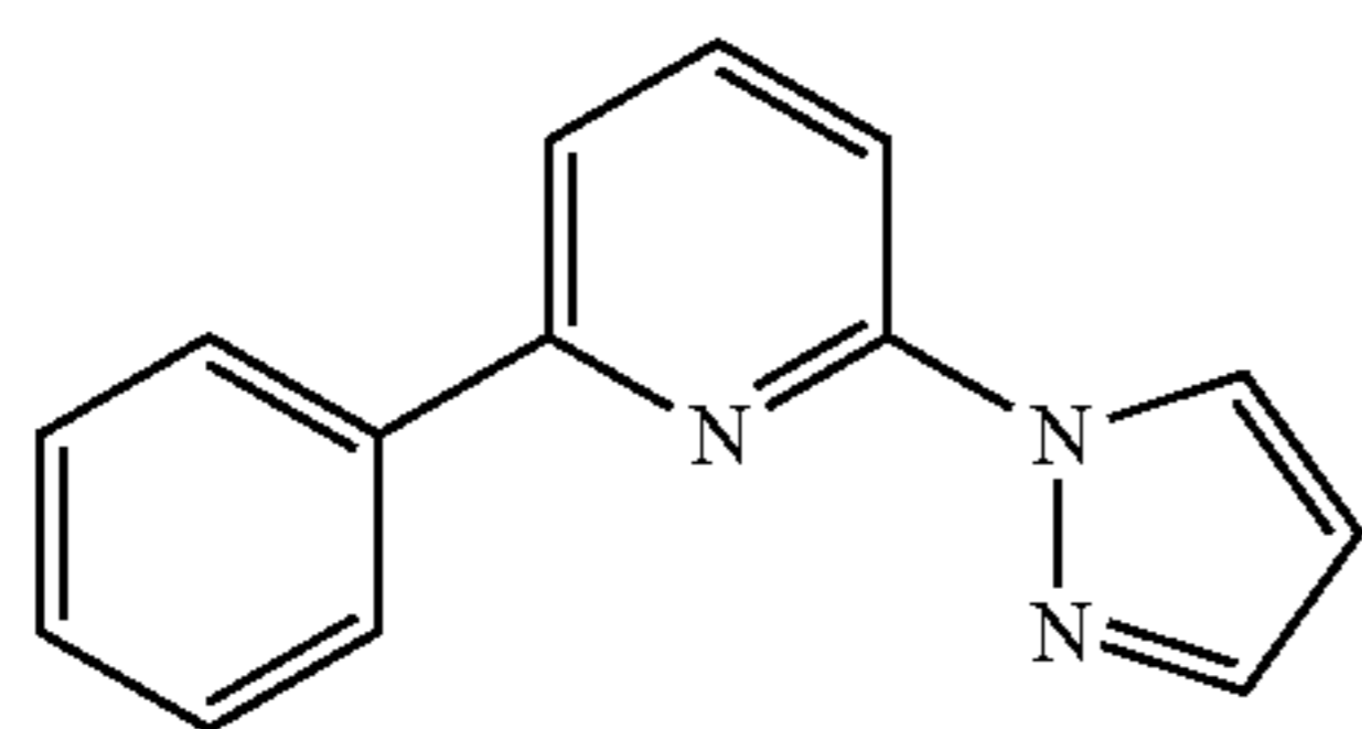
Ph-Py-Pz
