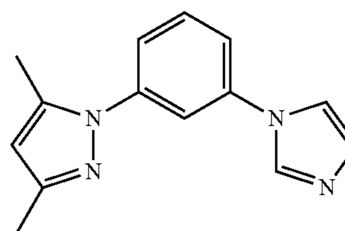
DMPz-Ph-Iz
