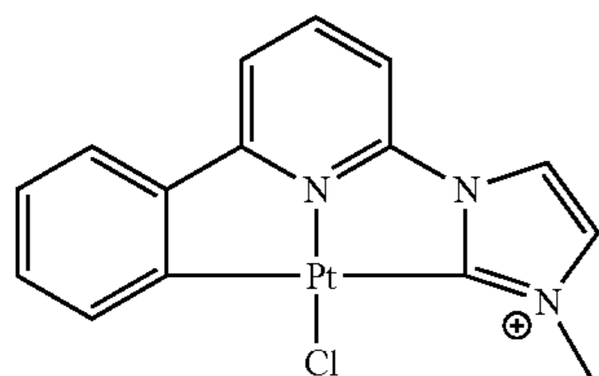
Ph-Py-MIzCb-PtCl
