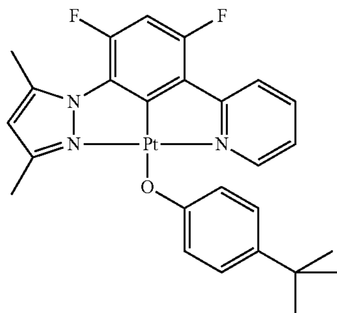
DMPz-DFPh-Py-PtOPhBu
