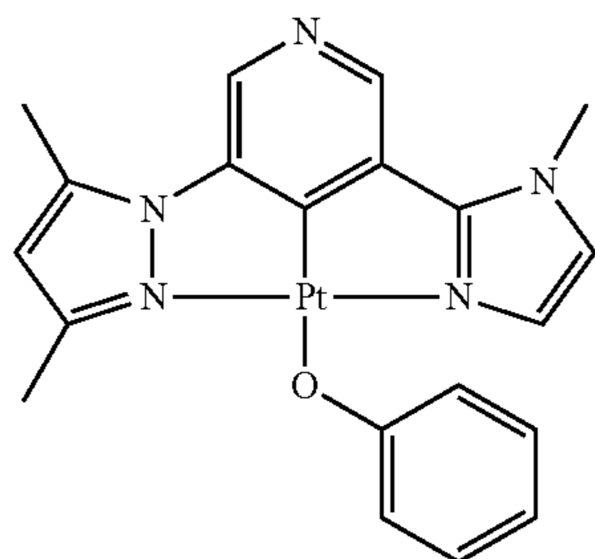
DMPz-Py-MIz-PtOPh
