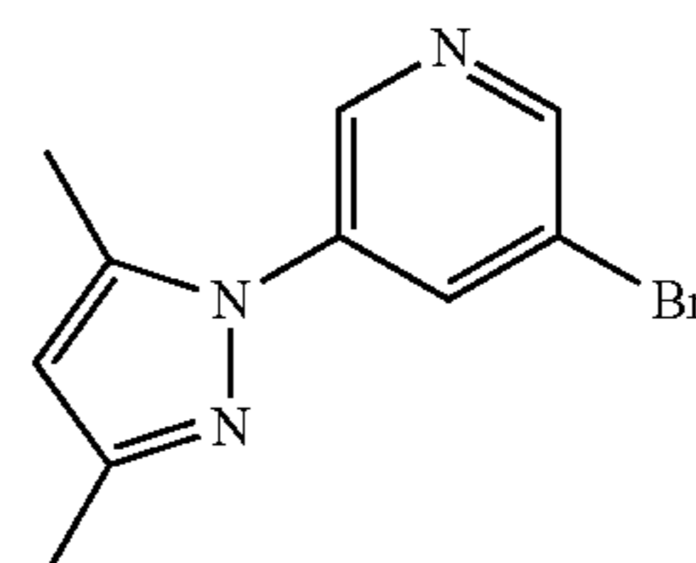
DMPz-Py-Br
