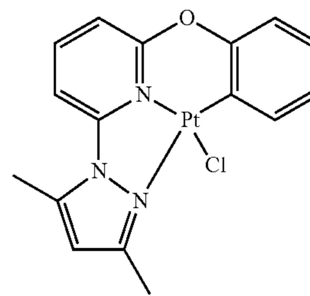
DMPz-Py-O-Ph-PtCl
