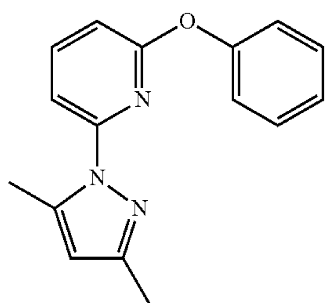
DMPz-Py-O-Ph
