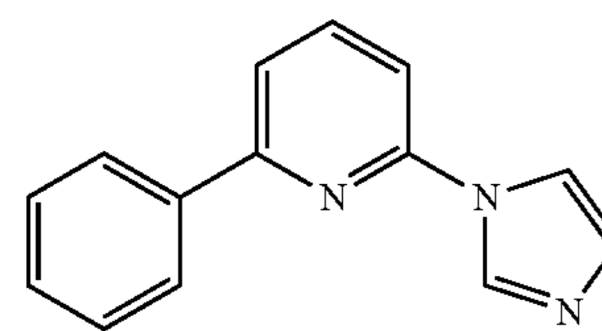
Ph-Py-Iz
