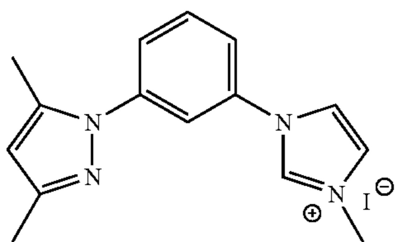
DMPz-Ph-IMz
