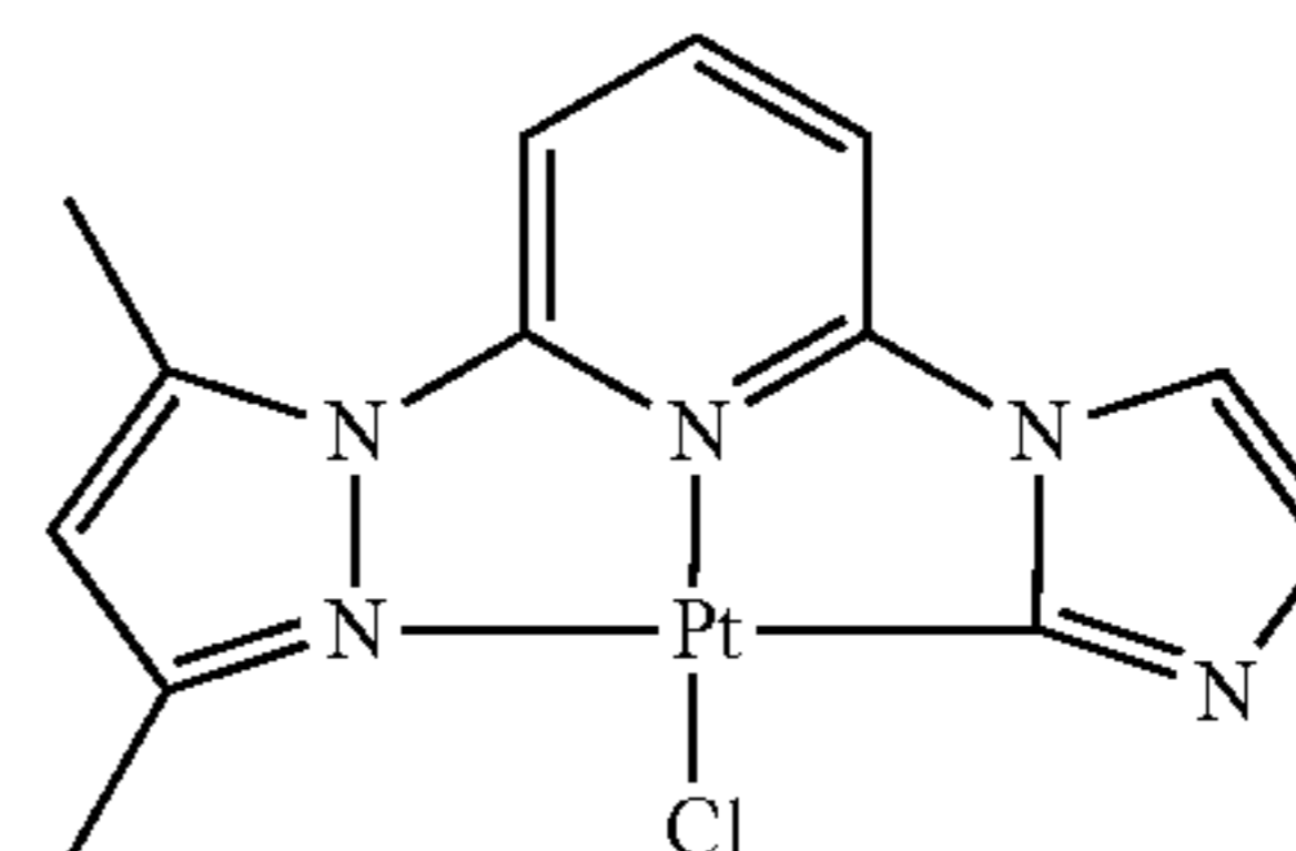
DMPz-Py-Iz-PtCl
