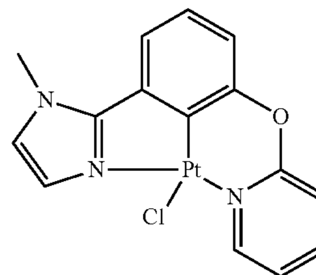
MIz-Ph-O-Py-PtCl
