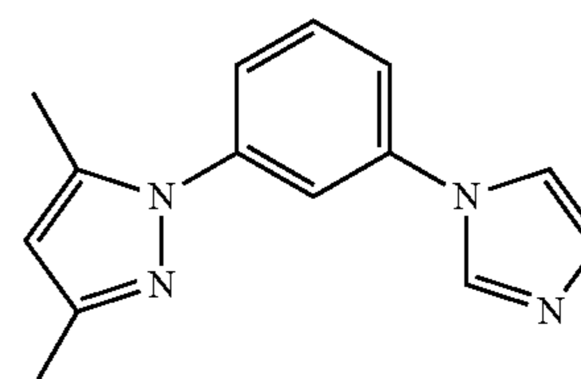
DMPz-Ph-Iz
