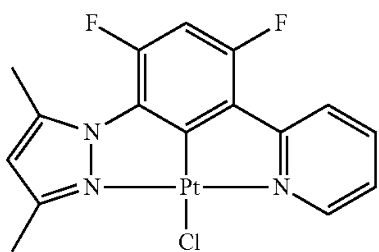
DMPz-DFPh-Py-PtCl
