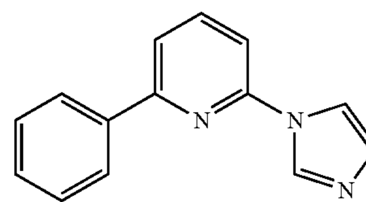
Ph-Py-Iz
