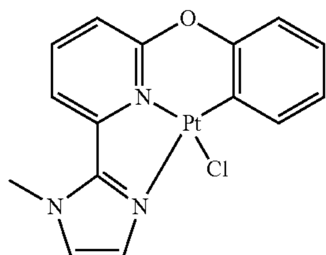
MIz-Py-Ph-PtCl
