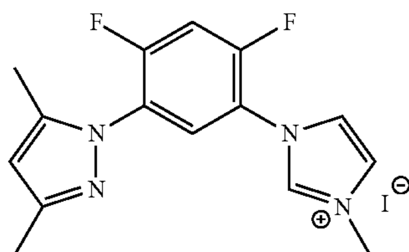
DMPz-Ph-IMIz
