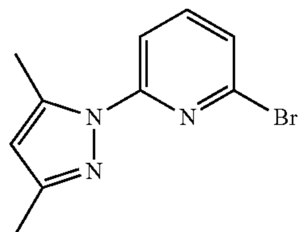
DMPz-Py-Br
