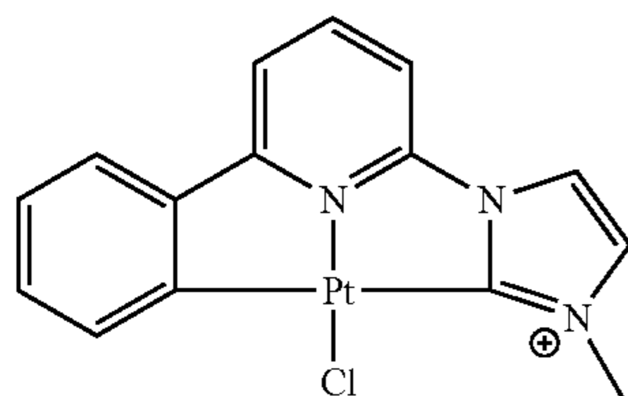
Ph-Py-MIzCb-PtCl
