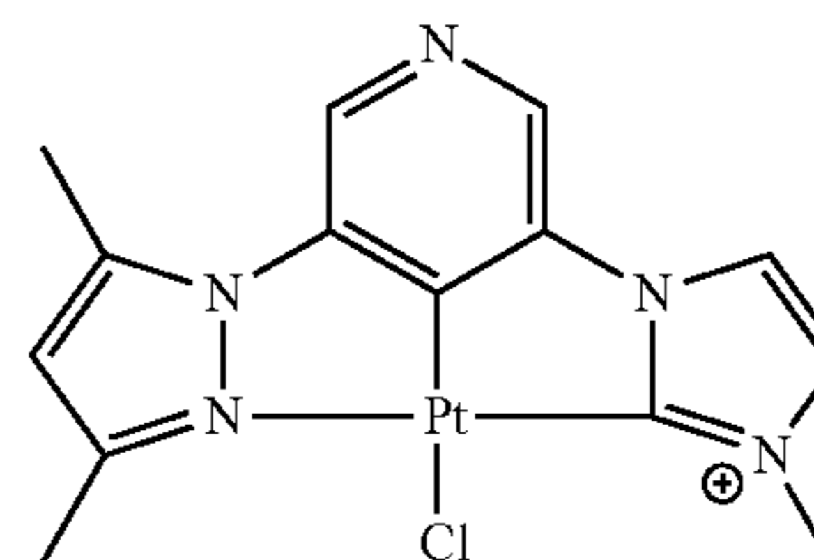
DMPz-Py-MIzCb-PtCl
