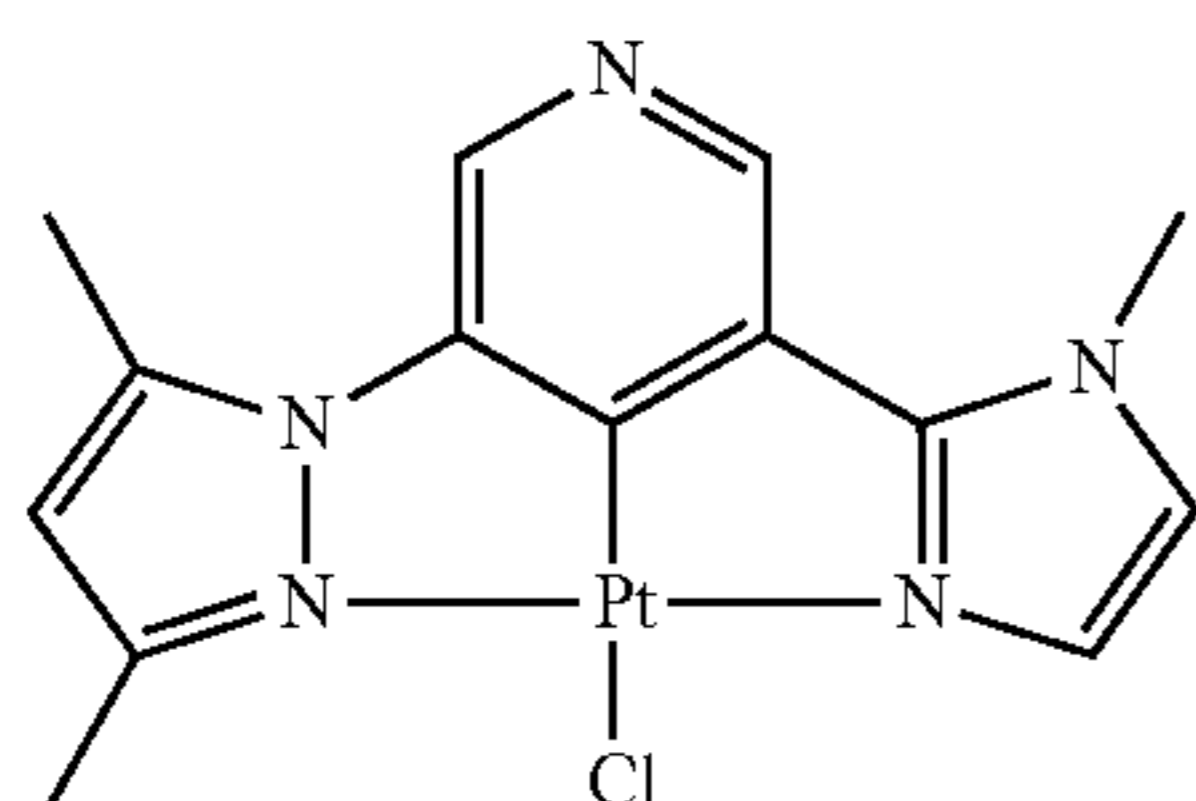
DMPz-Ph-MIz-PtCl
