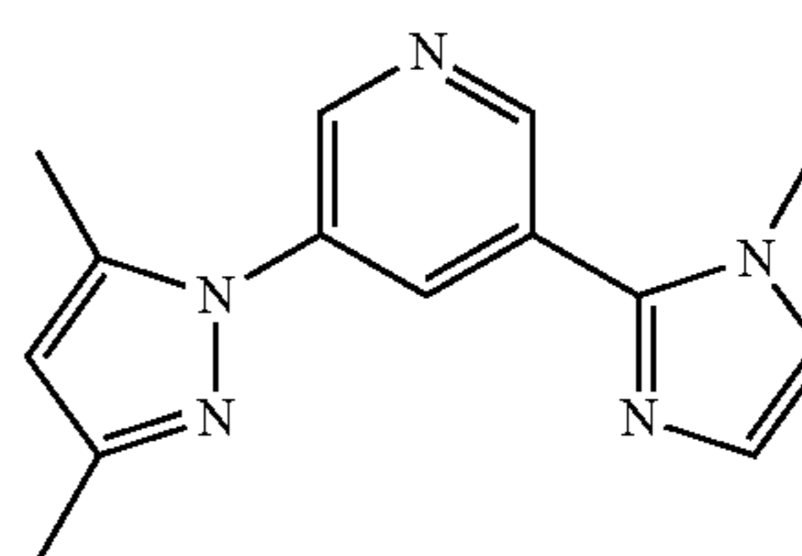
DMPz-Py-IMz
