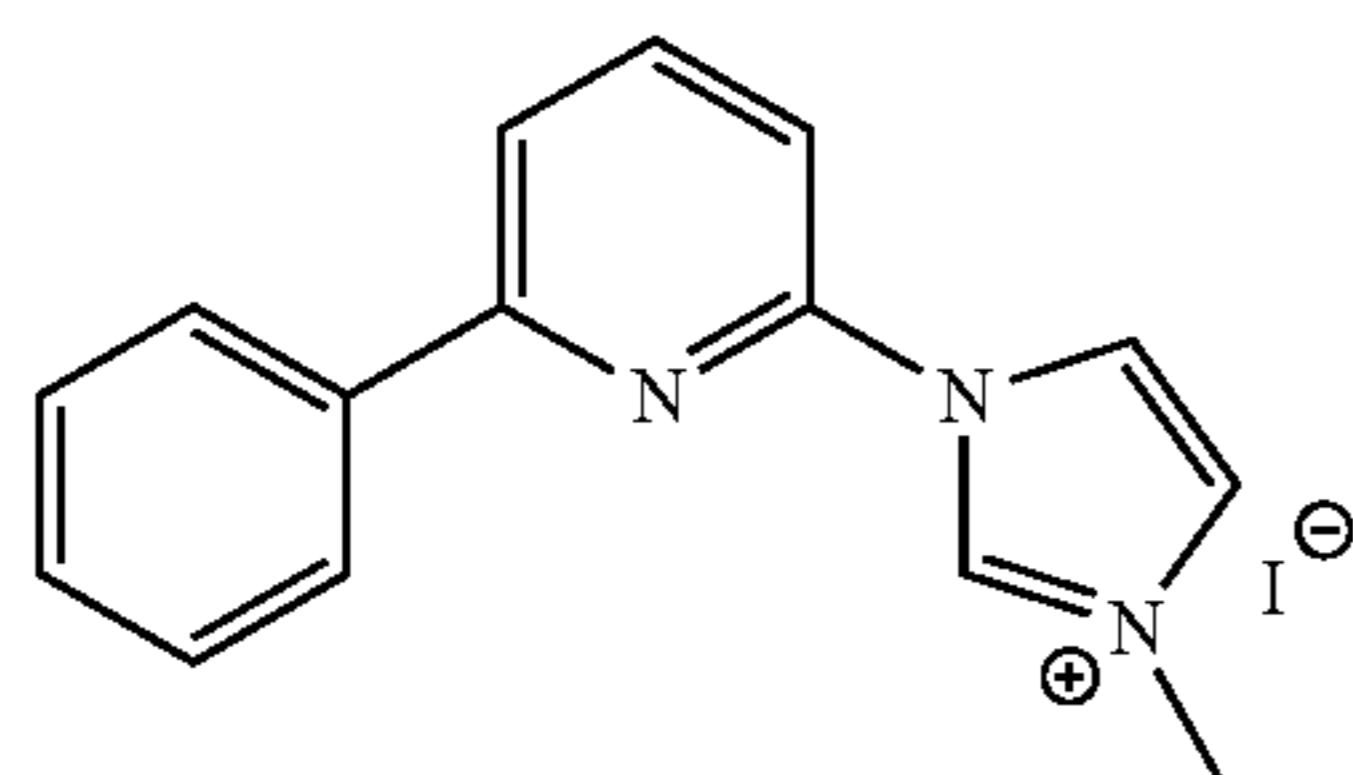
Ph-Py-IMiz
