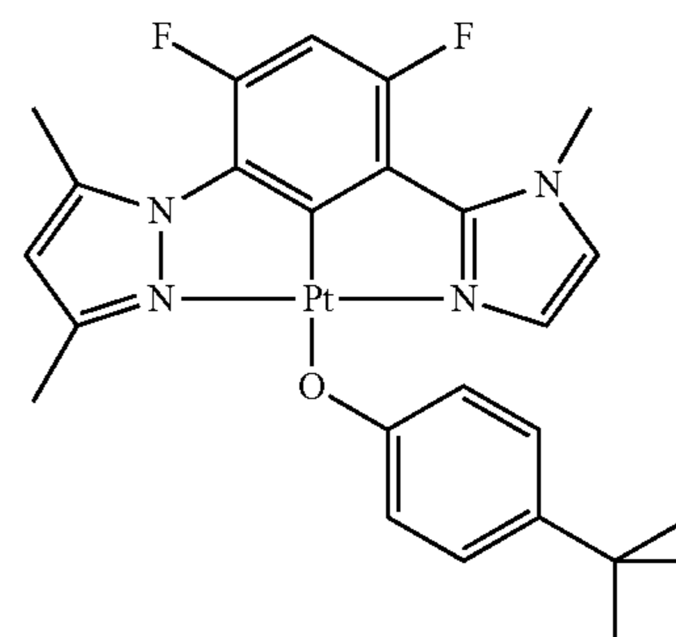
DMPz-DFPh-MIz-PtOPhBu
