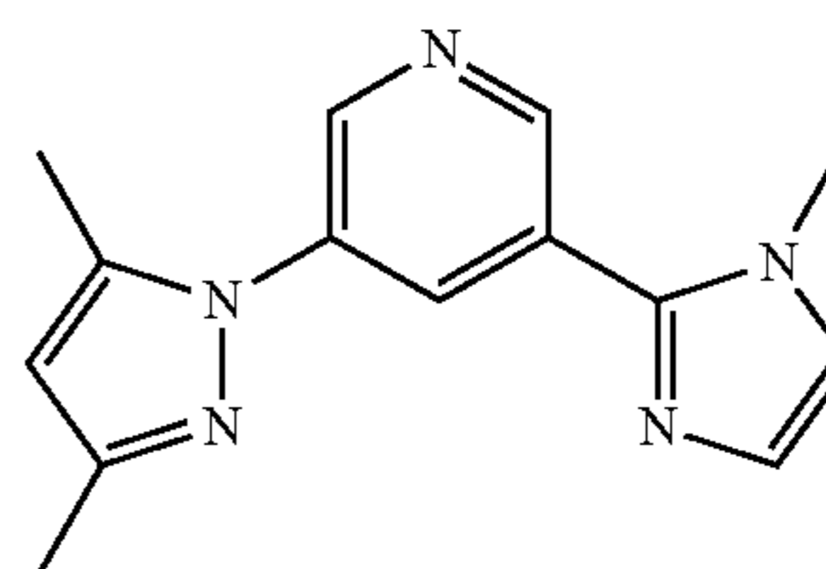
DMPz-Py-IMz
