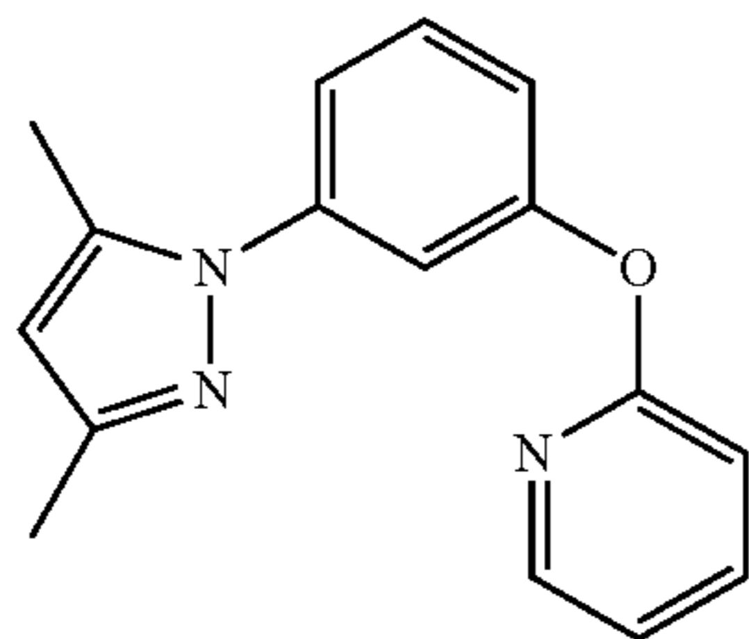
DMPz-Ph-O-Py
