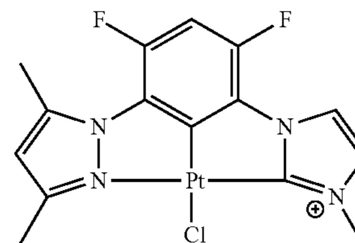
DMPz-Ph-MIzCb-PtCl
