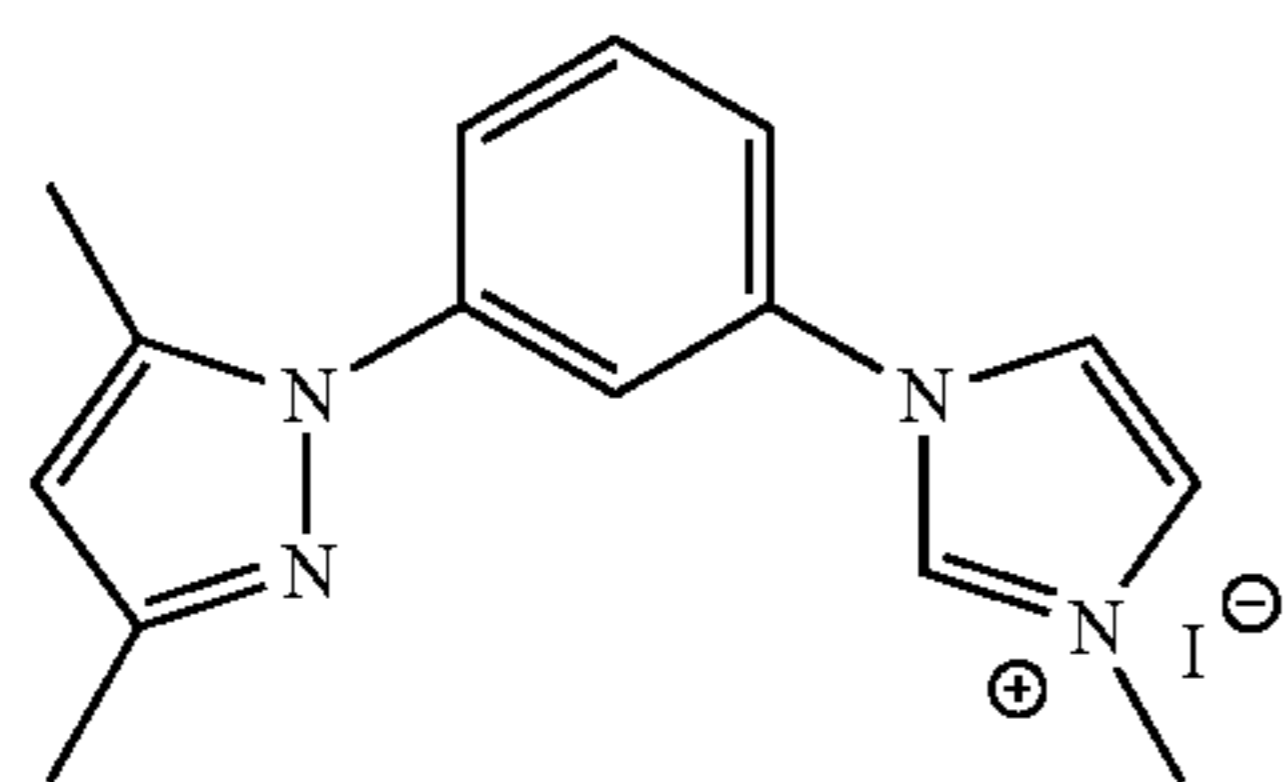
DMPz-Ph-IMz
