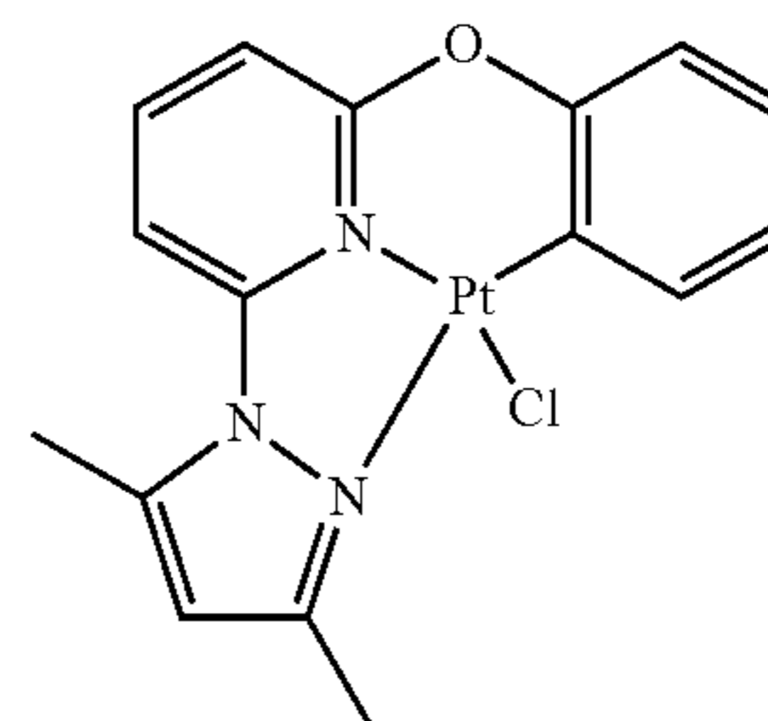
DMPz-Py-O-Ph-PtCl
