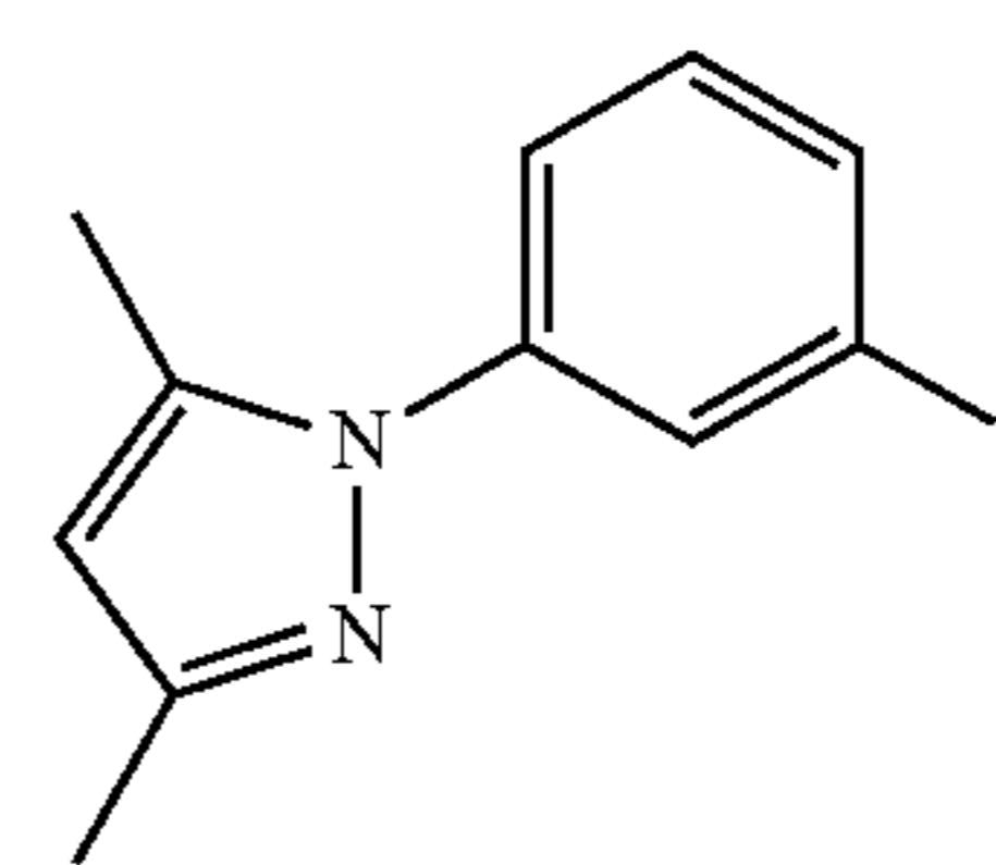
DMPz-Ph-I
