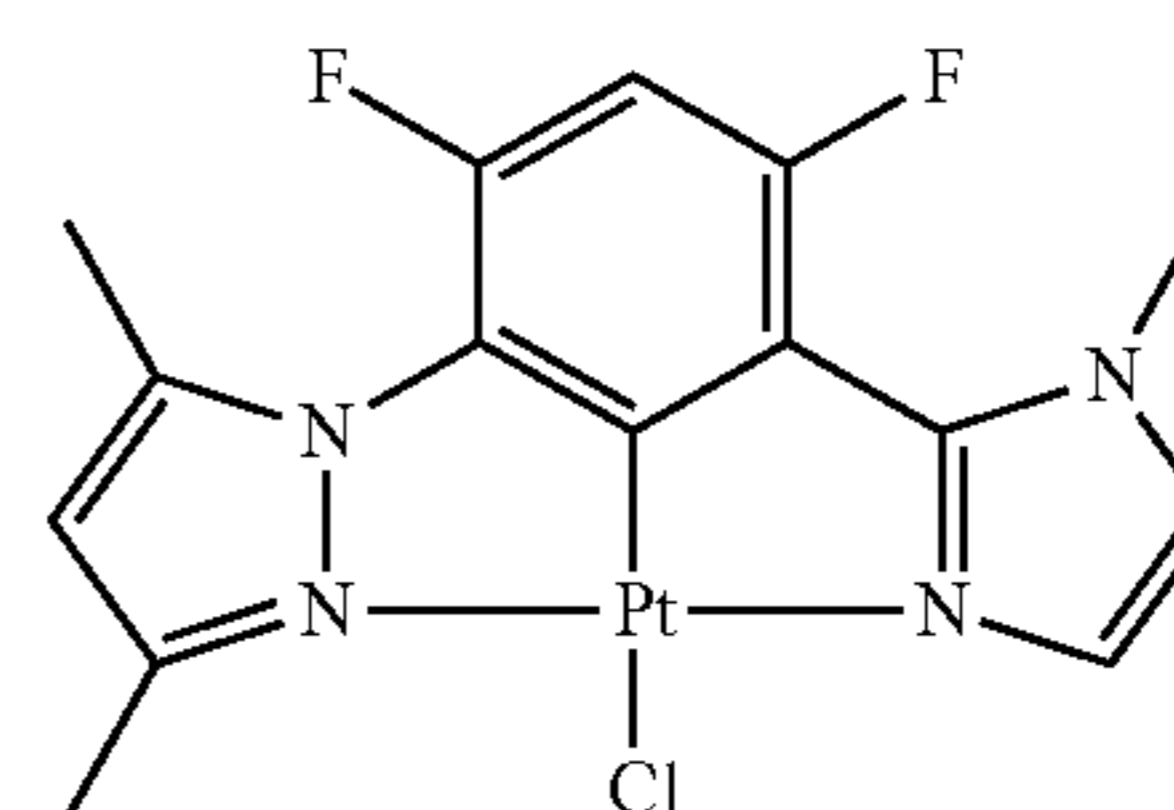
DMPz-DFPh-MIz-PtCl
