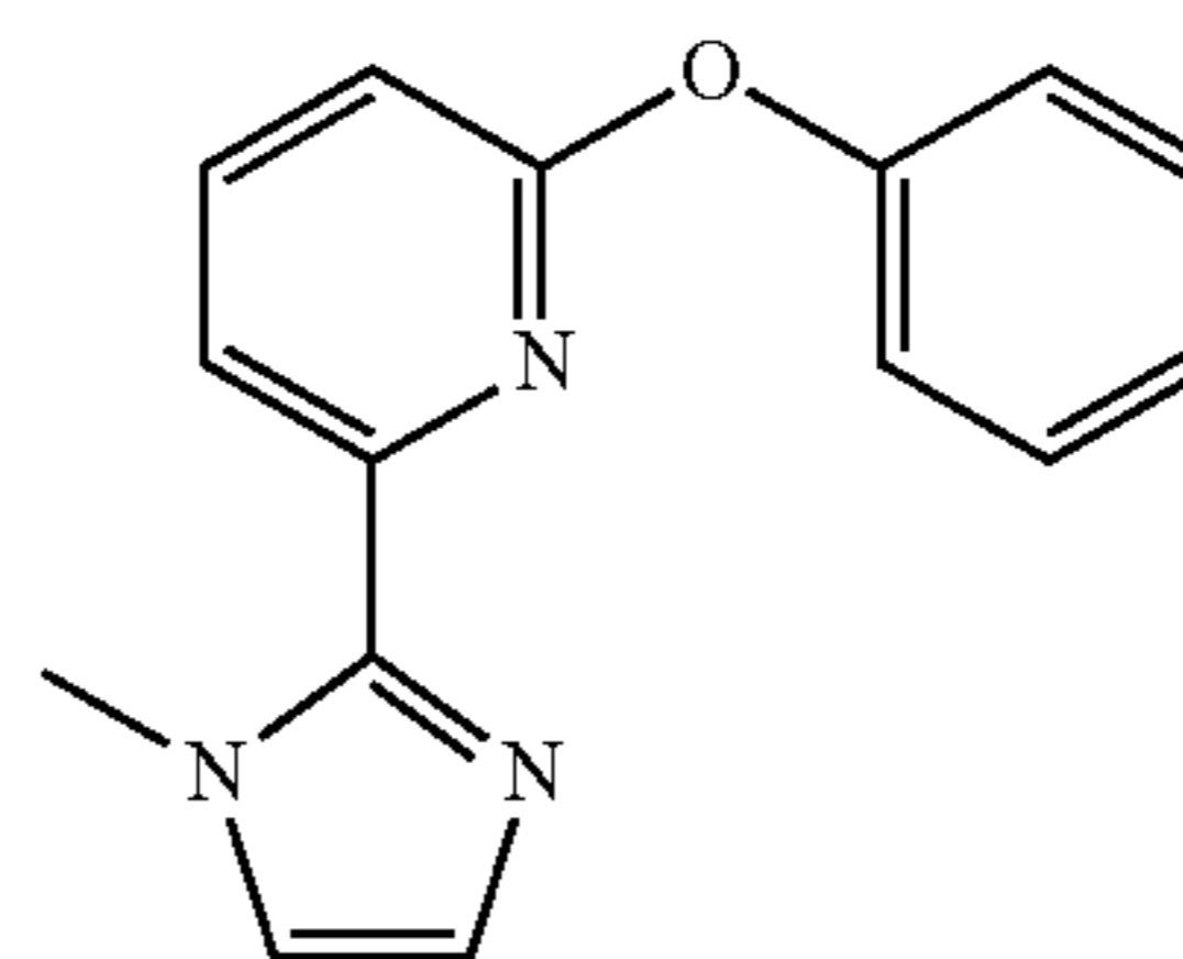
MIz-Py-O-Ph
