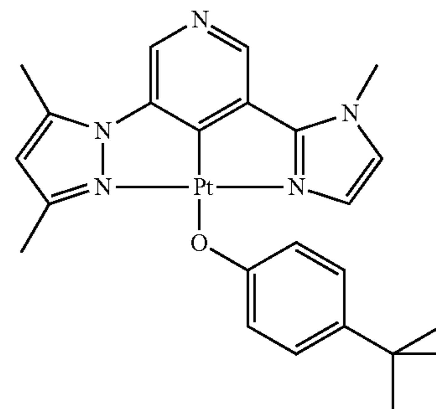
DMPz-Py-MIz-PtOPhBu
