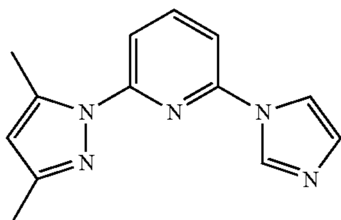
DMPz-Py-Iz
