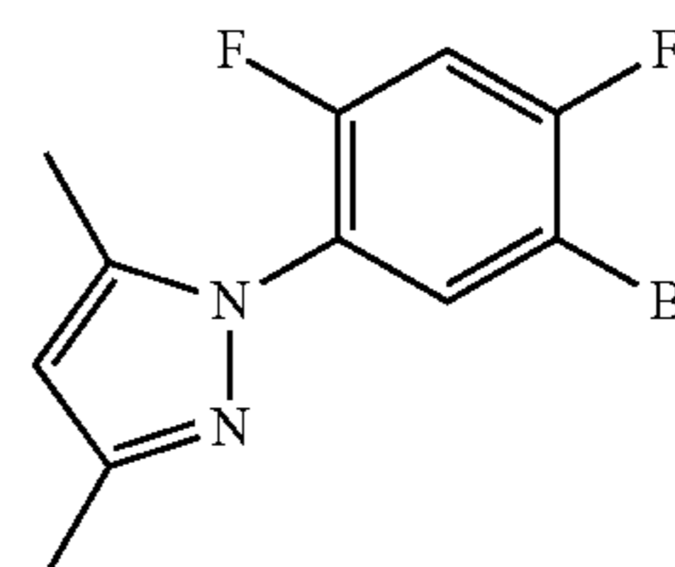
DMPz-DFPh-Br
