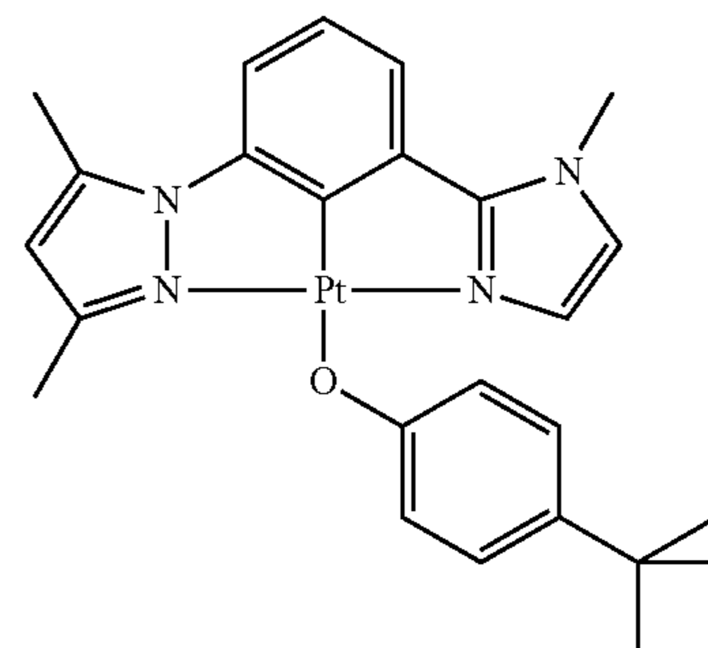
DMPz-Ph-MIz-PtOPhBu
