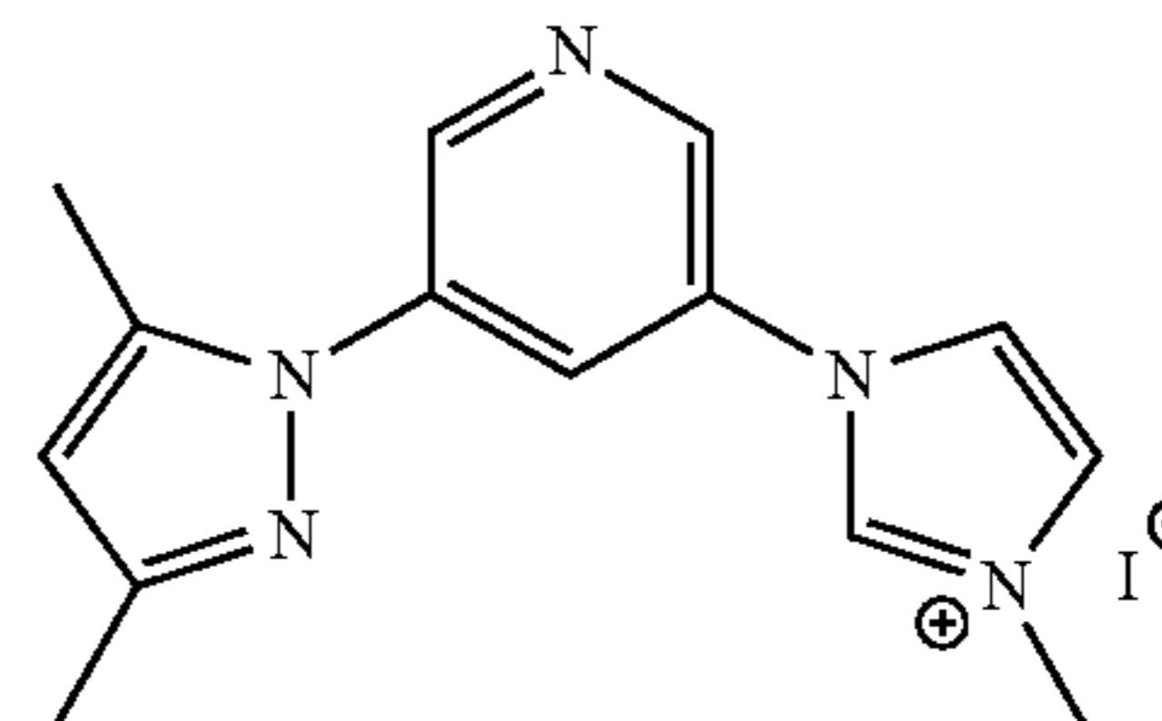
DMPz-Py-IMIz
