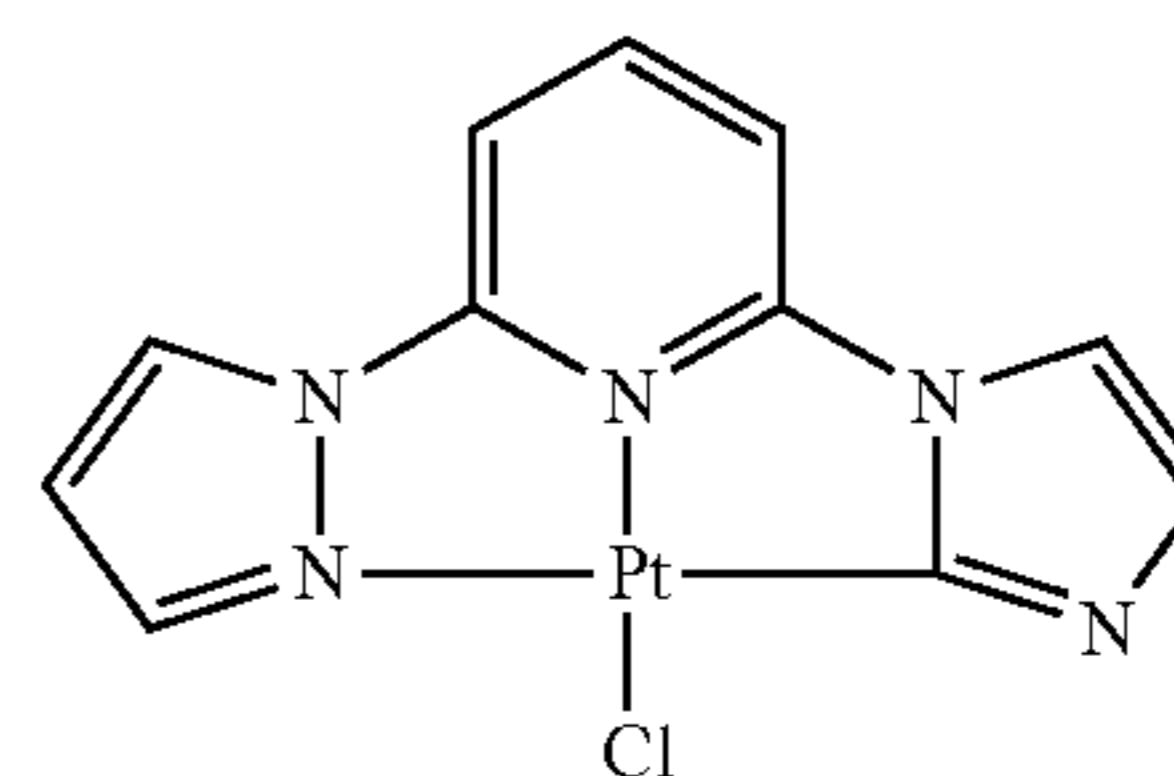
Pz-Py-Iz-PtCl
