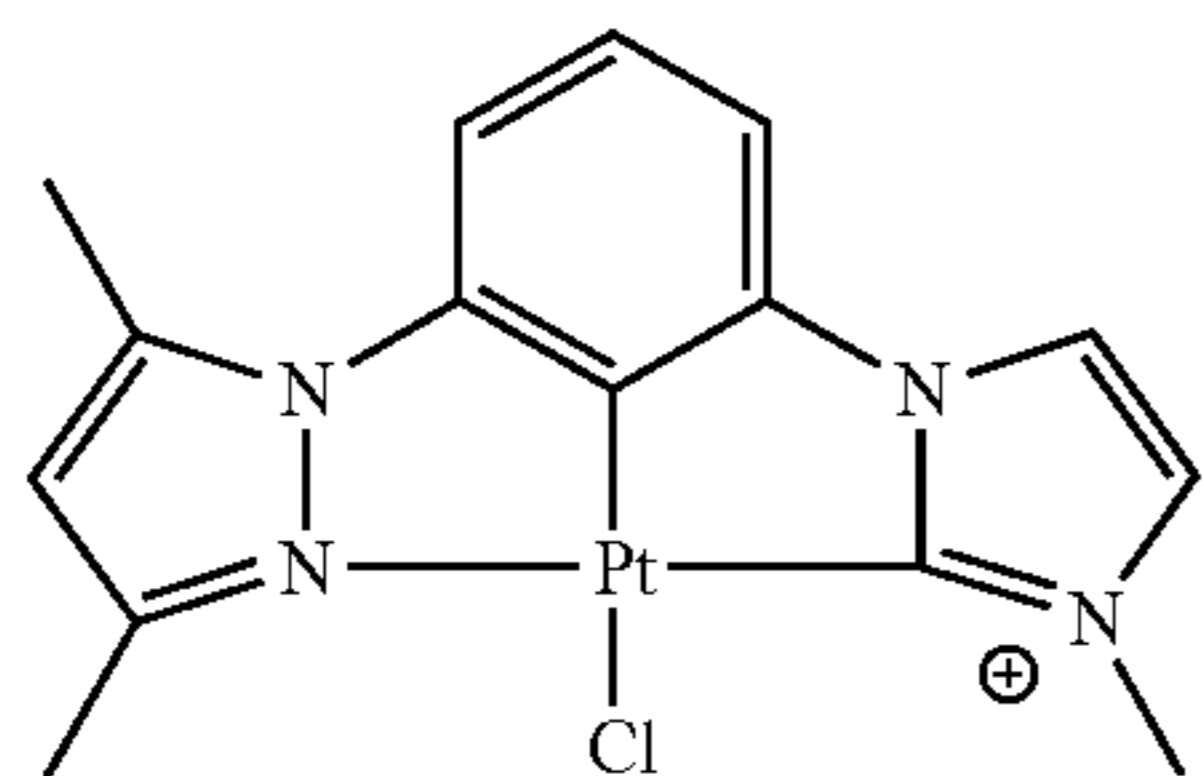
DMPz-Ph-MIzCb-PtCl
