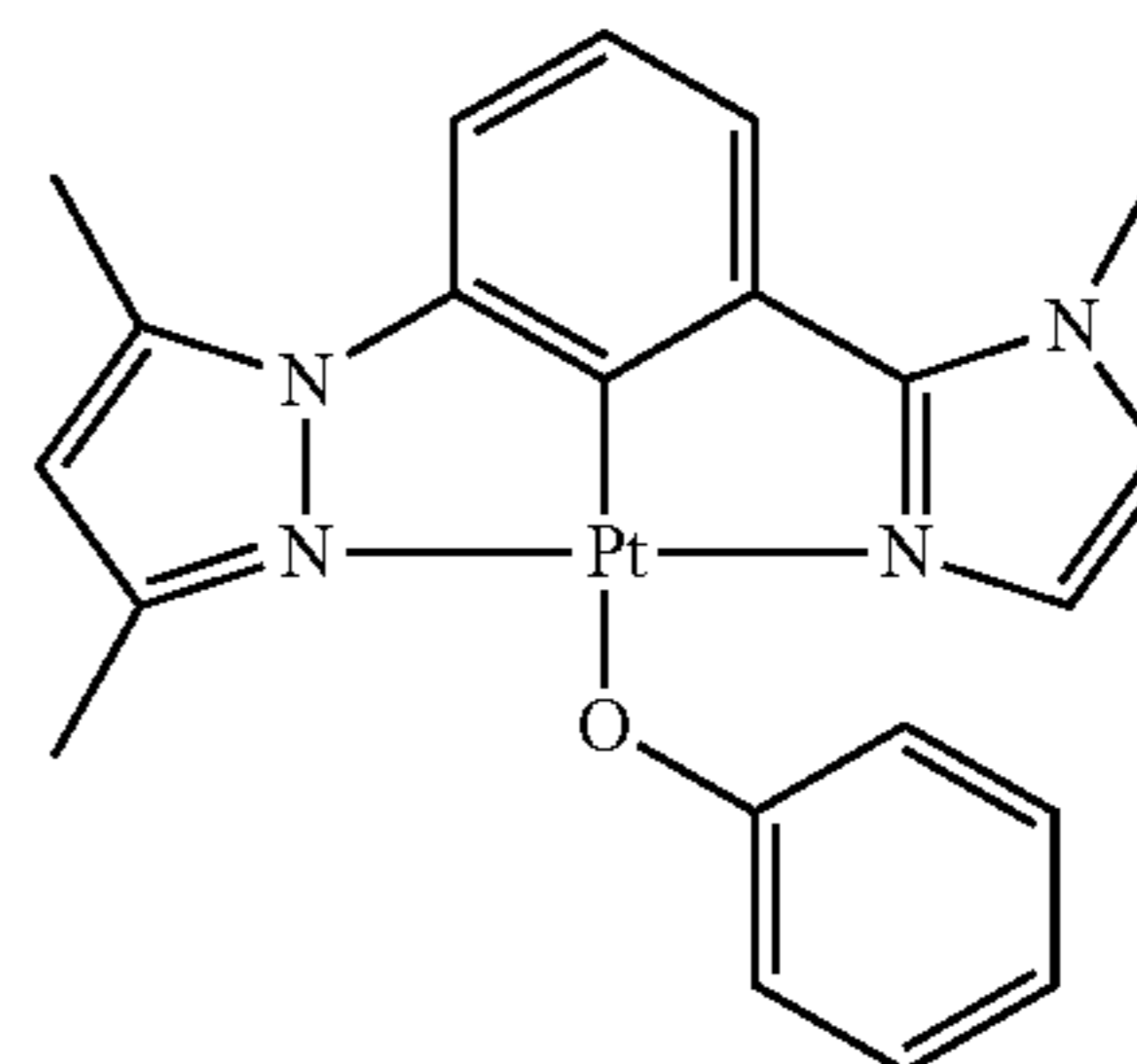
DMPz-Ph-MIz-PtOPh
