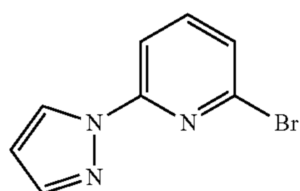
Pz-Py-Br
