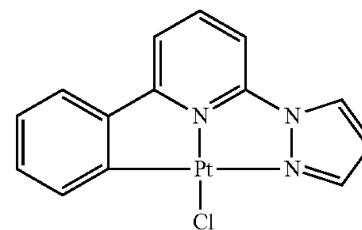
Ph-Py-Pz-PtCl
