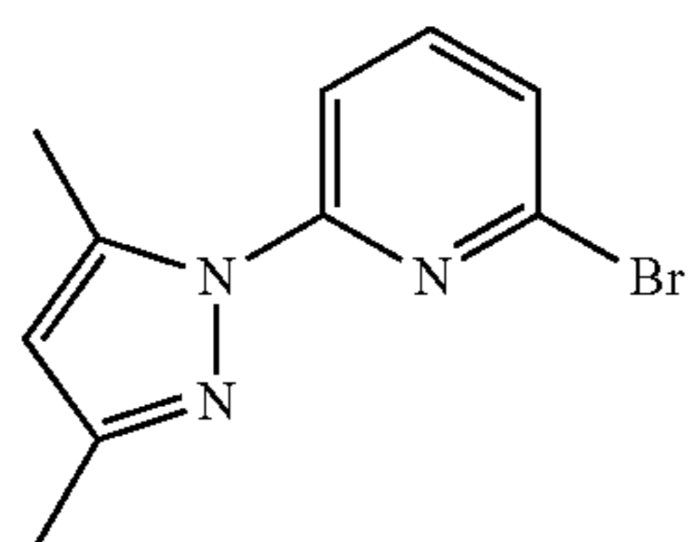
DMPz-Py-Br
