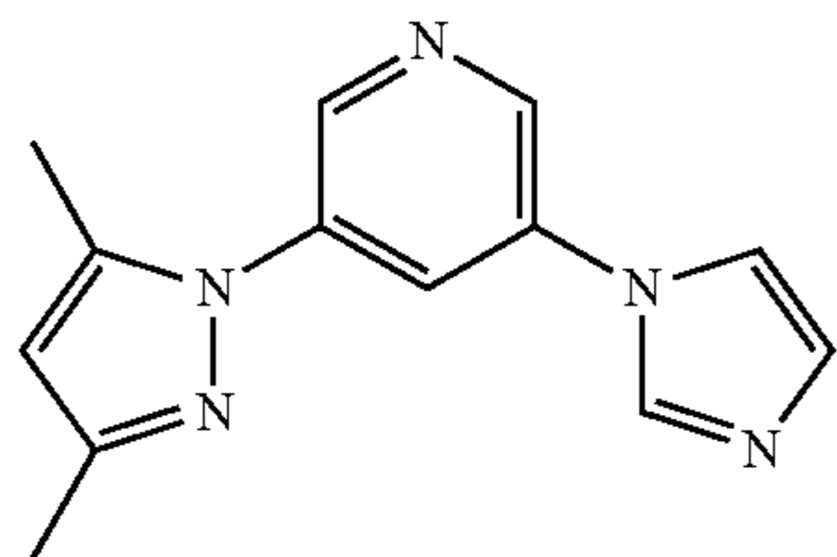
DMPz-Py-Iz
