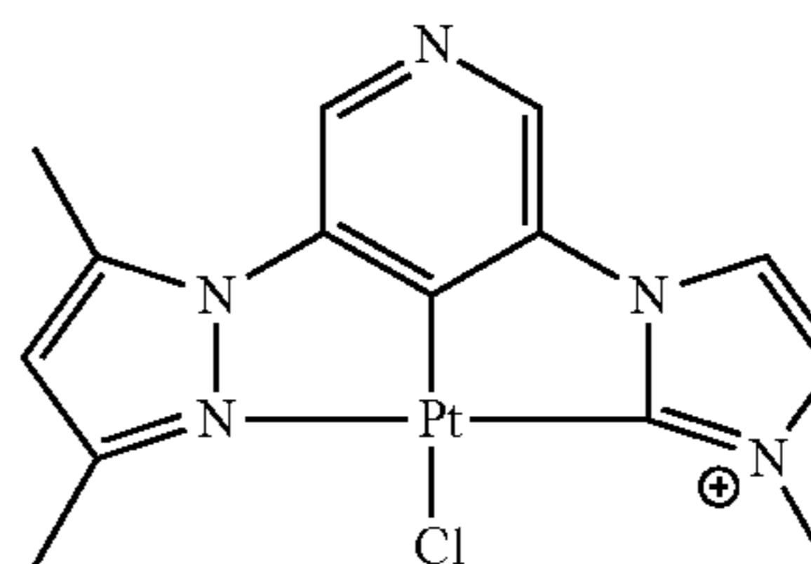
DMPz-Py-MIzCb-PtCl
