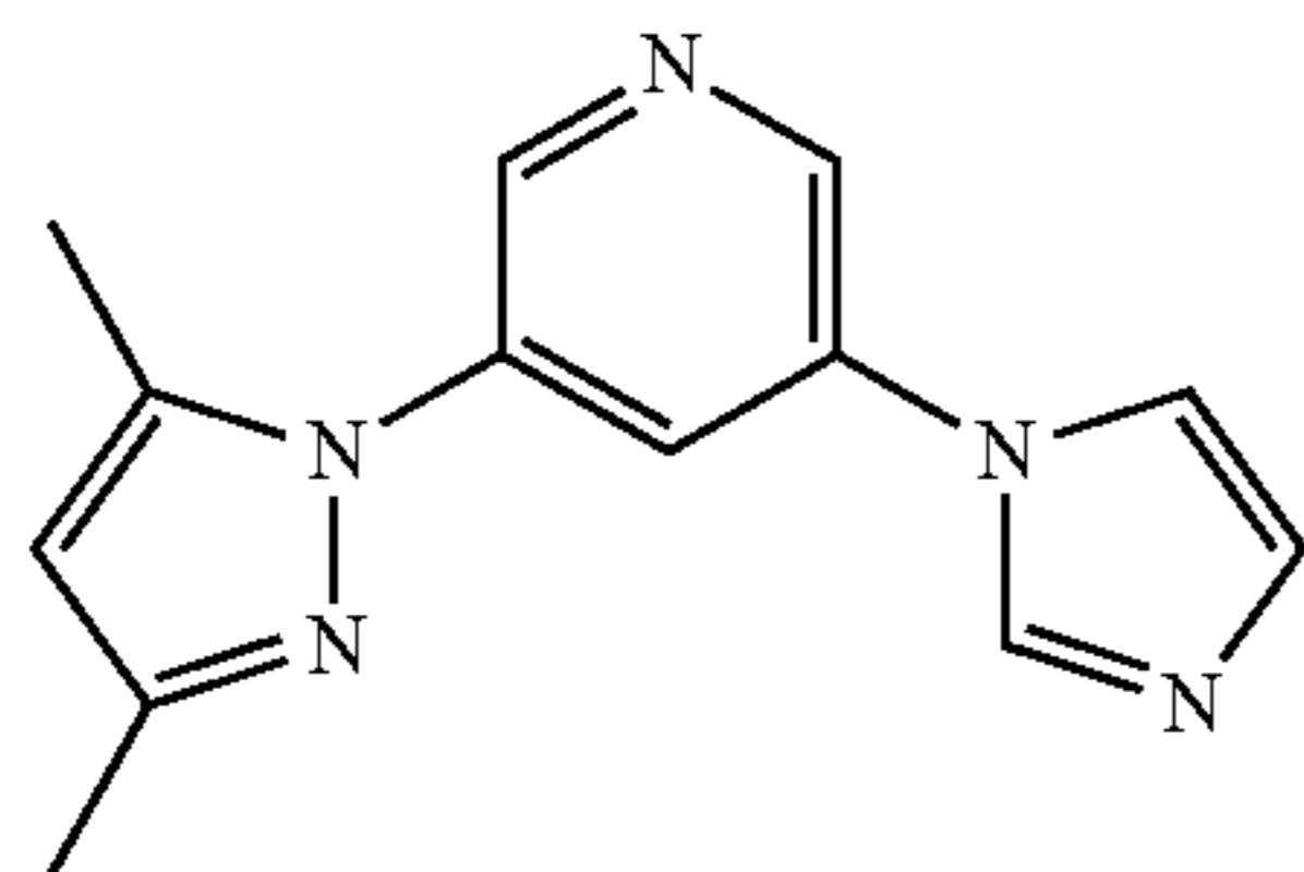
DMPz-Py-Iz
