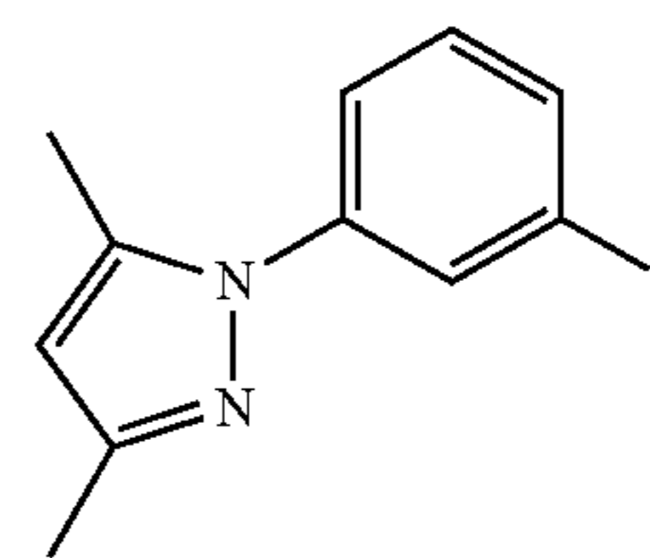
DMPz-Ph-I
