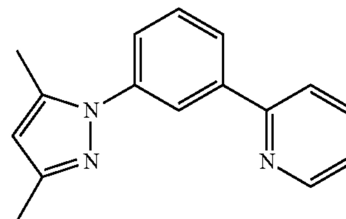
DMPz-Ph-Py
