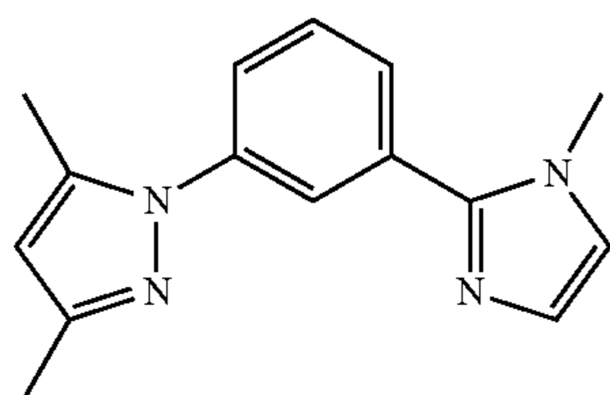
DMPz-Ph-MIz
