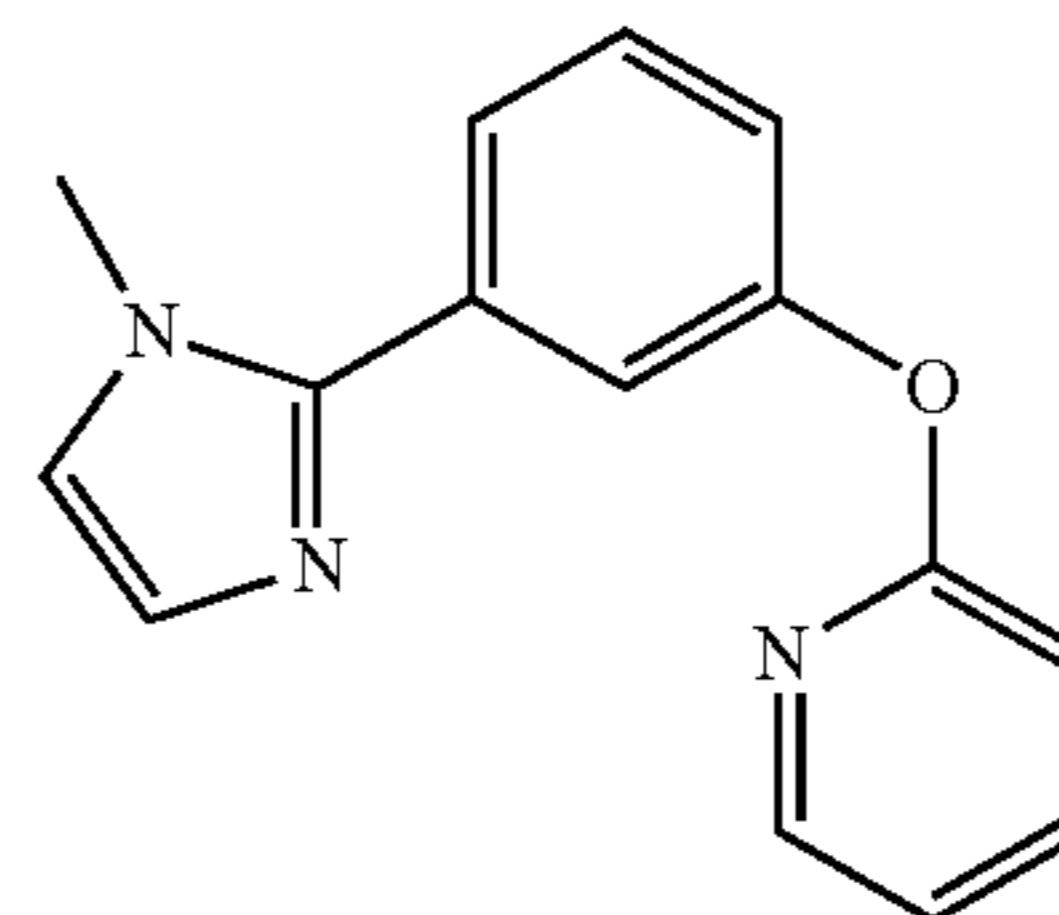
MIz-Ph-O-Py
