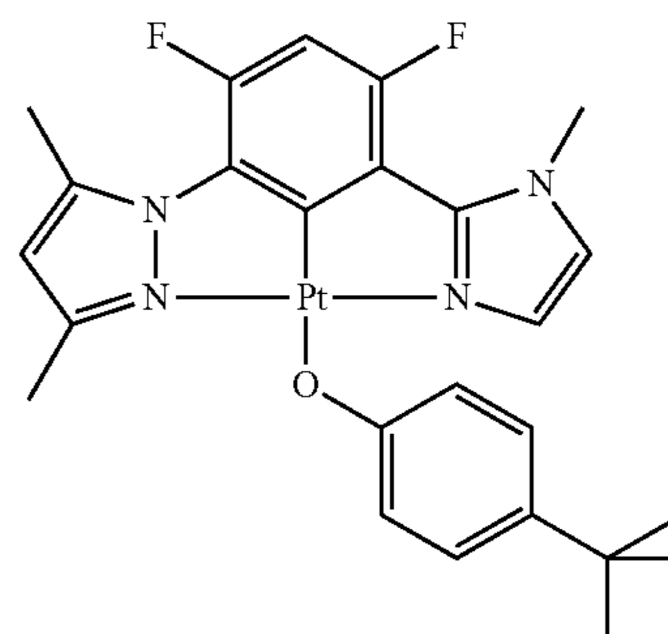
DMPz-DFPh-MIz-PtOPhBu
