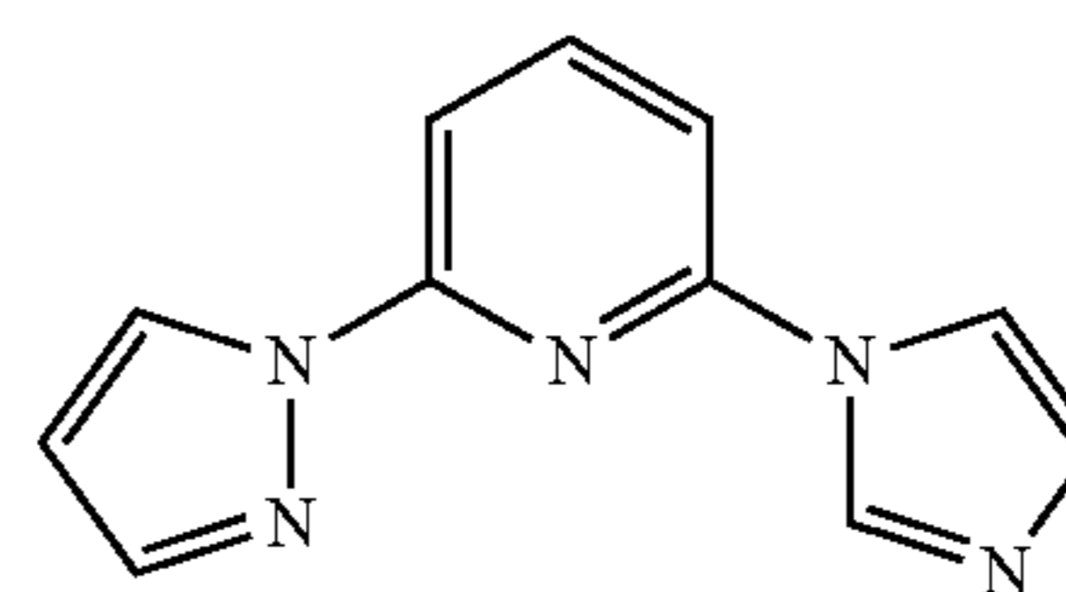
Pz-Py-Iz
