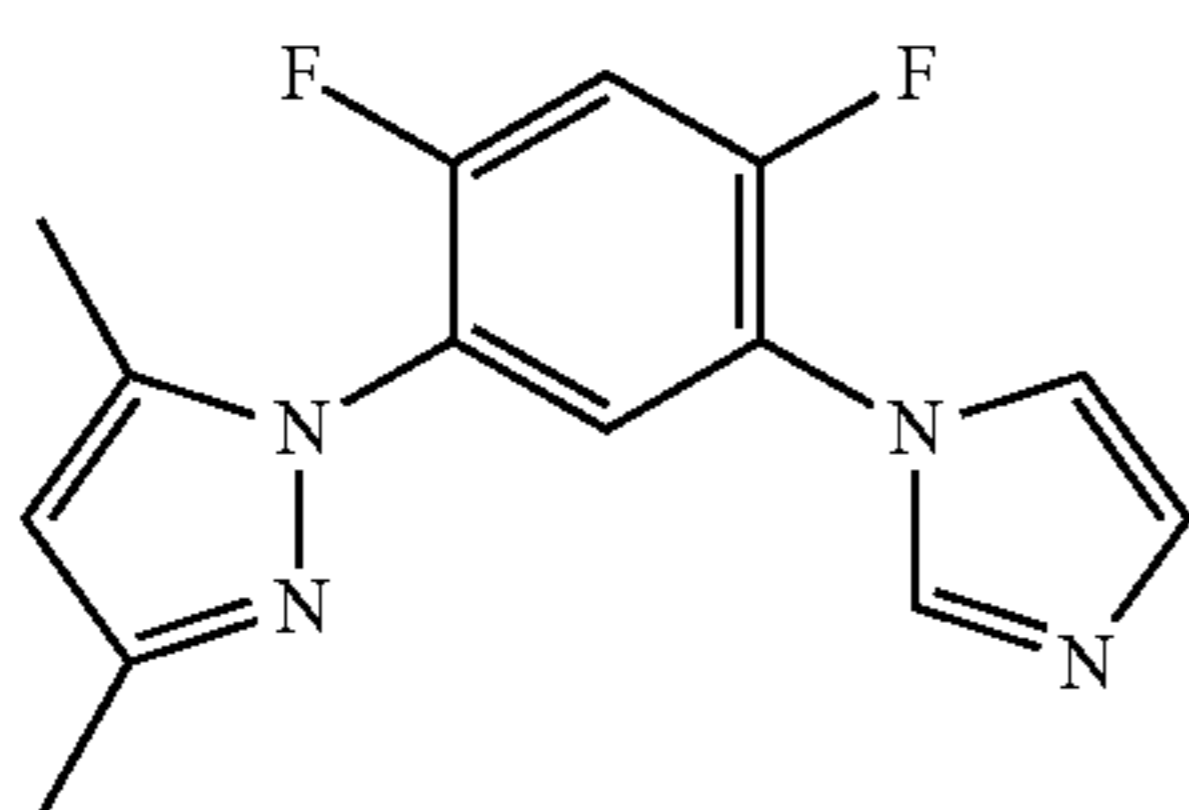
DMPz-DFPh-Iz
