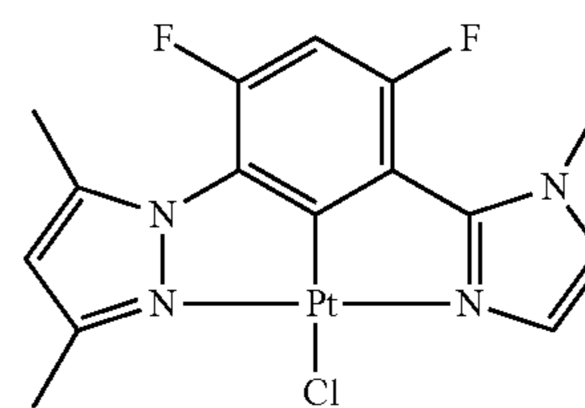
DMPz-DFPh-MIz-PtCl
