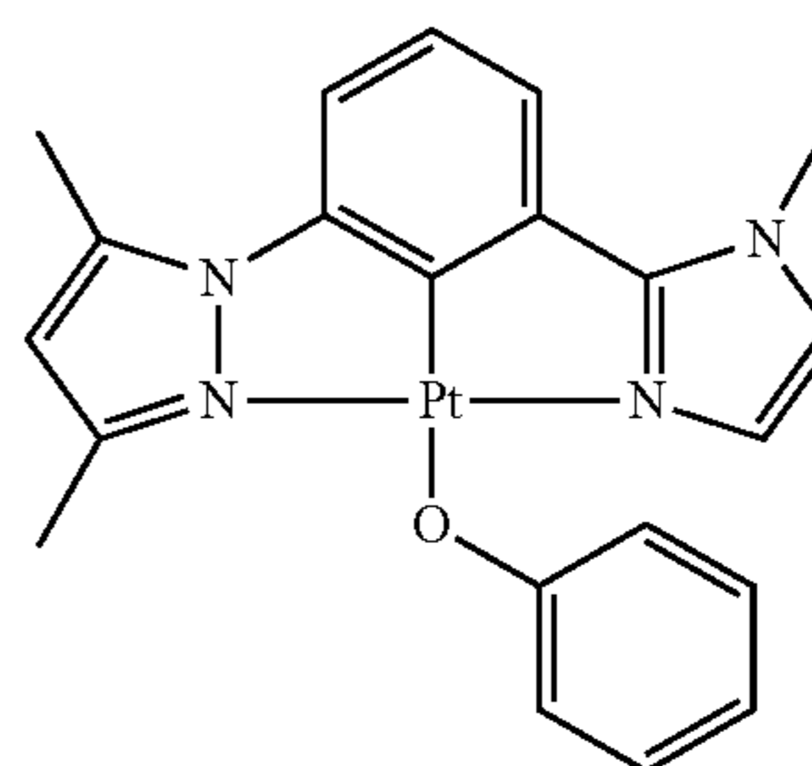
DMPz-Ph-MIz-PtOPh
