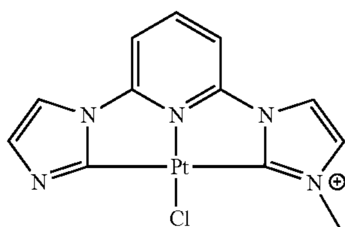
Iz-Py-MIzCb-PtCl
