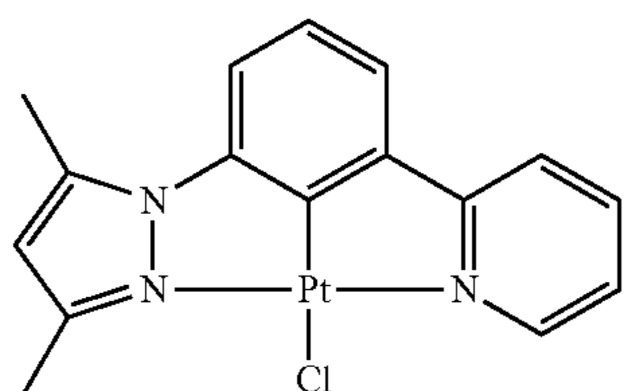
DMPz-Ph-Py-PtCl
