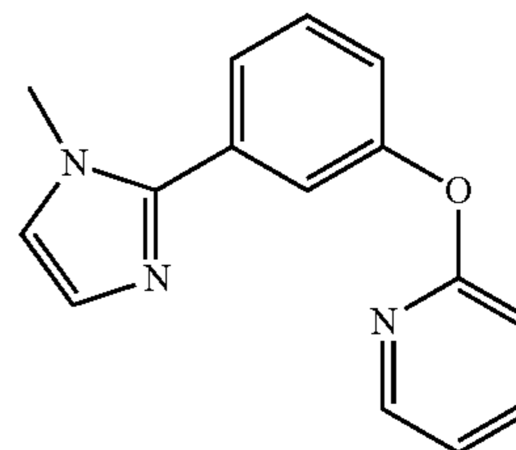
MIz-Ph-O-Py
