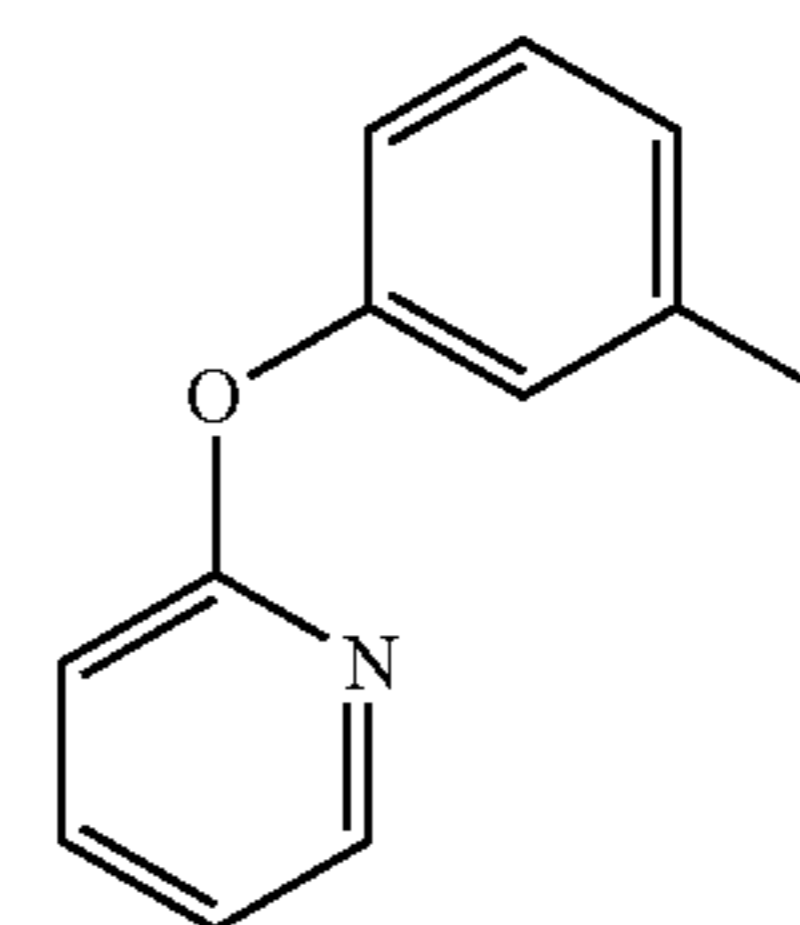
Py-O-Ph-I
