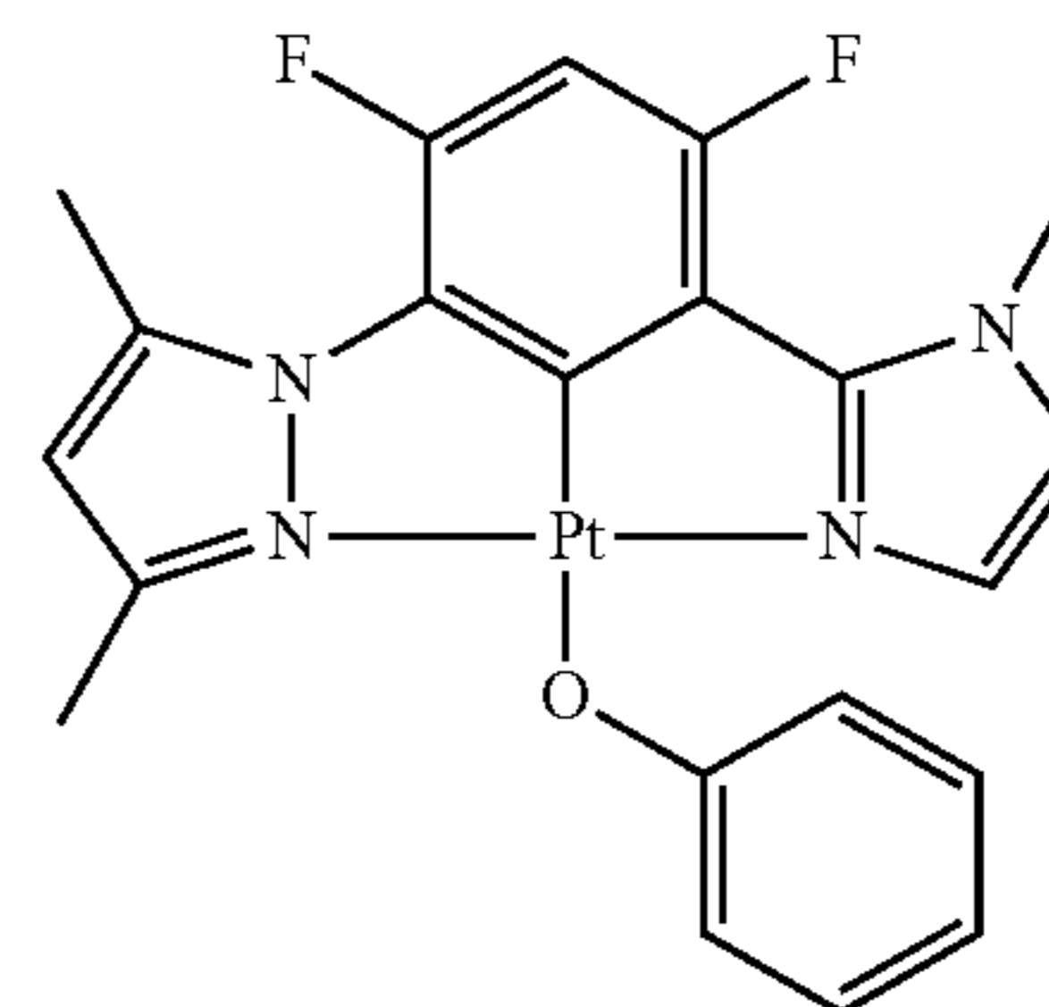
DMPz-DFPh-MIz-PtOPh
