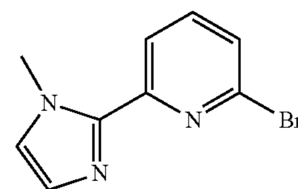
MIz-Py-Br
