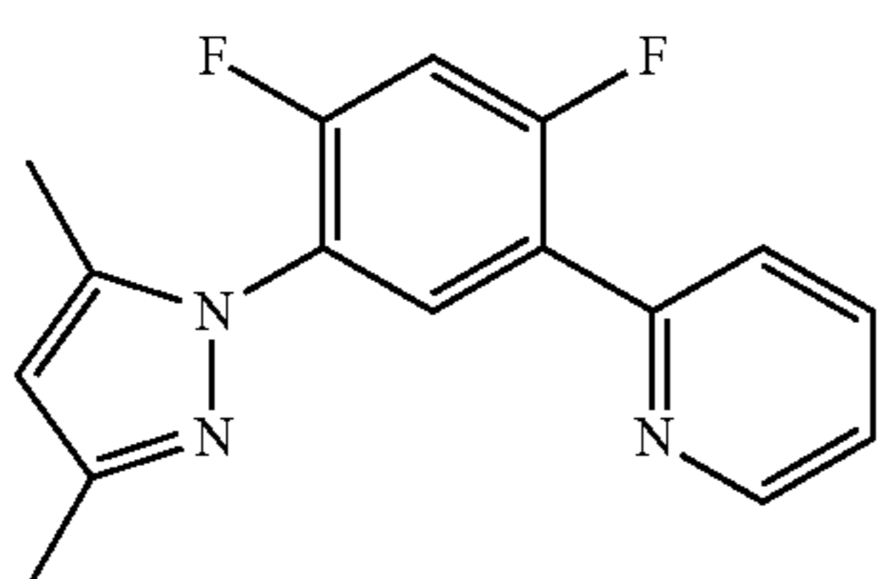
DMPz-DFPh-Py
