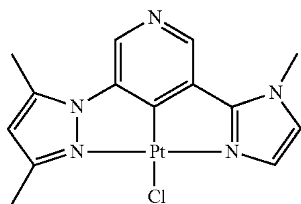
DMPz-Ph-MIz-PtCl
