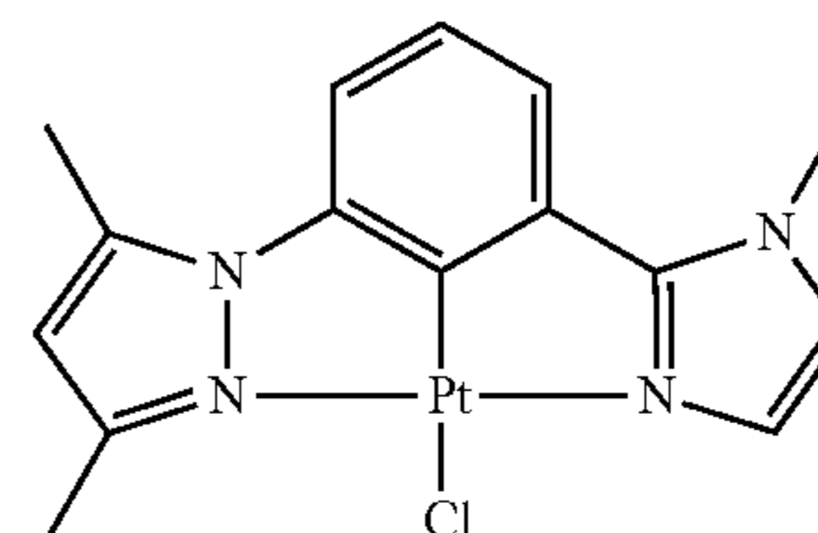
DMPz-Ph-MIz-PtCl
