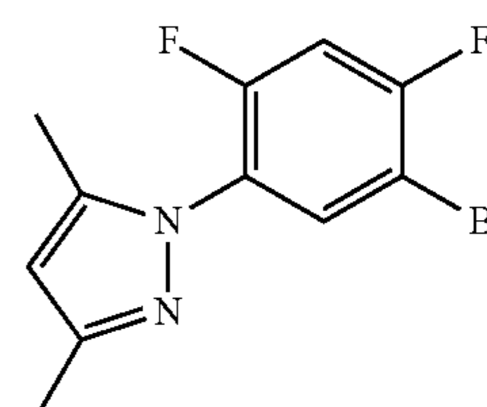
DMPz-DFPh-Br
