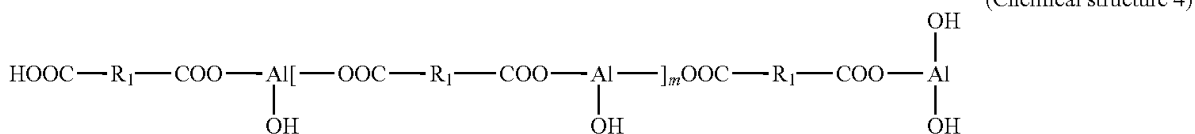
(Chemical structure 4)
