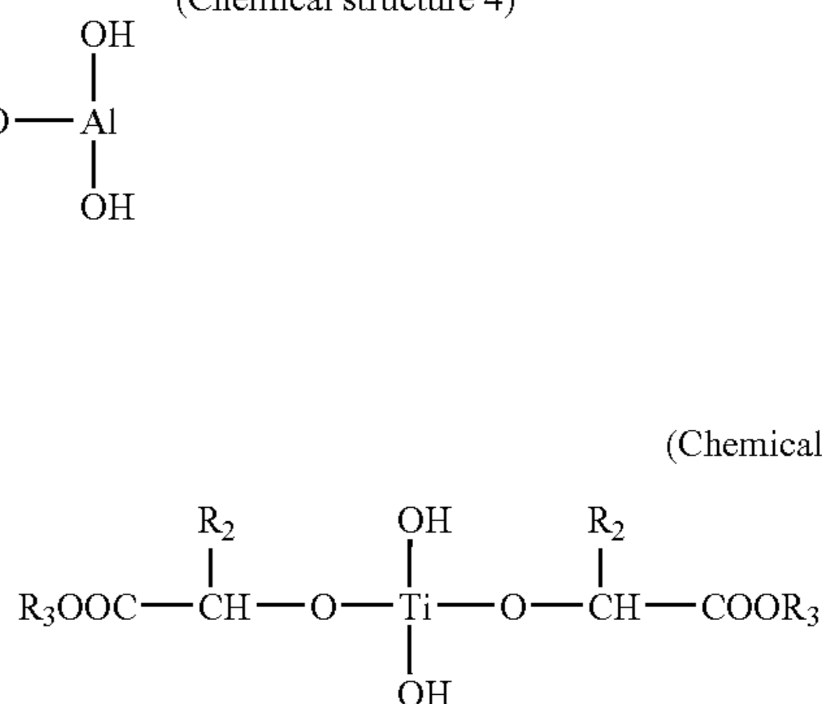
(Chemical structure 4)
