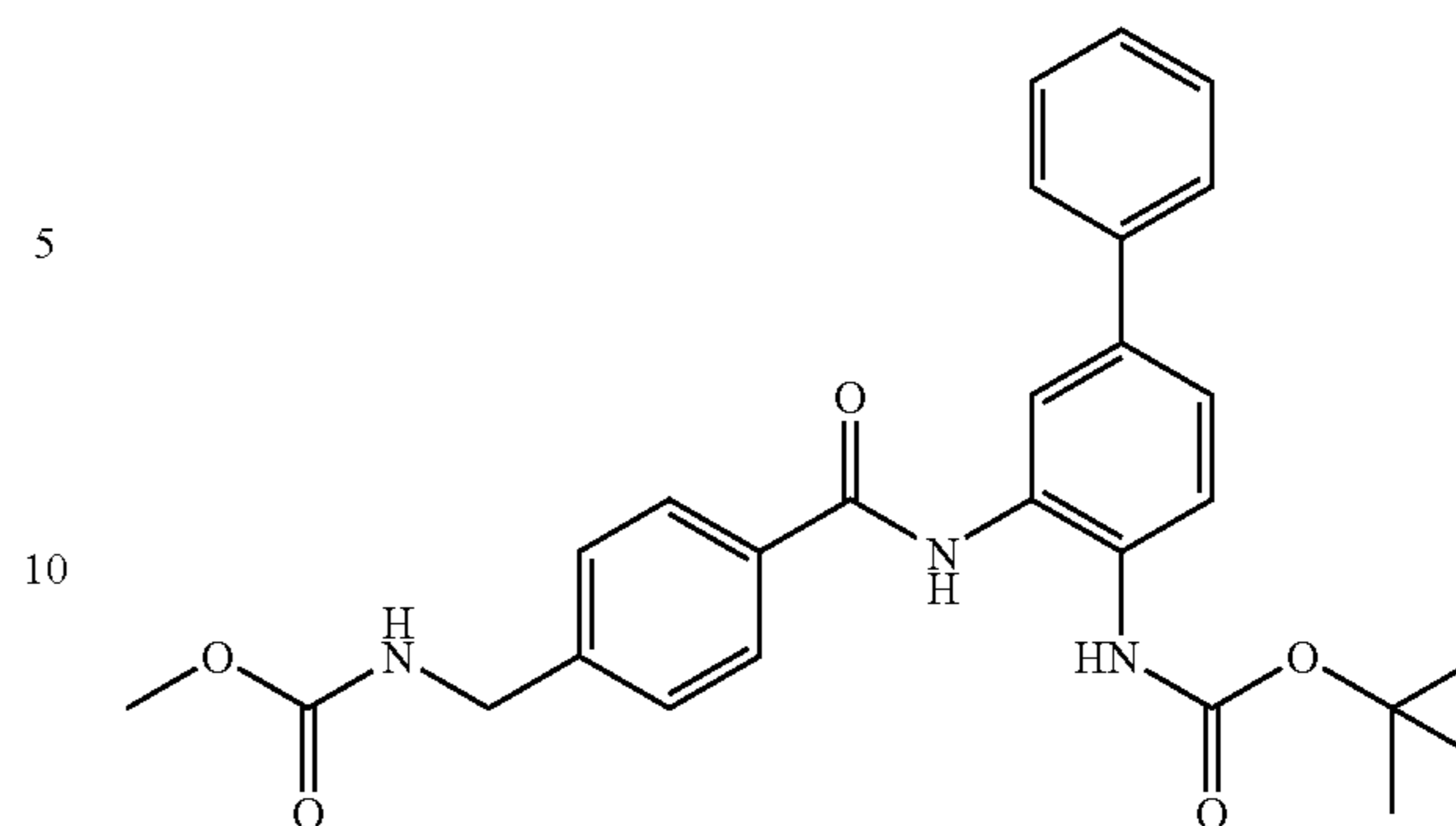
1,1-dimethylethyl[3-({[4-({[(methoxy)carbonyl]amino}methyl)phenyl]carbonyl}amino)biphenyl-4-yl]carbamate
