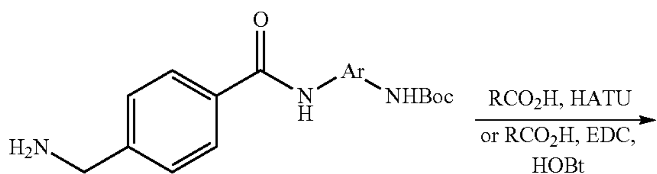
Scheme 3
