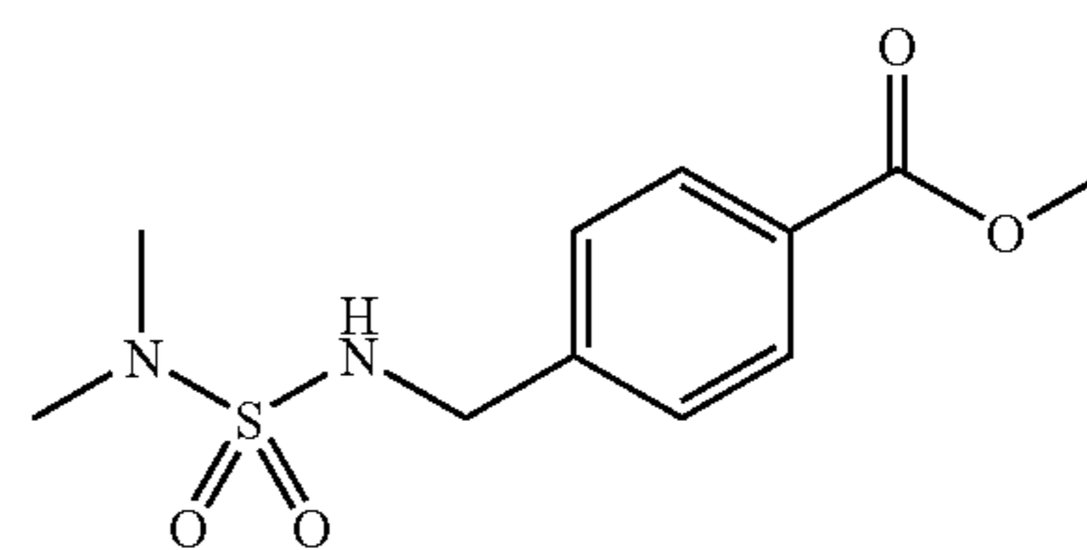
Methyl 4-(((dimethylamino)sulfonyl)amino)methylbenzoate
