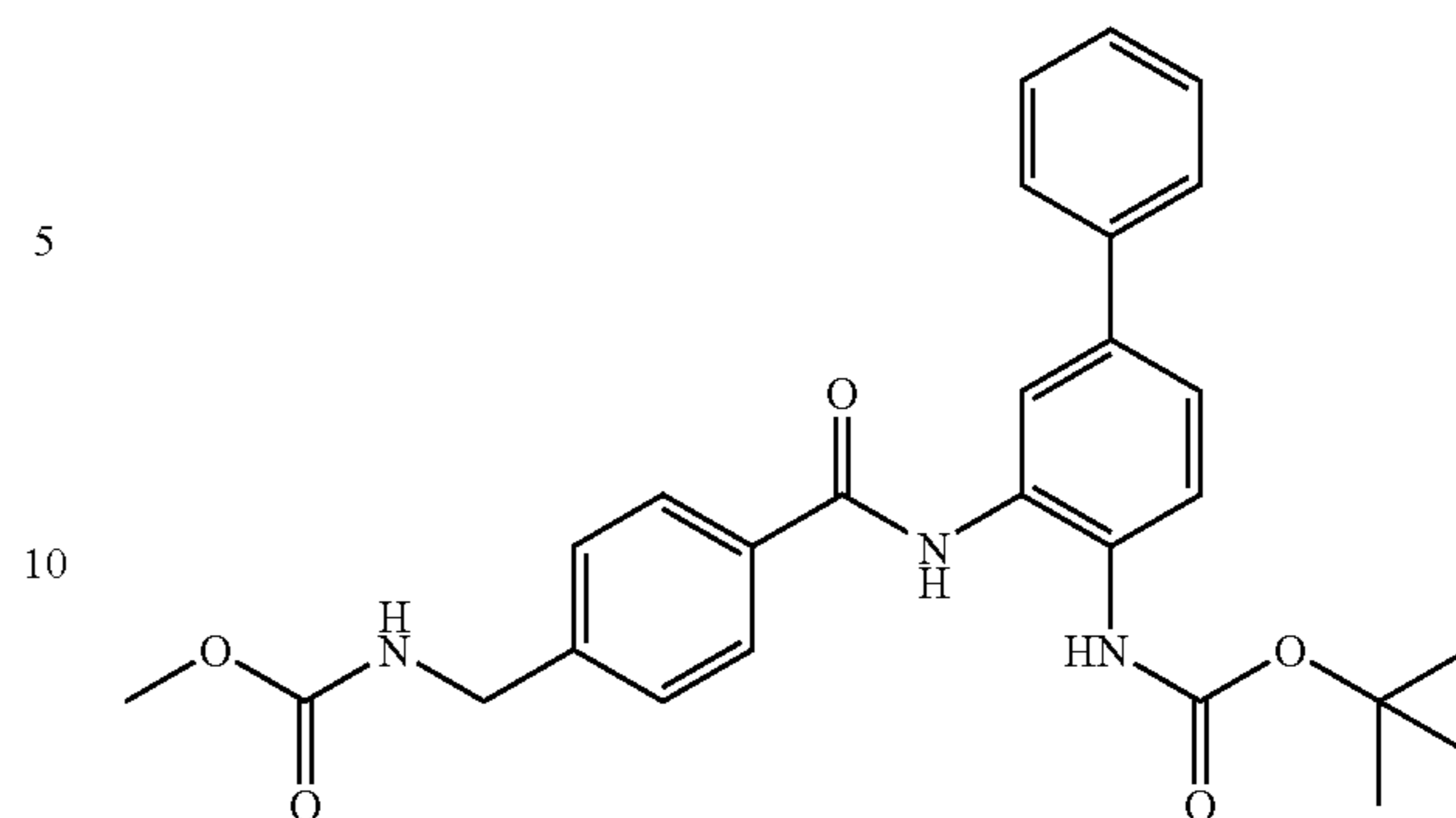
1,1-dimethylethyl[3-({[4-({[(methoxy)carbonyl]amino}methyl)phenyl]carbonyl}amino)biphenyl-4-yl]carbamate
