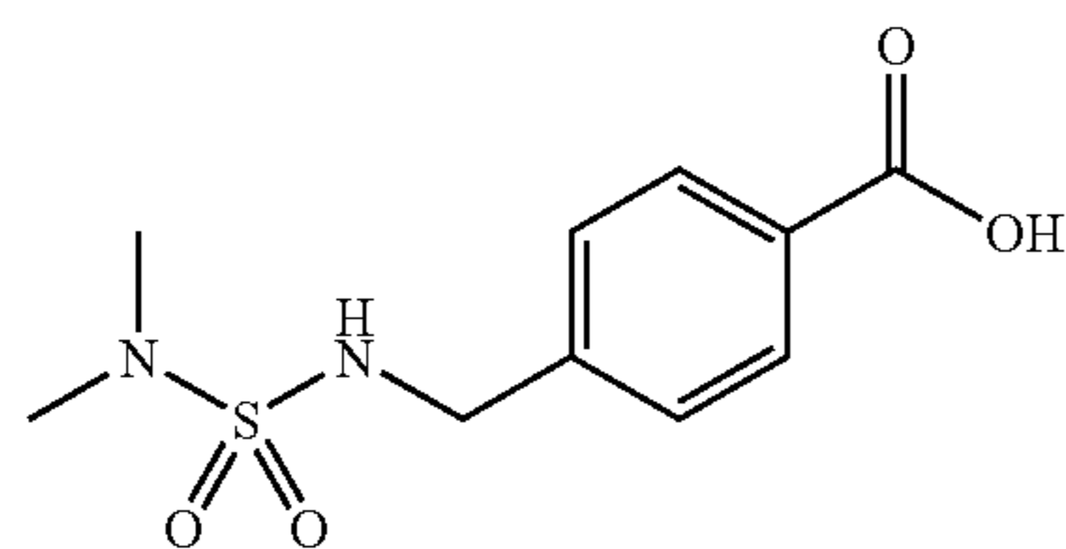
4-((dimethylamino)sulfonyl)aminomethylbenzoic acid
