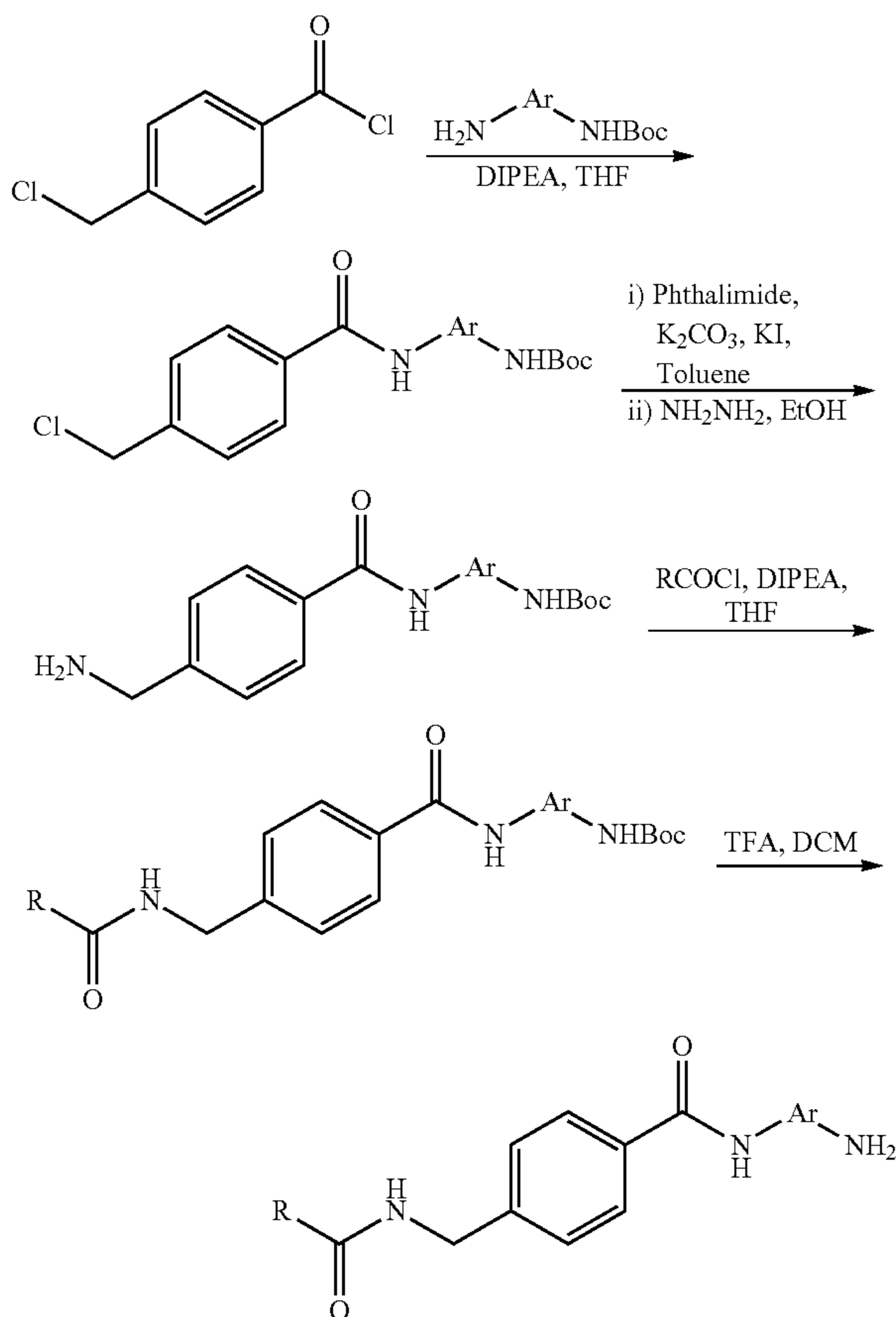
Scheme 2
