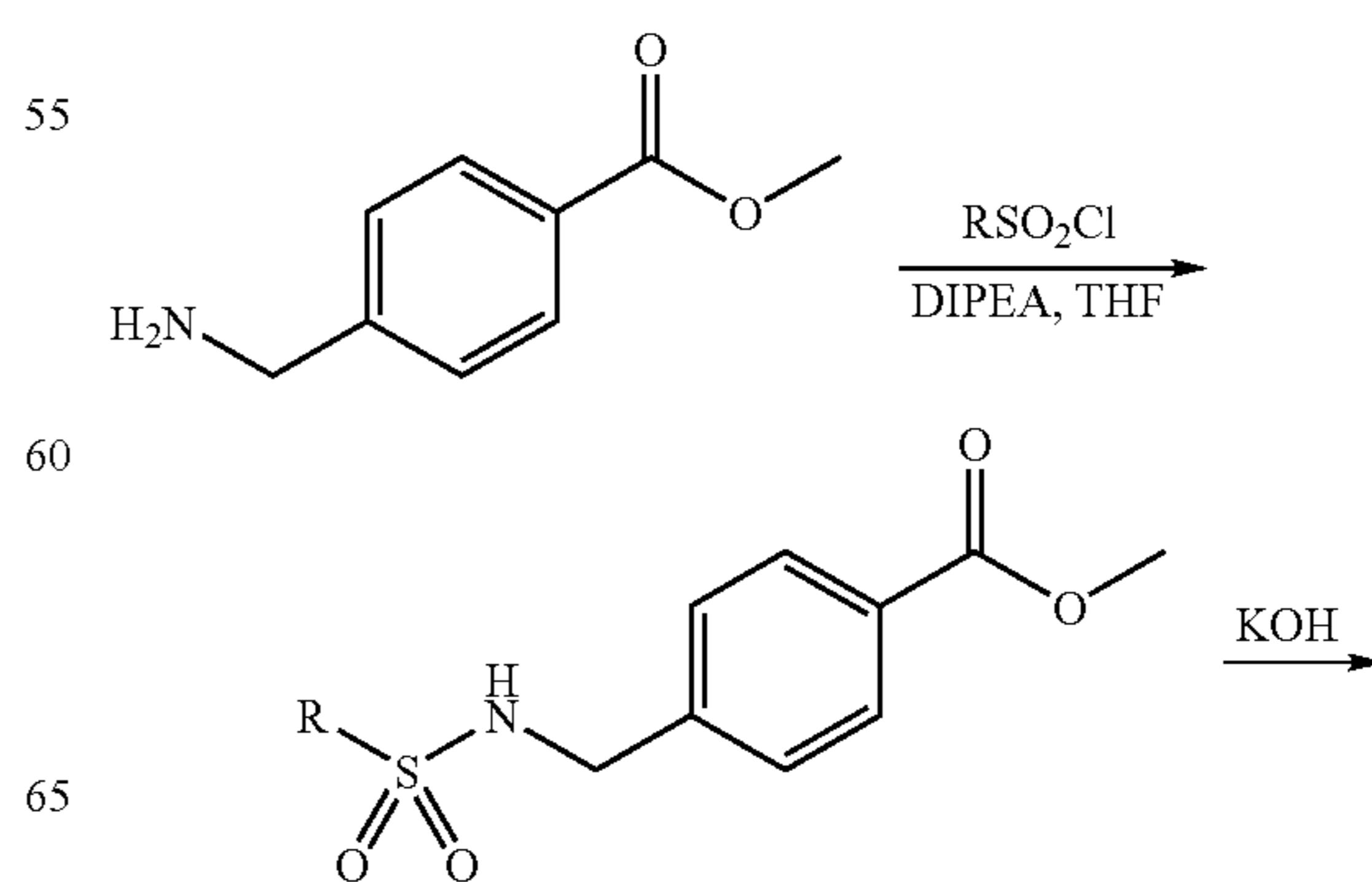
Scheme 5
