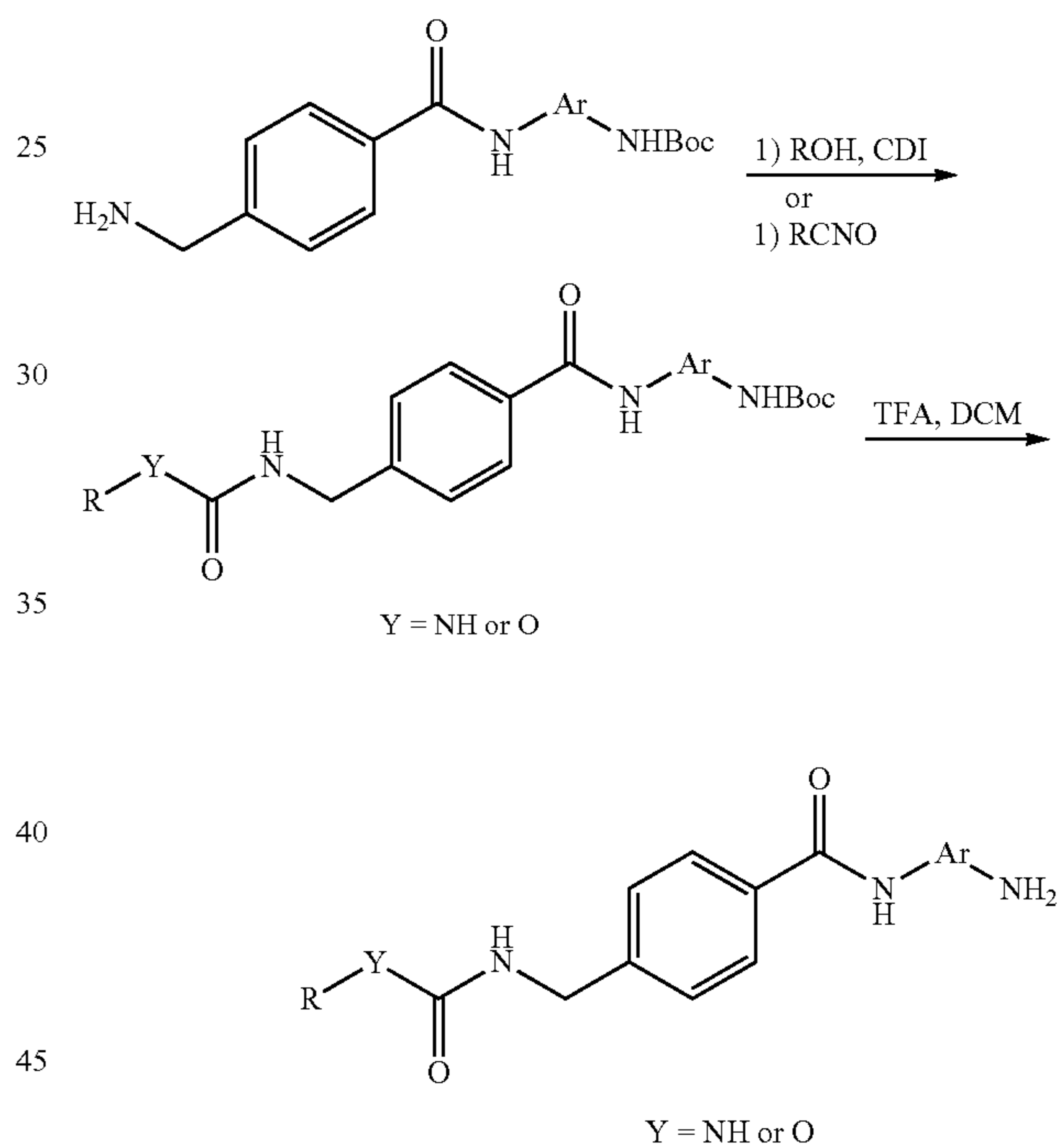
Scheme 4
