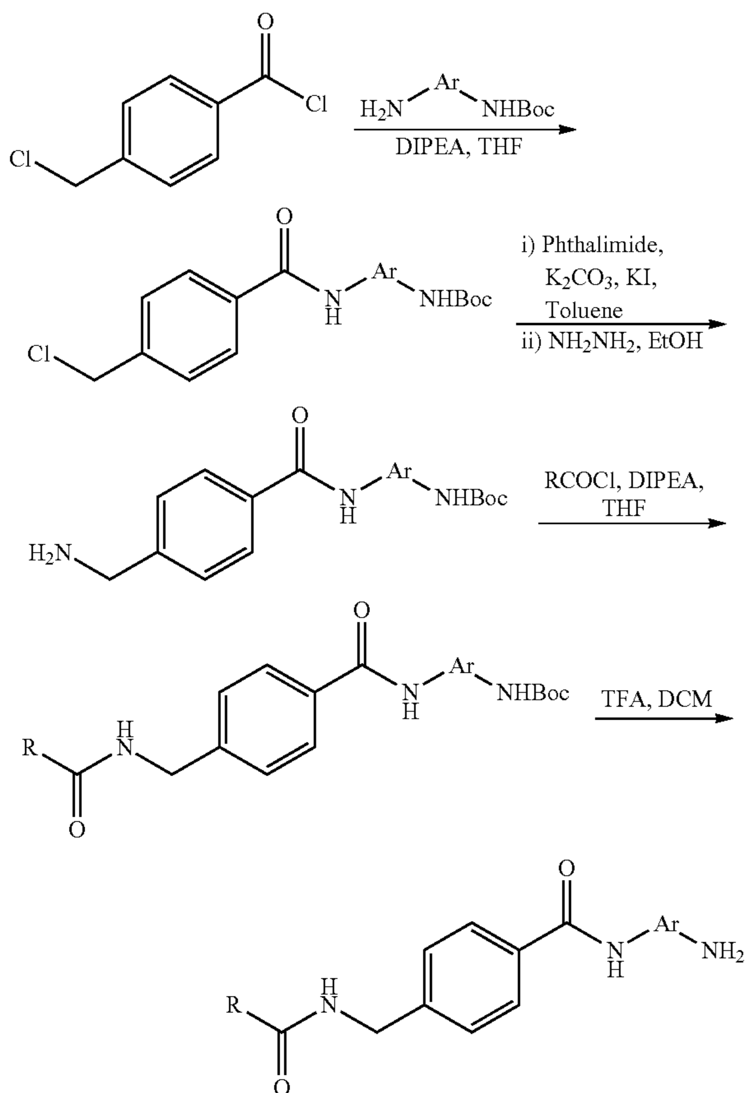
Scheme 2
