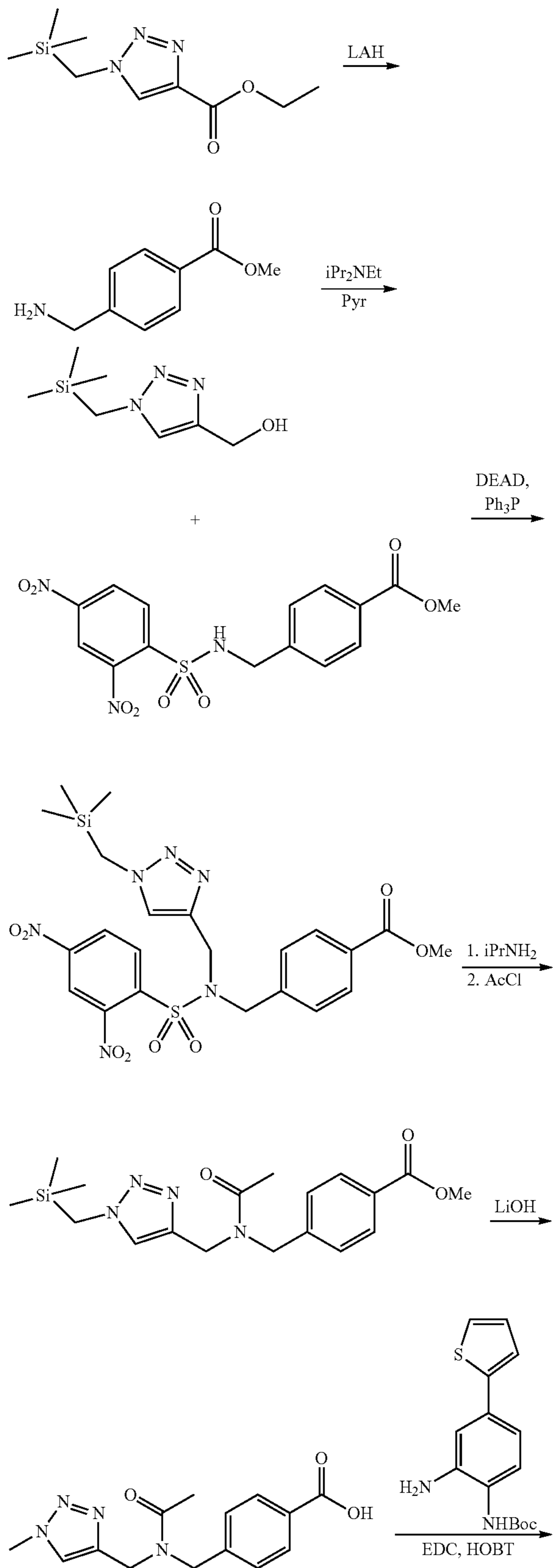
Scheme 9
