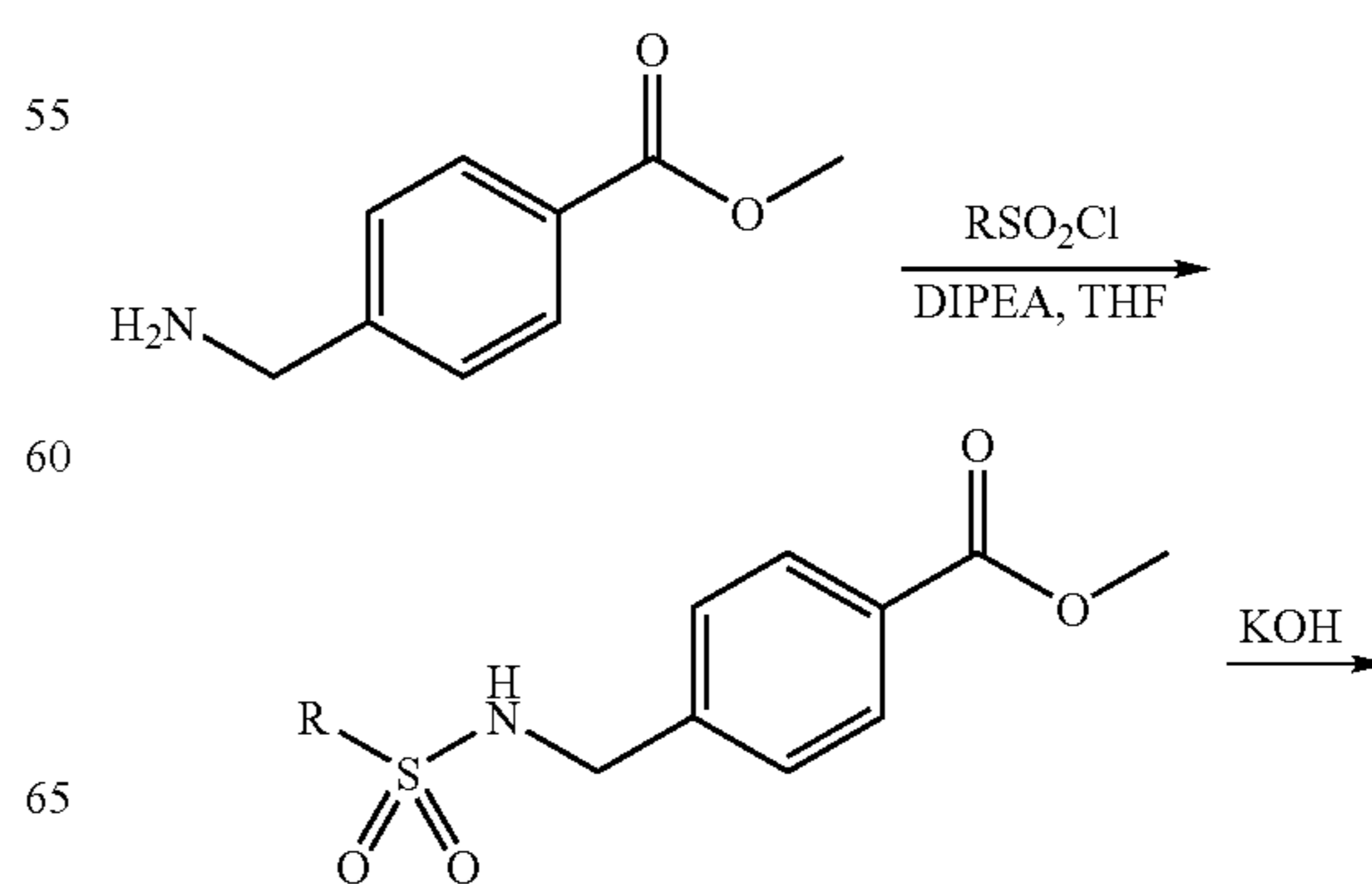
Scheme 5
