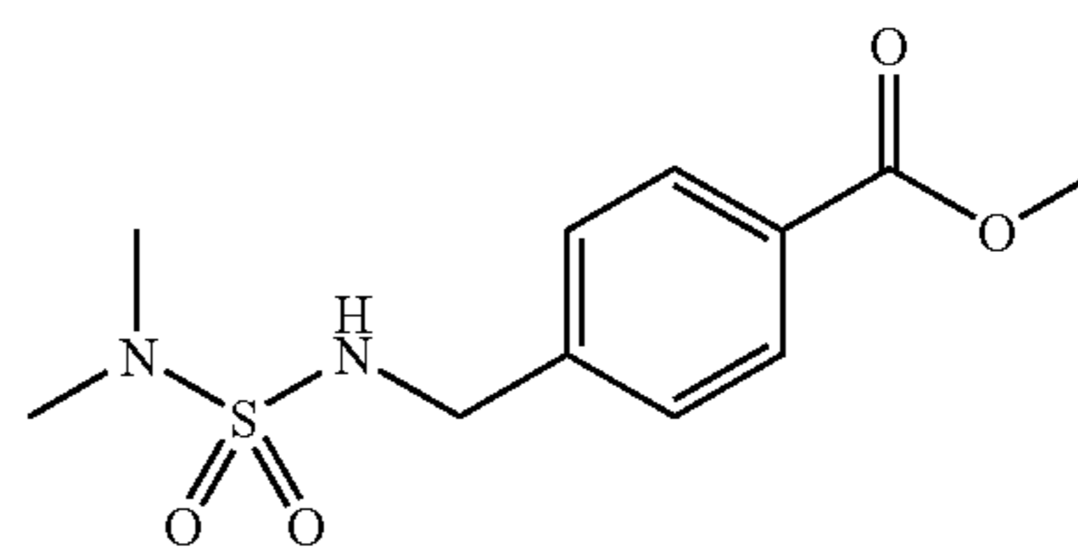
Methyl 4-(((dimethylamino)sulfonyl)amino)methylbenzoate
