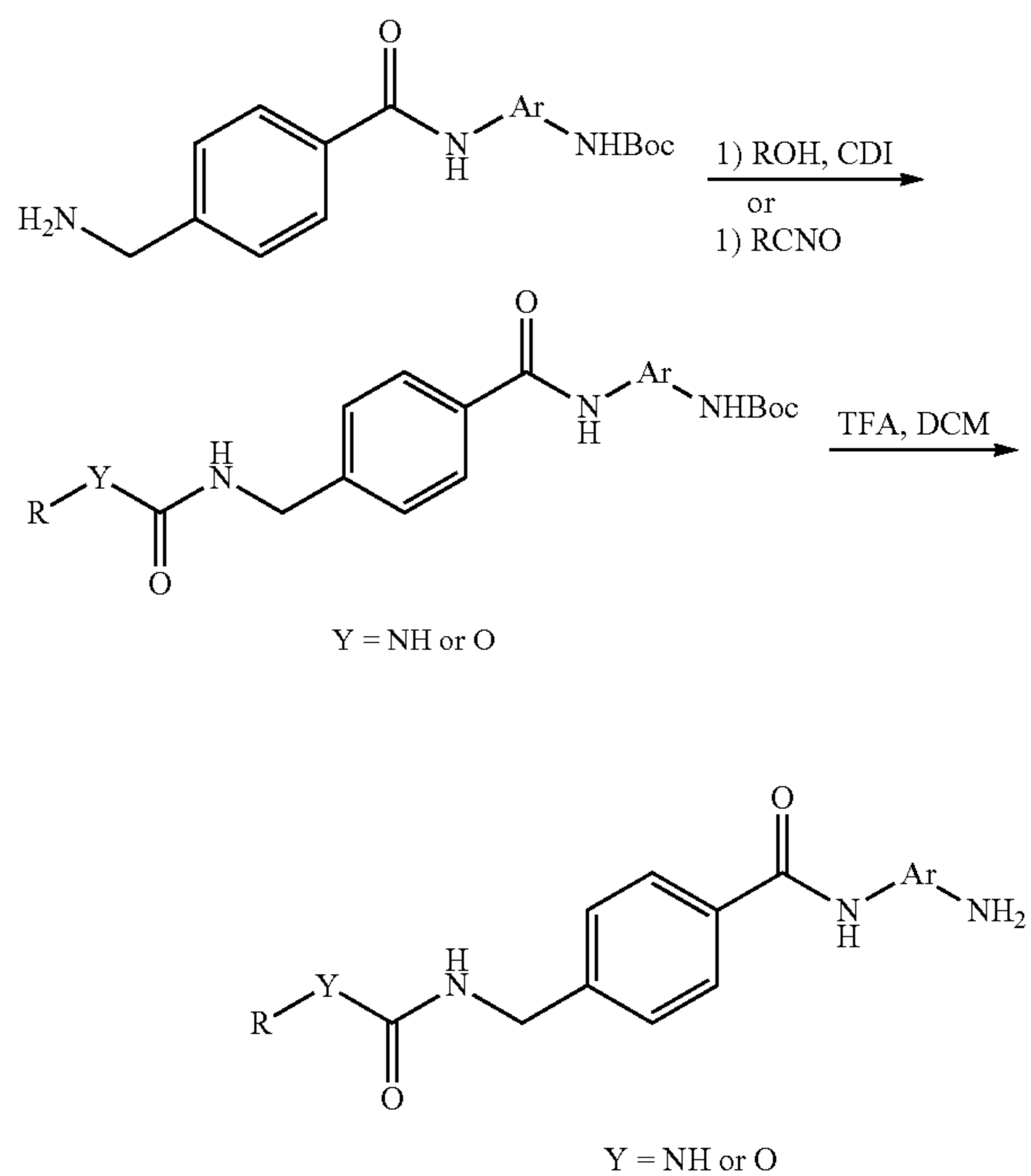
Scheme 4
