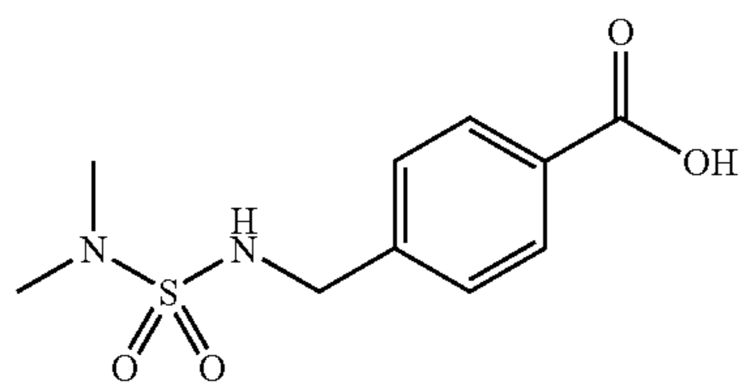
4-((dimethylamino)sulfonyl)aminomethylbenzoic acid
