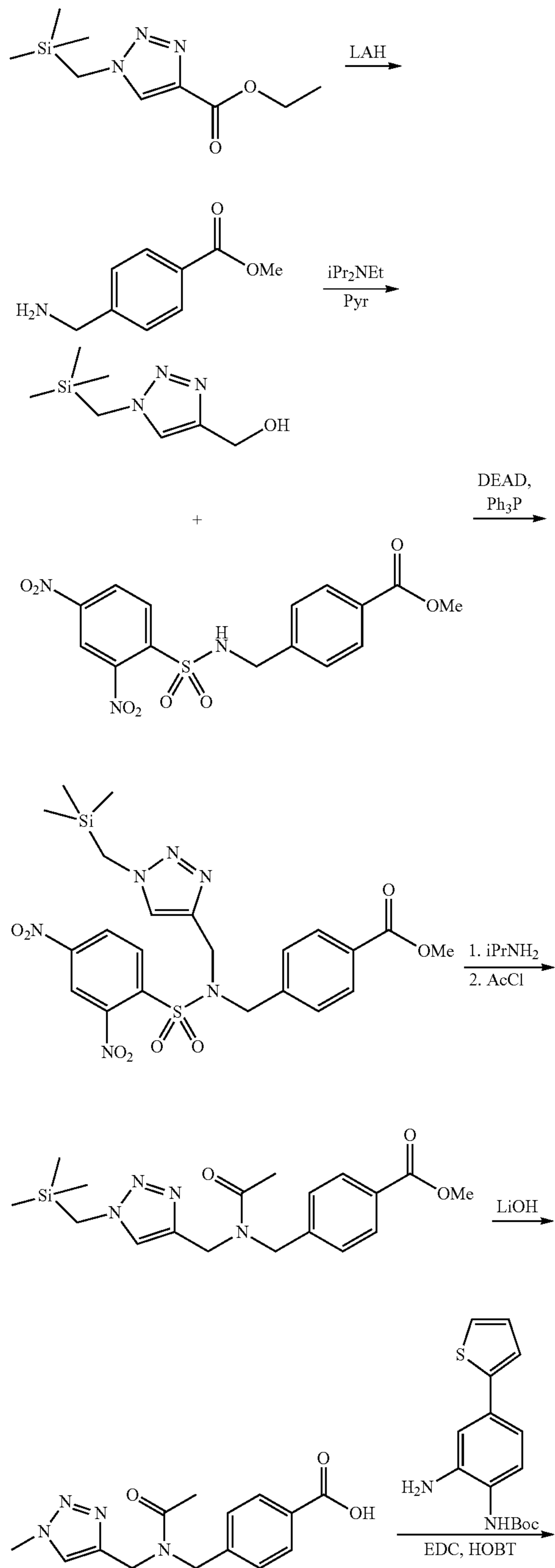
Scheme 9
