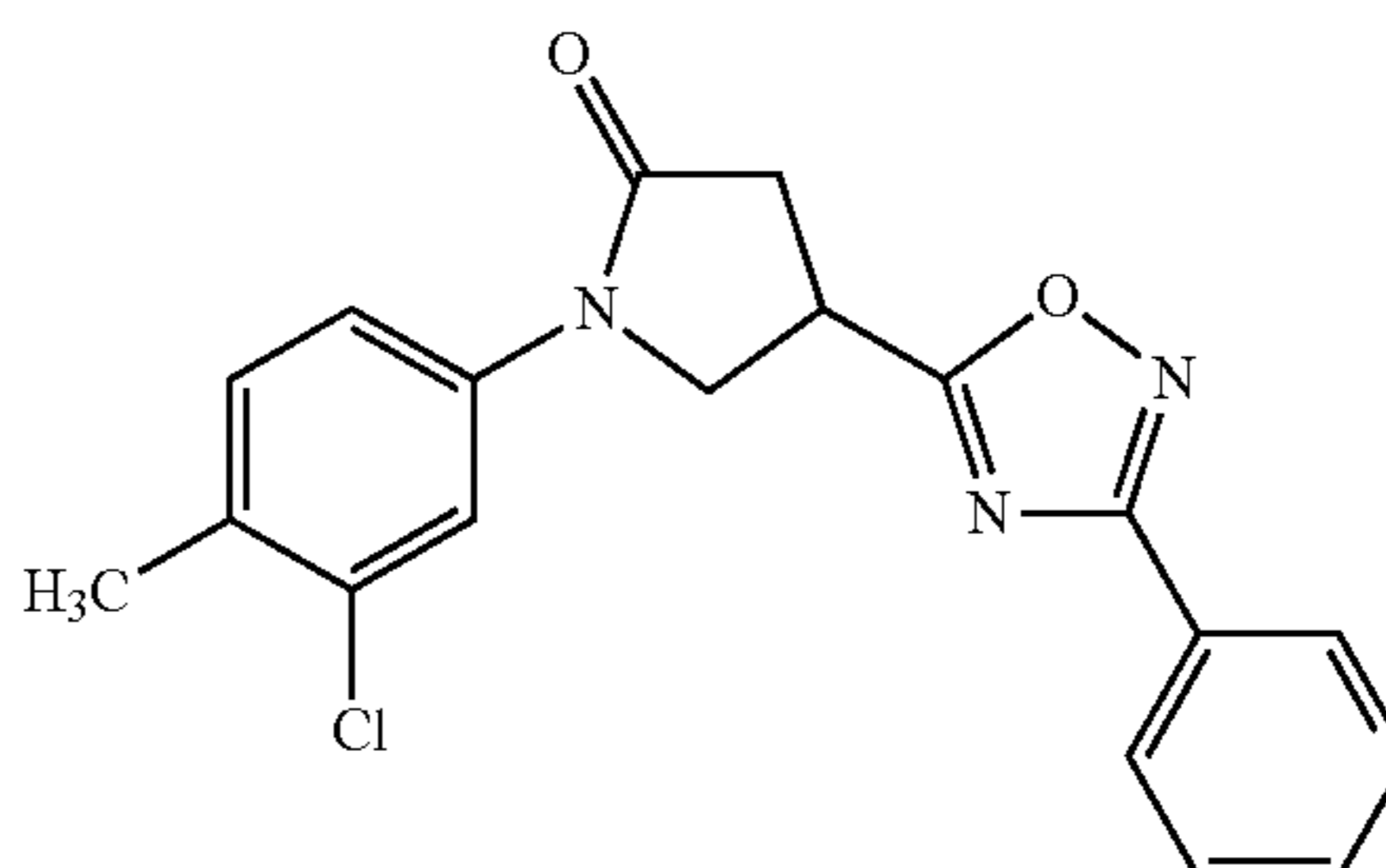
Compound Alda-69: 1-(3-chloro-4-methyl-phenyl)-4-(3-pyridin-3-yl-[1,2,4]oxadiazol-5-yl)-pyrrolidin-2-one.
