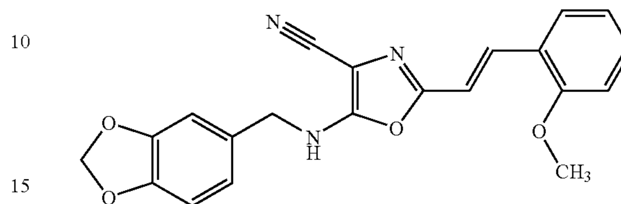
Compound Alda-58: 5-[(benzo[1,3]dioxol-5-ylmethyl)amino]-2-[2-(2-methoxy-phenyl)-vinyl]-oxazole-4-carbonitrile.
