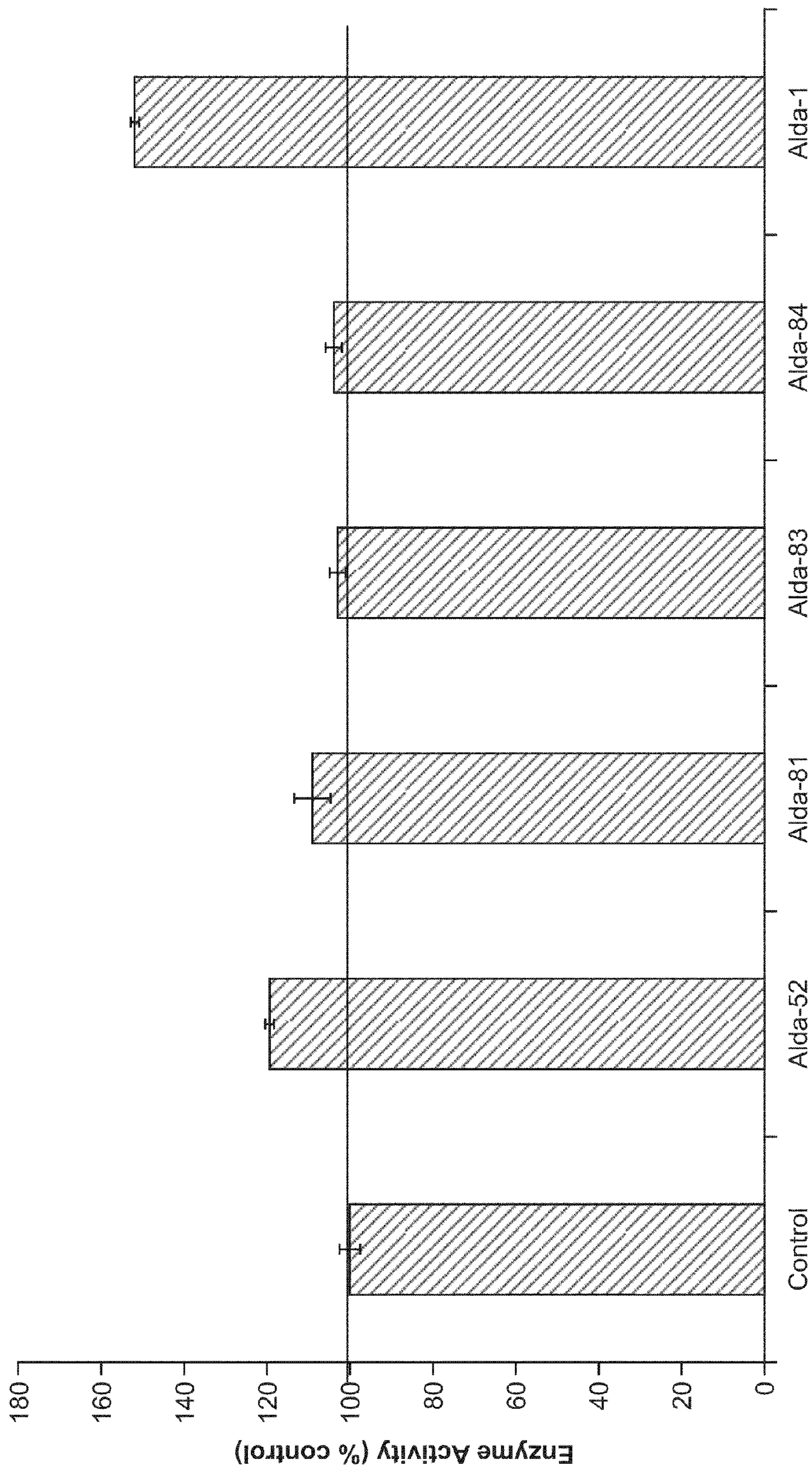
Alda-52, Alda-81, Alda-1 activate ALDH2 using acetaldehyde as a substrate
