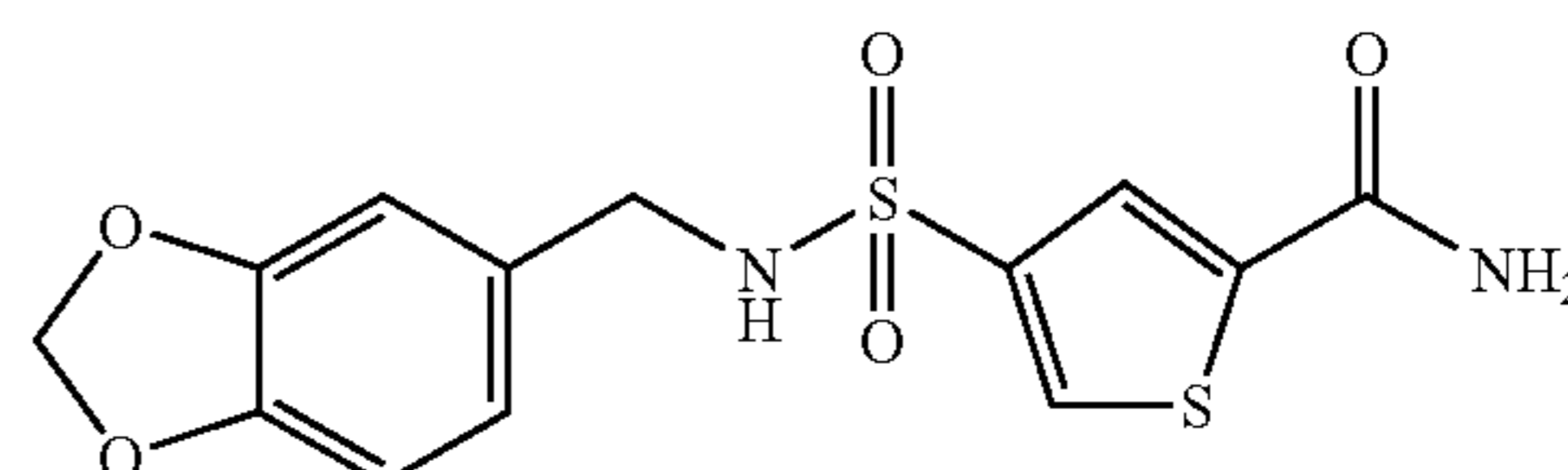
Compound Alda-59: 4-[(benzo[1,3]dioxol-5-ylmethyl)-sulfamoyl]-thiophene-2-carboxylic acid amide.
