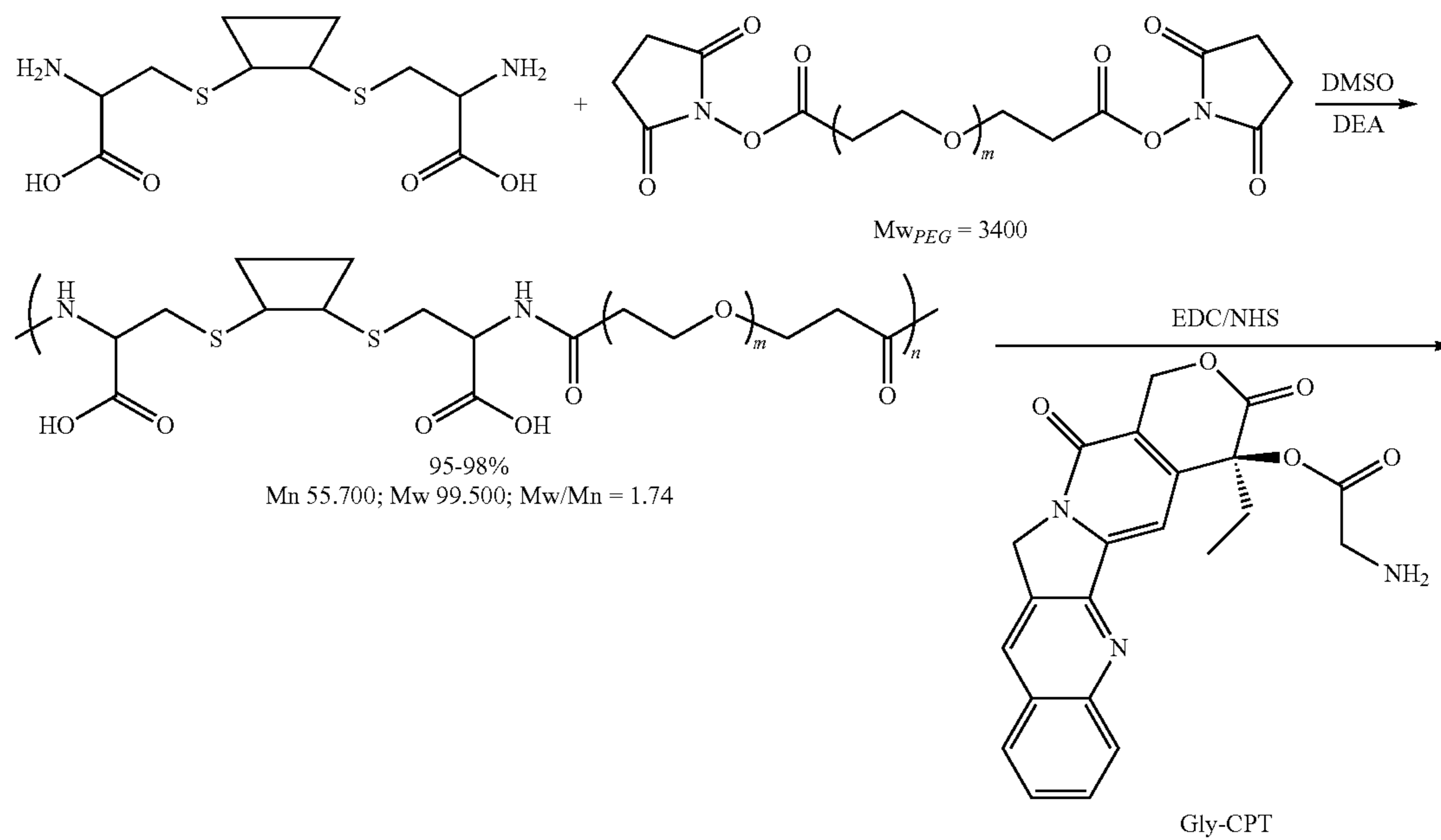
Scheme XIII
