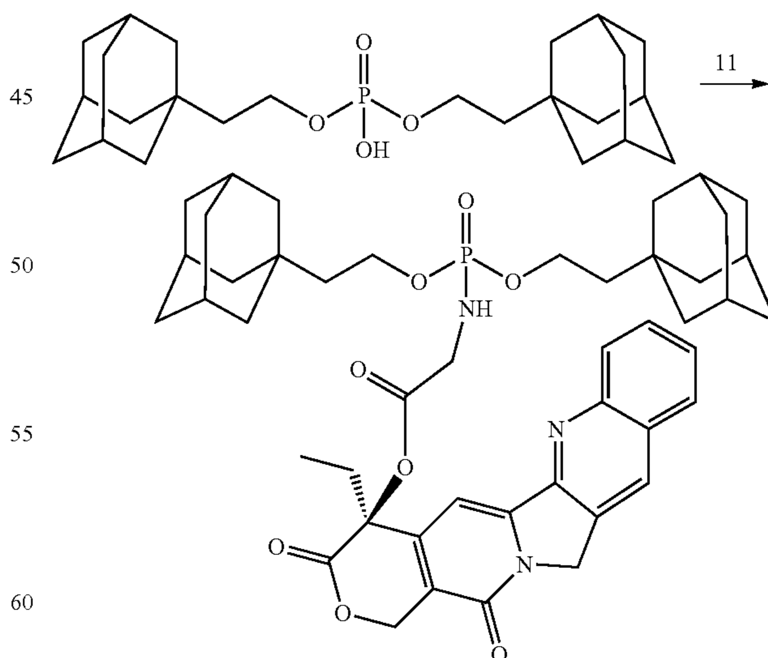
Scheme XXXXVIII
