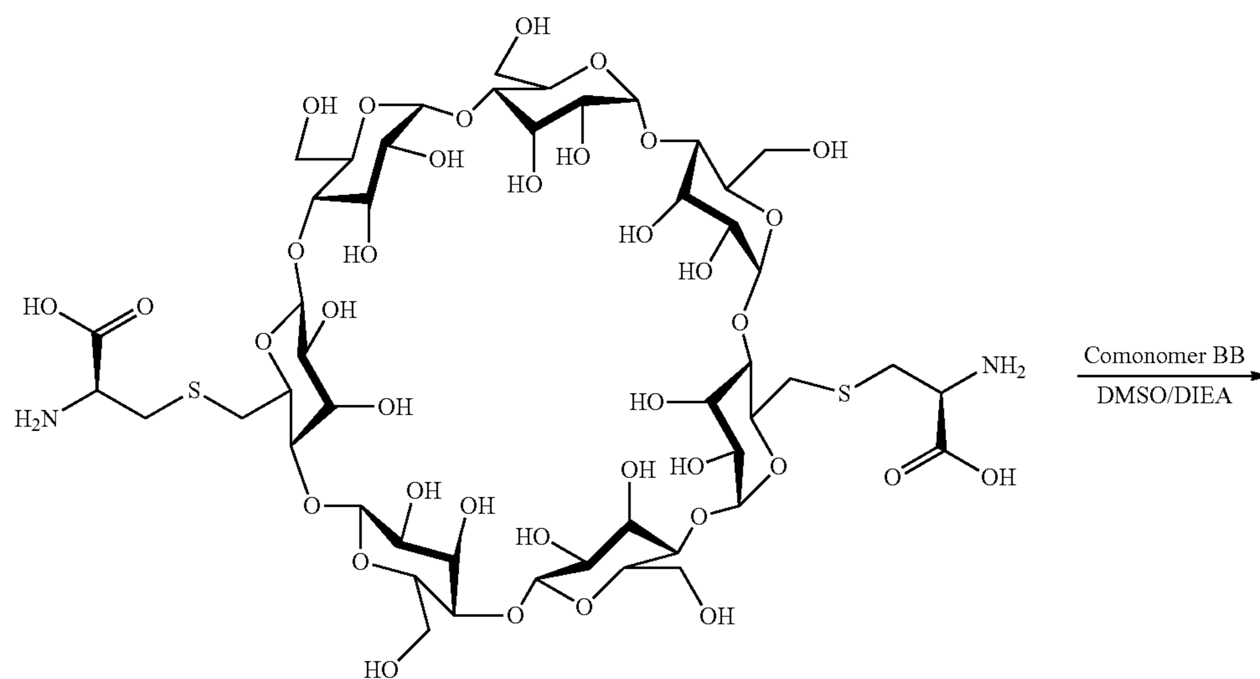
Scheme XXXVIIIb
