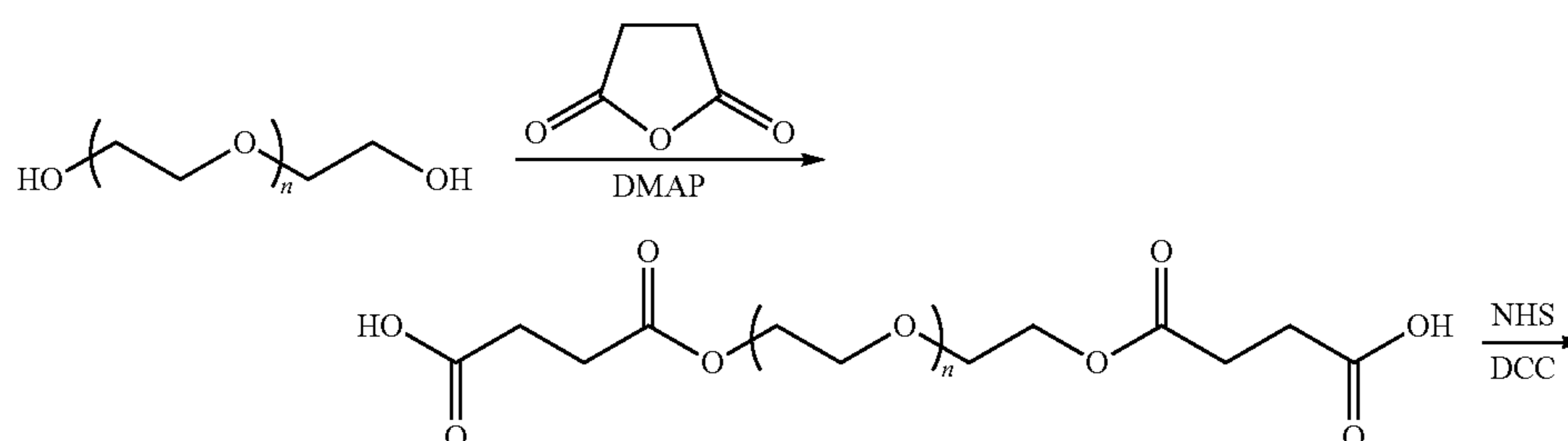
Scheme XIV
