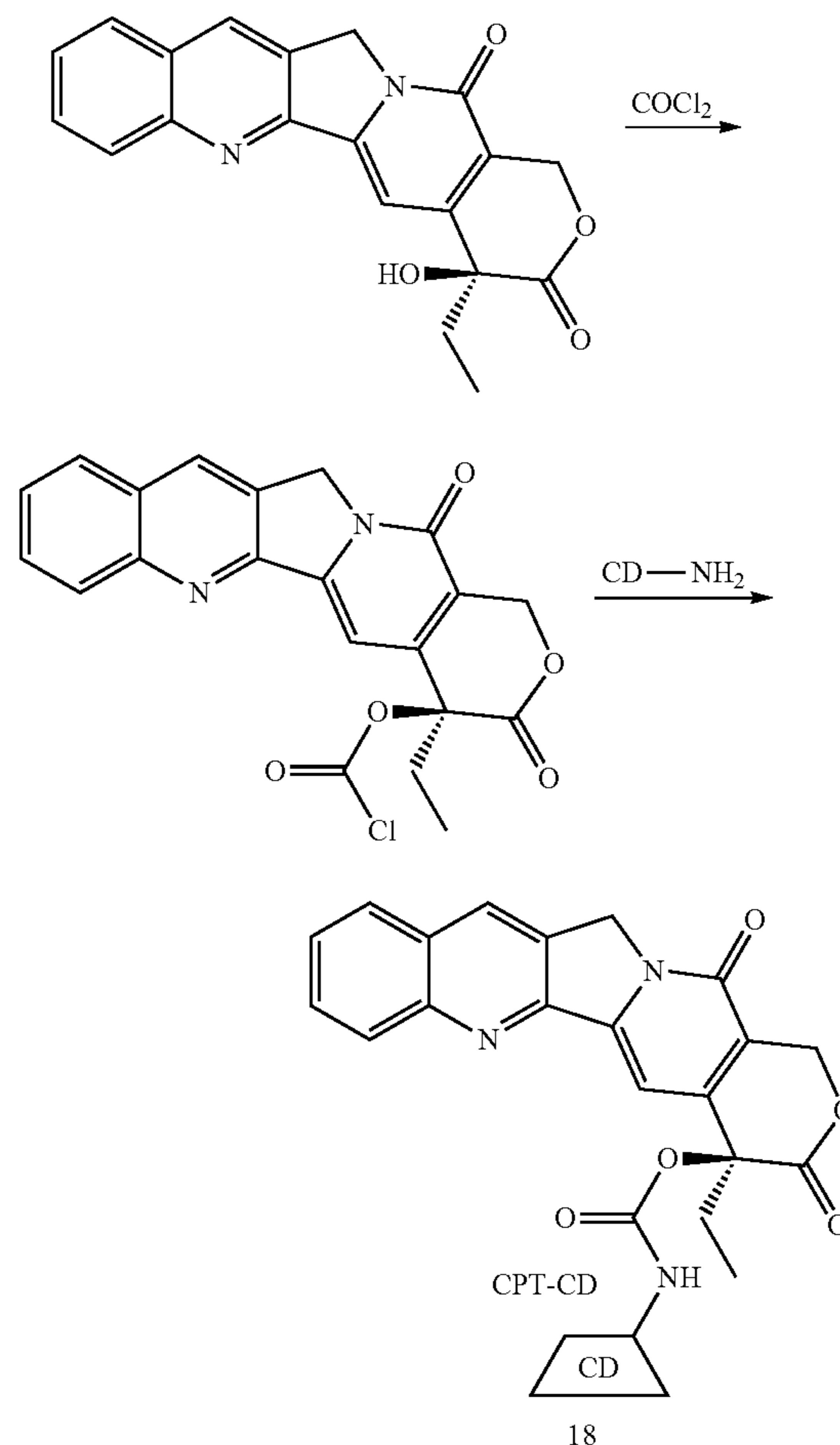
Scheme XXVIII
