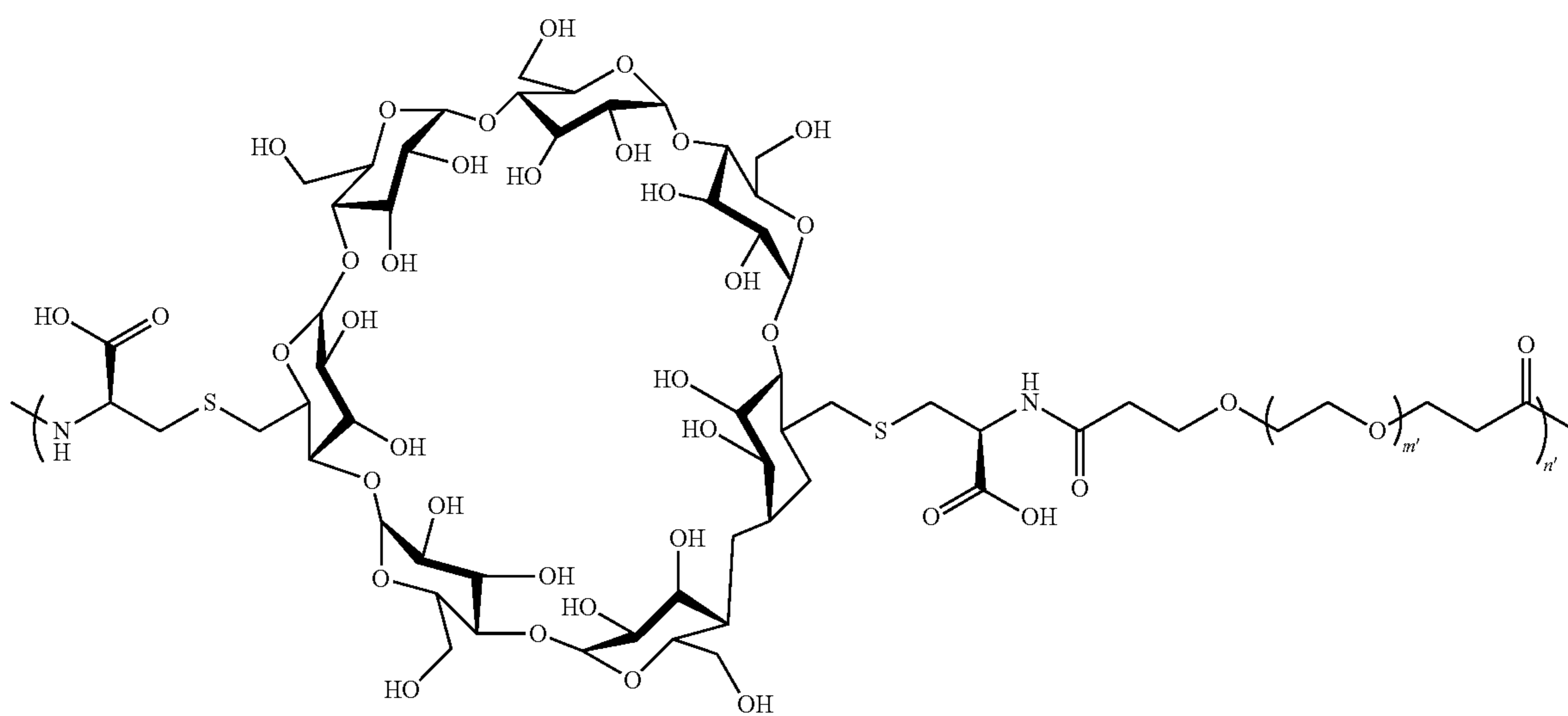
36a-f Poly(CDDCys-PA-PEG) Abbr: PA = propanoicamide bond between PEG and CD
