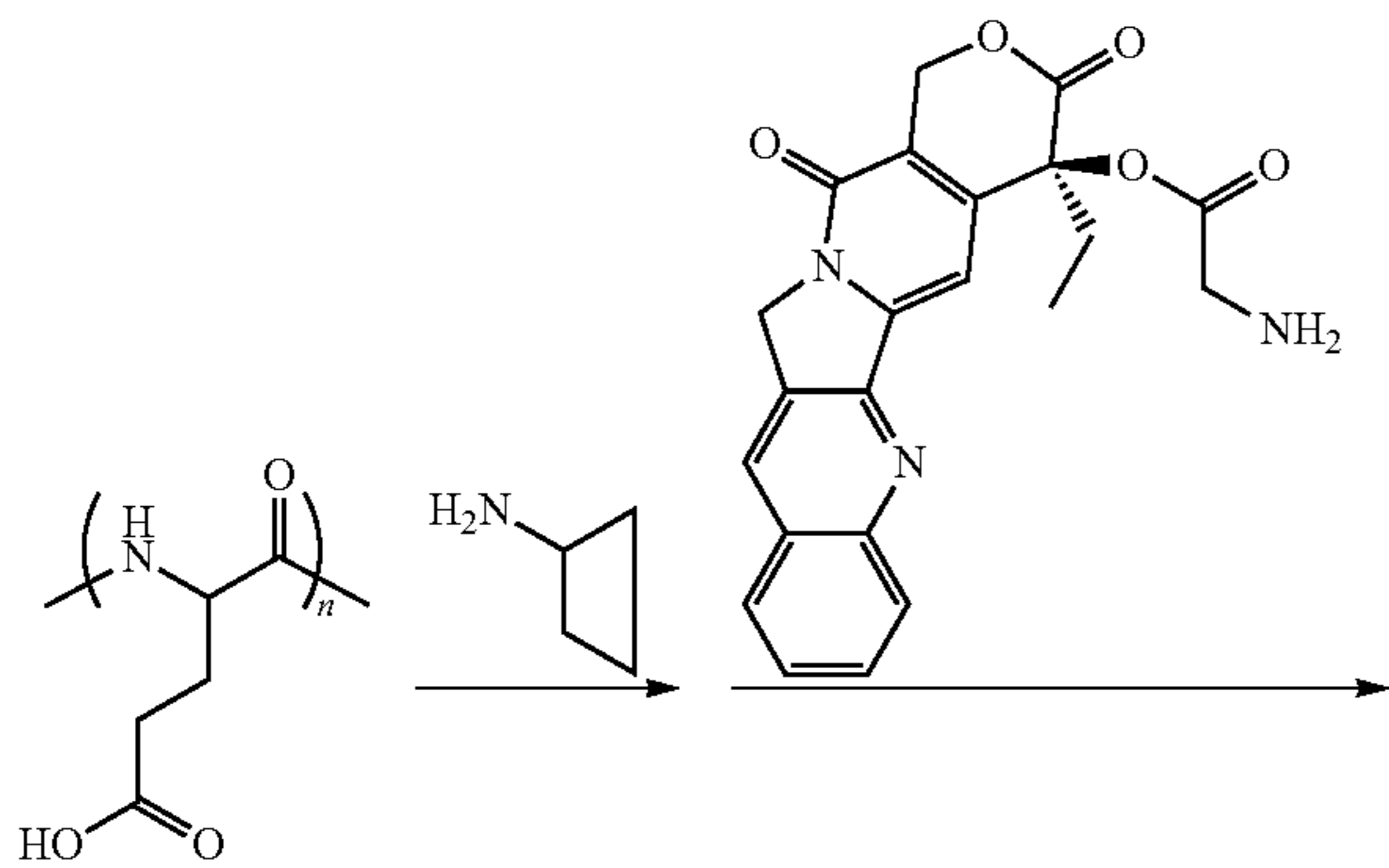
Scheme XXXVII
