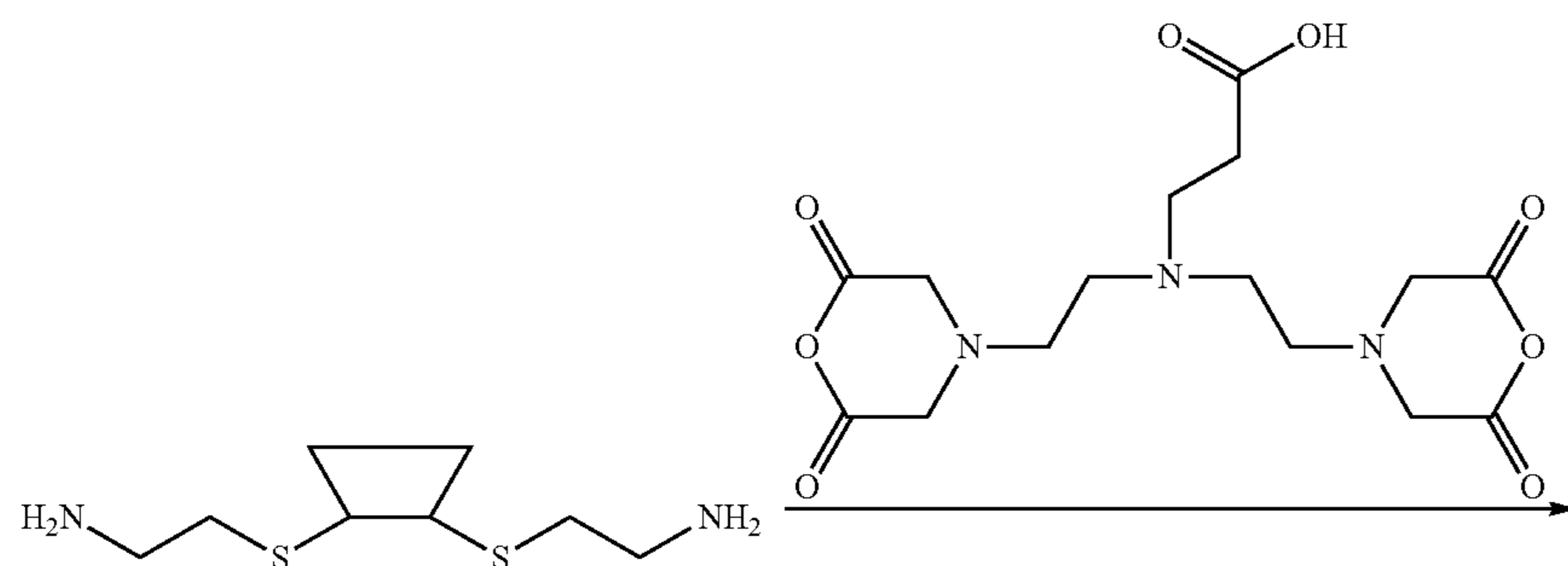
Scheme V
