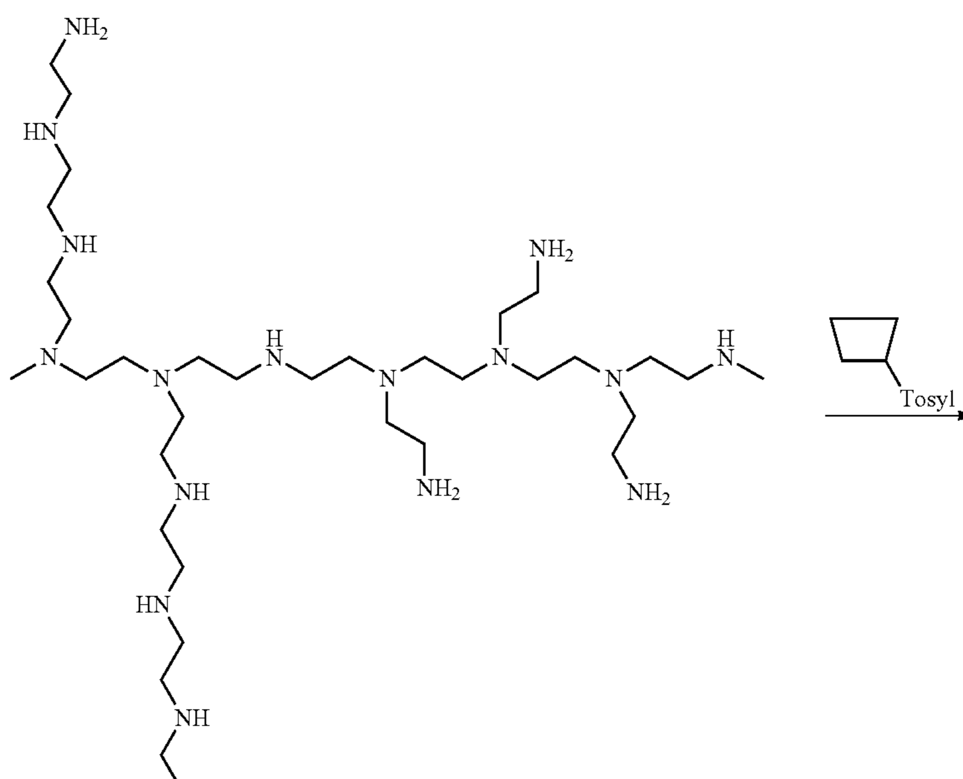
Scheme XXXXIV
