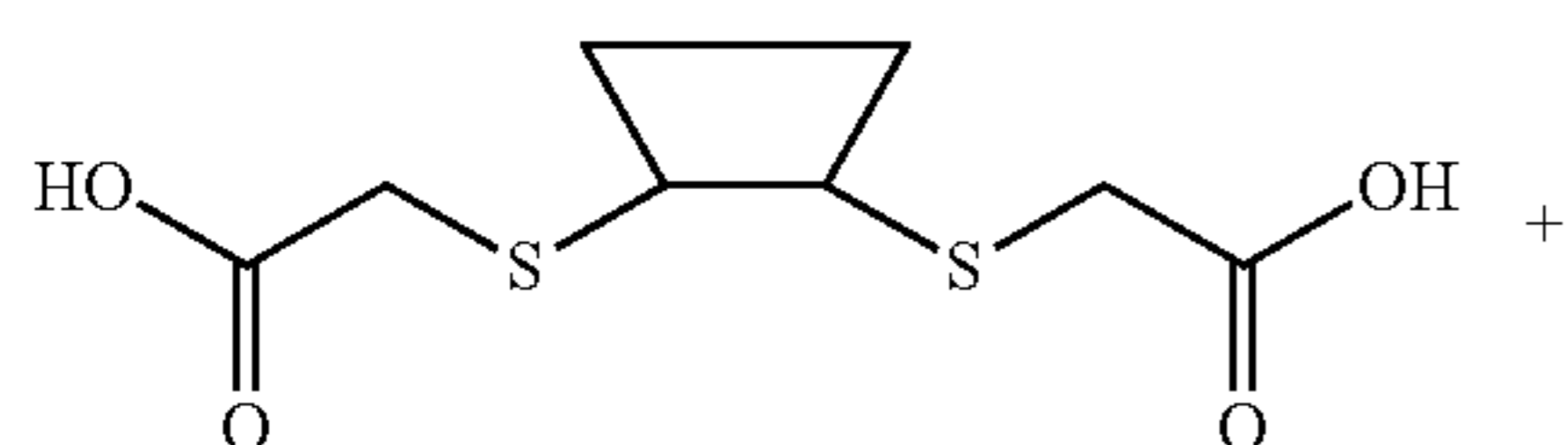
Scheme XXXII
