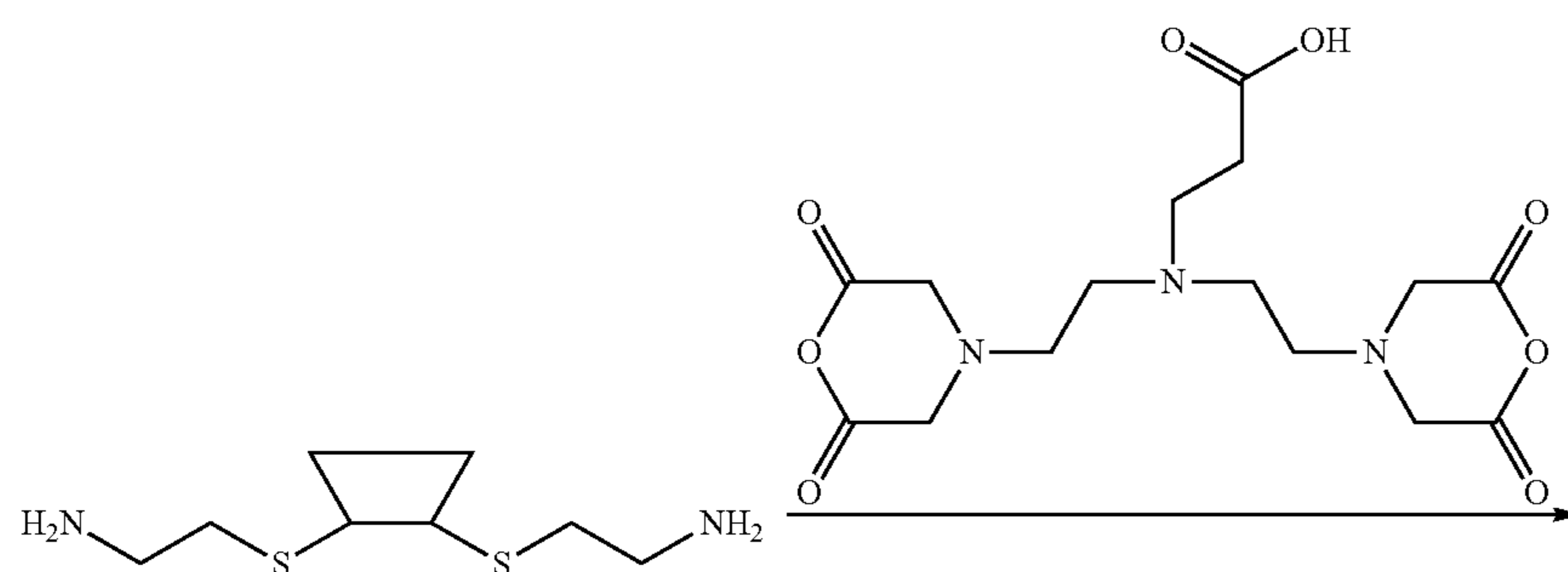
Scheme V
