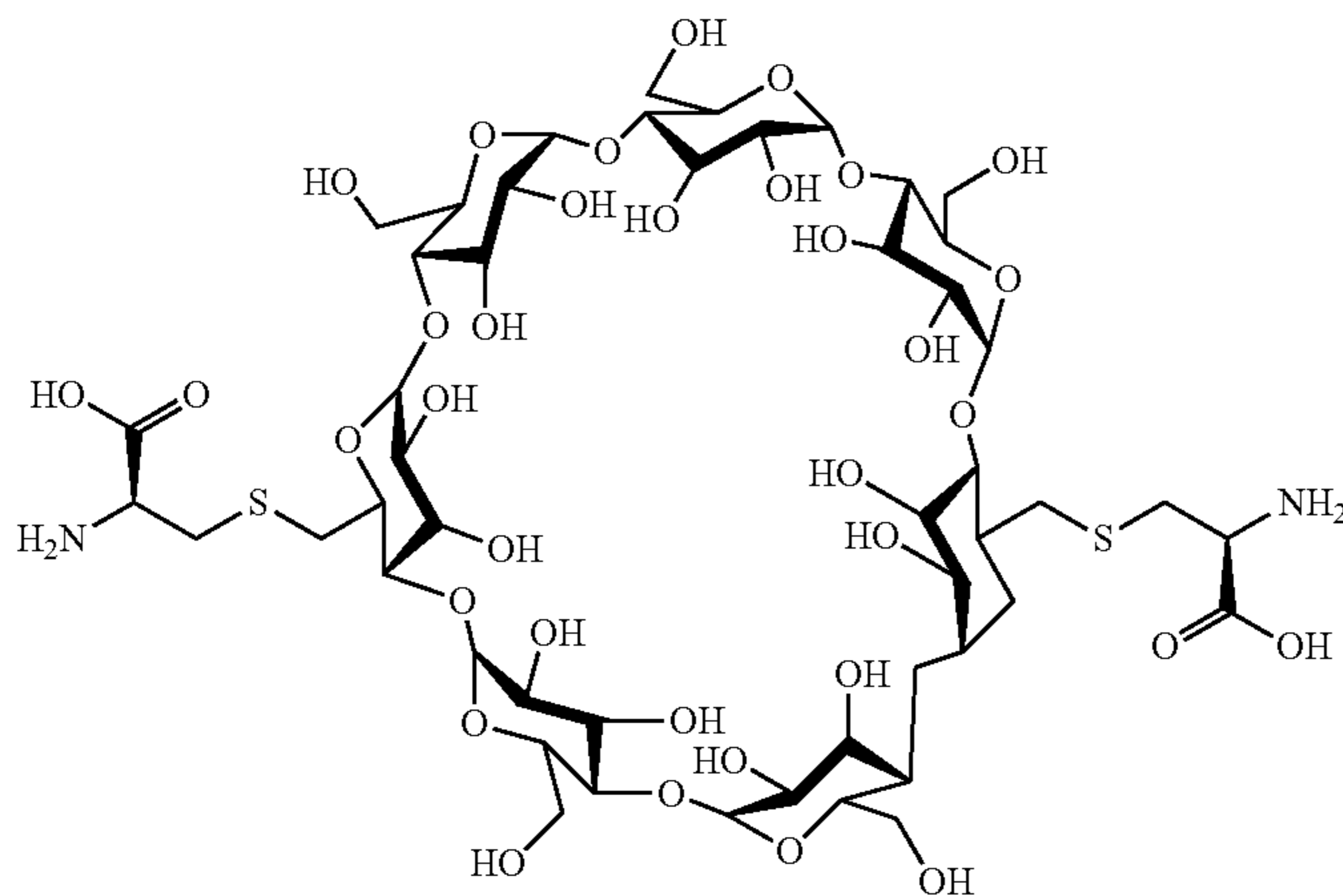
Scheme XXXVIIIa
