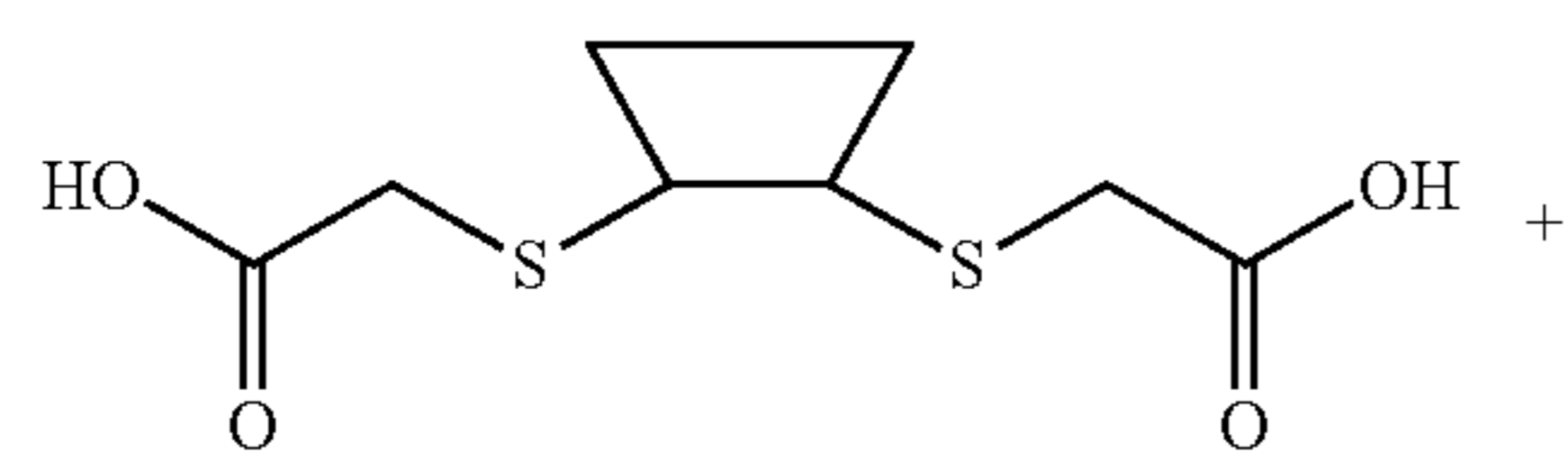
Scheme XXXII
