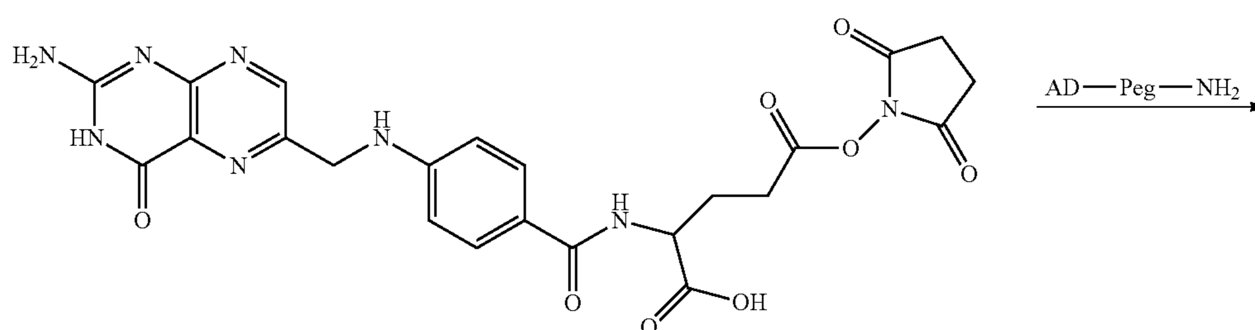
Scheme L
