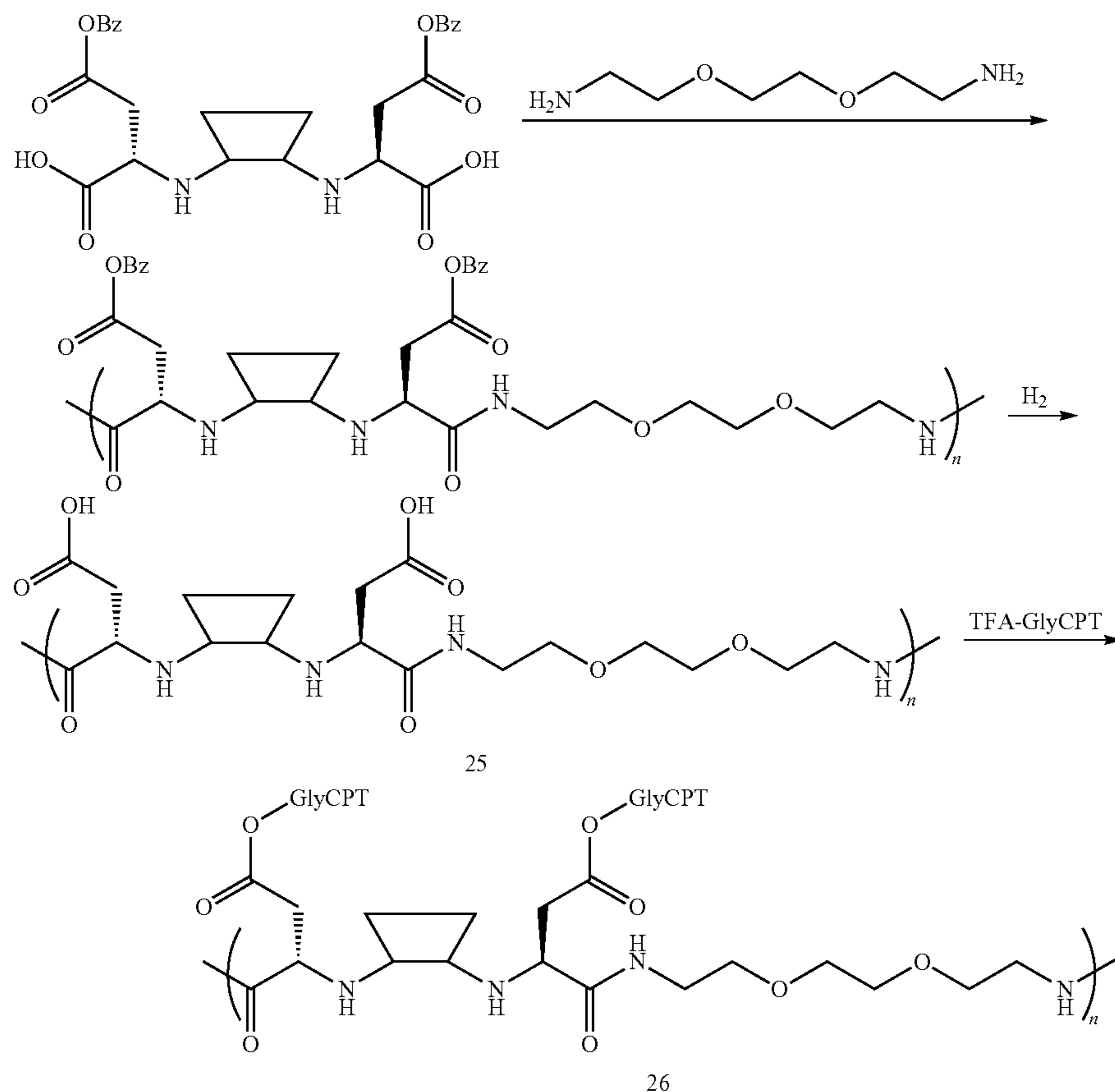
Scheme XXXI
