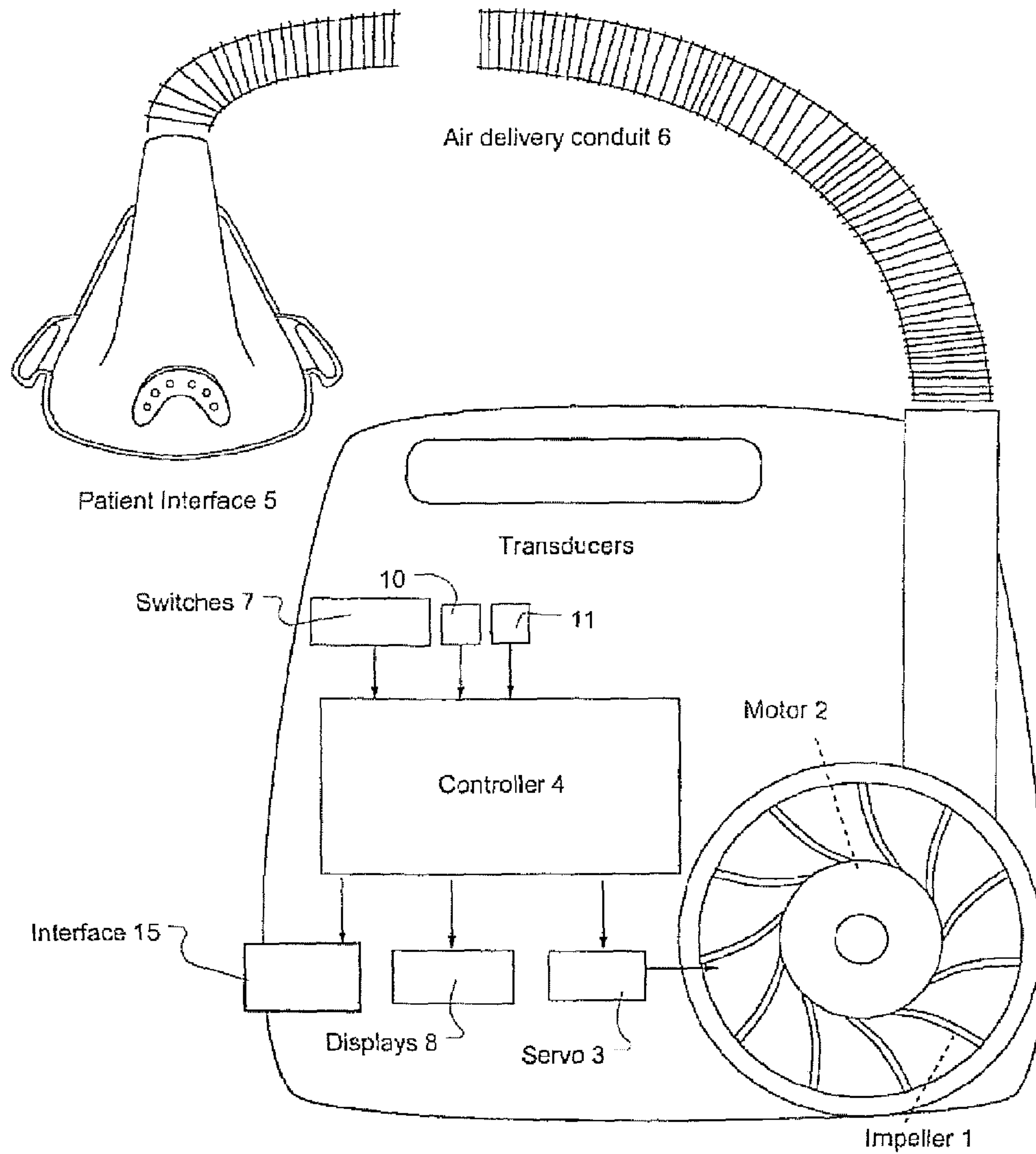
Fig. 1 (Prior Art)
