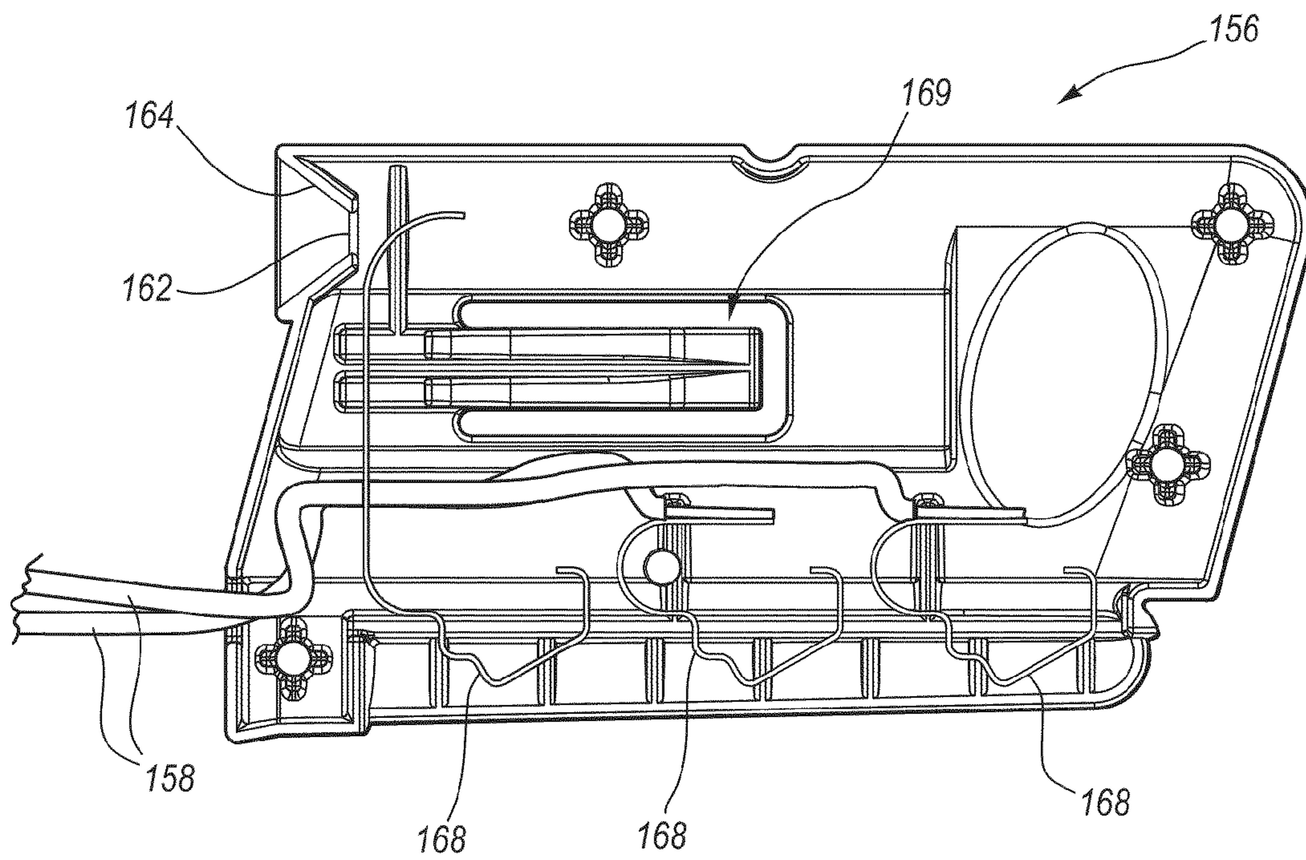
FIG. 13D
