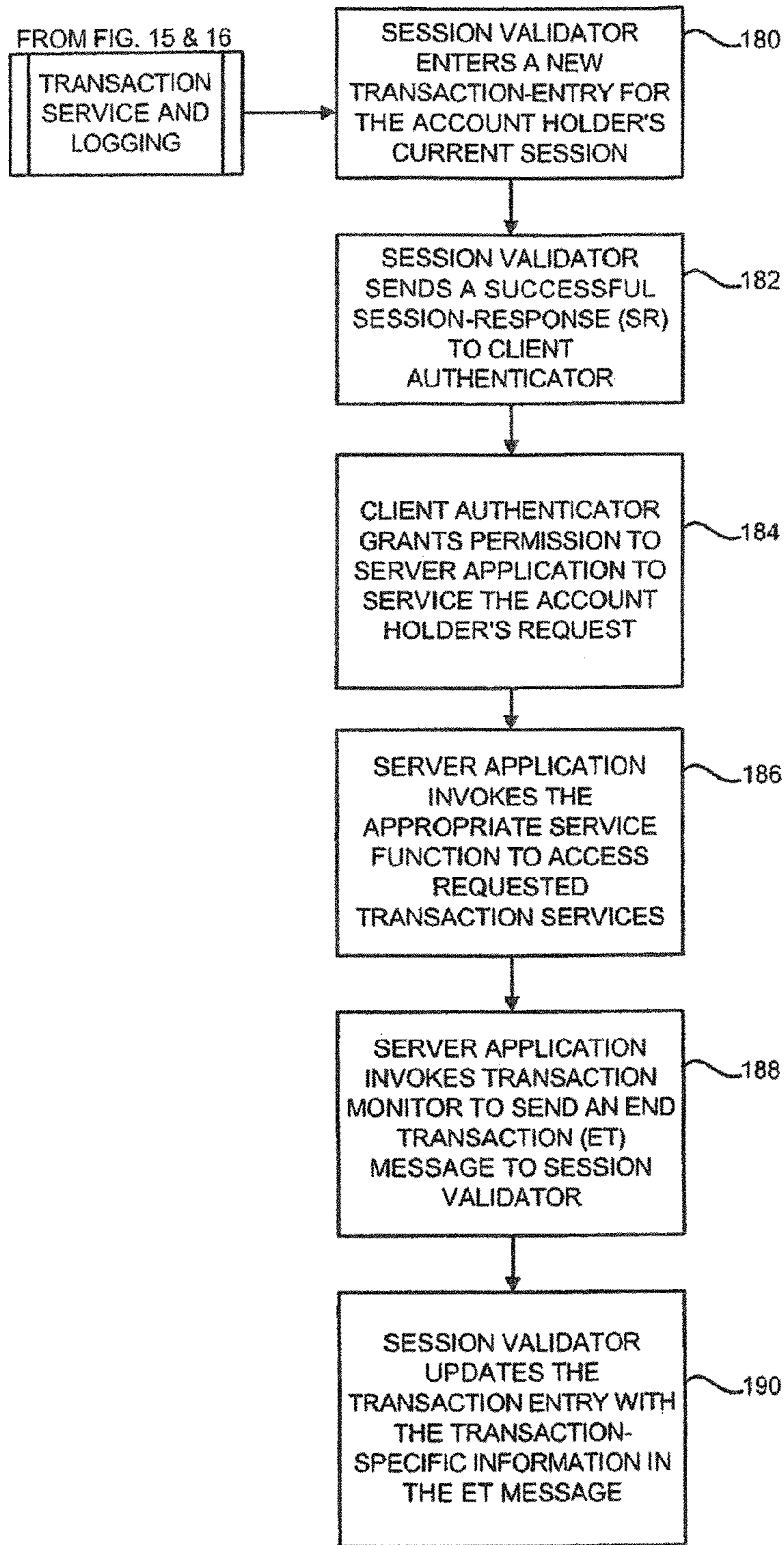
FIG. 17 - TRANSACTION SERVICE AND LOGGING
