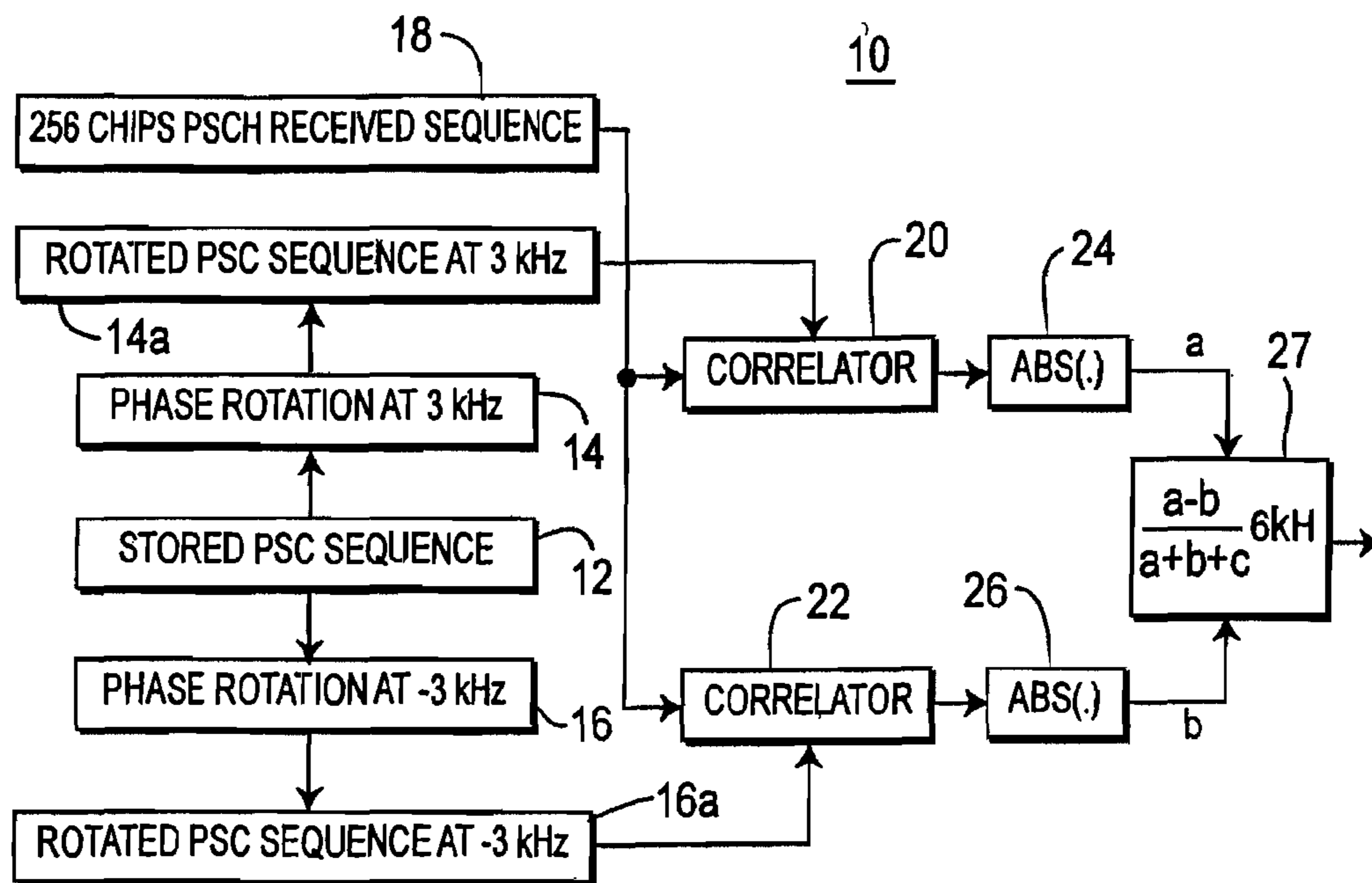
PHASE ROTATION APPROACH FOR START_UP AFC
