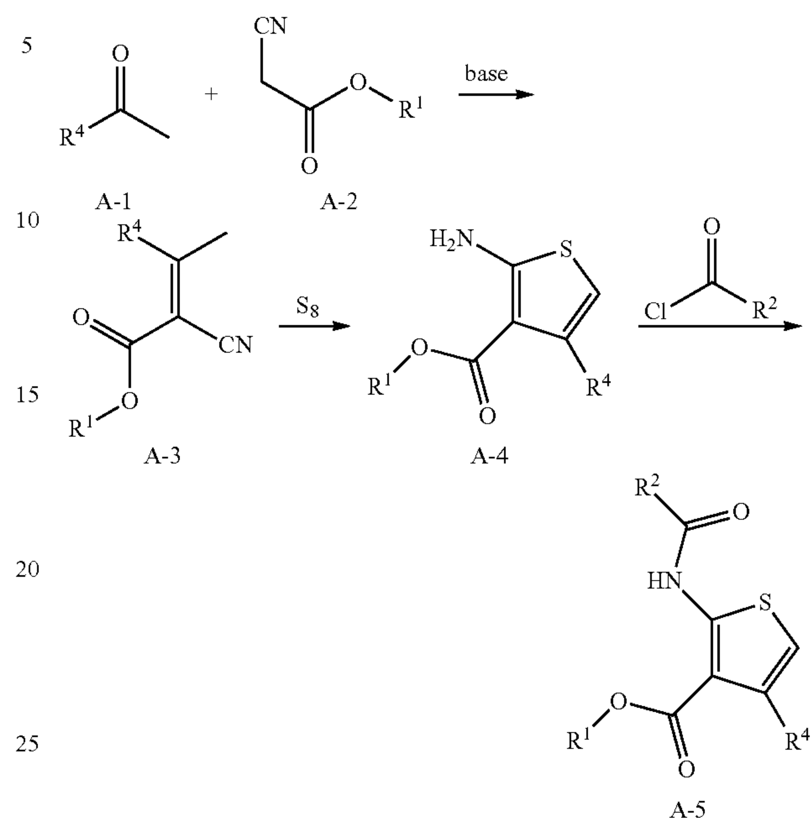
Scheme A. Non-limiting Example of the Synthesis of Compounds of Formula (I) - (V)
