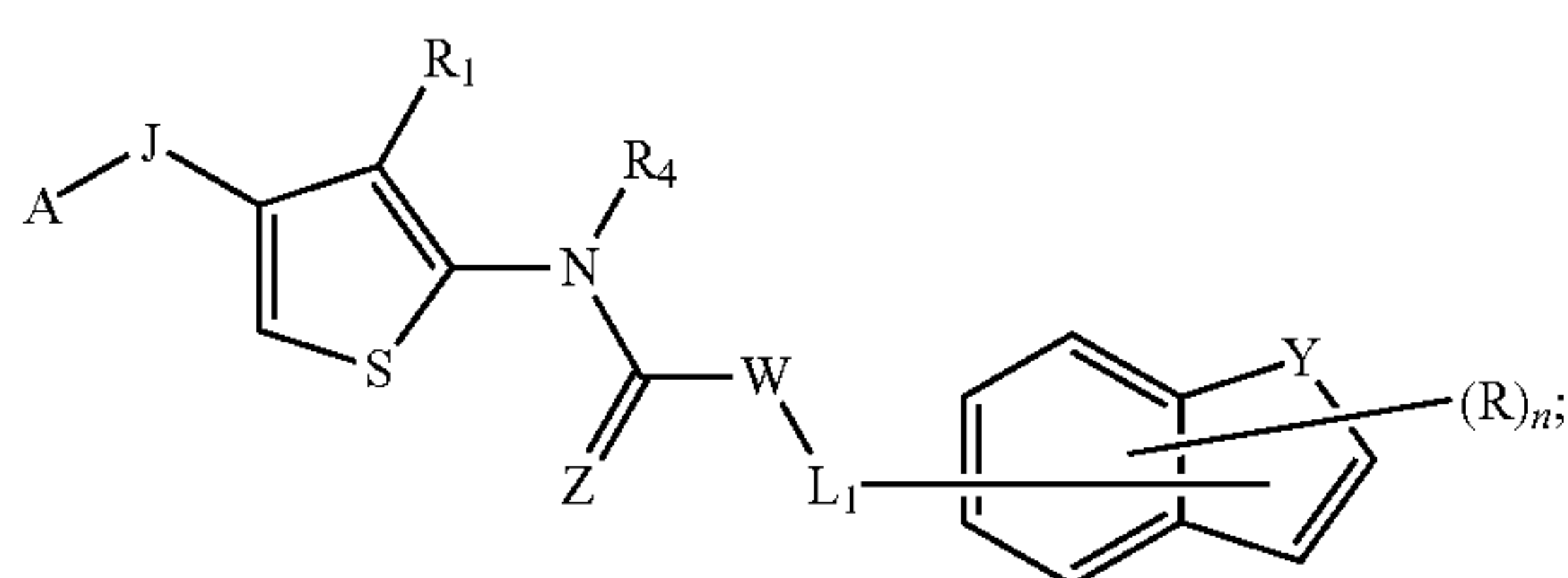
Formula (II)
