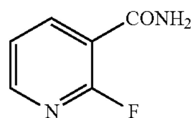
2-fluoronicotinamide
