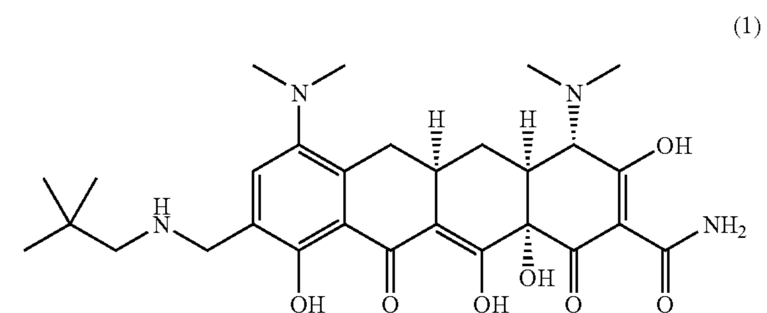
(1) (4S,4AS,5AR,12AS)-4-7-Bis(dimethylamino)-9{[(2,2-dimethylpropyl)amino]methyl}-3,10,12,12A-tetrahydroxy-1,11-dioxo-1,4,4A,5,5A,6,11,12A-octahydrotetracene-2-carboxamide
