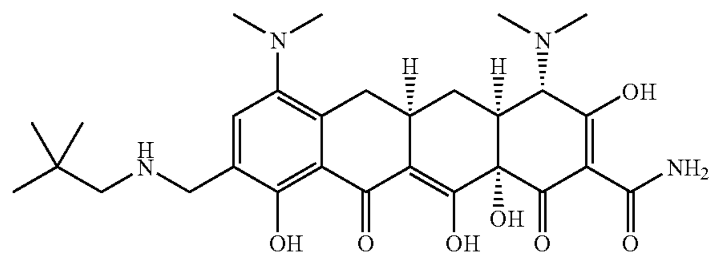
(1) (4S,4AS,5AR,12AS)-4-7-Bis(dimethylamino)-9-[(2,2-dimethylpropyl)amino]methyl-3,10,12,12A-tetrahydroxy-1,11-dioxo-1,4,4A,5,5A,6,11,12A-octahydro-2-carboxamide (9-(2,2-dimethylpropyl-aminomethyl)-minocycline)
