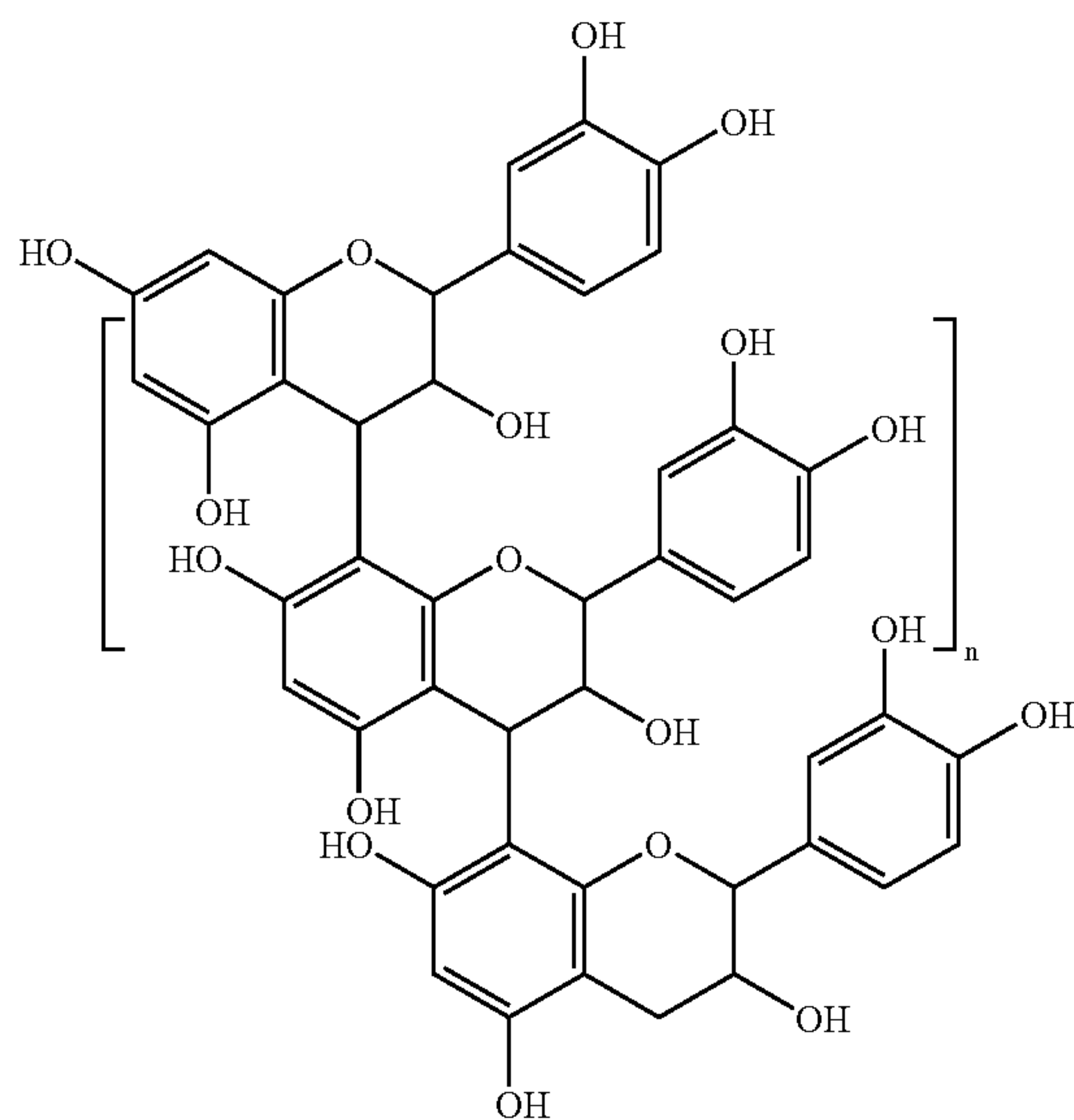
Structural formula 1
