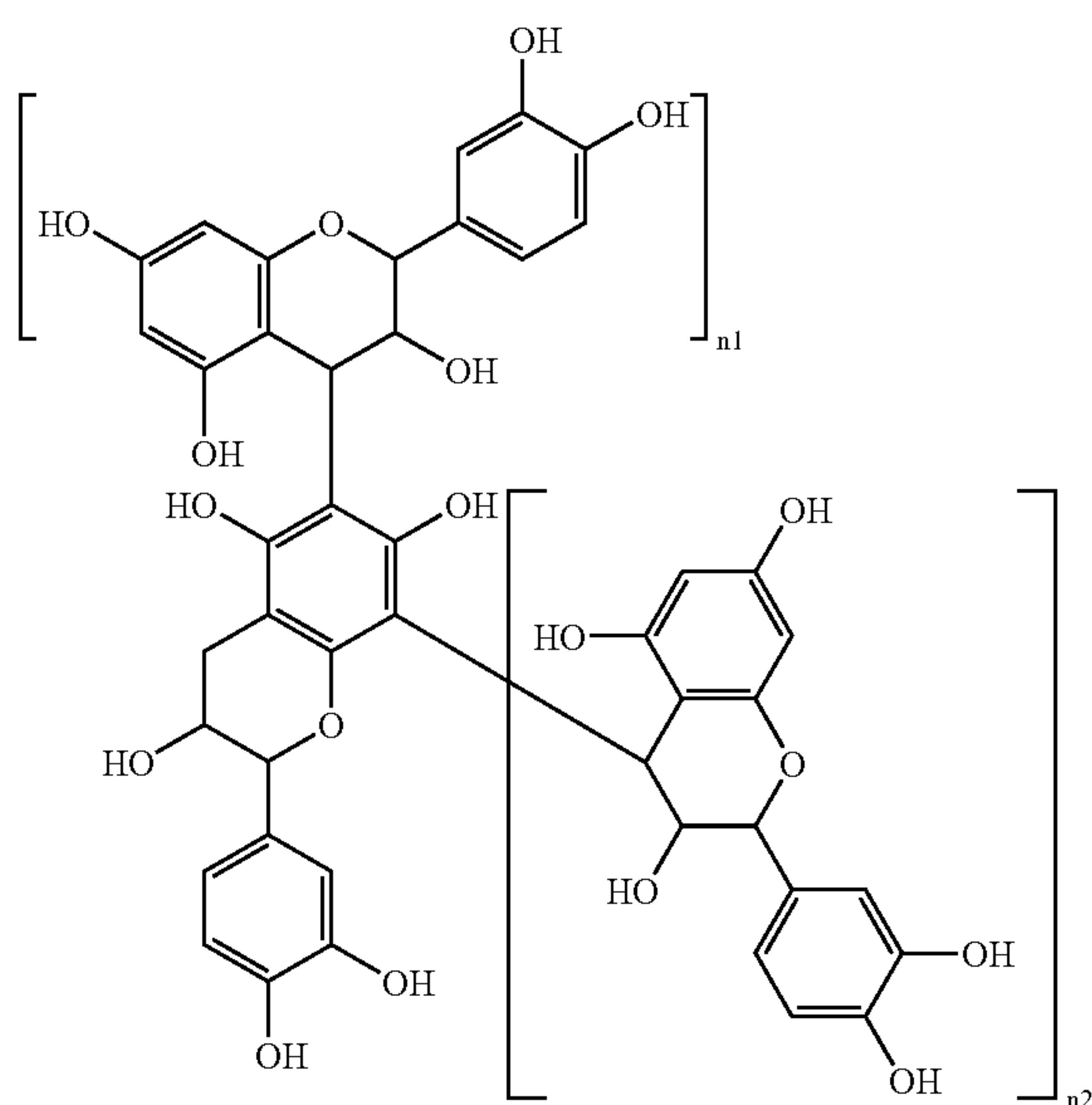
Structural formula 2
