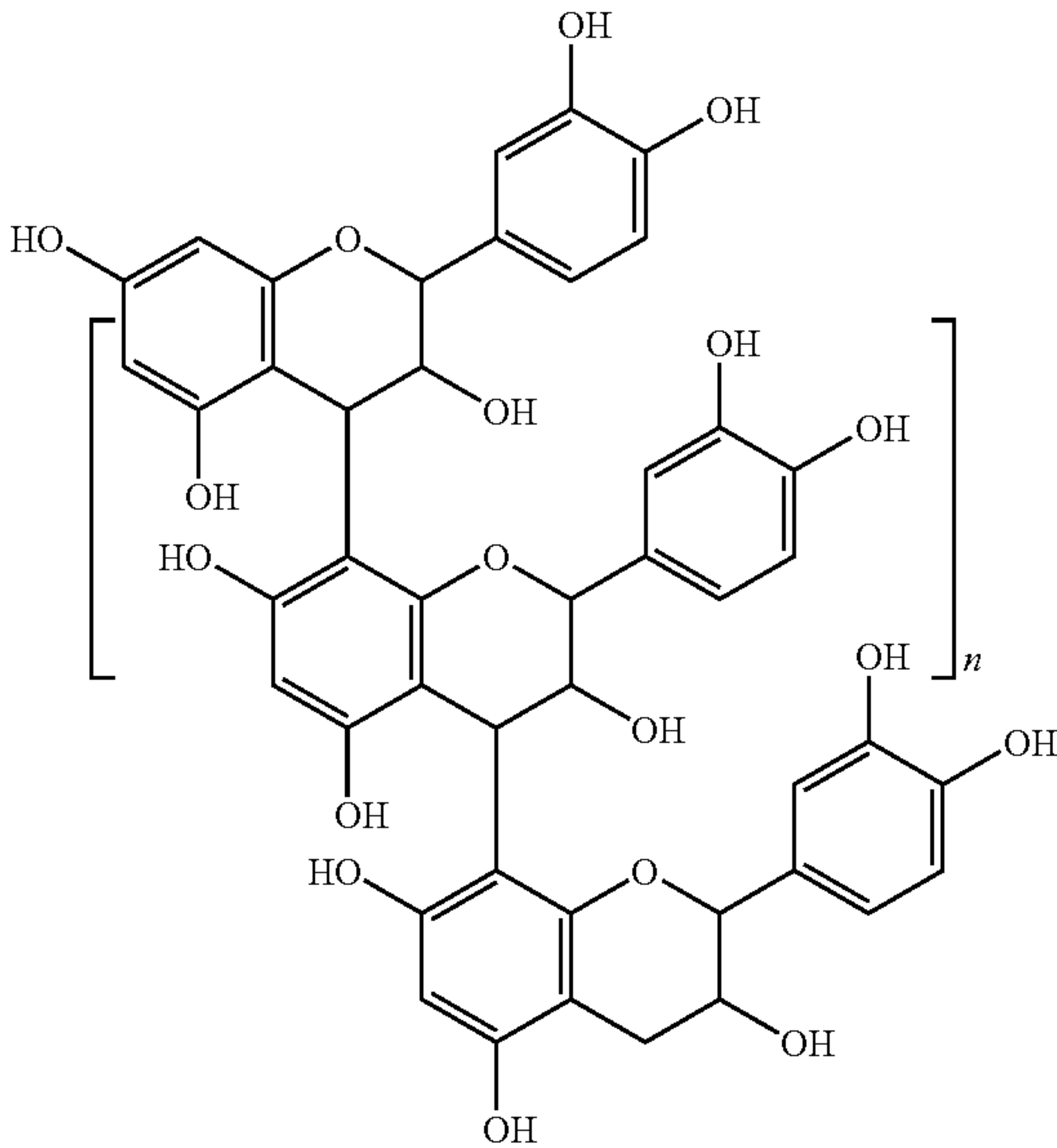
[Chemical formulas 1]
