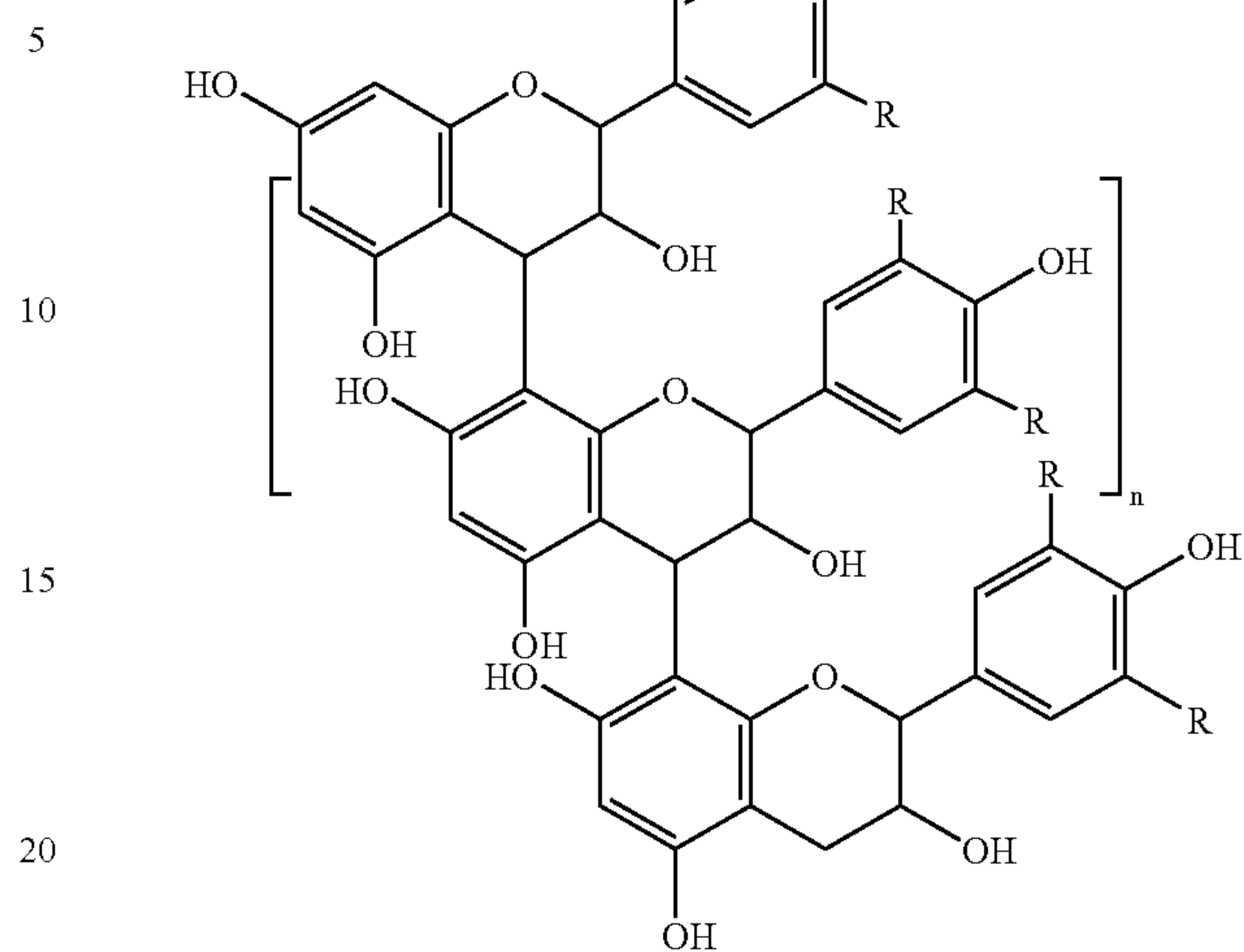
Structural formula 3
