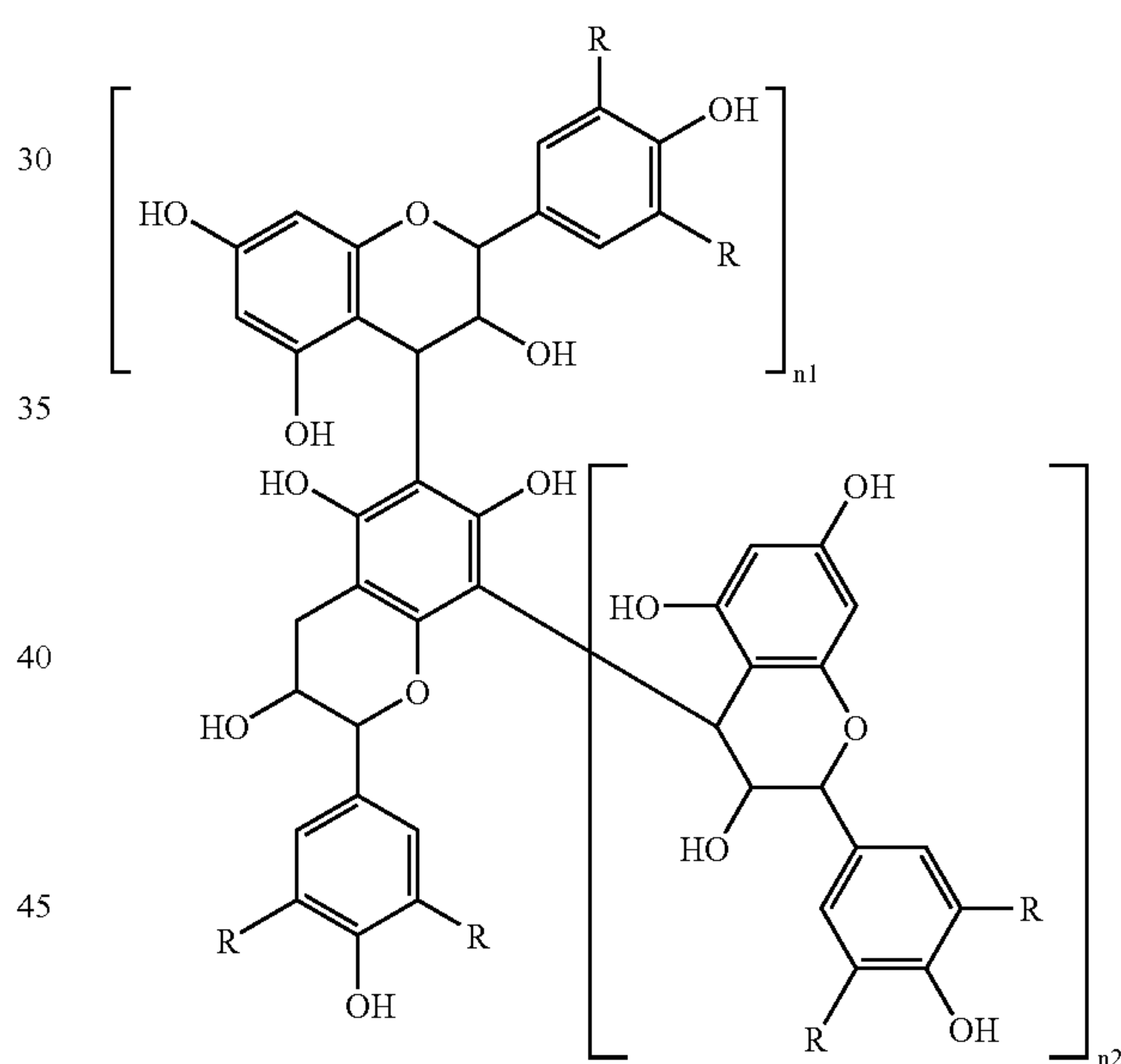
Structural formula 4
