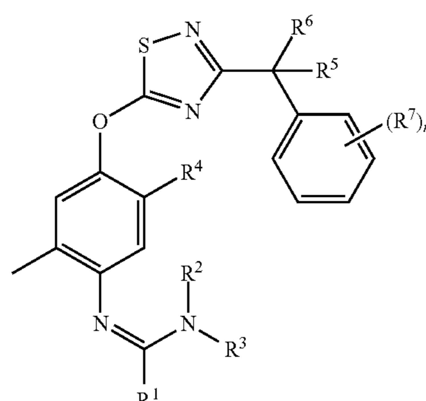
Z-isomer
