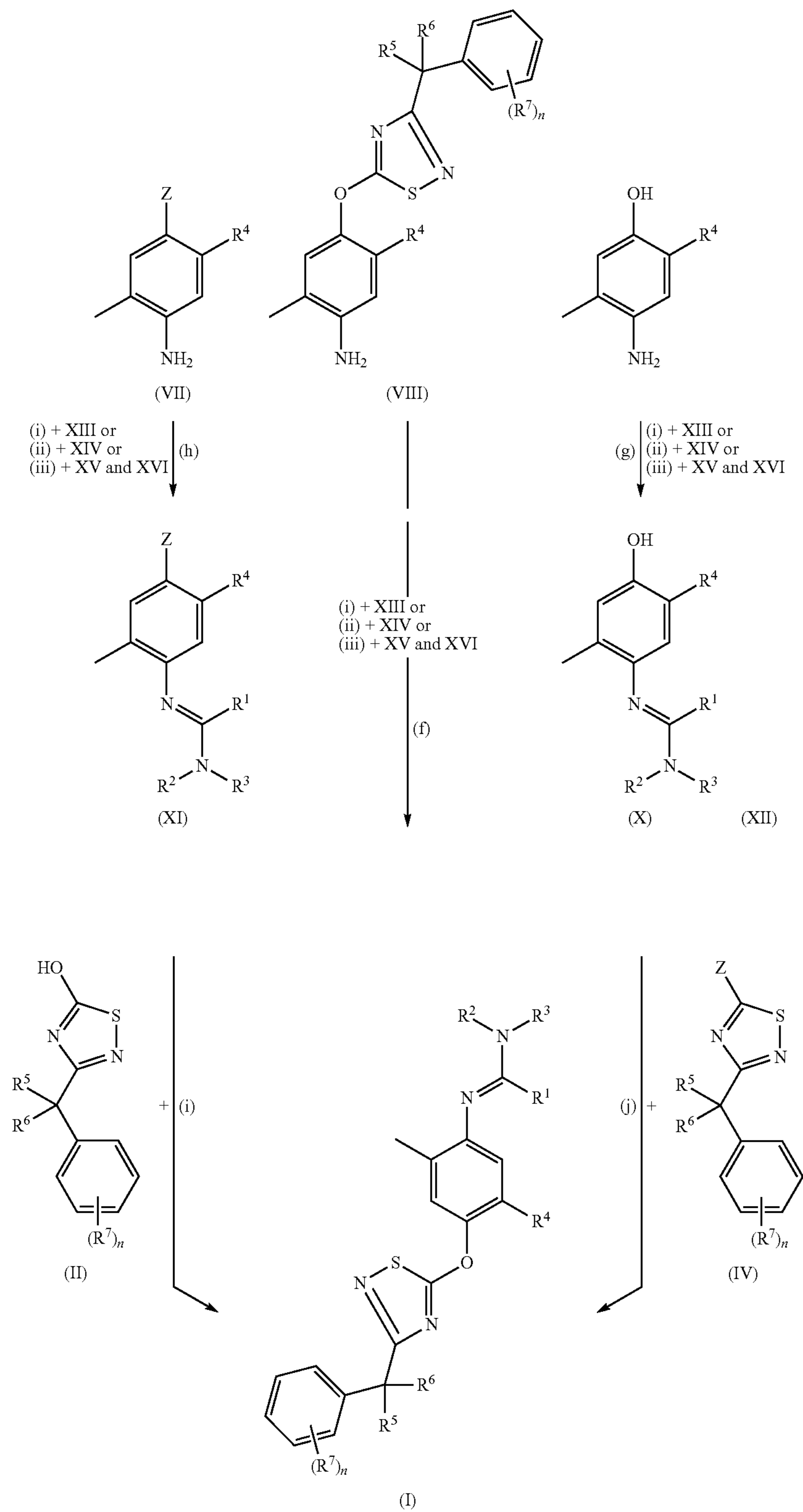
Scheme (Ib)
