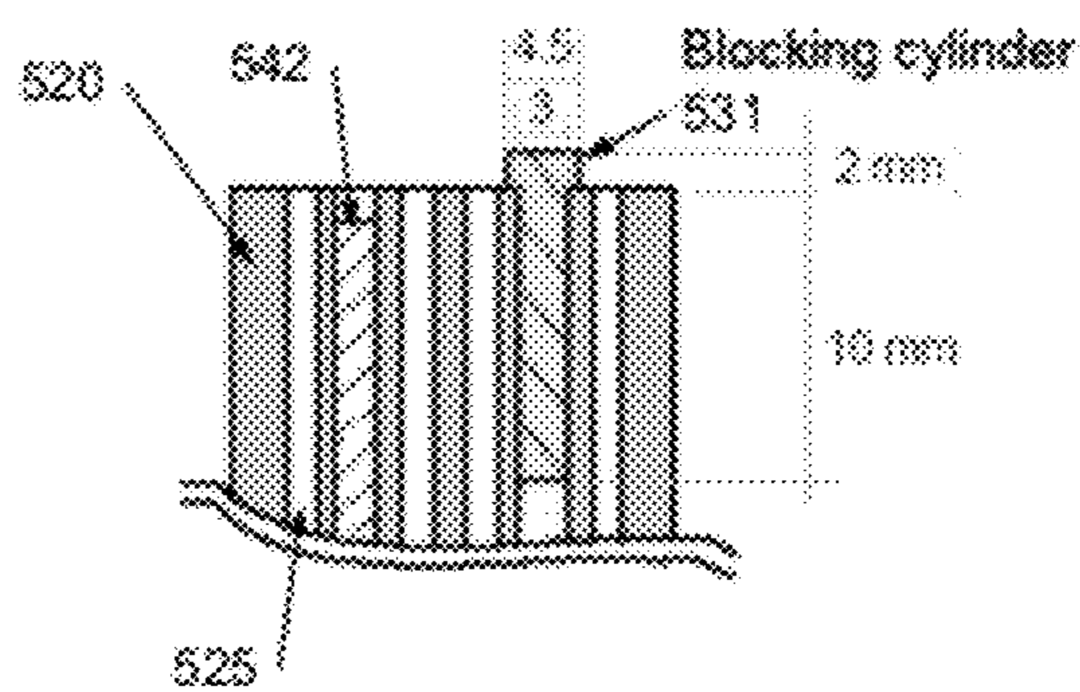
B-B view
