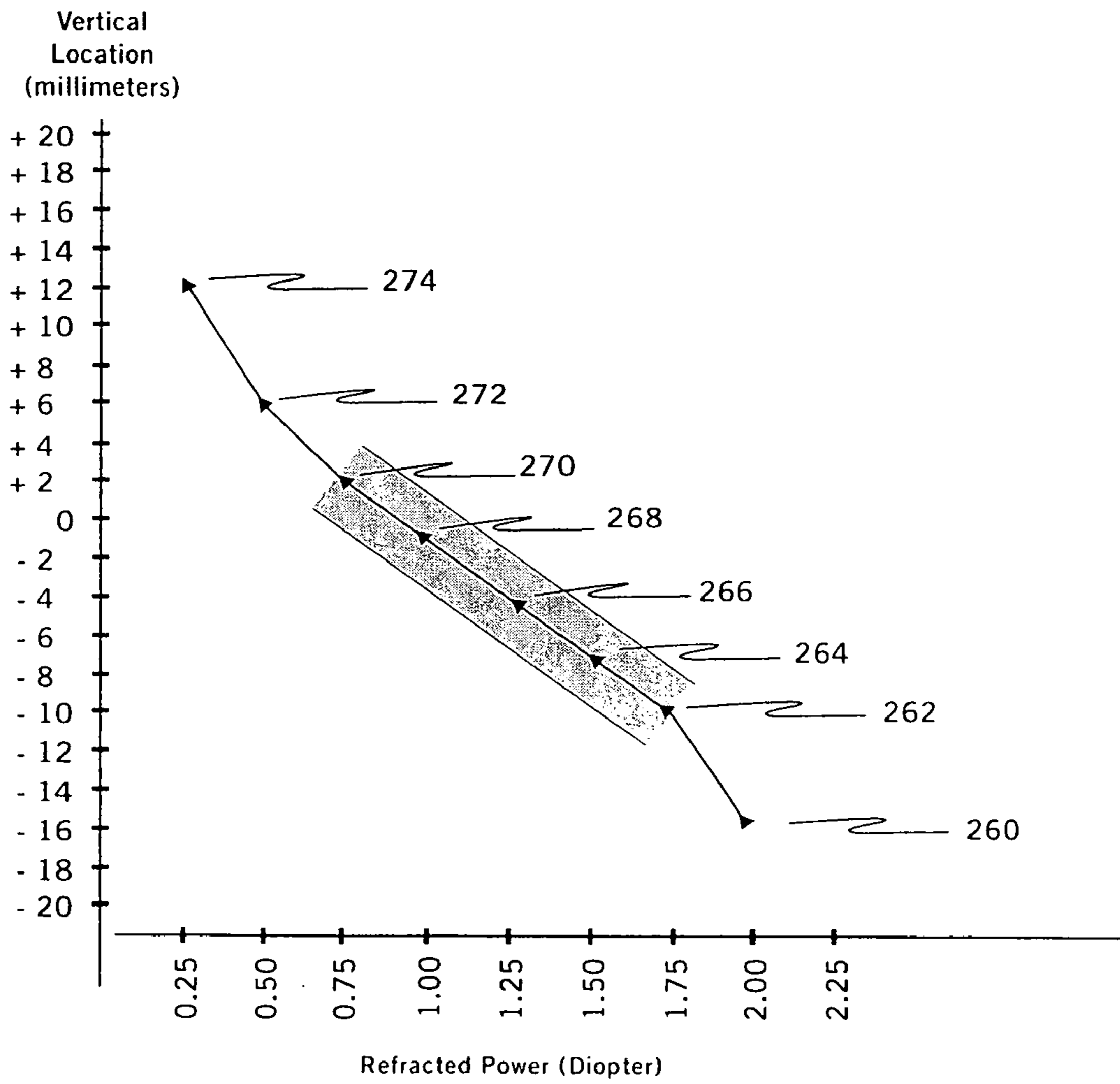
PROGRESSION OF REFRACTED POWER IN A 2.0 DIOPTER LENS-DIOPTER
