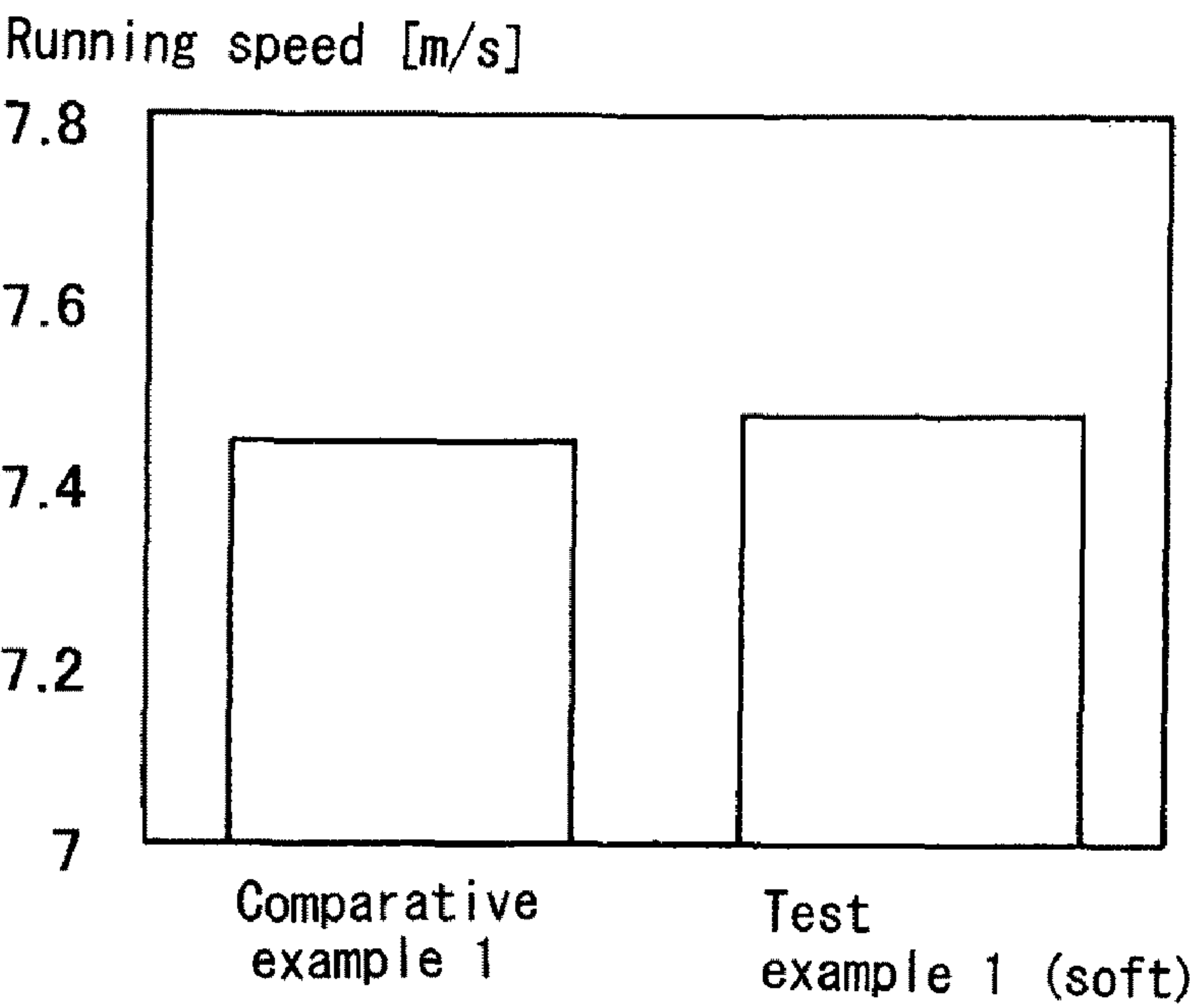
FIG. 11 A : Short-distance running
