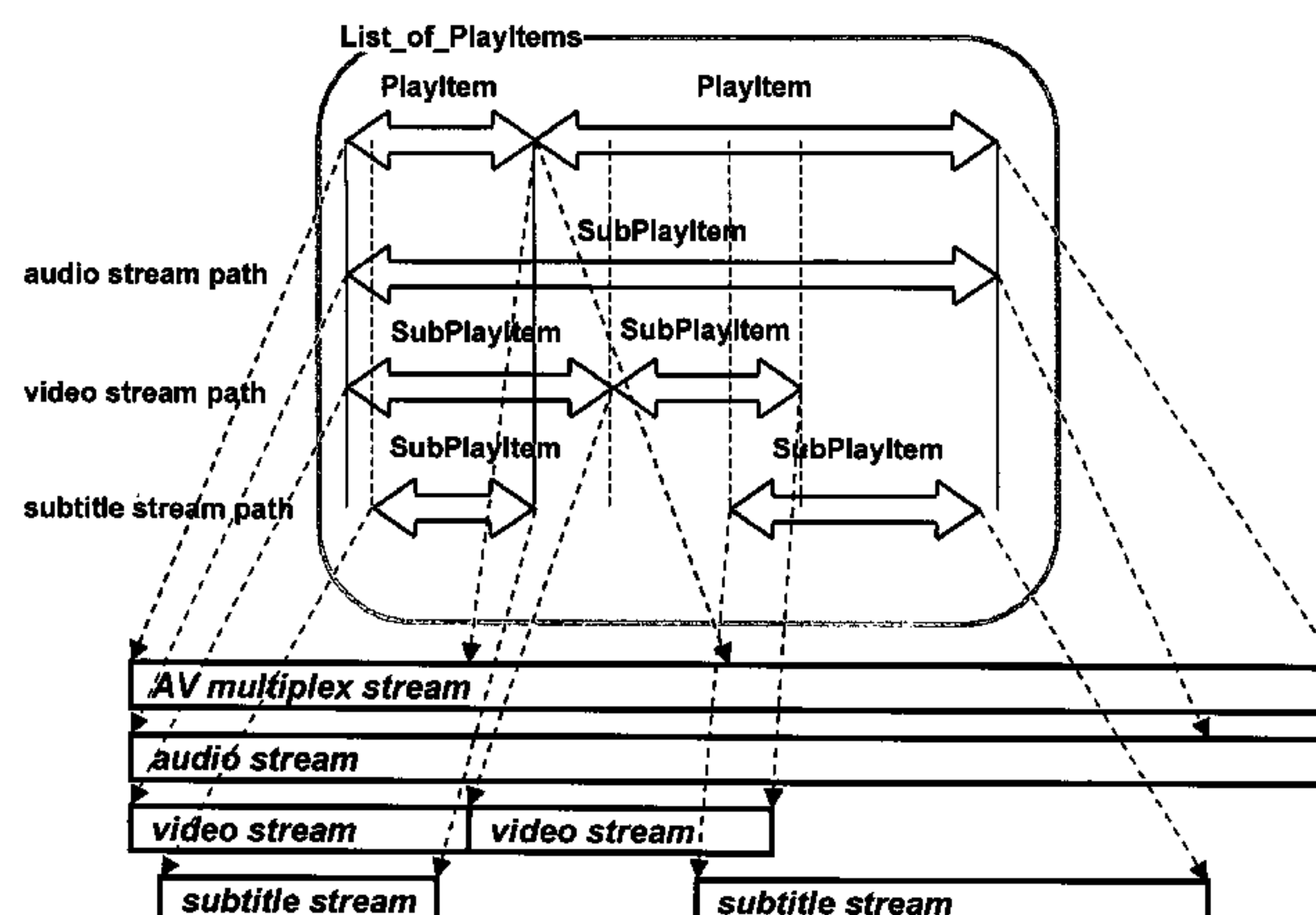
List_of_PlayItems Example
