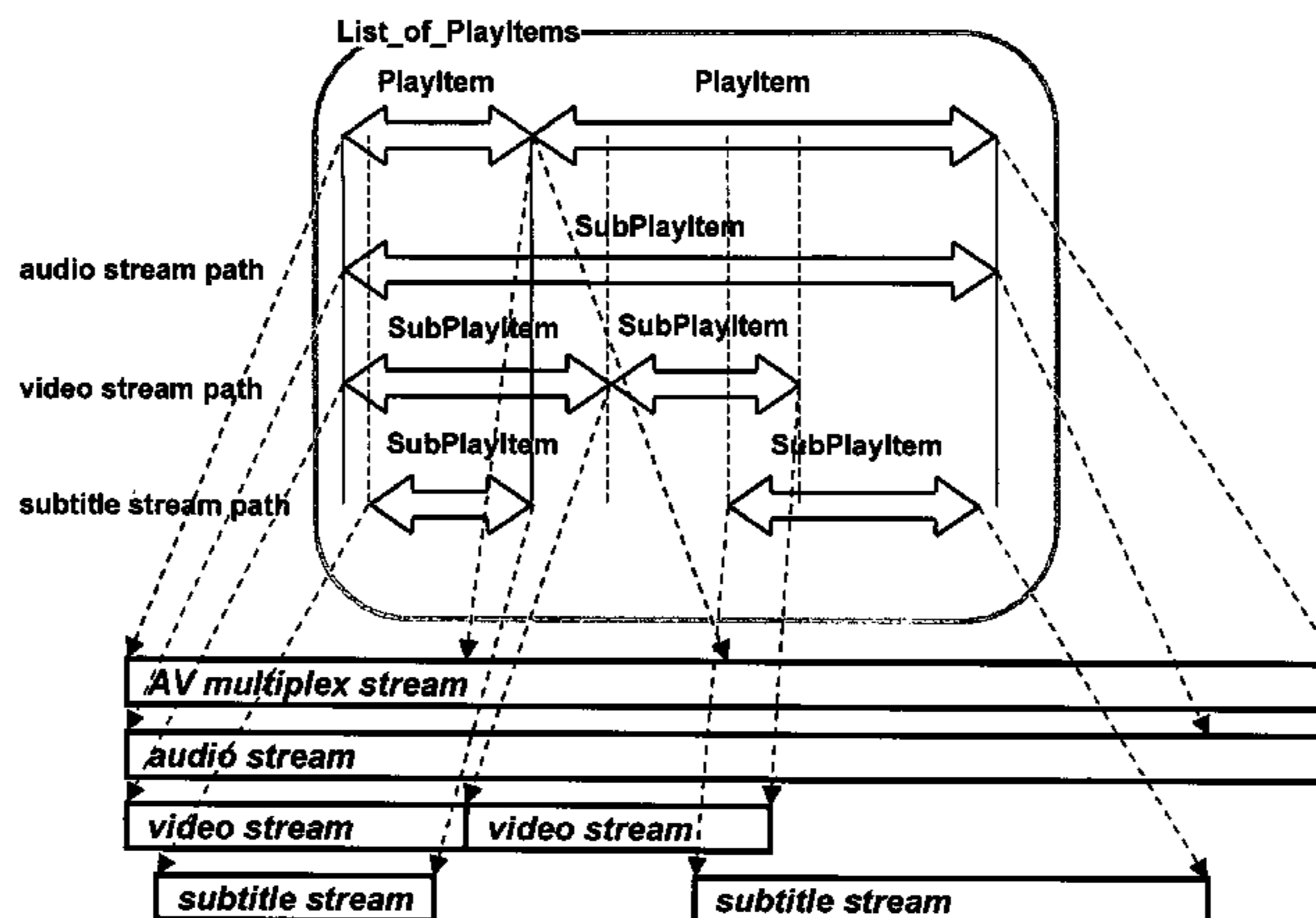
List_of_PlayItems Example
