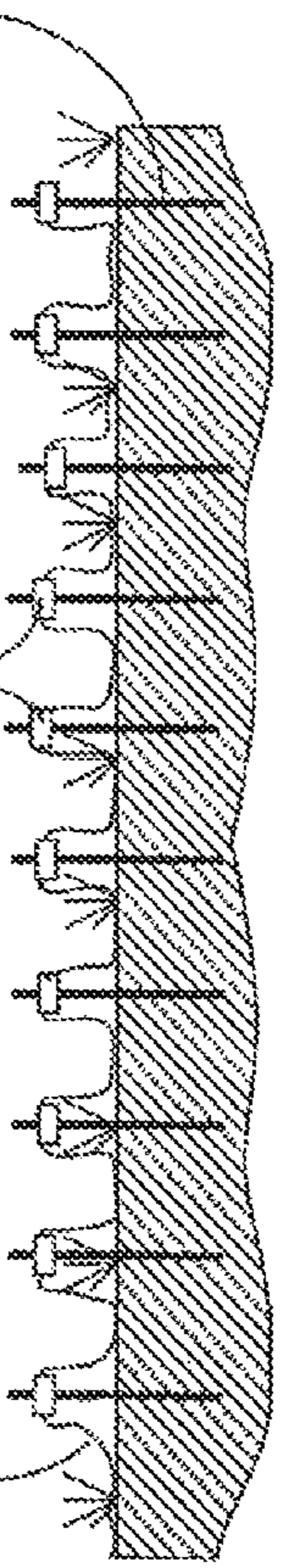
FIG. 6 Horizontal section showing vertical borehole probe array
