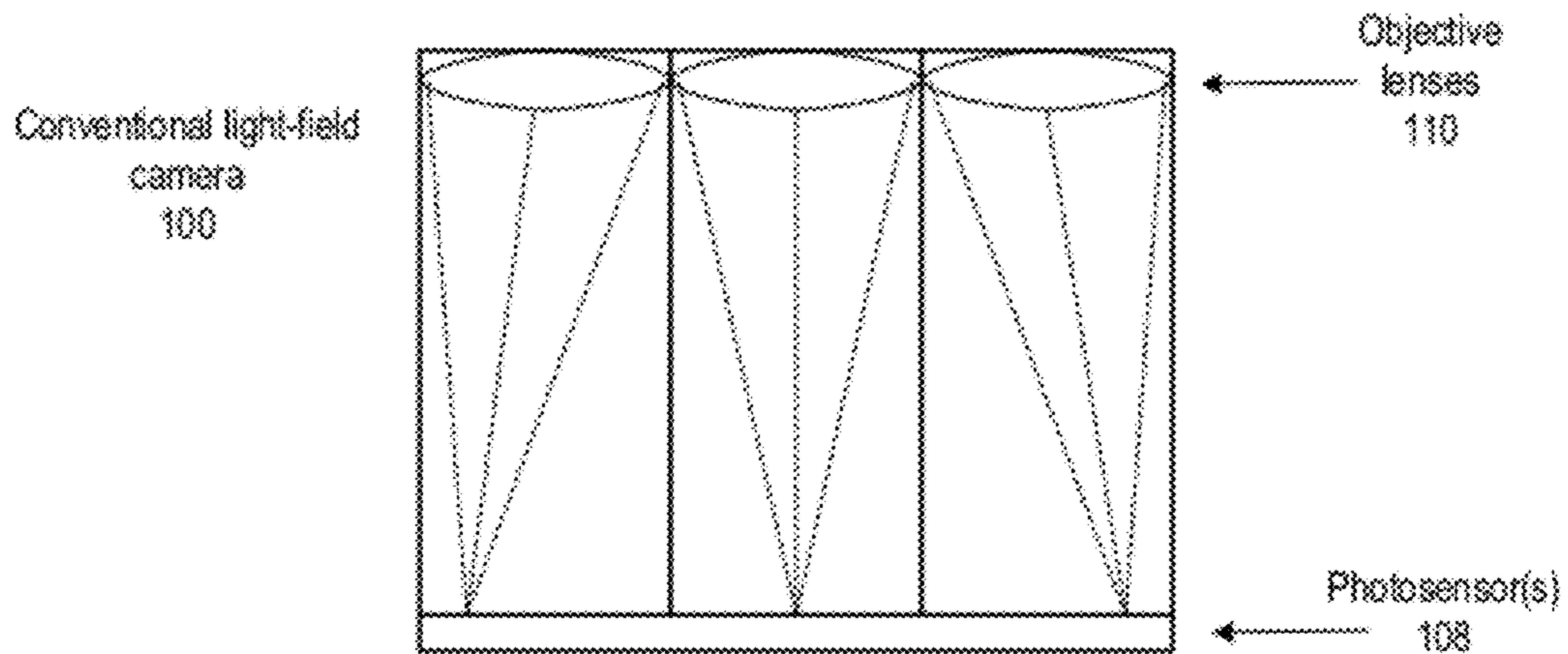
Figure 2 (PRIOR ART)
