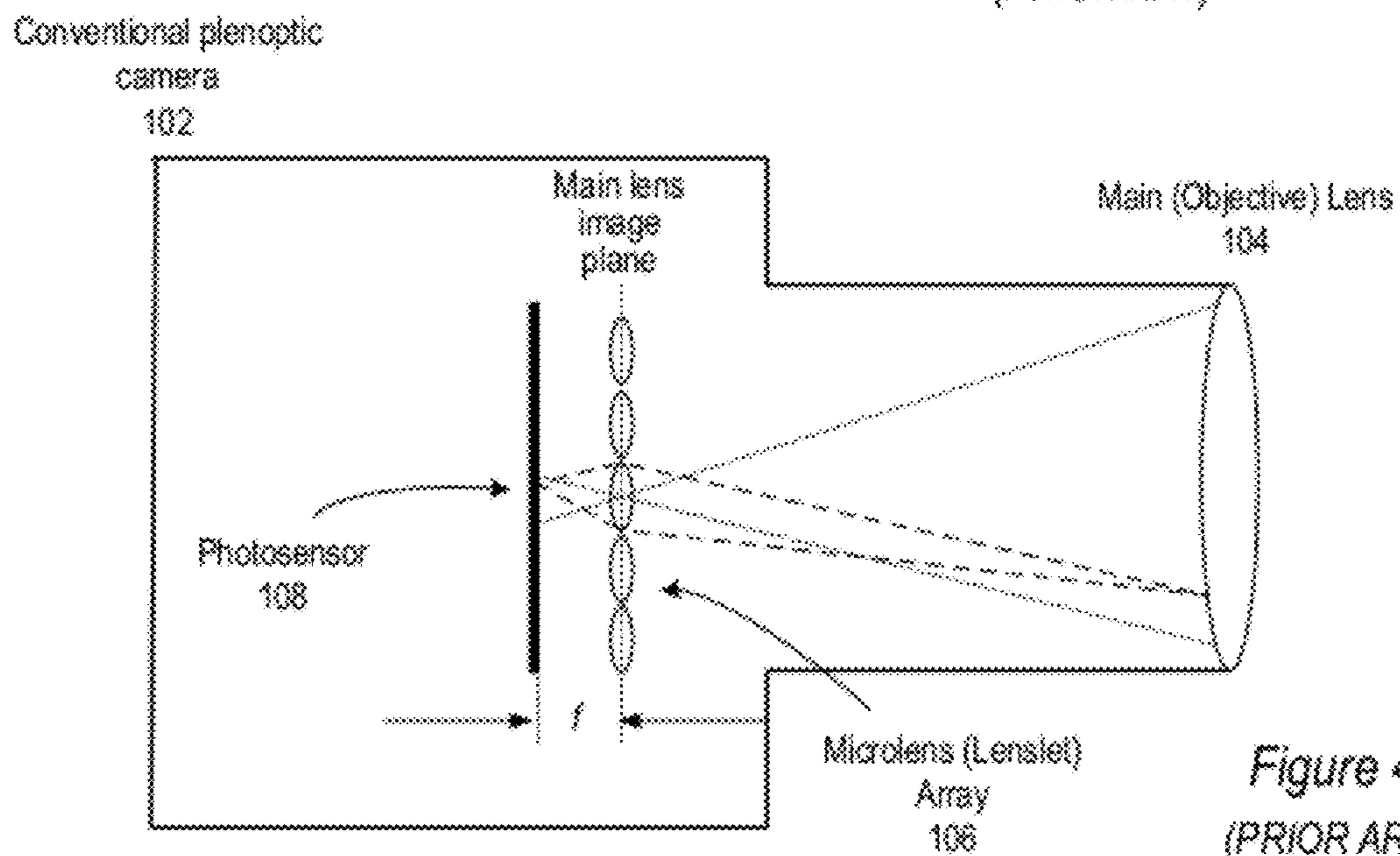
Figure 3 (PRIOR ART)
