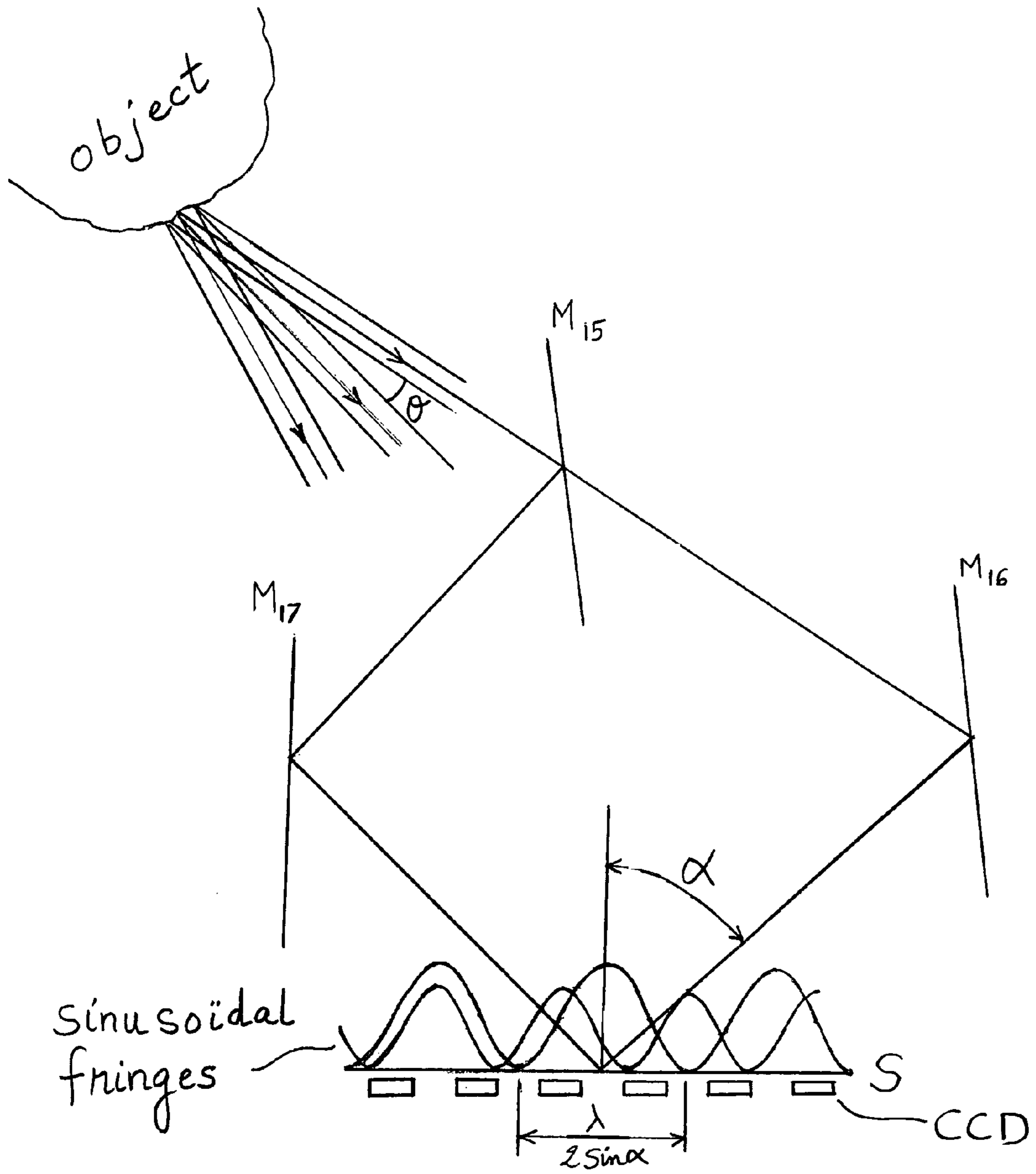
Fig. 6 Amplitude Splitting Imaging Interferometer
