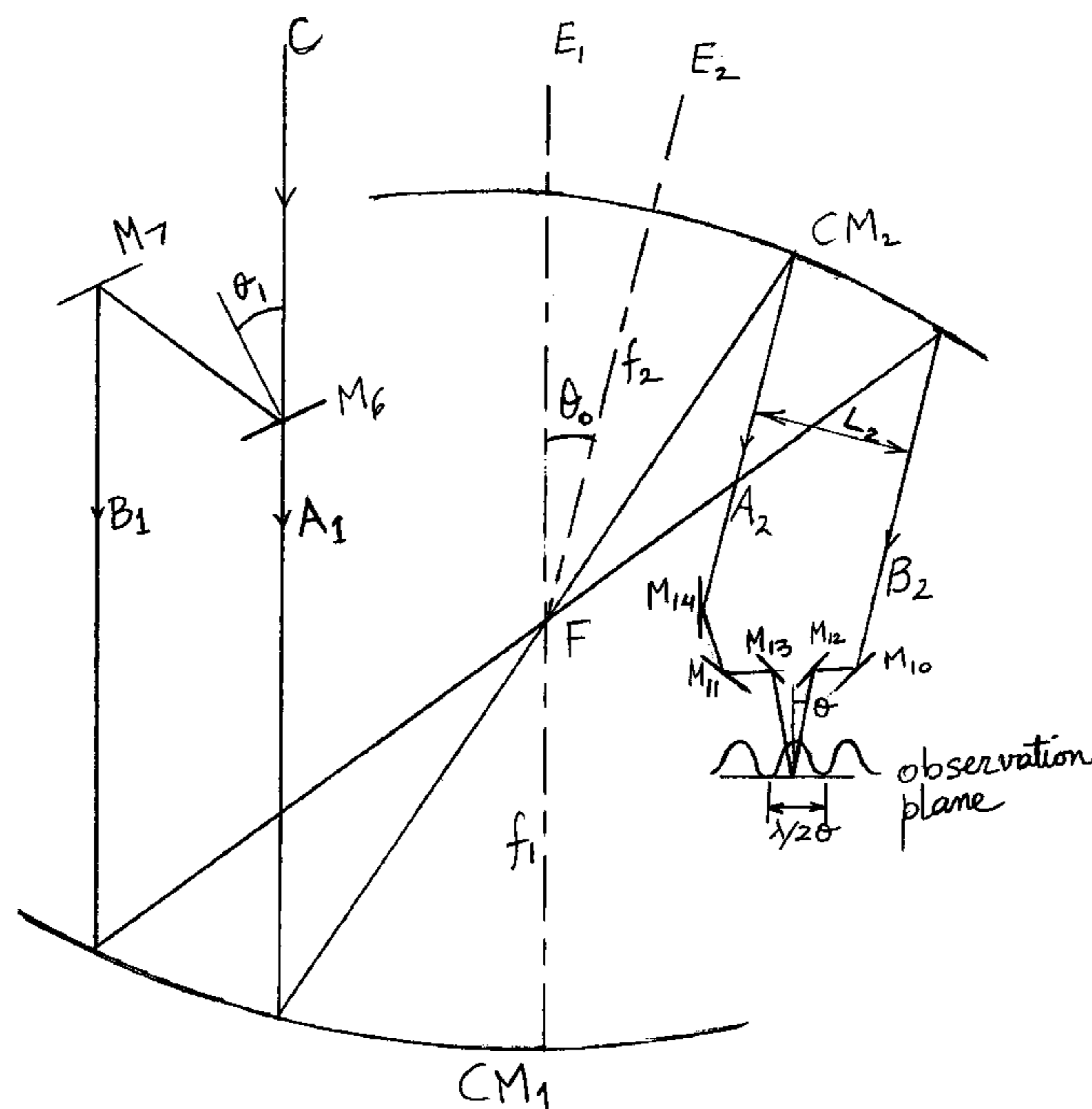
Interferometer with reduced cross section
