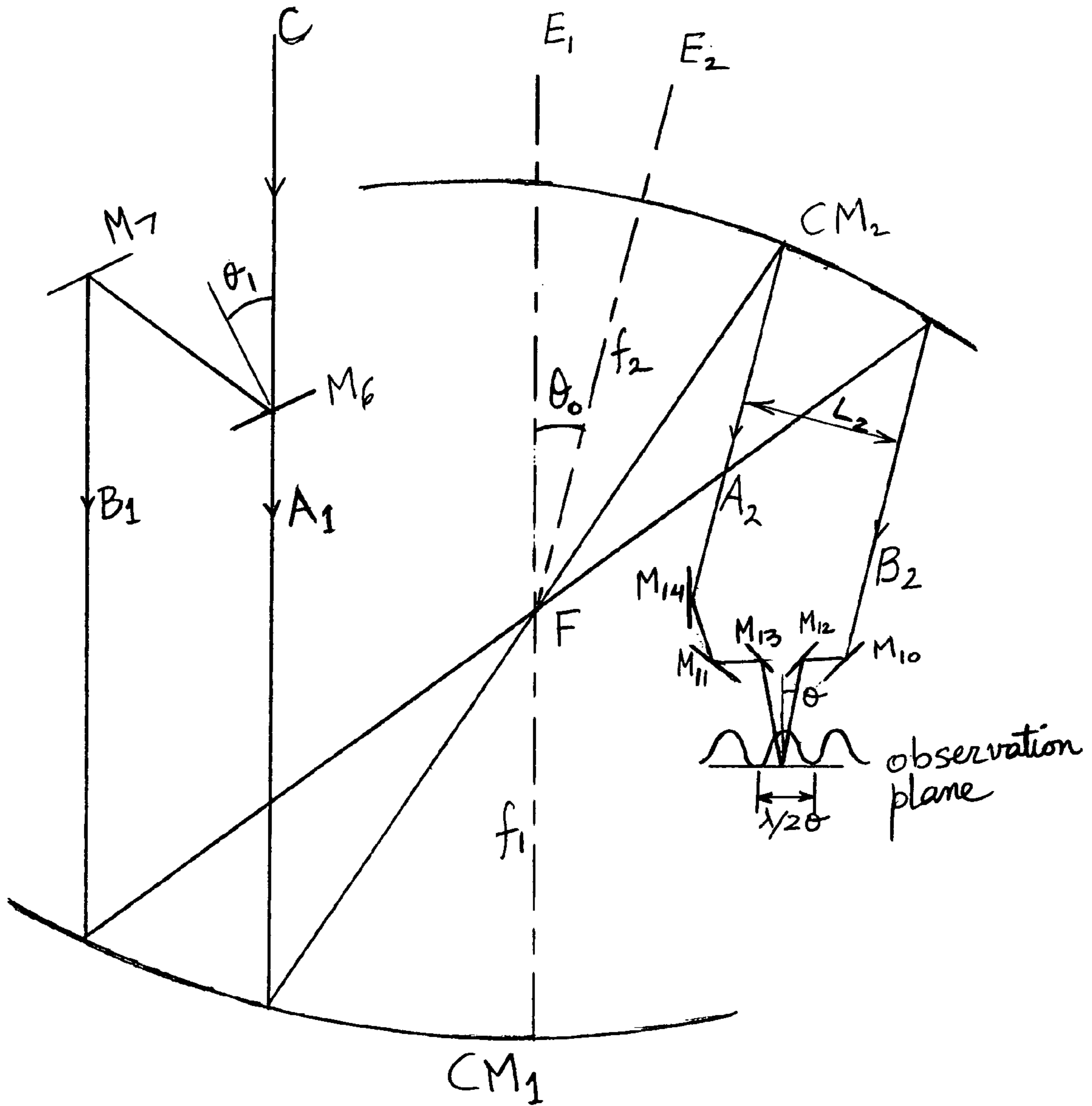
Fig. 5. Interferometer with reduced cross section
