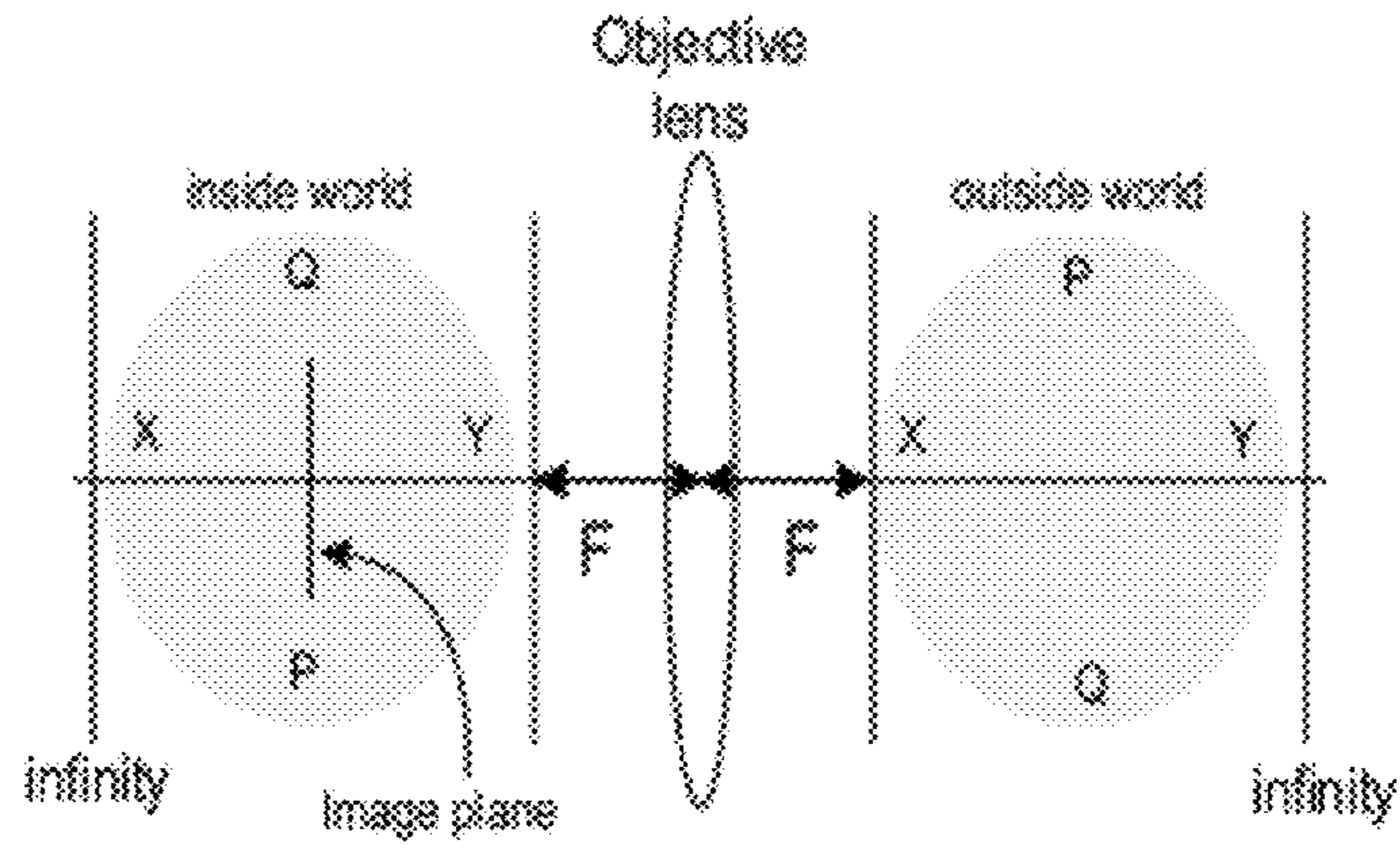
Figure 1 (PRIOR ART)
