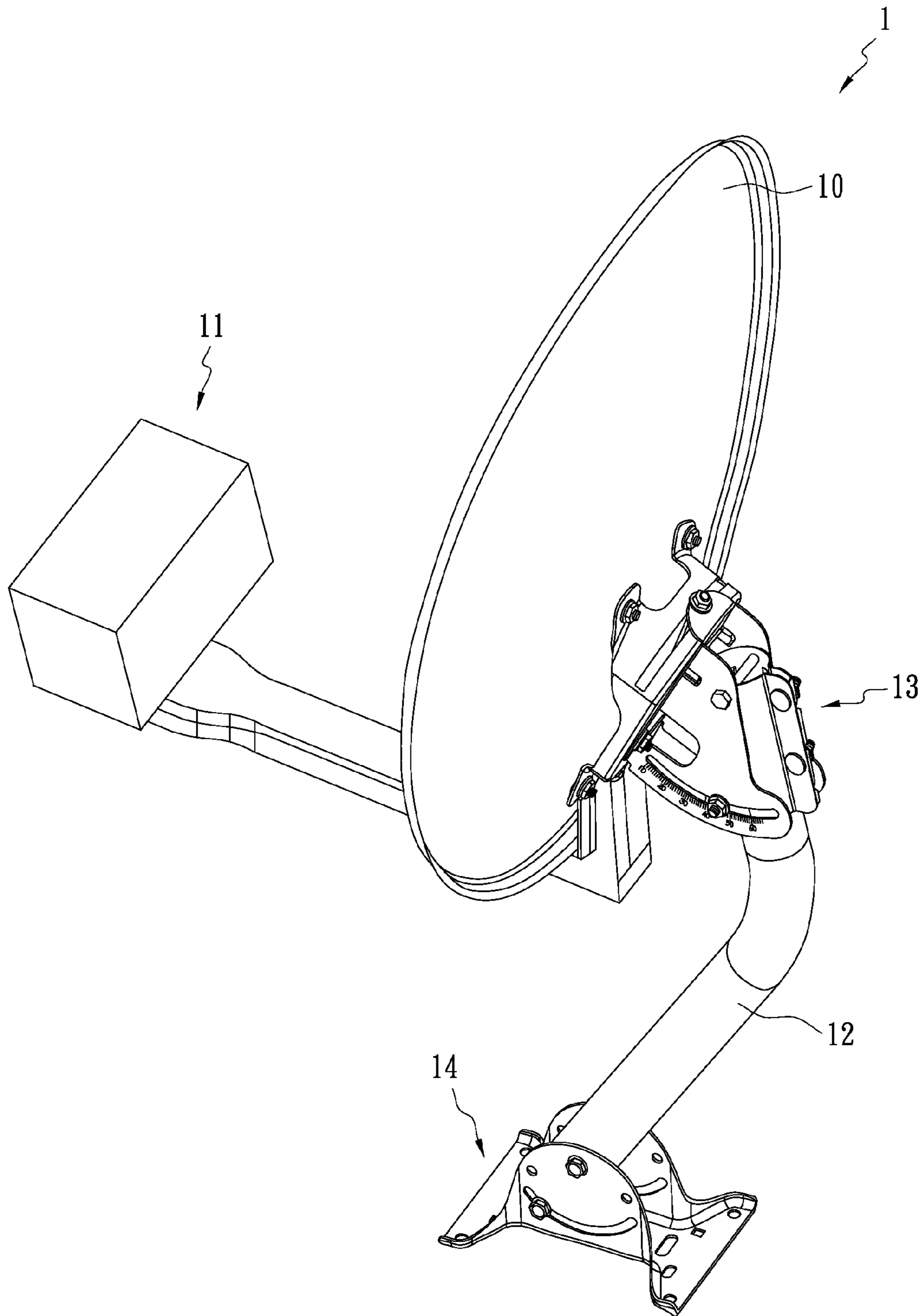
FIG. 1 (Prior Art)
