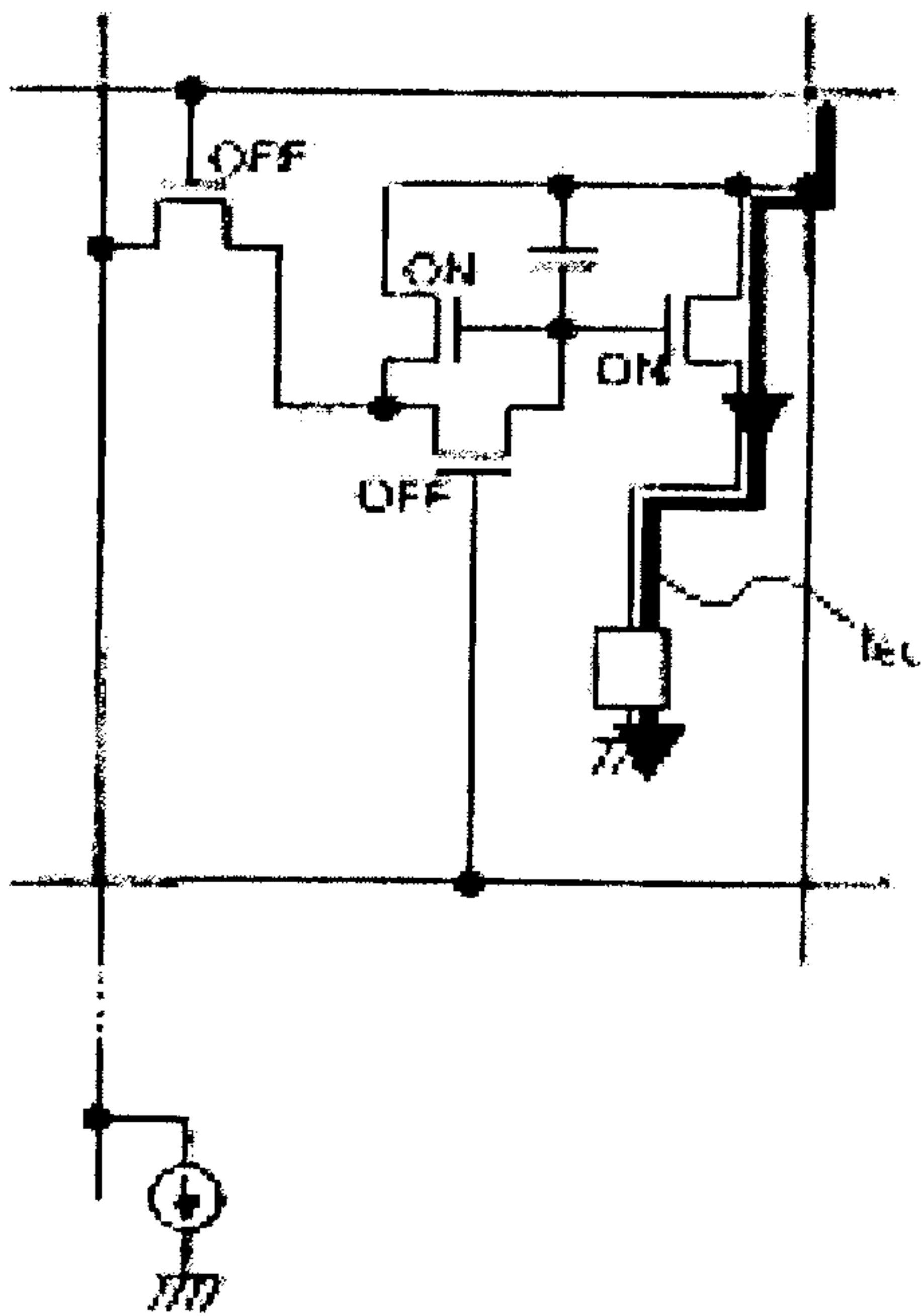
Fig. 20C Prior Art
