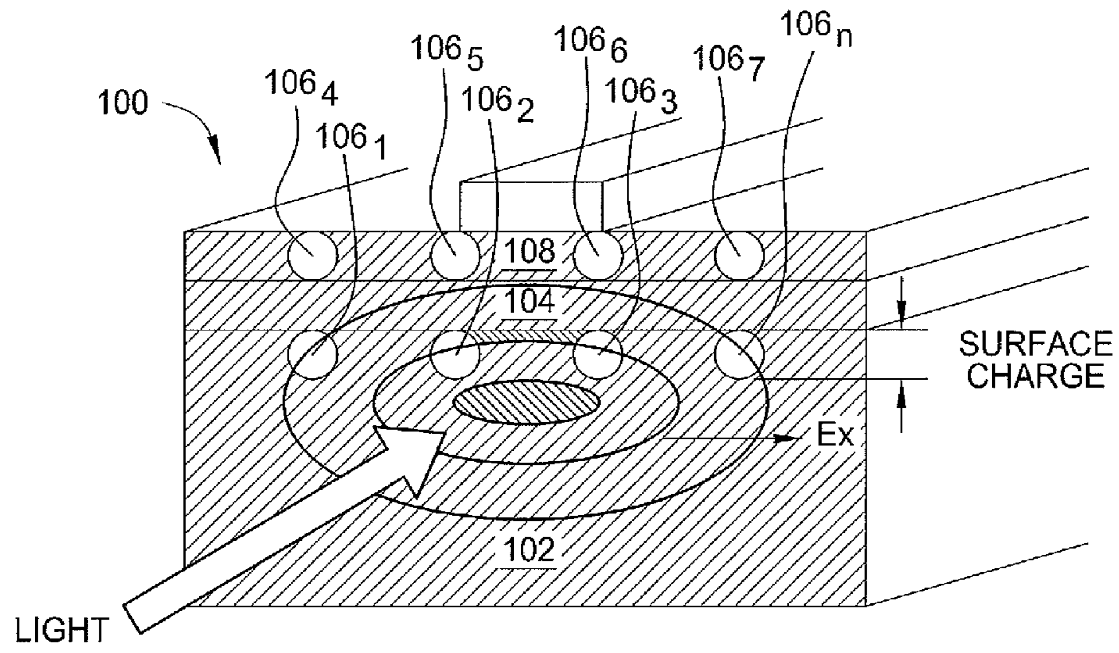
FIG. 1 (PRIOR ART)
